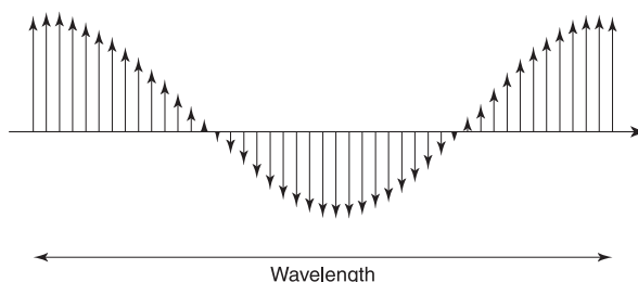
Figure 1 Representation of a ray of electromagnetic radiation traveling through space, left to right. The small vertical arrows represent the strength and direction of the electric field component of the radiation at discrete locations (the magnetic field behaves in an analogous manner). The disturbance is periodic, with the distance between field components of identical strength and direction being the wavelength of the radiation.
