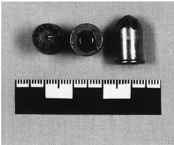
Figure 3 Blank ammunition for captive-bolt stunners. Cattle-killing cartridges RWS 9 × 17 mm; the case mouth is sealed by crimping the metal and inserting a wax plug. The strength of the cartridge is designated by a green color marking on the base of the case ('green' meant for small cattle and pigs).
