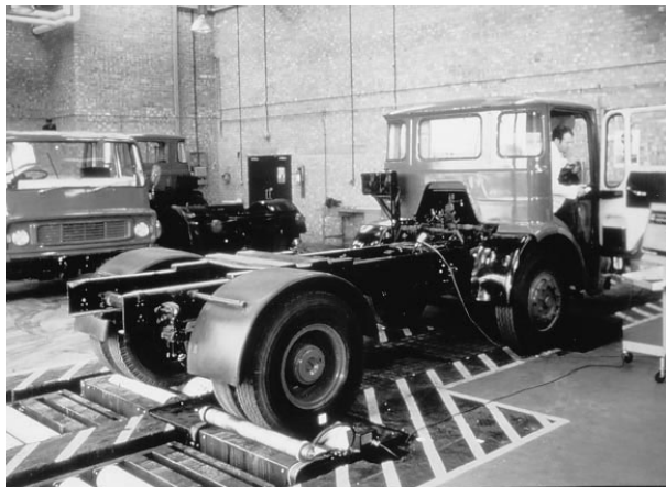
Figure 10 Calibration of a tachograph installation on a Hartridge Rolling Road. (VDO Kienzle (UK) Ltd)
