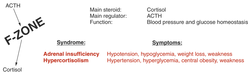
FIGURE 20-8. F-zone disorders.
