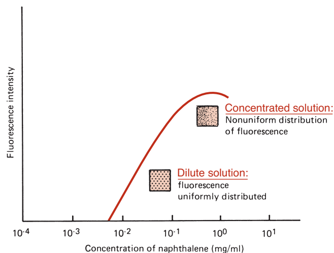
FIGURE 5-14. Dependence of fluorescence on the concentration of fluorophor. (Reprinted with permission from Guilbault GG. Practical fluorescence, theory, methods and techniques. New York, N.Y.: Marcel Dekker, 1973.)
