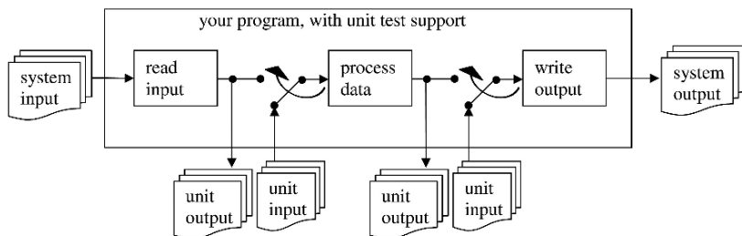
Fig. 2.3 Simple test system with unit test support
