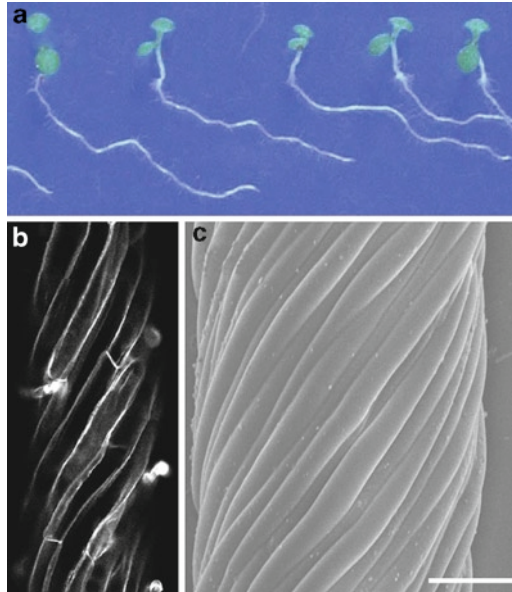
Fig. 11.1 Helical growth in a right-handed twisting mutant, spiral 3 . This mutant is caused by an amino-acid missense mutation in the GCP2 subunit of the \gamma -tubulin nucleating complex, and results in wider and more divergent nucleating angles of newly formed MTs with respect to the wall of previously existing MTs. (a) Seedlings grown on a hard agar surface. Primary roots grow toward the right side of the plate when viewed from above. (b) Epidermal cell files of the mutant roots (stained with propidium iodide) twist to form right-handed helices at the differentiated region. Root hairs are stained intensely. (c) Epidermal cell files of the etiolated mutant hypocotyls (viewed with scanning electron microscopy) also form right-handed helices. Bar: 100 \mu m
