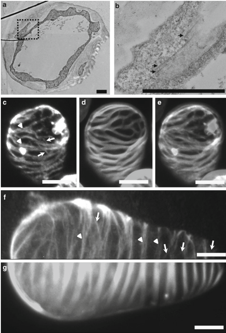
Fig. 13.3 Microtubules in plant tracheary elements. (a, b) TEM images of microtubules relative to the secondary cell wall in in vitro differentiating Arabidopsis TE. Overview of cell morphology (a) and focusing within the boxed area (b) where microtubules are indicated by arrows, bars=700 nm. (c–e) confocal images of immunolocalisation of \alpha -tubulin using YOL 1/34 antibody (c) on Arabidopsis TEs differentiating in vitro compared to the TE secondary cell wall stained with Calcofluor (d) ; the corresponding merged image of both channels is shown in (e) , bars=9 \mu m. (f, g) Confocal images of Arabidopsis TEs differentiating in vitro constitutively expressing \alpha -tubulin-GFP. (f) Shows half of the cell's secondary cell wall stained with GFP and (g) shows the other half stained with Calcofluor. Note the arrows that indicate the interconnecting microtubules and the arrowhead that define the underlying microtubules bundle beneath the secondary thickenings, bars=6 \mu m
