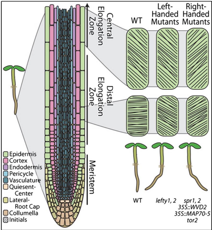
Fig. 14.1 Arabidopsis root tip, cortical microtubule arrangements, and helical growth. A schematic of a longitudinal section of the root tip highlights the different cell types along with the meristem and the distal and central elongation zones. Epidermal cells of the elongation zones are enhanced to show microtubule alignments in these sections for wild-type and selected helical growth mutants
