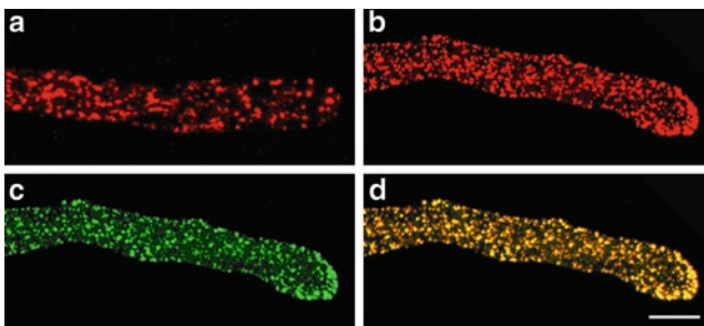
Fig. 3.1 AtVLN4 promotes punctate actin foci formation in tobacco pollens. Actin organization was imaged using rhodamine-phalloidin staining. (a) Actin organization in the control pollen tube; (b) Actin organization in the AtVLN4-GFP transformed tobacco pollen treated with 10 \mu\text{M} A23187 in the presence of 200 \mu\text{M} \text{Ca}^{2+} ; (c) AtVLN4-GFP; (d) Merged image of (b) and (c); Bar = 10 \mu\text{m}
