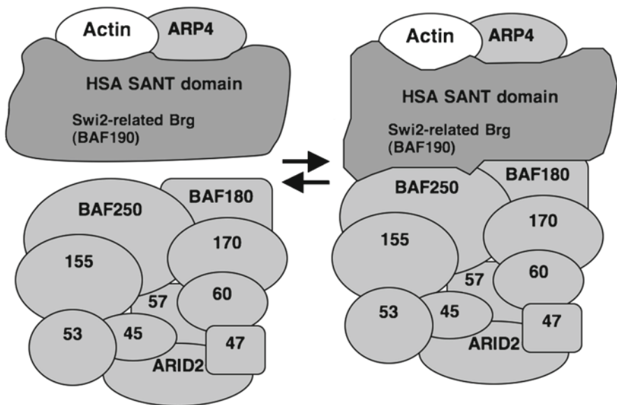
Fig. 1.6 Nuclear ARP4 (Baf53) and actin bind the HSA domain of the Swi2-related Brg DNA dependent ATPase in the mammalian Swi/Snf BRG chromatin remodeling complex. This model illustrates that \beta -actin and ARP4 bind Brg, and then the \beta -actin/ARP4/Brg sub-complex binds to a second sub-complex containing several other Brg proteins to form an active chromatin-remodeling machine [83, 145]. A related model may be proposed for a large number of chromatin-active complexes. Two nuclear ARPs or a nuclear ARP and actin bind as dimmers or heterodimers to the helicase-SANT (HSA) domain of the large Swi2-related DNA dependent ATPase subunit in chromatin remodeling complexes or the Vid21-related helicase subunit in chromatin modifying complexes. Again, the ARP-containing sub-complex then binds a second sub-complex with a larger number of subunits
