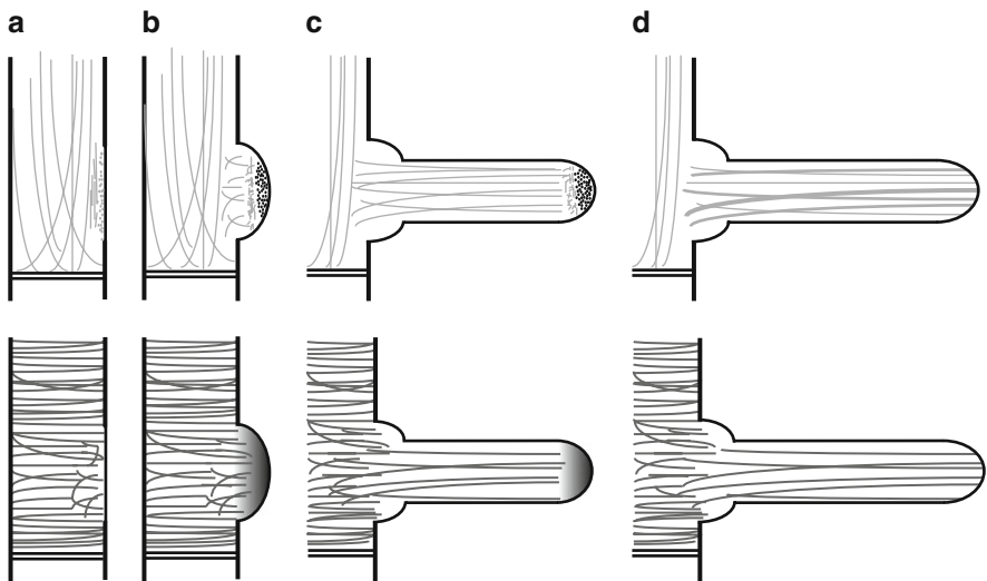
Fig. 12.2 Cellular architecture during root hair development. Schematic representation of root hairs during four stages of root hair development. Upper panels show actin filaments ( grey lines ) and secretory vesicles ( black dots ). Lower panels show microtubules ( darker grey lines ) and the tip-focused calcium gradient ( darker color represents higher calcium concentration). (a) Early events after bulge site selection. Note the fragmentation of actin filaments and the local loss of microtubule organization. (b) Initial outgrowth and bulge formation. Actin filaments begin to form a dense mesh behind the tip region where vesicles accumulate and the calcium gradient forms. (c) Tip growth. Cytoskeletal elements are mostly longitudinal along the shank but do not reach into the apex. Vesicle accumulation and calcium accumulation are maximal at the apex. (d) Fully grown hair. Vesicle accumulation and calcium gradient at the tip disappear and longitudinal actin filaments and microtubules reach into the apex
