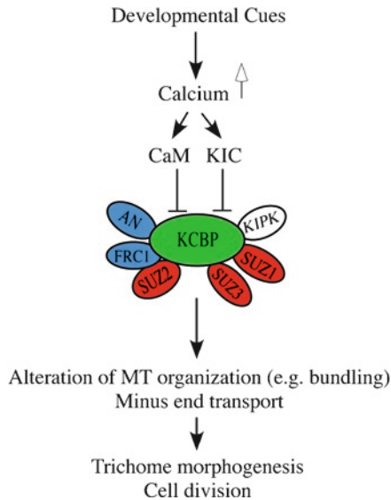
Fig. 6.8 Regulation of KCBP function. A model illustrating how changes in \text{Ca}^{2+} levels regulate trichome morphogenesis and cell division through \text{Ca}^{2+} -sensors, calmodulin (CaM) and KIC, and an MT-based motor, KCBP, in Arabidopsis. Based on the magnitude of changes in \text{Ca}^{2+} levels in trichome cells in response to developmental cues, CaM or KIC can be activated which in turn negatively regulate the microtubule-based motor, KCBP in the trichome morphogenic complex or during cell division. The positive and negative regulation of intermediate components in the pathway is shown with an arrow and a line ending with solid-bar, respectively. Some of the known positive and negative regulators of trichome morphogenesis that interact with KCBP are shown in green and red, respectively. Biochemical and/or genetic analysis show interaction between positive (KCBP and AN/FRC1/KIPK) or between positive and negative (KCBP/SUZ) regulators [12, 23, 34, 50]. KIC KCBP interacting \text{Ca}^{2+} -binding protein; KCBP kinesin-like CaM-binding protein; KIPK kinesin-interacting protein kinase; AN angustifolia; FRC1 furca 1; SUZ suppressor of zwi3 . Adapted from Reddy et al. [50]
