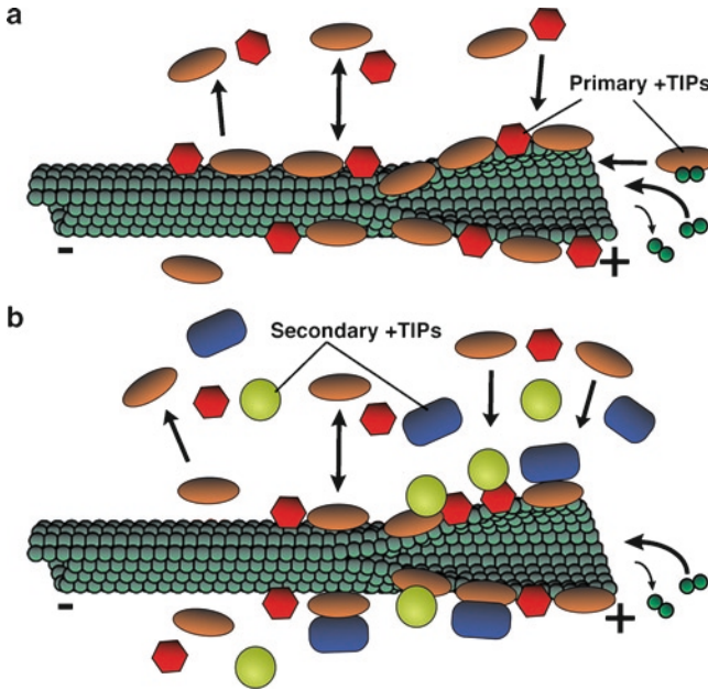
Fig. 5.1 +TIP complex formation on microtubule ends. (a) Primary +TIPs (hexagons and ovals) associate directly with the growing microtubule end. They can reach the microtubule by diffusing through the cytoplasm or by binding tubulin dimers (small circles) and assembling with them as they are incorporated into the growing microtubule. Some +TIPs may also associate with the tubule wall behind the tip and move along the microtubule lattice towards the end by diffusion or motor-driven transport (not shown). Primary +TIPs recognize structural and/or chemical features unique to the plus end. They bind to the end but do not translocate forward with it as it grows through the cytoplasm. Instead they are released from the microtubule when they become associated with the tubule wall. (b) Primary +TIPs (hexagons and ovals) such as EB1 are proposed to function as diffusional sinks for the recruitment of secondary +TIPs to microtubule ends (large circles and boxes). Secondary +TIPs comprise a large and diverse group of proteins that include signalling factors, regulators of the actin cytoskeleton, and proteins that mediate interactions with other structures in the cell. Together these +TIP families form a dynamic network of proteins that can be modified and changed depending on the needs of the cell. For simplicity only two secondary +TIPs are depicted here
