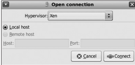
Figure 7-21. Starting the virt-manager GUI
