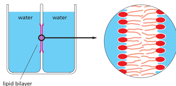
lipid bilayer
