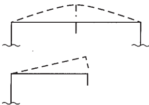
Figure 7.16 Assumed failure mode for reinforced elements.
