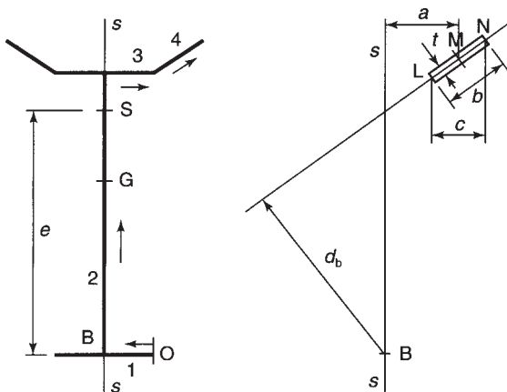
Figure 10.19 Monosymmetric section, type 2.
