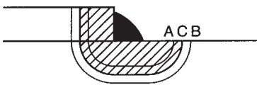
Figure 6.9 Extent of nominal HAZ (line C) for thick plate.
