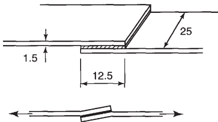
Figure 11.13 Adhesive lap shear test. Standard specimen.
