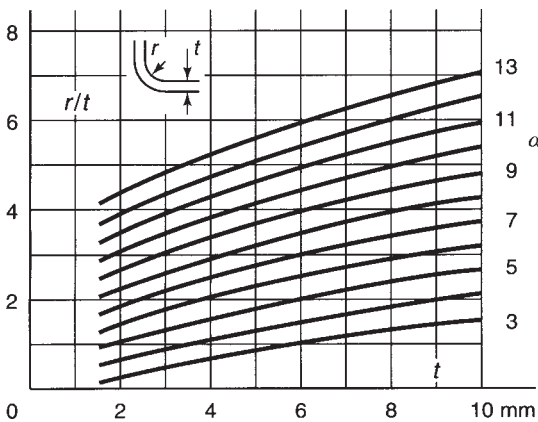
Figure 4.5 Approximate variation of minimum r/t with t for 90^\circ bends in flat material. Values of the bendability index \alpha are listed in Table 4.6 .
