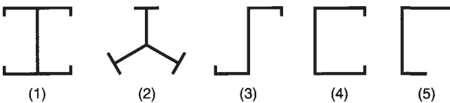
Figure 9.5 Degrees of symmetry for strut sections: (1) bisymmetric; (2) radial-symmetric; (3) skew-symmetric; (4) monosymmetric; (5) asymmetric.
