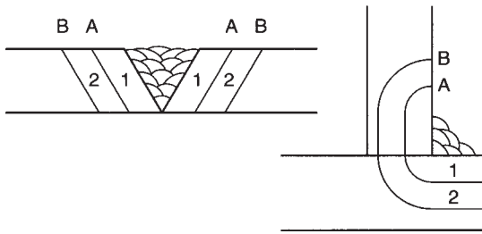
Figure 6.5 Pattern of softening at multi-pass weld on thick material.
