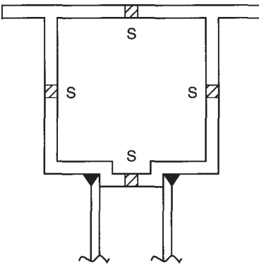
Figure 2.7 Seam welds (S) in a hollow profile.
