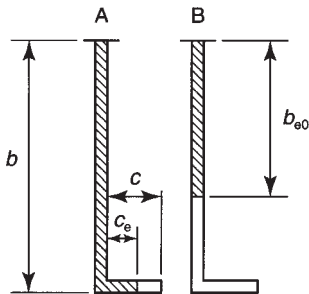
Figure 7.21 Slender reinforced outsands, effective area.
