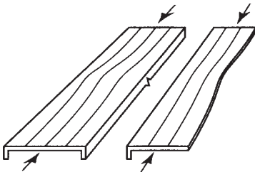
Figure 7.1 Local buckling.
