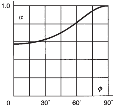
Figure 11.9 Variation of \alpha with \phi (equation (11.16)).
