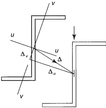
Figure 8.26 Components of deflection for asymmetric bending.
