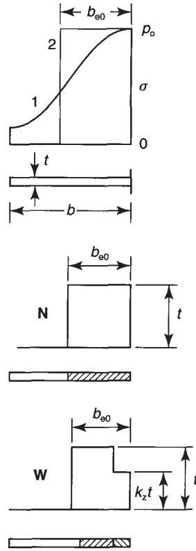
Figure 7.5 Slender outstand. Stress-pattern at failure, and assumed effective section. N=non-welded, W=with edge-welds.
