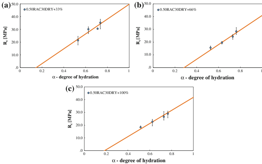
Fig. 7.27 Results of the validation
