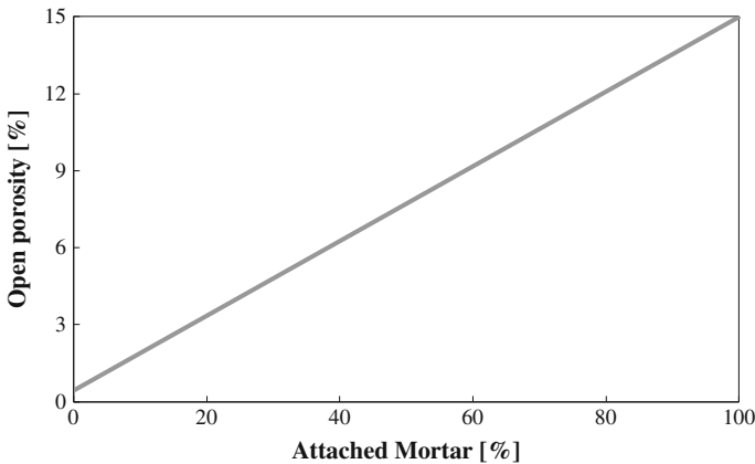
Fig. 8.3 Typical correlation between open porosity and attached mortar
