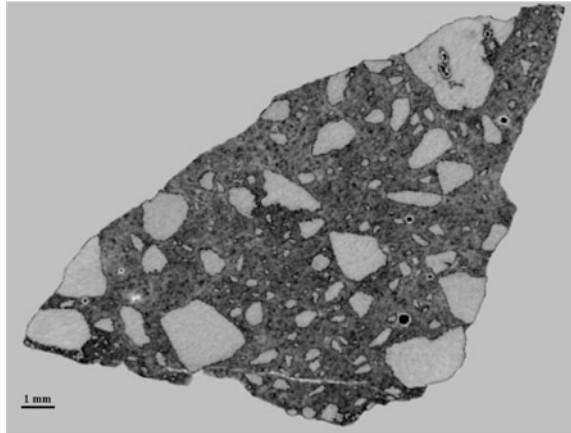
Fig. 4.3 Mesoscopic view of a recycled concrete coarse aggregate
