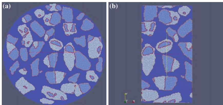
Fig. 7.13 Triangular mesh discretisation for RAC lattice simulation
