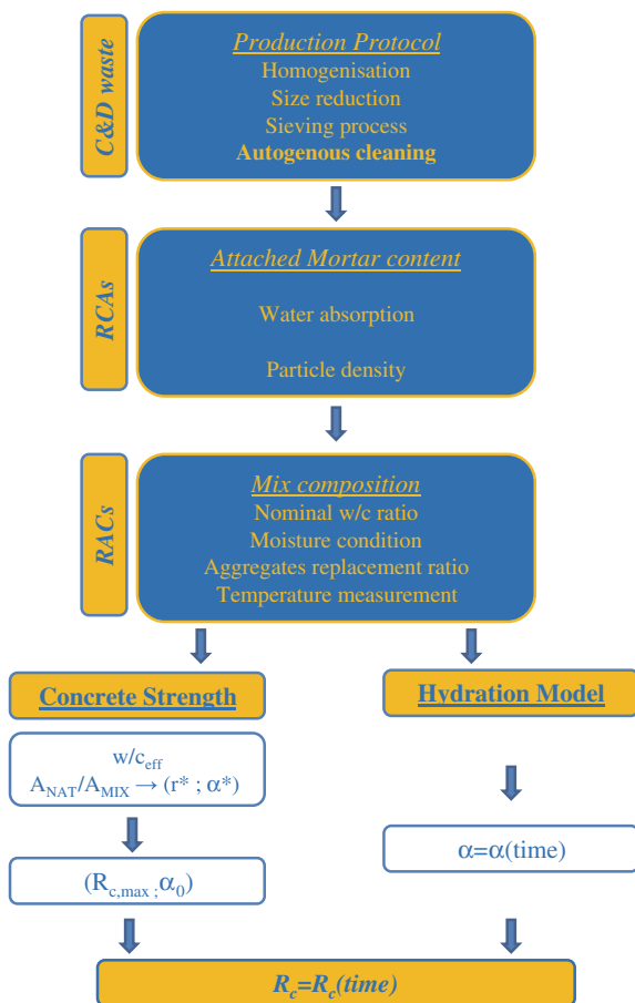
Fig. 8.1 Flow chart of the conceptual model for RACs
