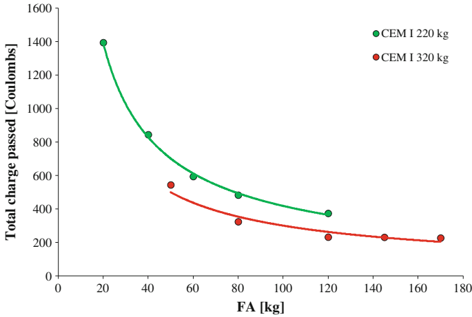
Fig. 6.5 Relation between chloride ion penetrability and fly ash content in concrete mixture (Valente et al. 2011)
