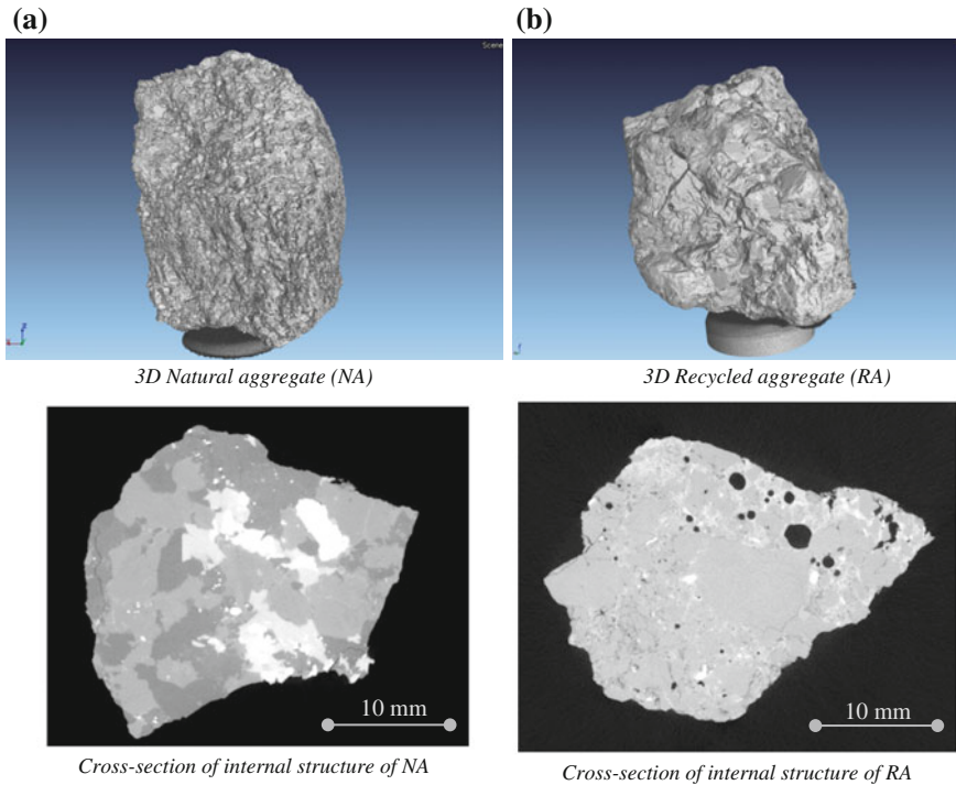
Fig. 4.2 3D scanner analysis of aggregates: a Natural. b Recycled
