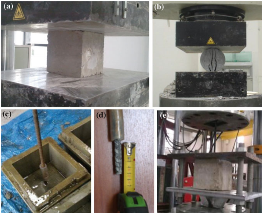
Fig. 6.6 Specimens for investigating mechanical properties of RAC
