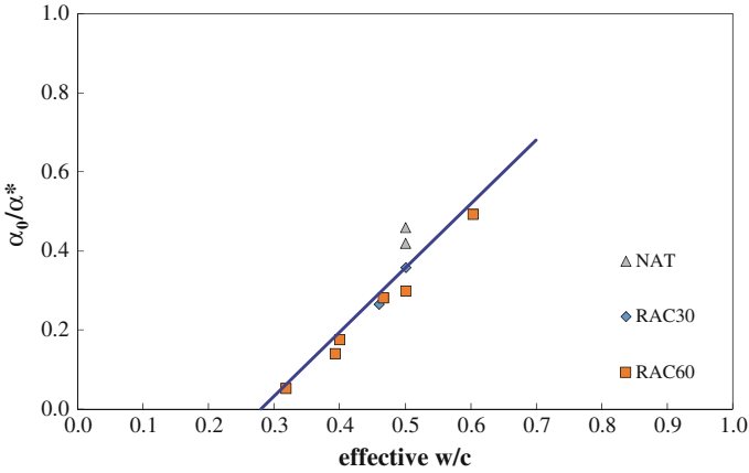
Fig. 7.26 Proposed formulation for \alpha_0
