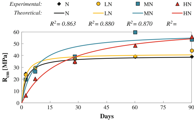
Fig. 6.16 Time evolution of the compressive strength for NAC
