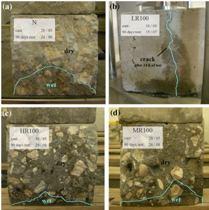
Fig. 6.13 Wet profiles derived by permeability tests: a N mixture. b LR100 mixture. c HR100 mixture. d MR100 mixture
