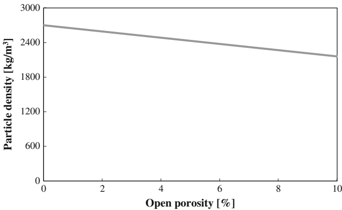
Fig. 8.5 Typical correlation between open porosity and particle density
