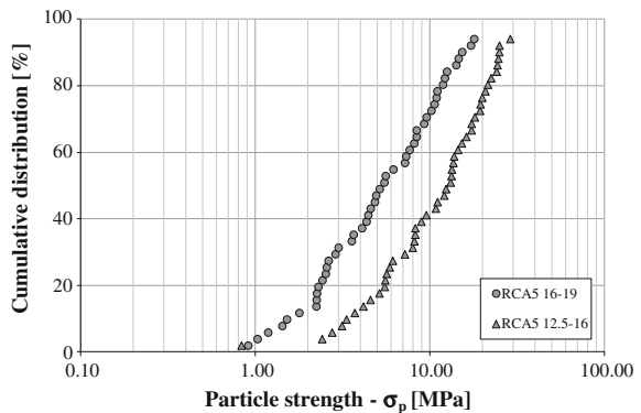
Fig. 4.11 Particle strength, recycled concrete aggregates: influence of nominal diameter
