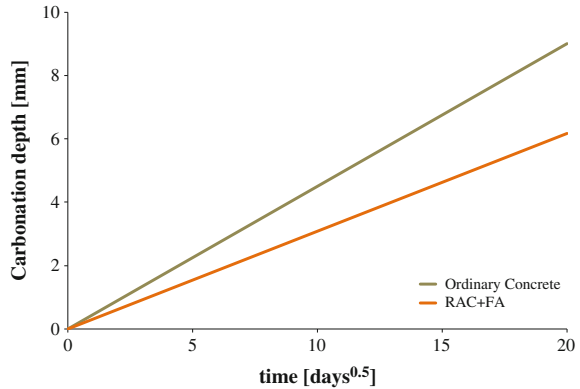
Fig. 6.3 Carbonation depth for ordinary concrete and RAC+FA, as function of time of exposure (Corinaldesi and Moriconi 2009)
