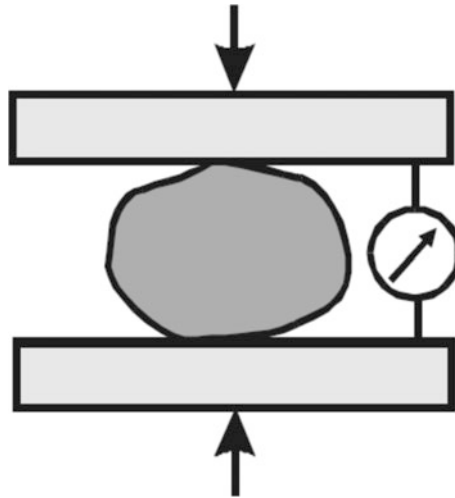
Fig. 4.7 Compressive strength test on single particles (Tavares 2007)
