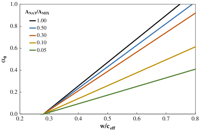
Fig. 8.7 Influence of A_{NAT}/A_{MIX} on \alpha_0
