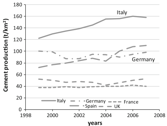
Fig. 2.8 Cement production per km 2 in Europe (AITEC 2011)
