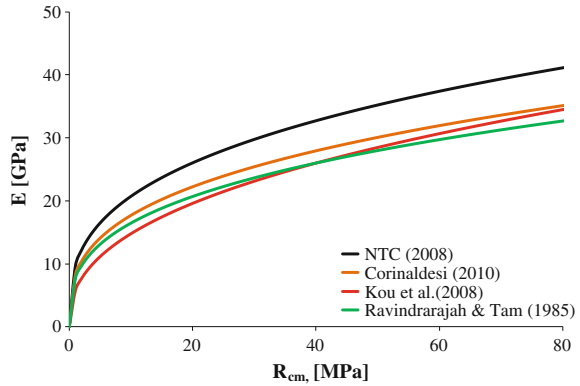
Fig. 5.5 Relation between 28 days compressive strength and static elastic modulus
