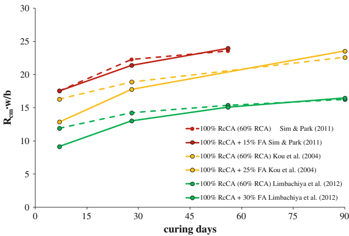
Fig. 6.1 Compressive strength development using class F fly ash as partial Portland cement for concrete with 100 % RcCA
