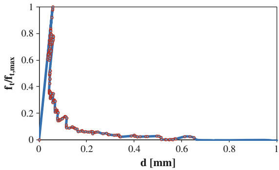
Fig. 7.15 Lattice model simulation, results of direct tensile strength test
