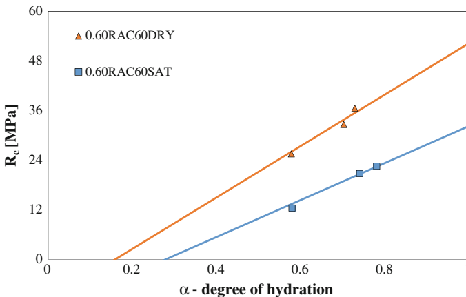
Fig. 7.20 Degree of hydration-Compressive strength
