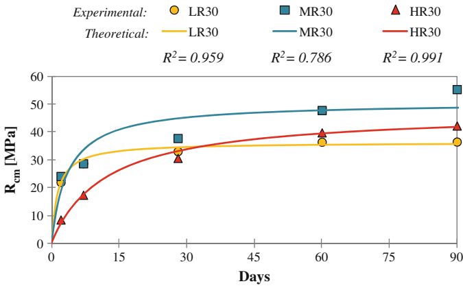
Fig. 6.17 Time evolution of the compressive strength for RAC30
