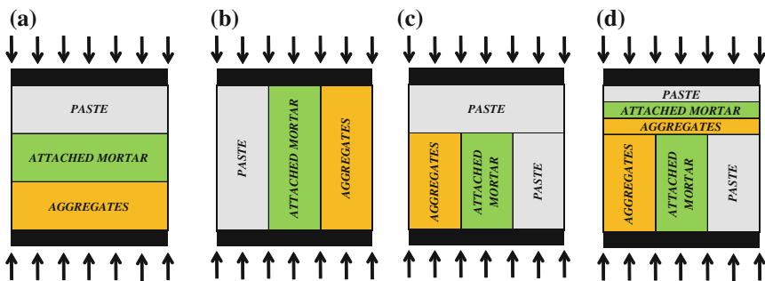
Fig. 8.11 Composite models for RACs. a Series model. b Parallel model. c Counto’s model. d Hirsch’s model
