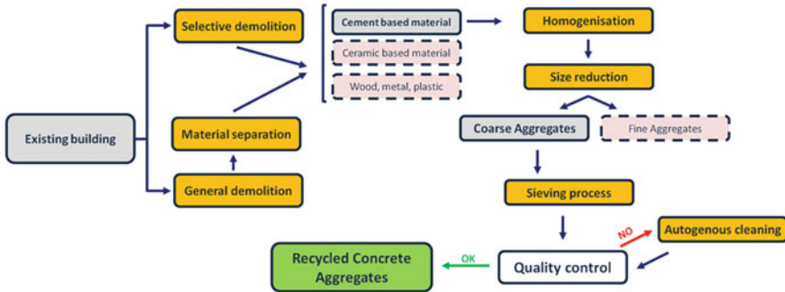
Fig. 8.2 Schematic representation of the production protocol
