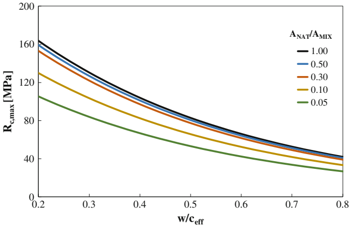
Fig. 8.6 Influence of A_{NAT}/A_{MIX} on R_{c,max}
