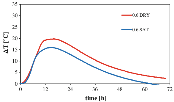
Fig. 5.14 Time evolution of temperature on curing concrete samples (w/c = 0.60)
