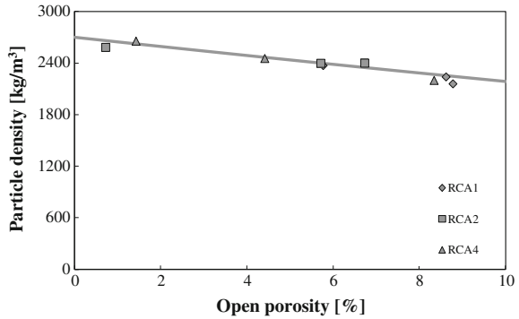
Fig. 4.6 Experimental values of particle density of RCA depending of the open porosity
