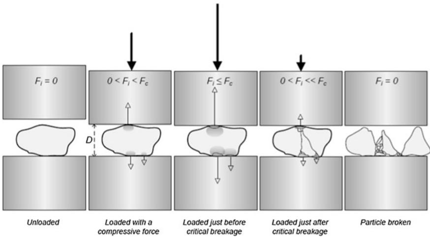
Fig. 4.8 Schematic illustration of the different phases during a single particle compressive strength test (Quist 2012)
