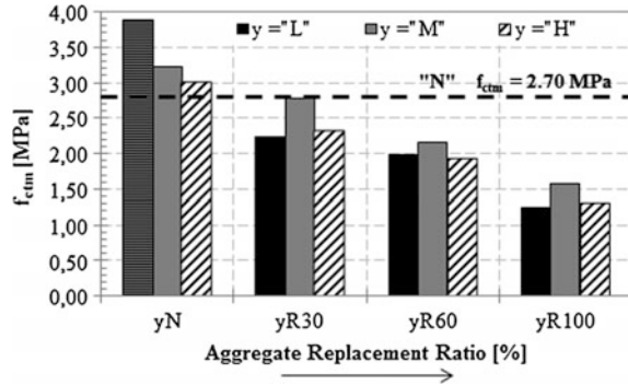
Fig. 6.11 Tensile strength of concrete mixes
