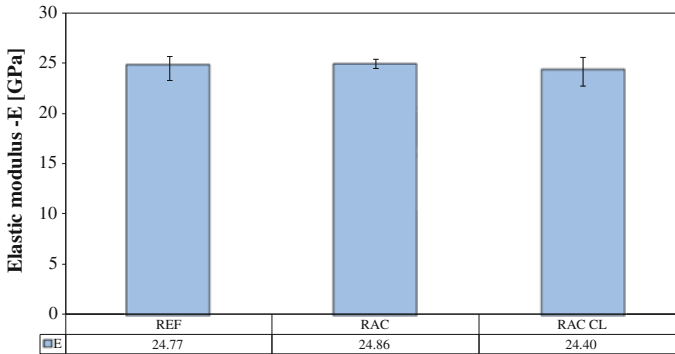
Fig. 5.8 Elastic modulus
