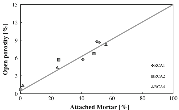
Fig. 4.4 Experimental values of open porosity depending on attached mortar of RCA
