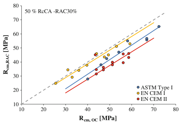
Fig. 5.4 Relation between 28 days compressive strength for RAC with 50 % of RcCA (30 % RCA) and corresponding strength of ordinary concrete (OC)
