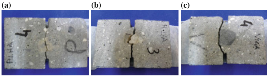
Fig. 4.16 Failure mechanisms for bond strength test. a AM. b ITZ AM-NA. c ITZ Agg.-Paste
