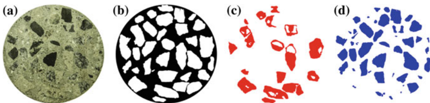
Fig. 7.12 Lattice model simulation, introduction of heterogeneity. b CP. c AM. d NA
