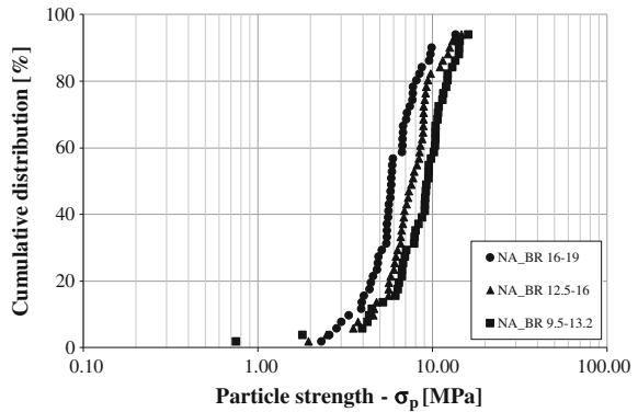
Fig. 4.10 Particle strength, natural aggregates: influence of nominal diameter
