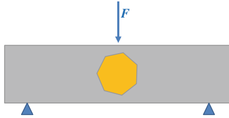
Fig. 4.14 Bond strength test on single particles
