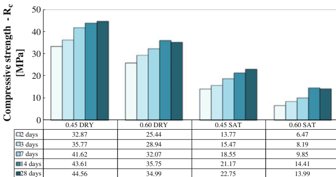
Fig. 5.15 Time evolution of the average compressive strength on concrete samples
