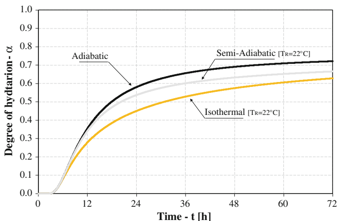
Fig. 7.19 Time evolution of the degree of hydration with different curing boundary conditions
