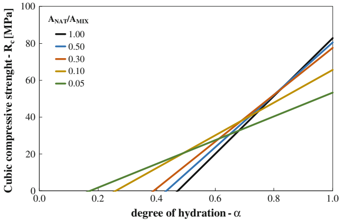
Fig. 8.8 Influence of A_{NAT}/A_{MIX} on cubic compressive strength evolution
