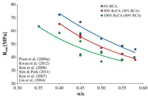
Fig. 5.3 28 days compressive strength for RCA with ASTM Portland cement Type I versus effective w/c ratio, at different RcCA percentage
