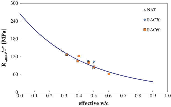
Fig. 7.25 Proposed formulation for R_{c,max}
