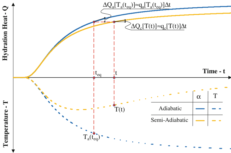
Fig. 7.18 Hydration heat produced and temperature developed in adiabatic and non-adiabatic conditions
