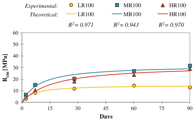
Fig. 6.19 Time evolution of the compressive strength for RAC100
