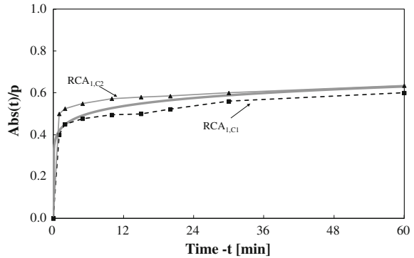
Fig. 4.5 Experimental measurements of water absorption rate for different aggregates
