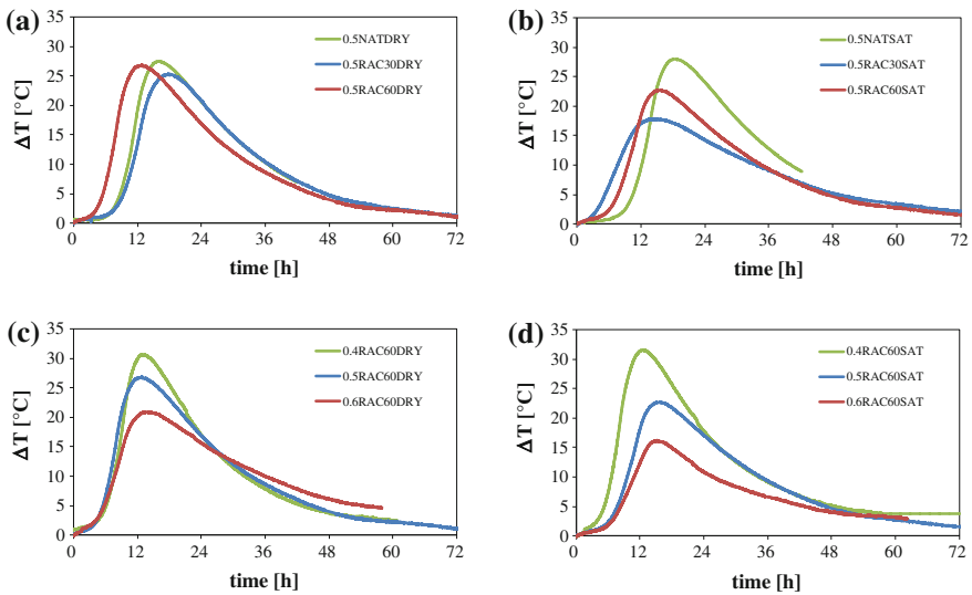
Fig. 5.18 Temperature-time evolution. a the role of RCA amount for DRY mixtures. b the role of RCA amount for SAT mixtures. c the role of w/c ratio for DRY mixtures. d the role of w/c ratio for SAT mixtures
