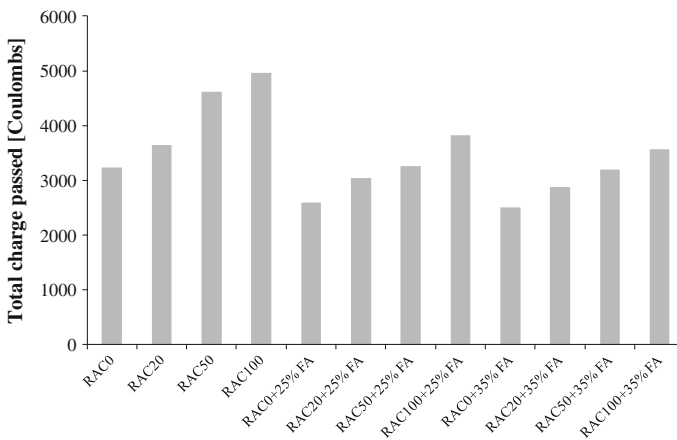
Fig. 6.4 Chloride ion penetrability described in total charge passed measured at different percentage of fly ash after 28 days of curing (Kou et al. 2007)
