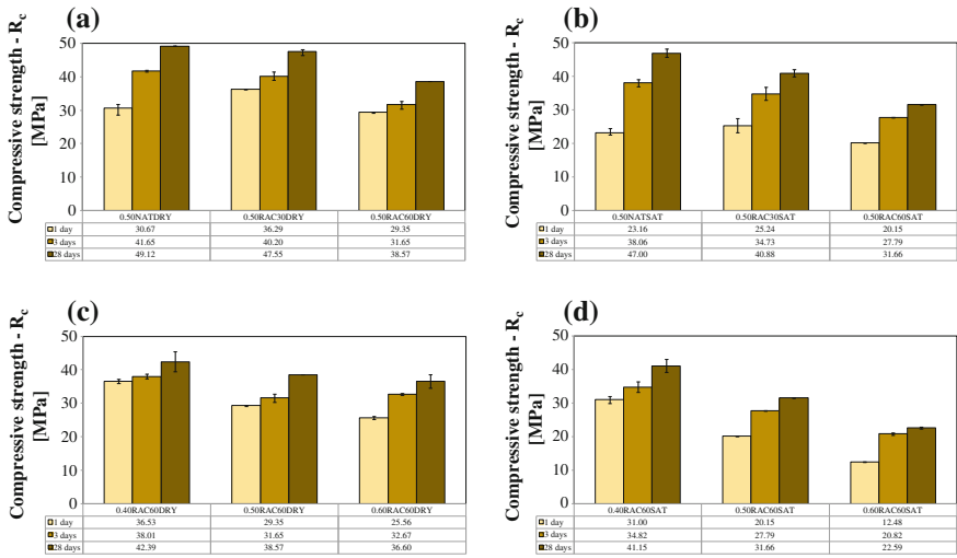
Fig. 5.17 Compressive strength time-evolution. a the role of RCA amount for DRY mixtures. b the role of RCA amount for SAT mixtures. c the role of w/c ratio for DRY mixtures. d the role of w/c ratio for SAT mixtures
