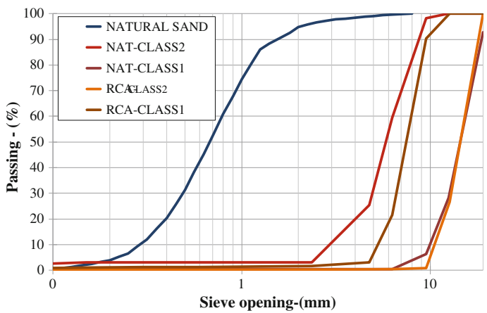
Fig. 7.7 Grain size distribution as input for CPM
