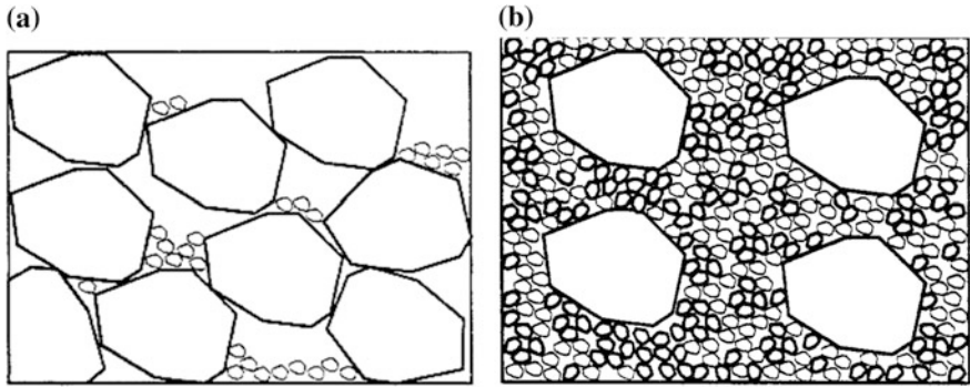
Fig. 7.2 Binary mixture without interaction, Coarse (a) and fine (b) grains dominant (de Larrard 1999)
