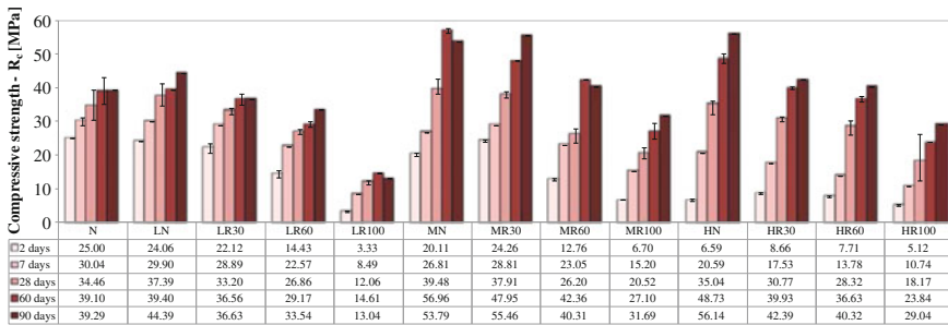
Fig. 6.10 Cube compressive strength of concrete for each curing time
