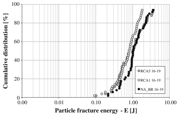
Fig. 4.13 Particle fracture energy: influence of aggregates source
