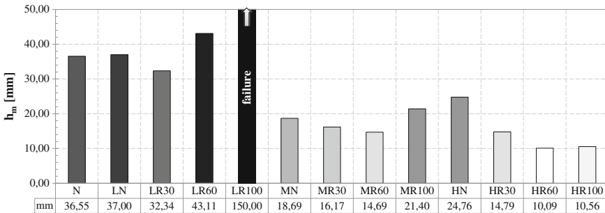
Fig. 6.14 Results of permeability tests
