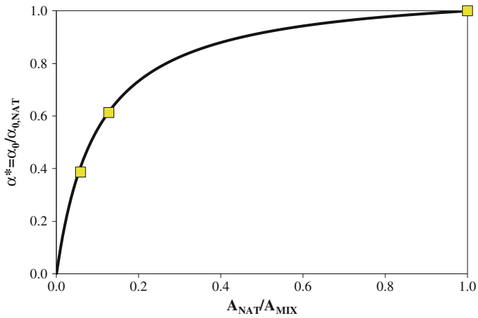
Fig. 7.24 Proposed formulation for \alpha^*
