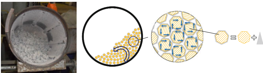
Fig. 4.20 Autogenous cleaning process
