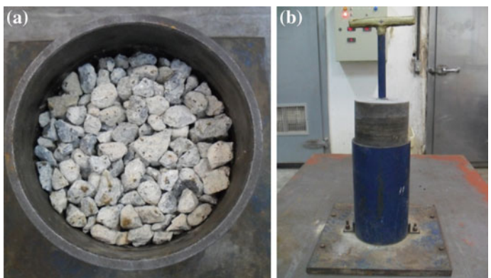
Fig. 7.8 Determination of the compaction index
