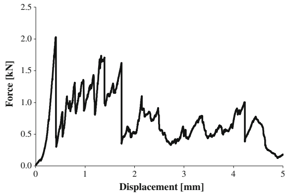
Fig. 4.9 Typical force-deformation diagram from single particle compressive strength test
