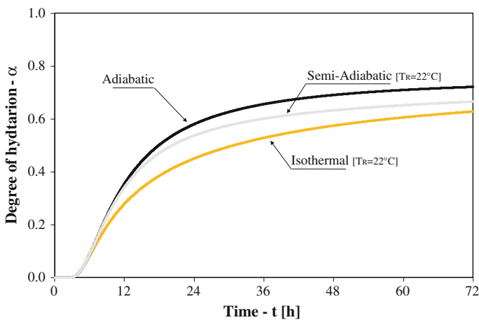
Fig. 8.9 Time evolution of the degree of hydration
