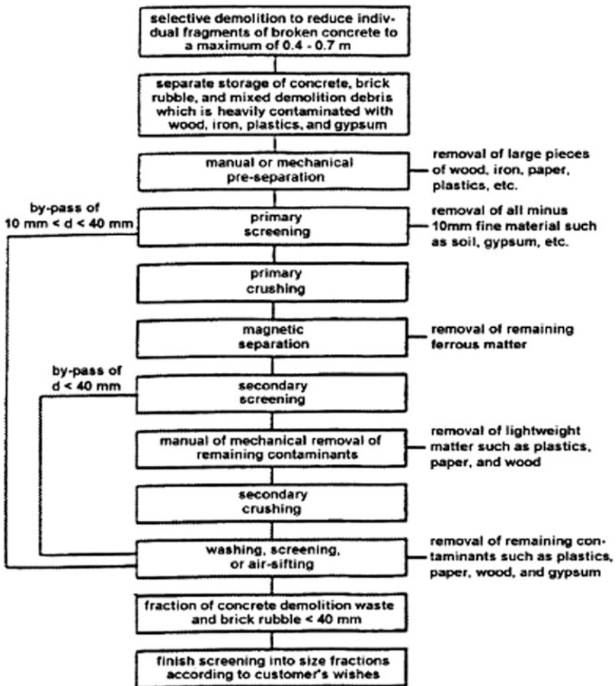
Fig. 3.1 Processing procedure for building and demolition waste (ACI 555R-01 2001)
