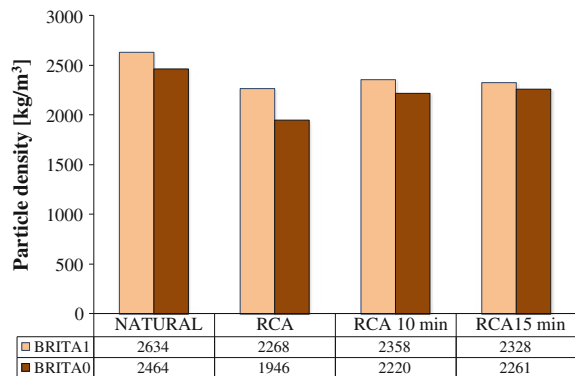
Fig. 4.22 Particle density
