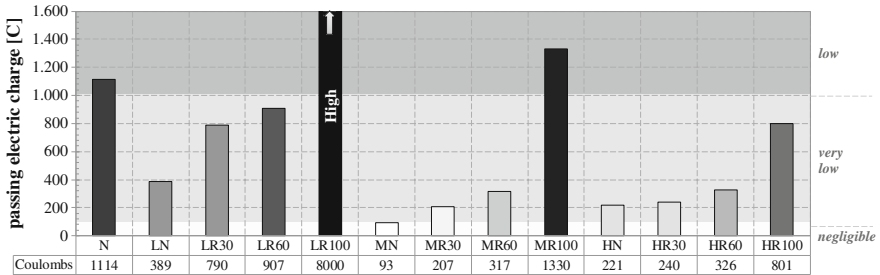
Fig. 6.15 Results of chloride diffusion tests
