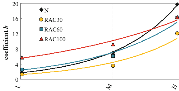
Fig. 6.21 Values of the b coefficient vs. the content of FA in concrete mixes
