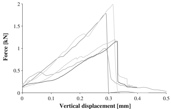
Fig. 4.15 Typical force-deformation diagram from singular particle bond strength test
