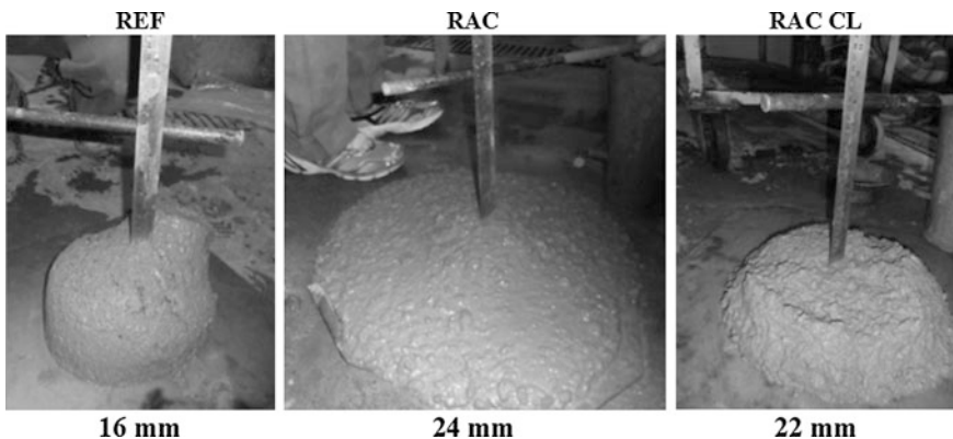
Fig. 5.6 Slump test results
