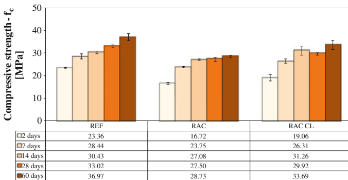
Fig. 5.7 Compressive strength results
