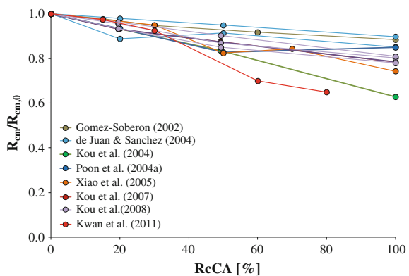
Fig. 5.2 Compressive strength reduction at 28 days compared to ordinary concrete, due to the increase of RcCA replacement percentage
