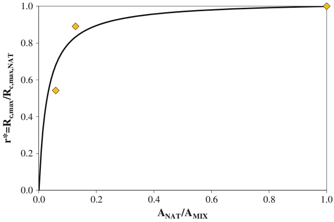
Fig. 7.23 Proposed formulation for r^*
