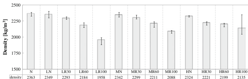
Fig. 6.9 Density of the concrete samples
