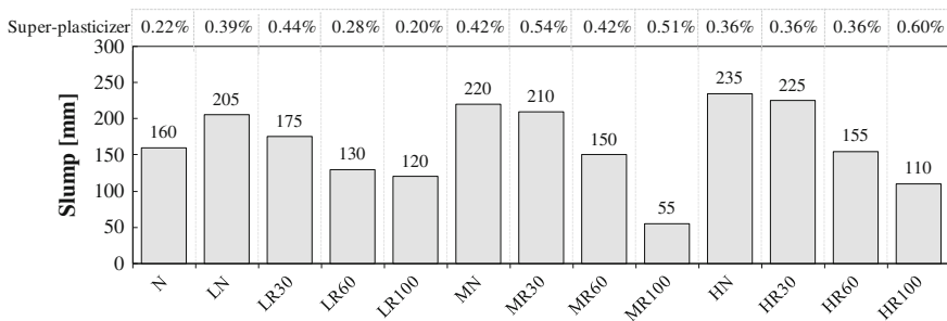
Fig. 6.8 Results of the slump tests
