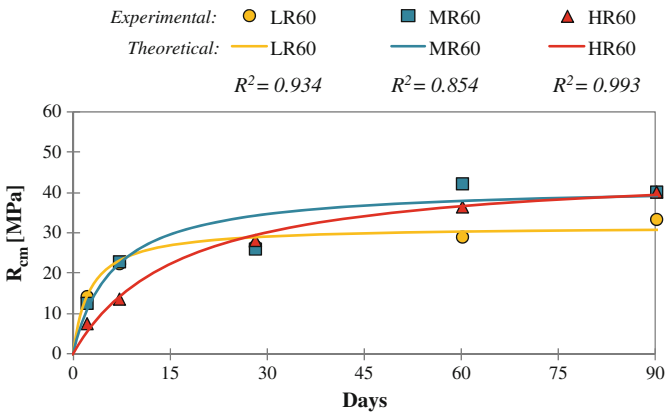
Fig. 6.18 Time evolution of the compressive strength for RAC60
