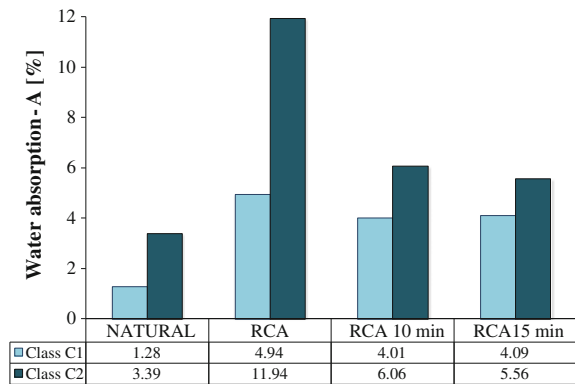
Fig. 4.21 Water absorption at 24 h of aggregates
