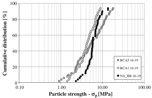
Fig. 4.12 Particle strength: influence of aggregates source
