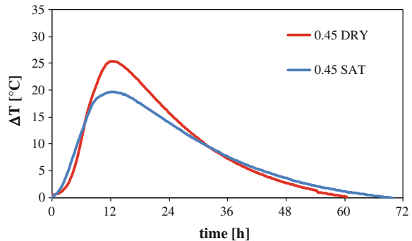
Fig. 5.13 Time evolution of temperature on curing concrete samples ( w/c = 0.45 )
