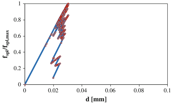
Fig. 7.14 Lattice model simulation, results of splitting test
