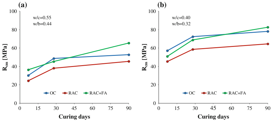
Fig. 6.2 Compressive strength development using class F fly ash in addition to Portland cement for concrete with 100 % RcCA, at different w/b ratio (Kou et al. 2008)
