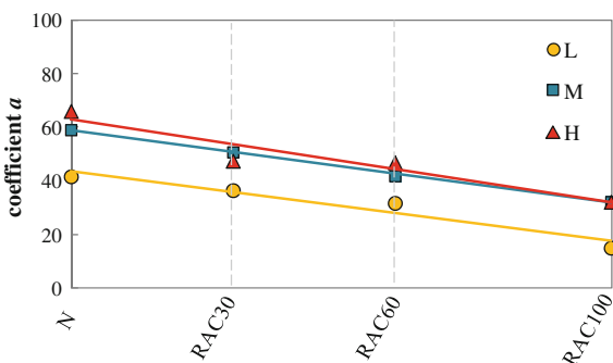
Fig. 6.20 Values of the a coefficient vs. the content of RCA in concrete mixes
