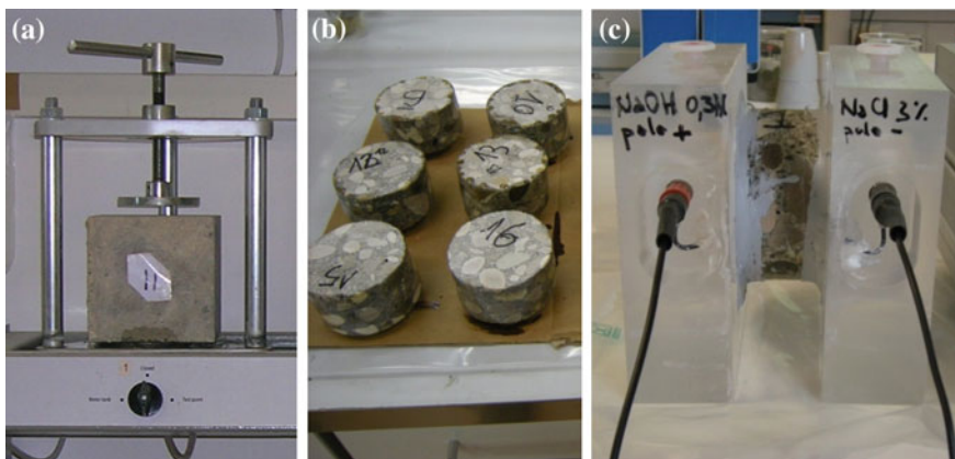
Fig. 6.7 Specimens for investigating the durability properties of the considered concretes
