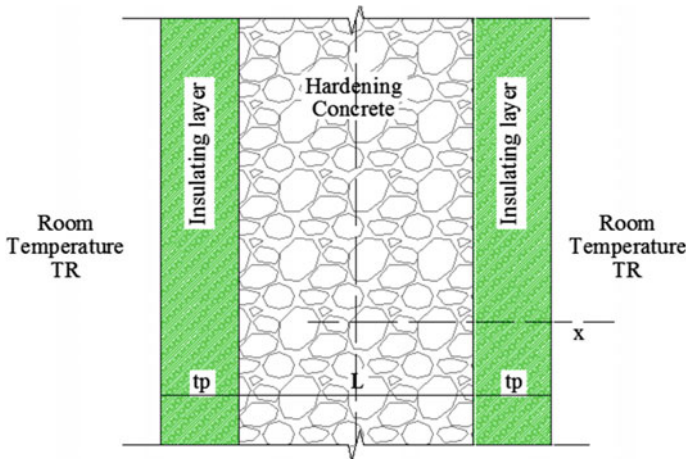
Fig. 7.17 Geometrical description of the 1D problem
