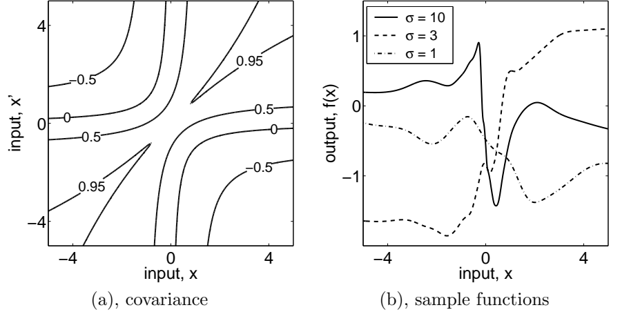
Figure 4.5: Panel (a): a plot of the covariance function k_{\text{NN}}(x, x') for \sigma_0 = 10 , \sigma = 10 . Panel (b): samples drawn from the neural network covariance function with \sigma_0 = 2 and \sigma as shown in the legend. The samples were obtained using a discretization of the x -axis of 500 equally-spaced points.
