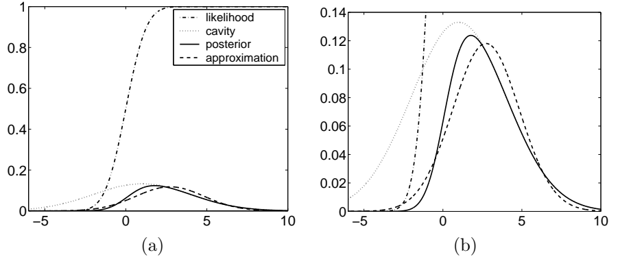
Figure 3.4: Approximating a single likelihood term by a Gaussian. Panel (a) dash-dotted: the exact likelihood, \Phi(f_i) (the corresponding target being y_i = 1 ) as a function of the latent f_i , dotted: Gaussian cavity distribution \mathcal{N}(f_i|\mu_{-i}=1, \sigma_{-i}^2=9) , solid: posterior, dashed: posterior approximation. Panel (b) shows an enlargement of panel (a).
