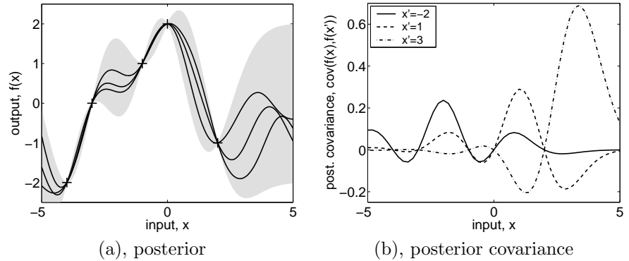
Figure 2.4: Panel (a) is identical to Figure 2.2(b) showing three random functions drawn from the posterior. Panel (b) shows the posterior co -variance between f(\mathbf{x}) and f(\mathbf{x}') for the same data for three different values of \mathbf{x}' . Note, that the covariance at close points is high, falling to zero at the training points (where there is no variance, since it is a noise-free process), then becomes negative, etc. This happens because if the smooth function happens to be less than the mean on one side of the data point, it tends to exceed the mean on the other side, causing a reversal of the sign of the covariance at the data points. Note for contrast that the prior covariance is simply of Gaussian shape and never negative.
