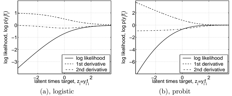
Figure 3.3: The log likelihood and its derivatives for a single case as a function of z_i = y_i f_i , for (a) the logistic, and (b) the cumulative Gaussian likelihood. The two likelihood functions are fairly similar, the main qualitative difference being that for large negative arguments the log logistic behaves linearly whereas the log cumulative Gaussian has a quadratic penalty. Both likelihoods are log concave.
