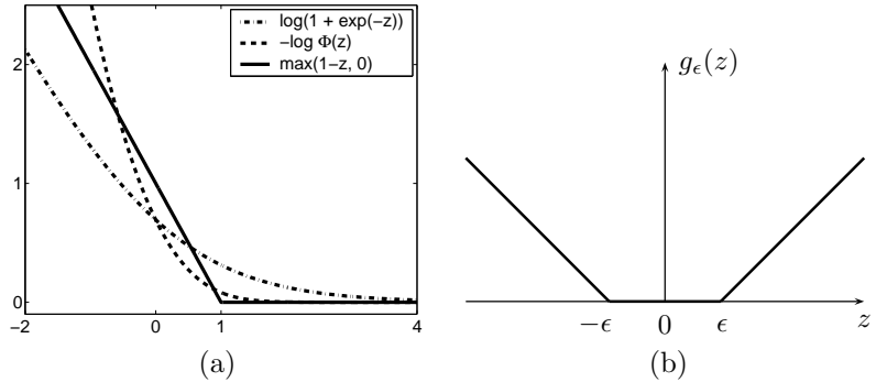
Figure 6.3: (a) A comparison of the hinge error, g_\lambda and g_\Phi . (b) The \epsilon -insensitive error function used in SVR.
