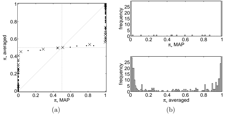
Figure 3.9: MAP vs. averaged predictions for the EP algorithm for the 3’s vs. 5’s digit discrimination using the USPS data. The optimal values of the hyperparameters from Figure 3.7(a) \log(\ell) = 2.6 and \log(\sigma_f) = 4.1 are used. The MAP predictions \sigma(\mathbb{E}_q[f_*|\mathbf{y}]) are “hard”, mostly being very close to zero or one. On the other hand, the averaged predictions \mathbb{E}_q[\pi_*|\mathbf{y}] from eq. (3.25) are a lot less extreme. In panel (a) the 21 cases that were misclassified are indicated by crosses (correctly classified cases are shown by points). Note that only 4 of the 21 misclassified points have confident predictions (i.e. outside [0.1, 0.9] ). Notice that all points fall in the triangles below and above the horizontal line, confirming that averaging does not change the “most probable” class, and that it always makes the probabilities less extreme (i.e. closer to 1/2 ). Panel (b) shows histograms of averaged and MAP predictions, where we have truncated values over 30.
