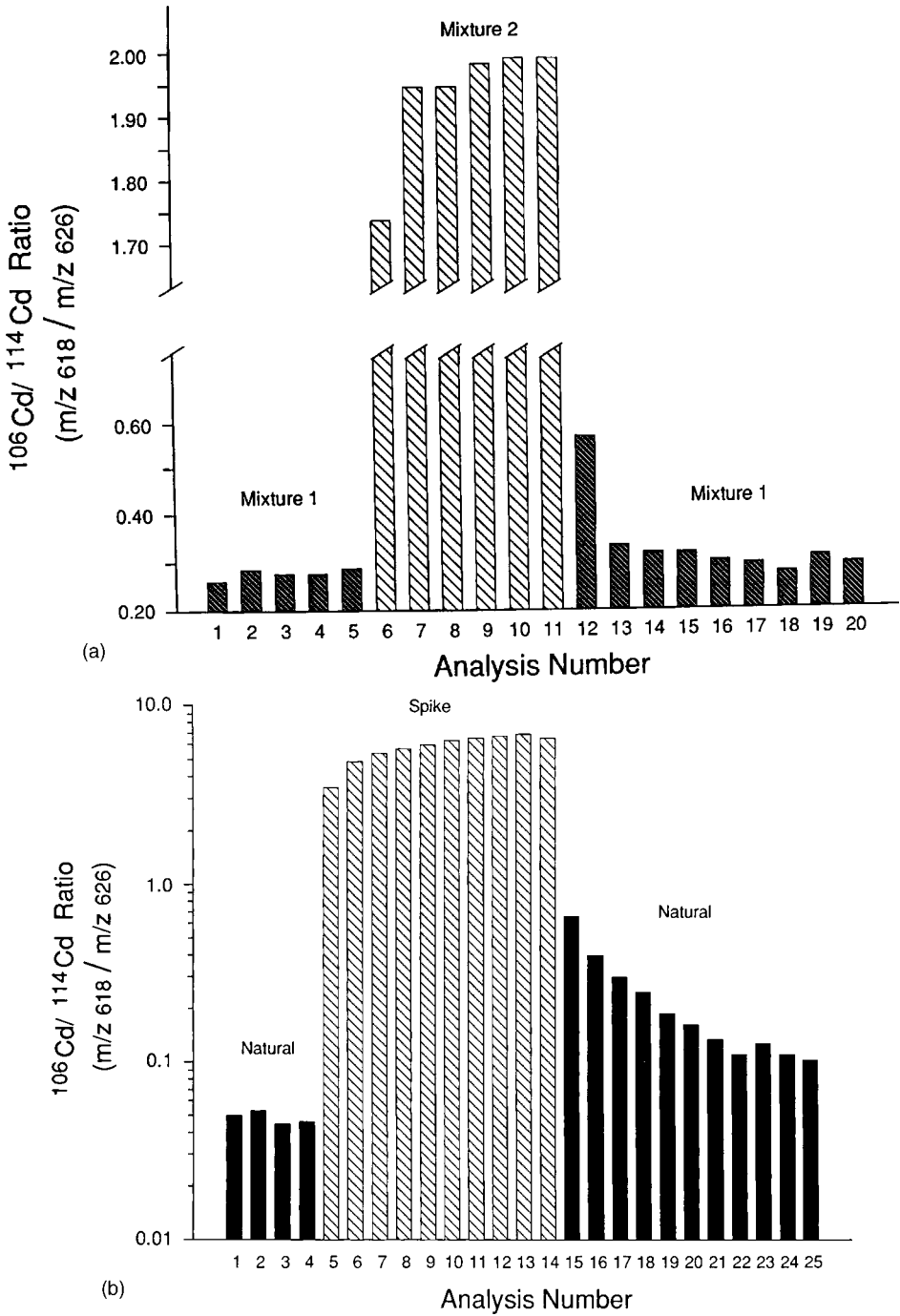
Figure 13.2 (a) Evaluation of cross-contamination in consecutive analyses of two Cd(FDEDTC) 2 samples with isotope ratio differing by a factor of ~10 (Ref. 8). (b) Evaluation of cross-contamination of consecutive analyses of two Cd(FDEDTC) 2 samples with isotope ratio differing by a factor of ~200 (Ref. 8)
