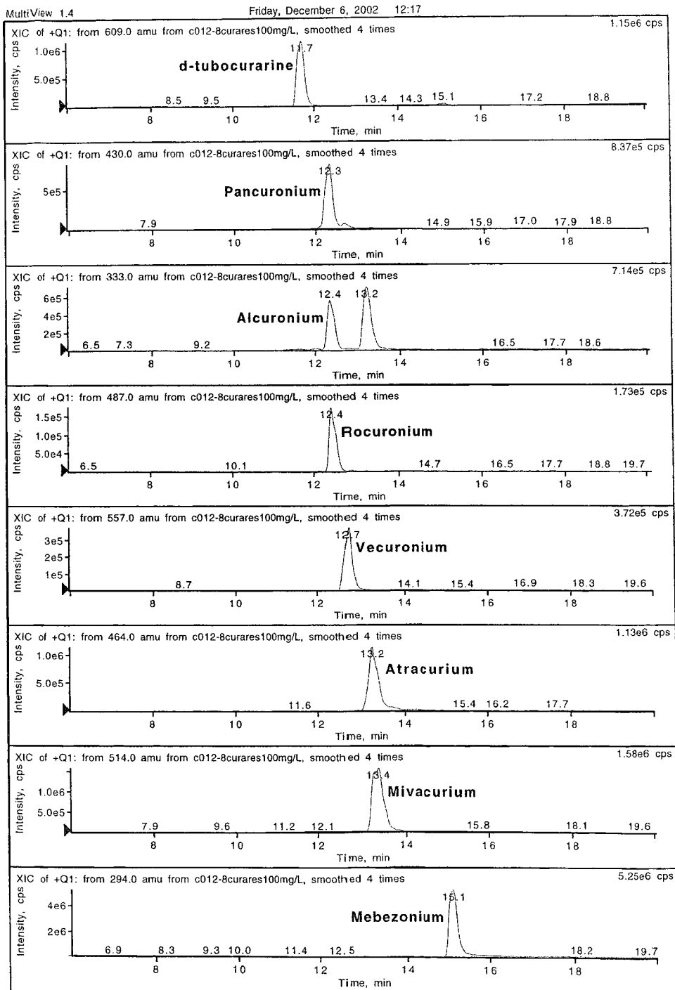
Figure 10.2 Typical chromatographic profiles for the eight quaternary muscle relaxants. Reprinted from Journal of Chromatography B , 789 , V. Cirimele, M. Villain, E. Pépin, B. Ludes and P. Kintz, Screening procedure for eight quaternary nitrogen muscle relaxants in blood by high-performance liquid chromatography–electrospray ionization mass spectrometry, 107–113, with permission from Elsevier
