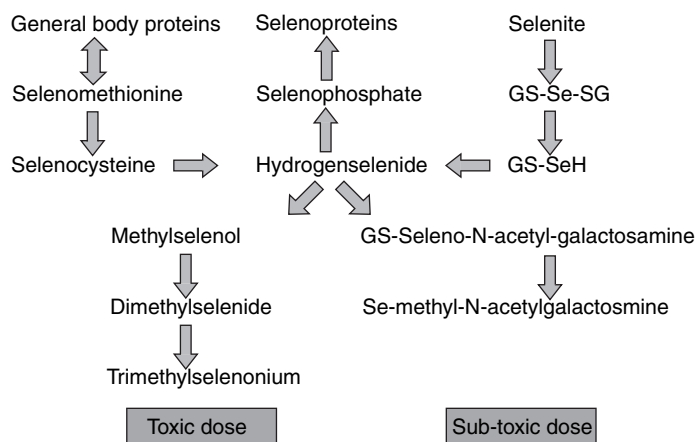
Figure 12.4 The proposed selenium metabolism (GS-: glutathione conjugate). From Gammelgaard, B., Bendahl, L. Selenium speciation in human urine samples by LC- and CE-ICP-MS separation and identification of selenosugars. J. Anal. At. Spectrom. 2004, 19 , 135–142. Reproduced by permission of The Royal Society of Chemistry
