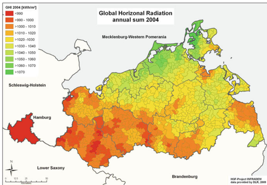
Fig. 8.8 Irradiation conditions for the year 2004 (total annual global radiation [ \text{kWh/m}^2 ]) (Source: DLR)
