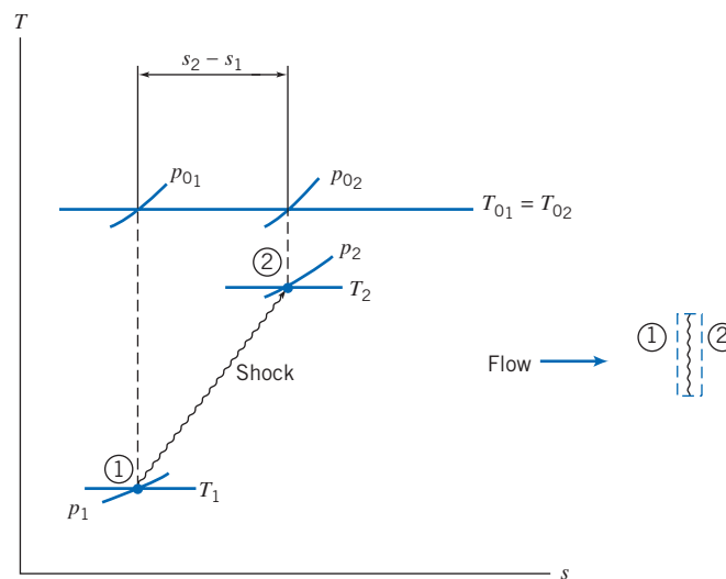
Fig. 13.10 Schematic of normal-shock process on the Ts plane.
