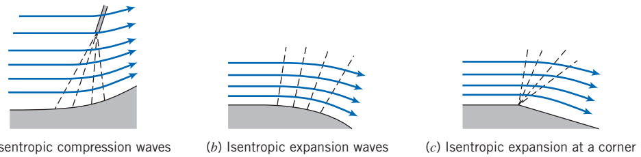
Fig. 13.30 Isentropic compression and expansion waves.
