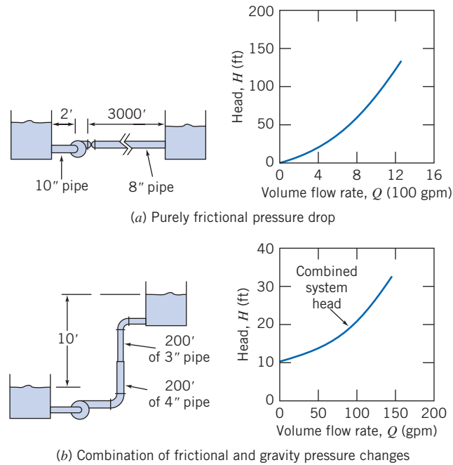
Fig. 10.18 Schematic diagrams illustrating basic types of system head-flow curves (adapted from [10]).
