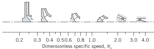
Fig. 10.8 Typical geometric proportions of commercial pumps as they vary with dimensionless specific speed [5].
