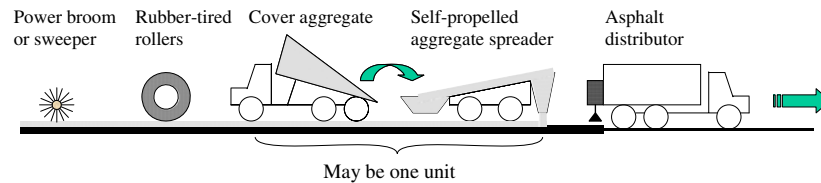
Schematic of Surface Treatment Construction Process
