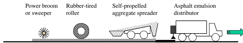
Schematic of Chip Seal Operation
