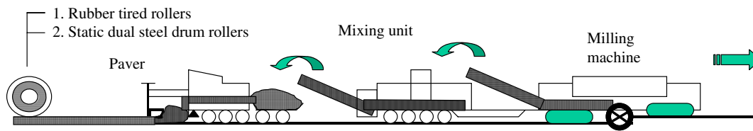
Schematic of Cold Recycling Process
