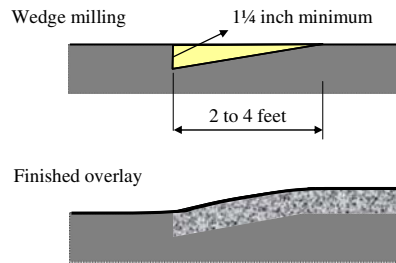
FIGURE B6 Wedge milling to key in a 1/4-in.-thick AC patch.
