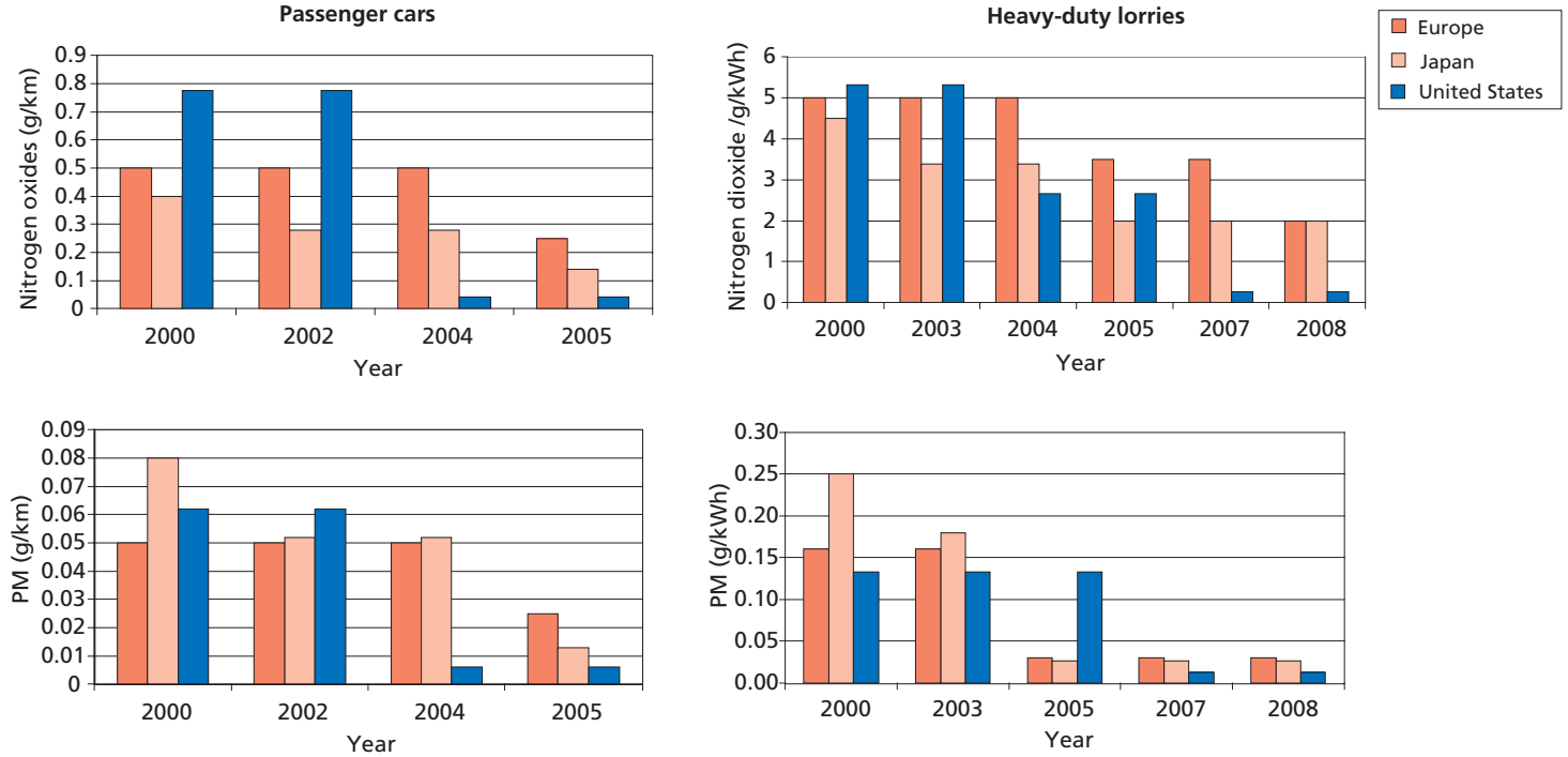
Fig. 1.20. Comparison of emission limits of PM and nitrogen oxides for passenger cars and heavy-duty lorries in the EU, Japan and the United States
