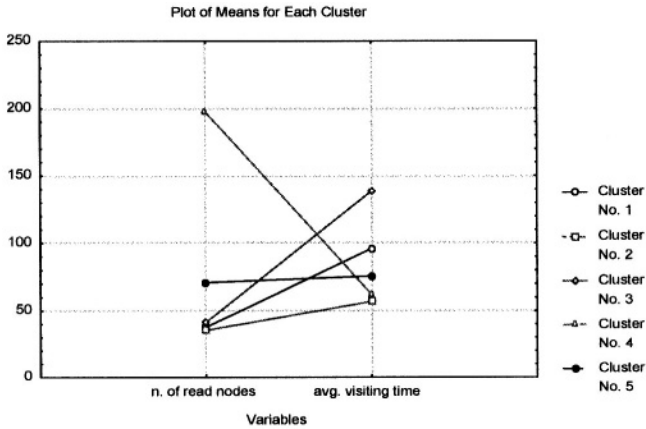
Figure 2. Five-cluster model.
