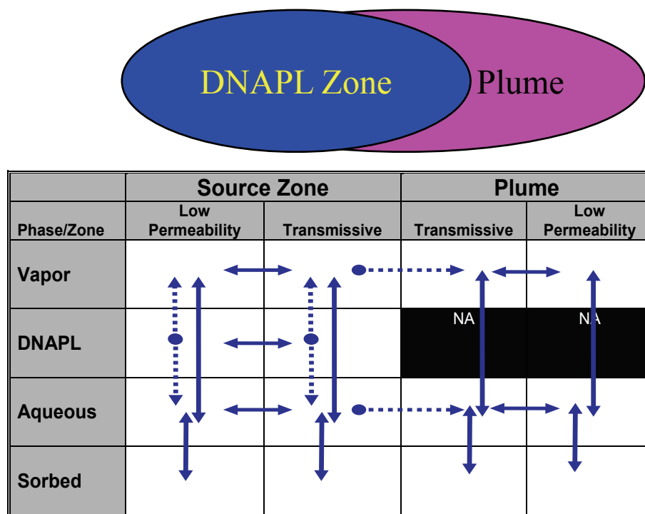
FIGURE 4-1 Conceptual model showing source zone and dissolved plume. The lower portion of the figure shows the 14-compartment model with common contaminant fluxes between compartments (solid arrows are reversible fluxes, dashed arrows are irreversible fluxes). SOURCE: ESTCP (2011).
