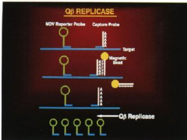
18-15 Principle of Q \beta replicase amplification system. In the Q \beta system, the enzyme Q \beta replicase amplifies the signal of the probe and not the target nucleic acid itself. The probe is an RNA molecule known as the midvariant (MDV-1) and a specific RNA fragment corresponding to a complementary piece of RNA or DNA in the organism to be detected. The probe RNA binds to the complementary target, and after removing the unbound MDV-1 molecules, the Q \beta replicase is added to replicate the RNA probe.
