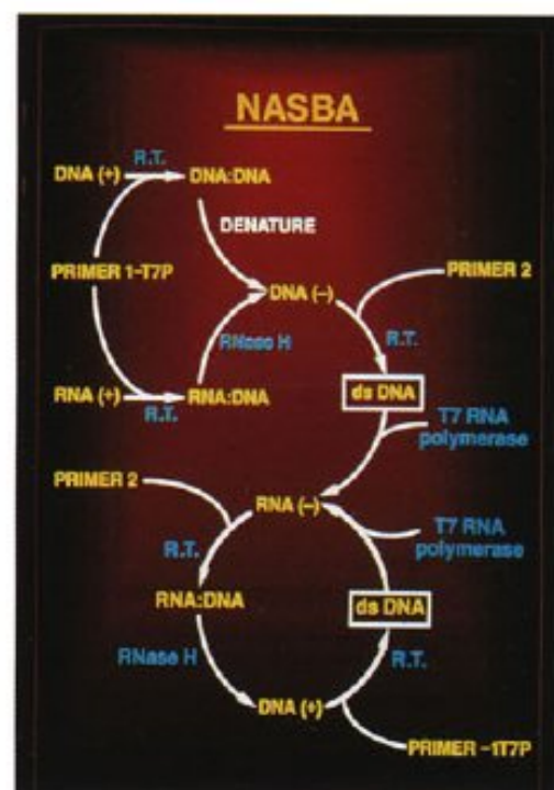
18-18 Nucleic acid sequence-based amplification (NASBA) method. Using components similar to those described for 3SR, this system also amplifies nucleic acids at room temperature.
