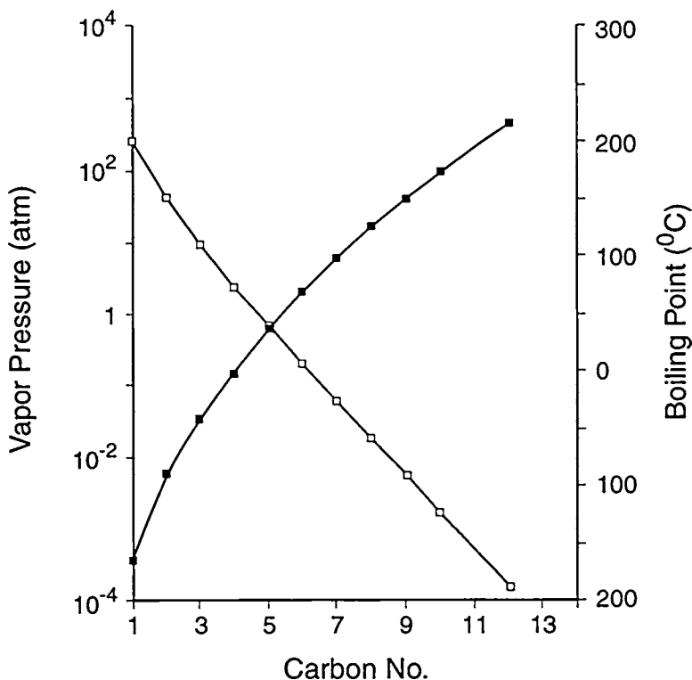
FIGURE 5.3 A plot of pure component vapor pressure (atm) and atmospheric pressure boiling points (°C) vs. carbon number for a series of n -alkanes.
