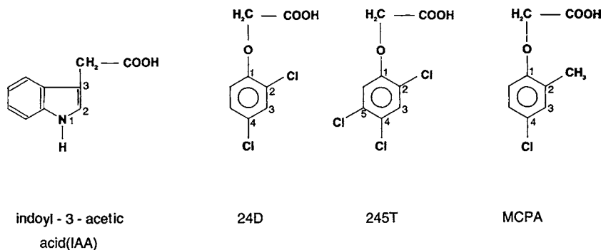
FIGURE 8.9 The chemical structures of some commonly used herbicides and IAA.
