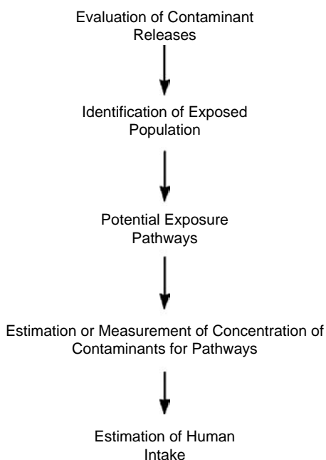
FIGURE 18.3 Evaluation of human exposure to a toxicant.
