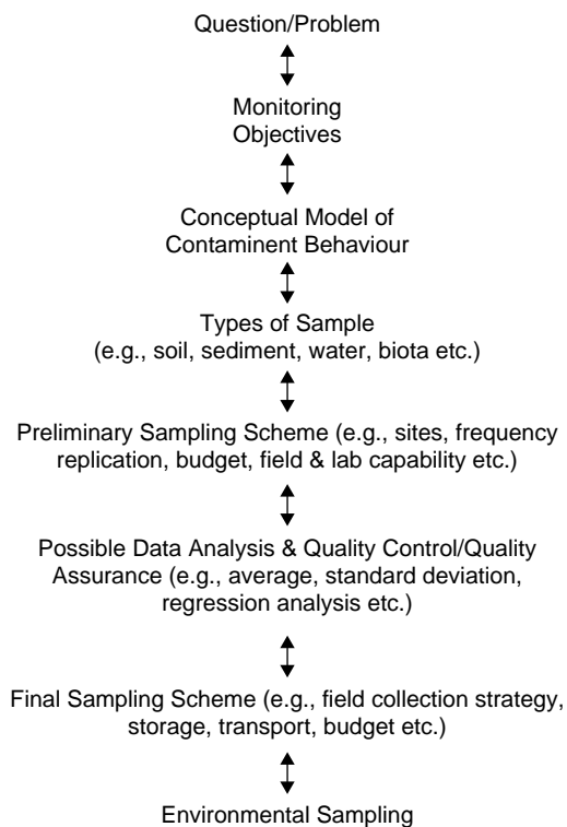
FIGURE 17.2 Steps involved in the design of a sampling strategy.
