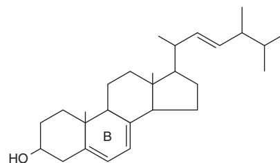
FIGURE 21-21 Ergosterol.
