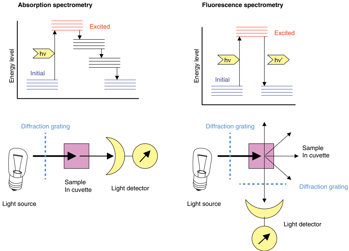
FIGURE 48-4 Absorption and fluorescence spectrometry. In absorption spectrometry, shown on the left, electrons are excited to an unstable higher energy level by the absorption of light, and then return to the basal energy level through a series of small quantum jumps. The energy is released as heat. The difference between the intensity of the exciting light and that transmitted through the sample, the absorbance, is proportional to the concentration of absorbing material in the cuvette (and the path length of the cuvette). In fluorescence spectrometry, shown on the right, the excited electrons return to the basal energy level in a single quantum jump. The energy is released as light of a lower energy (higher wavelength) than the exciting light. The intensity of the light emitted, measured at right angles to the exciting light, is proportional to the concentration of absorbing material in the cuvette (and the path length of the cuvette).
