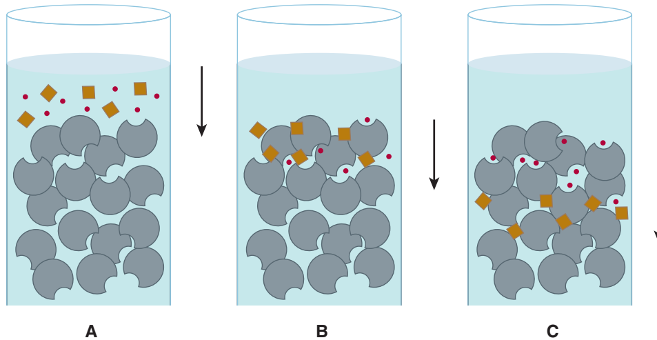
FIGURE 4-3 Size-exclusion chromatography. A: A mixture of large molecules (brown) and small molecules (red) is applied to the top of a gel filtration column. B: Upon entering the column, the small molecules enter pores in the stationary phase matrix (gray) from which the large molecules are excluded. C: As the mobile phase (blue) flows down the column, the large, excluded molecules flow with it, while the small molecules, which are temporarily sheltered from the flow when inside the pores, lag farther and farther behind.
