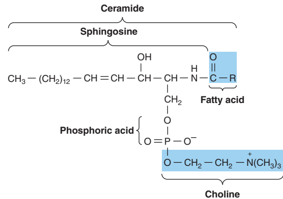
FIGURE 21-11 A sphingomyelin.
