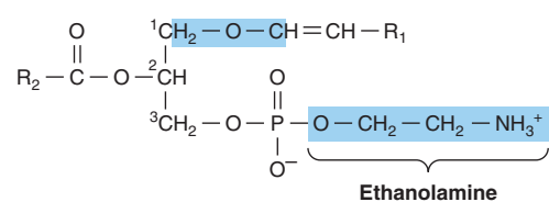
FIGURE 21-14 Plasmalogen.
