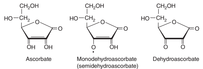
FIGURE 44-19 Vitamin C.
