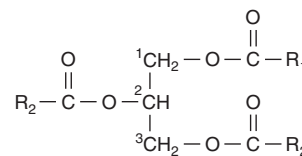
FIGURE 21-8 Triacylglycerol.
