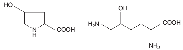
FIGURE 3-2 4-Hydroxyproline & 5-hydroxylysine.
