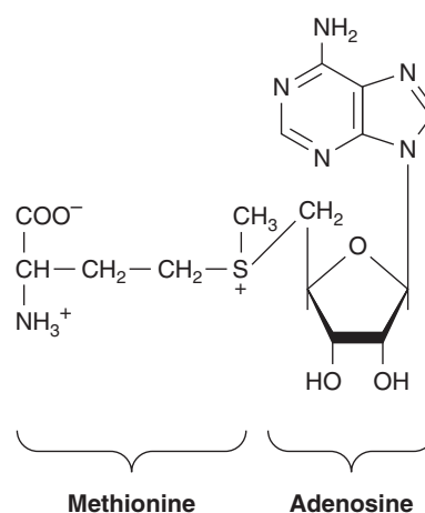
FIGURE 32-12 S -Adenosylmethionine.
