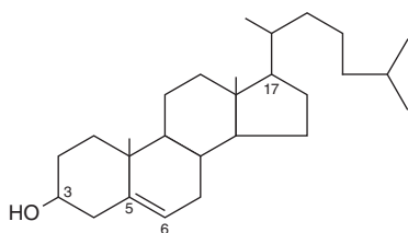
FIGURE 21-20 Cholesterol.
