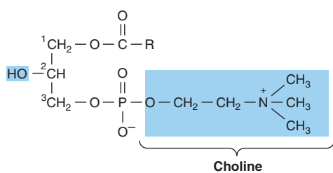
FIGURE 21-13 Lysophosphatidylcholine (lysolecithin).
