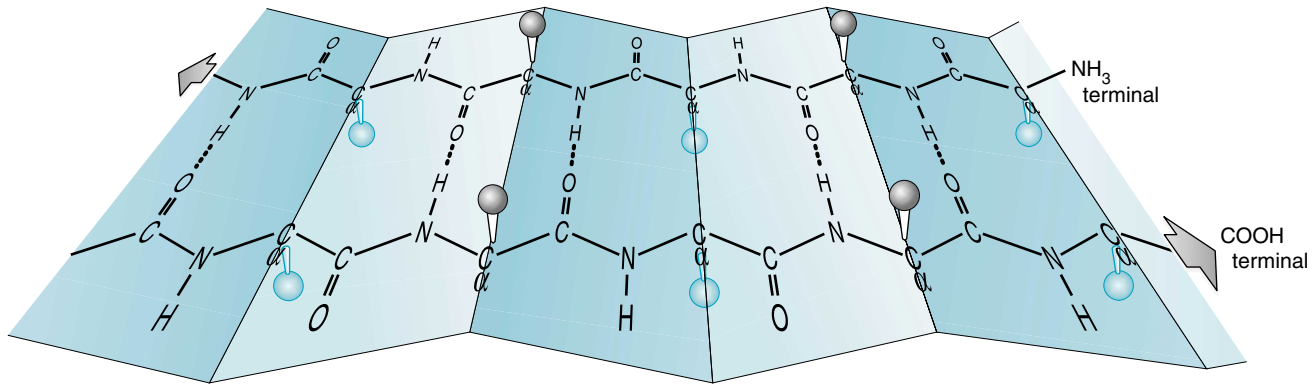
Fig. 7.6. A \beta -pleated sheet. In this case, the chains are oriented in opposite directions (antiparallel). The large arrows show the direction of the carboxy terminal. The amino acid side chains (R) in one strand are trans to each other, and alternate above and below the plane of the sheet, which can have a hydrophobic face and a polar face that engages in hydrogen bonding.
