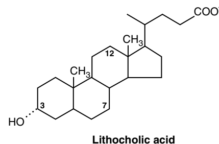
Fig. 34.13. Structures of the primary and secondary bile salts. Primary bile salts form conjugates with taurine or glycine in the liver. After secretion into the intestine, they may be deconjugated and dehydroxylated by the bacterial flora, forming secondary bile salts. Note that dehydroxylation occurs at position 7, forming the deoxy family of bile salts.
