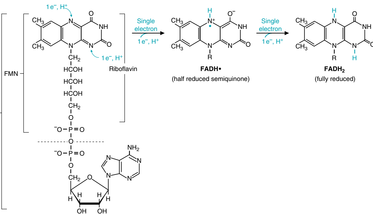
Fig. 20.4. One-electron steps in the reduction of FAD. When FAD and FMN accept single electrons, they are converted to the half-reduced semiquinone, a semistable free radical form. They can also accept two electrons to form the fully reduced form, FADH 2 . However, in most dehydrogenases, FADH 2 is never formed. Instead, the first electron is shared with a group on the protein as the next electron is transferred. Therefore, in this text, overall acceptance of two electrons by FAD has been denoted by the more general abbreviation, FAD(2H).
