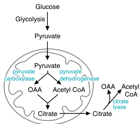
Fig. 33.6. Conversion of glucose to cytosolic acetyl CoA. OAA = oxaloacetate.
