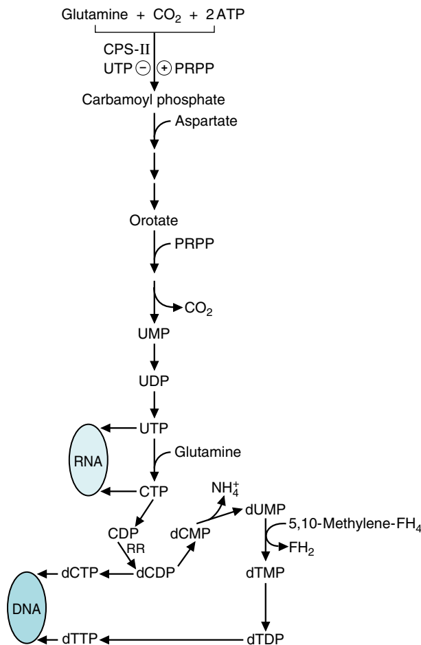
Fig. 41.14. Synthesis of the pyrimidine bases. CPSII = carbamoyl phosphate synthetase II. RR = ribonucleotide reductase; \oplus = stimulated by; \ominus = inhibited by; FH 2 and FH 4 = forms of folate.
