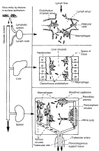
Fig. 132: Hypothetical model of Selye and Mailing hemomorphogenic liver. After Schmitt & Pothmann (1998).
