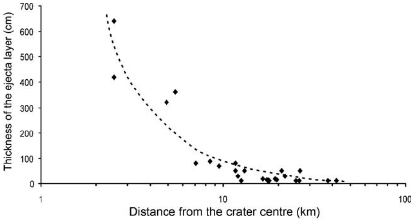
Fig. 3. Thickness of the Kärđla ejecta layer versus distance from the impact centre.
