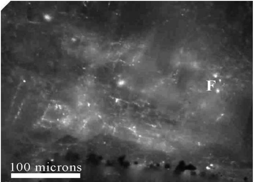
Fig. 6. Hydrocarbon inclusions (largest at F) fluorescing under U-V light in thin section of calcite from hydrothermal mineral vein, Houghton Crater. Each inclusion 5-10 micrometers size.
