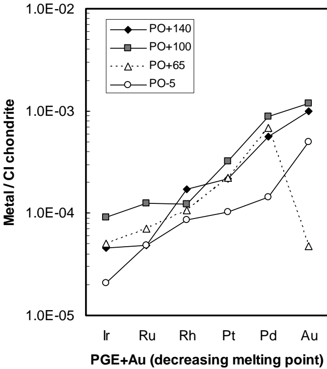
Fig. 4. Chondrite-normalized PGE and Au concentrations for some of the most PGE-rich units at Pointe aux Oises. Chondrite values used for normalization are from Jochum (1996).
