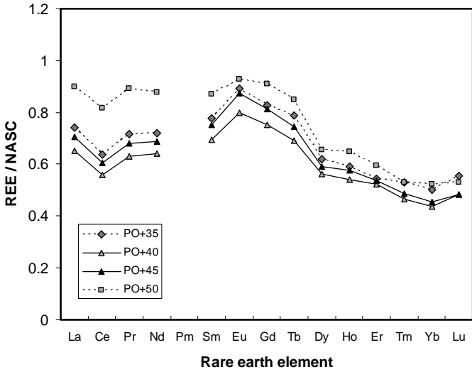
Fig. 5. North American Shale Composite (NASC) normalized rare earth element patterns for different units at Pointe aux Oies (see text for discussion).
