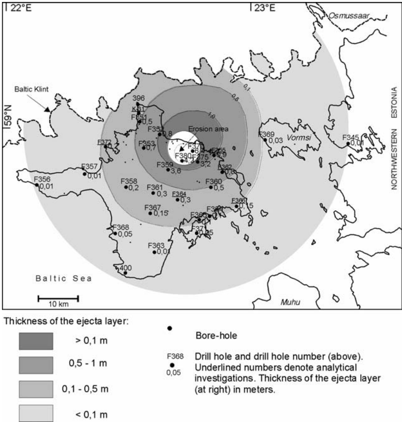
Fig. 2. Distribution of the ejecta blanket of the Kärđla crater, Estonia.
