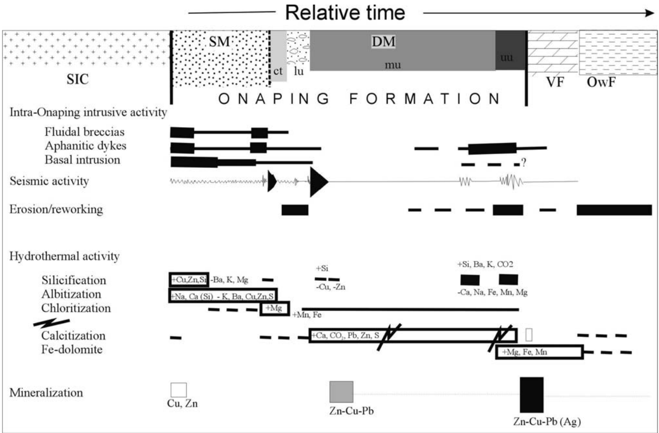
Fig. 9. Relative time-space chart for events in the Sudbury Basin (Ames 1999).
