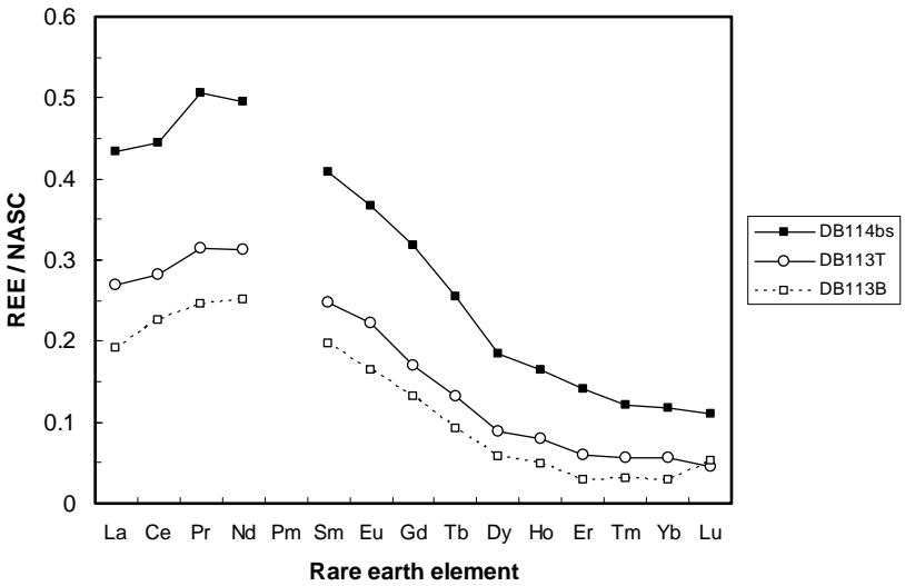
Fig. 7. North American Shale Composite (NASC) normalized rare earth element patterns for different units at Durlston Bay (see text for discussion).
