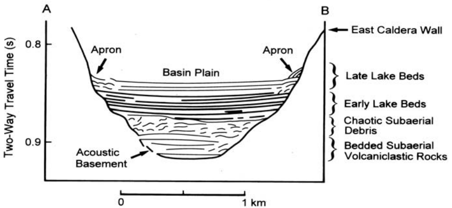
Fig. 4. Interpreted airgun ( 16.4 \text{ cm}^3 ) profile oriented east to west across the east basin of Crater Lake, Oregon (after Nelson et al. 1994).
