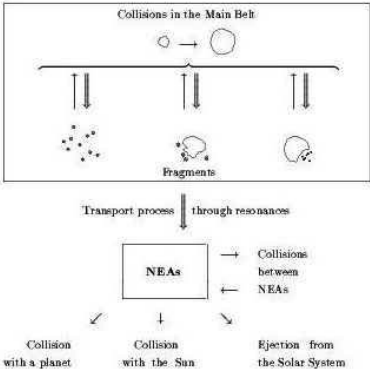
Fig. 9. A scenario for the life of NEAs.
