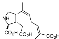
Isodomoic acid A (40)
