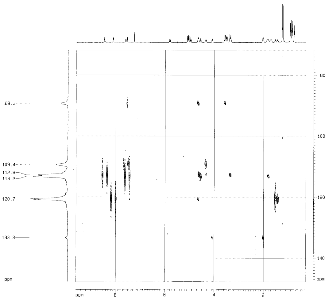
FIGURE 17.2 ^1\text{H} - ^{15}\text{N} GHMQC spectrum of keenamamide A ( 1 ).
