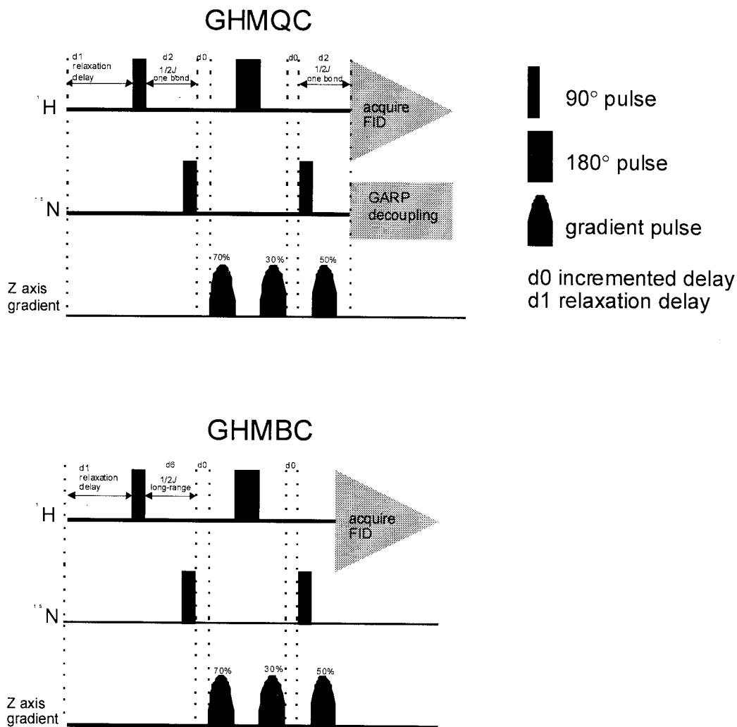
FIGURE 17.1 Pulse diagrams used for ^{15}\text{N} studies.
