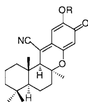
68 R = H (15-cyanopuupehenone) 69 R = OCOCH 3
