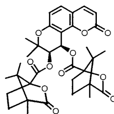
74 DCK
