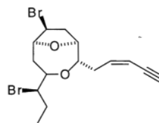
Z-Isolaureatin ( 26 )
