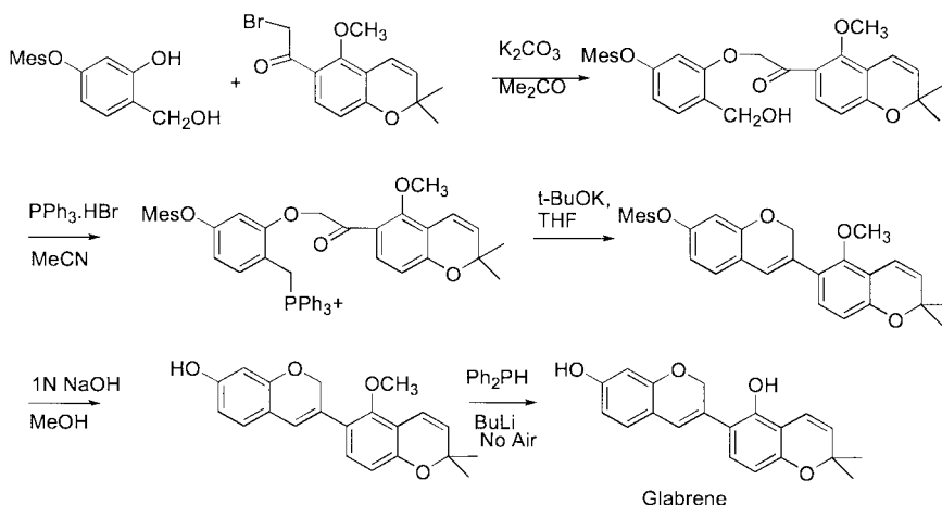
FIGURE 10.13 Total chemical synthesis of glabrene.
