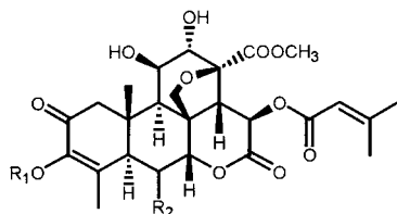
27 Bruceoside-C: R_1 = \beta\text{-D-glucose} R_2 =
