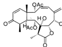
Ptilosarcenone ( 29 )
