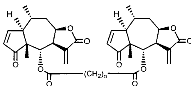
22 Bis(helenaliny)glutarate, n = 3
