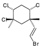
Telfairine ( 22 )
