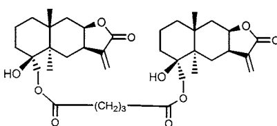
25 Bis(isoalantodiol-B)glutarate
