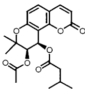
73 Suksdorfin
