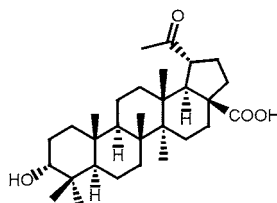
70 Platanic Acid
