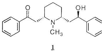
FIGURE 11.1 Structure of lobeline (1).
