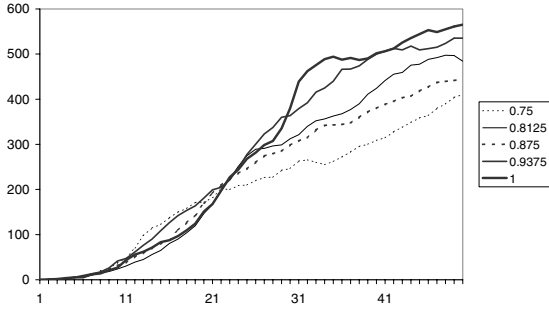
Fig. 14. Average number of communications for runs with different racial biases
