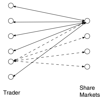
Fig. 6. Star graphs as building blocks of the communication structure
