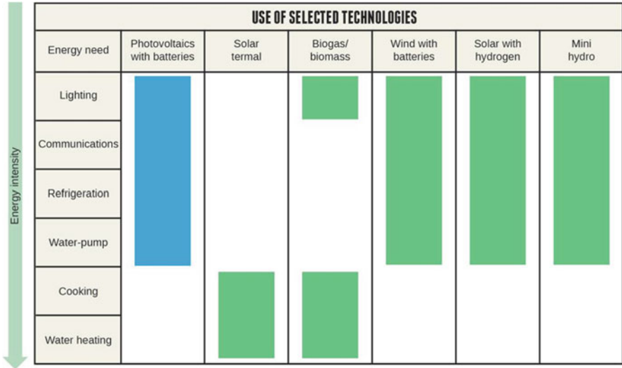
Fig. 14.2 The increasing energy intensity of energy demand for various tasks, and technologies that match requirements [6]
