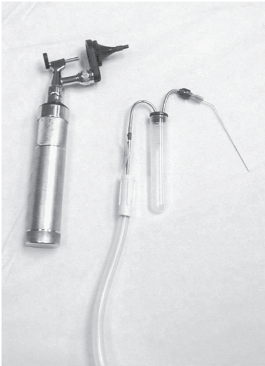
▲ Figure 18–3. Operating head and Alden-Senturia trap for tympanocentesis. Eighteen-gauge spinal needle is attached and bent.
