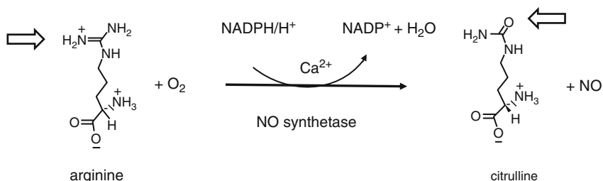
Fig. 8.1 Scheme of synthesis of NO. L-arginine is catalyzed to L-citrulline by a complex enzyme (NO synthetase) producing one molecule of NO. For this reaction, the oxygen and NADPH/H + are necessary
