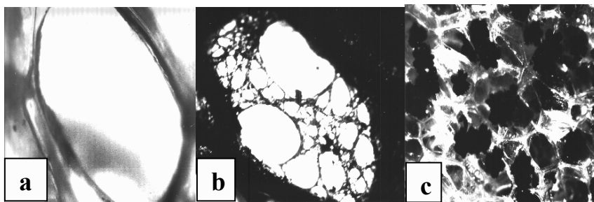
Figure 4. Deterioration of a polyurethane foam (PU) by fungal exoenzymes; (a) fresh PU showing an intact thin membrane as closing space between the foam structural bunks; (b) same membrane deteriorated; (c) PU deteriorated, and shown lacking membranes and disrupted structural bunks (Photo: Filip).
