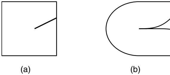
FIGURE 7.4. Lipschitz domains
