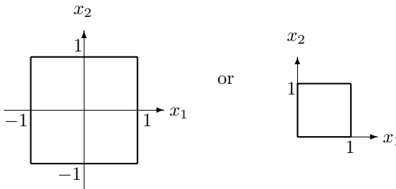
Figure 10.3: Reference rectangular elements in \mathbb{R}^2
