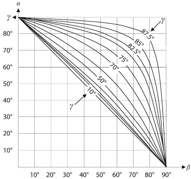
Fig. B5. Angle of inclination of drill holes for drilling oblique to strike to achieve optimal drill intersections (summary diagram)
