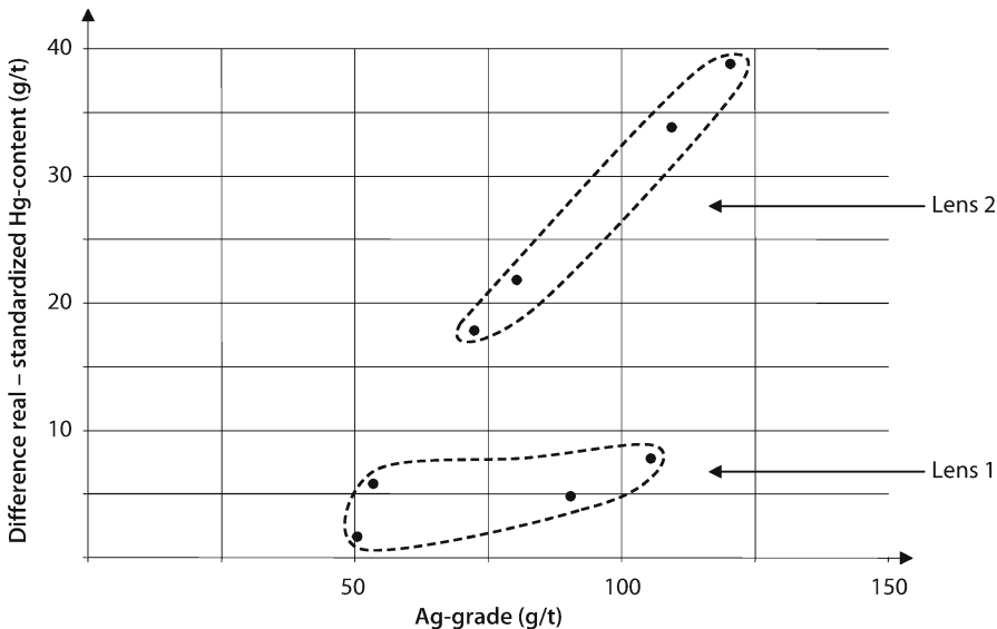
Fig. 3.6. Hg as a function of Ag-grades in a Zn-Pb-Ag-deposit, using Hg-values standardized against Zn
