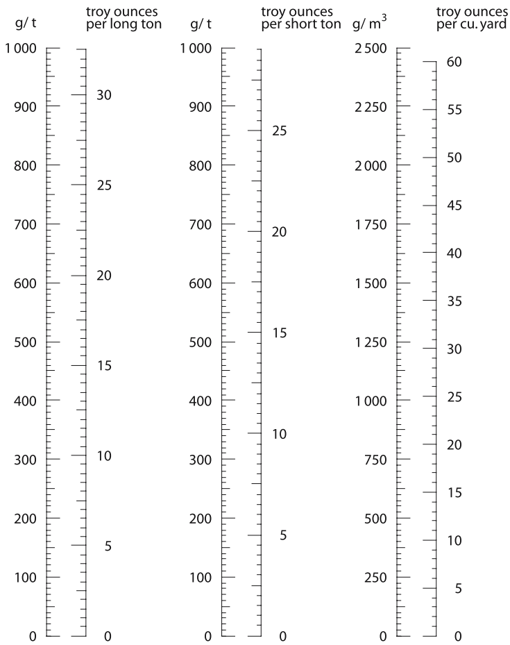
Fig. A5. Conversion between some concentration measures
