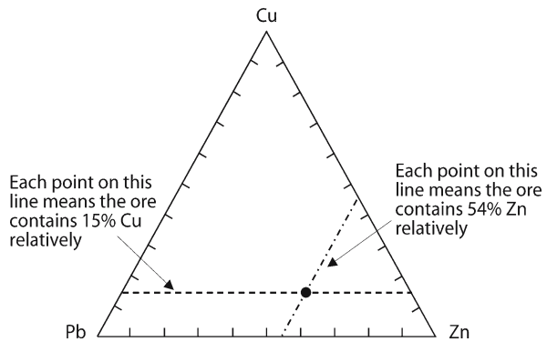
Fig. 3.1a. Pb-Zn-Cu ternary diagram
