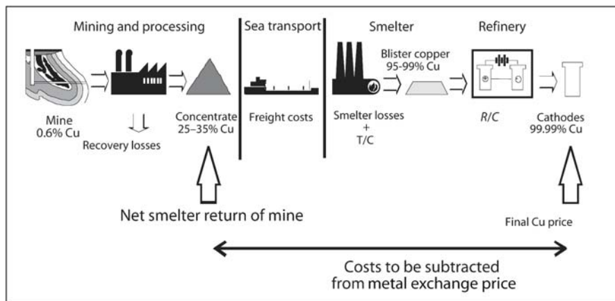
Fig. 7.1. Flow sheet for the recovery process copper
