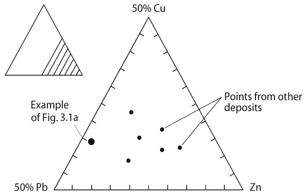
Fig. 3.1b. Modified ternary diagram of Fig. 3.1a
