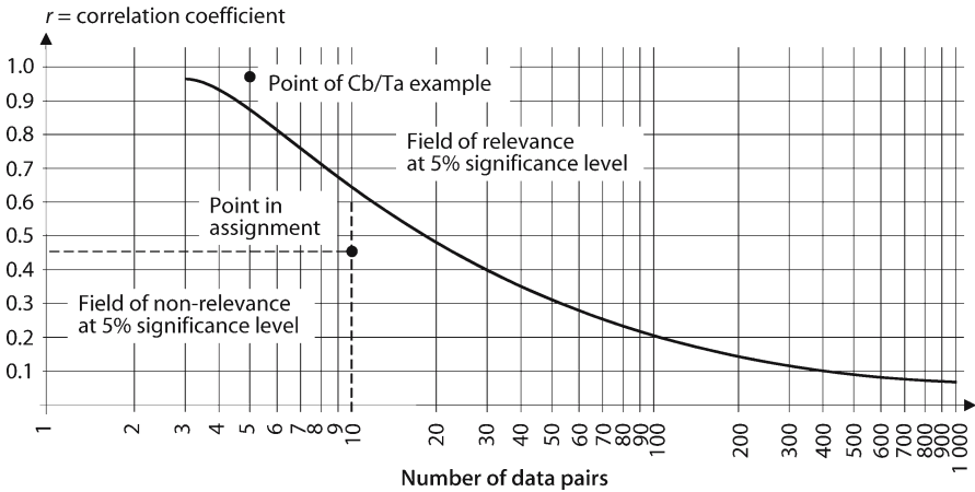
Fig. 3.5. Minimum correlation coefficients at a significance level of 5%
