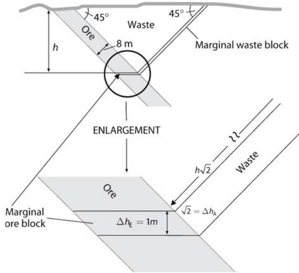
Fig. 10.1. Vertical section for the calculation of a marginal stripping ratio
