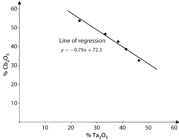
Fig. 3.4. Negative correlation of Cb and Ta in five concentrates
