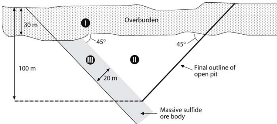
Fig. 9.4. Vertical section to calculate the waste:ore ratio
