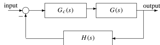
Figure 1.2. Typical linear feedback structure.
