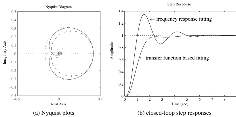
Figure 6.11. PID controller responses.
