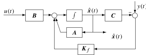
Figure 7.1. Kalman filter.
