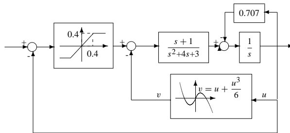
Figure 4.9. An example of a nonlinear system.
