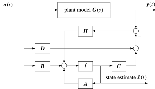
Figure 5.20. A typical structure of state observers.
