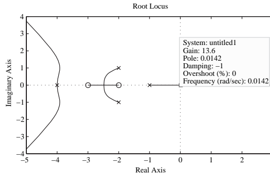
Figure 3.16. Root locus for positive feedback systems.
