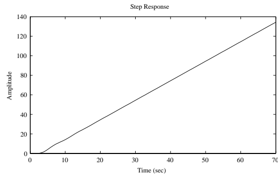
Figure 3.12. Ramp response of the system in Example 3.21.
