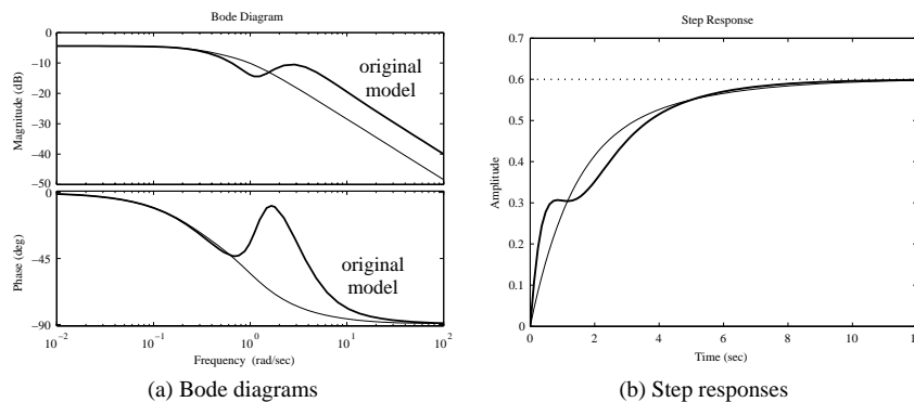
Figure 3.30. Bode diagram and step response comparisons.
