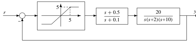
Figure 4.47. The block diagram for Problem 16.
