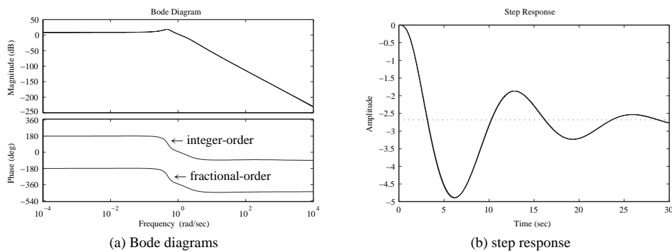
Figure 8.1. Time and frequency domain comparisons.
