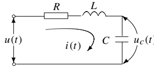
Figure 2.1. An RLC series circuit.
