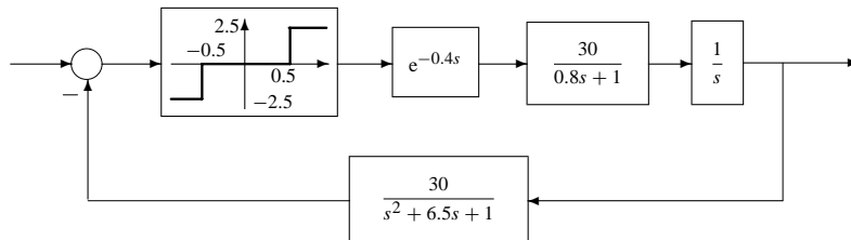
Figure 4.43. Block diagram in Problem 10.
