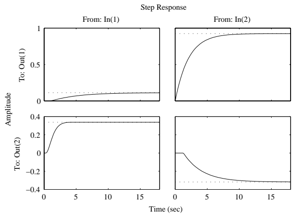
Figure 3.10. Step response of a multivariable system.
