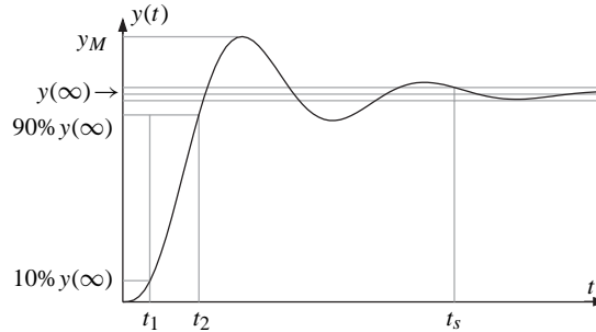
Figure 3.6. Typical step response specifications.
