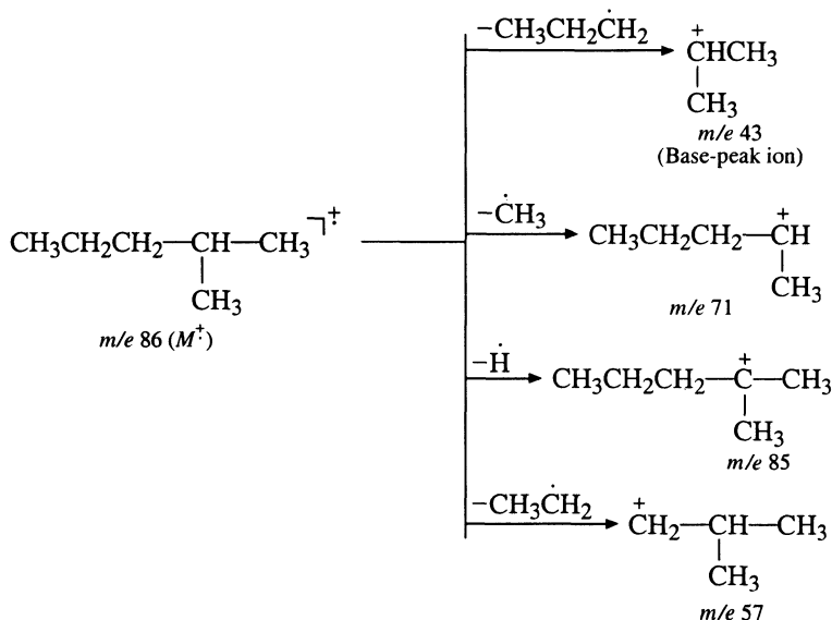
Scheme 8.2 Fragmentation pattern of 2-methylpentane
