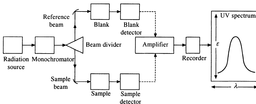
Fig. 2.1 Schematic diagram of a double-beam UV-visible spectrophotometer
