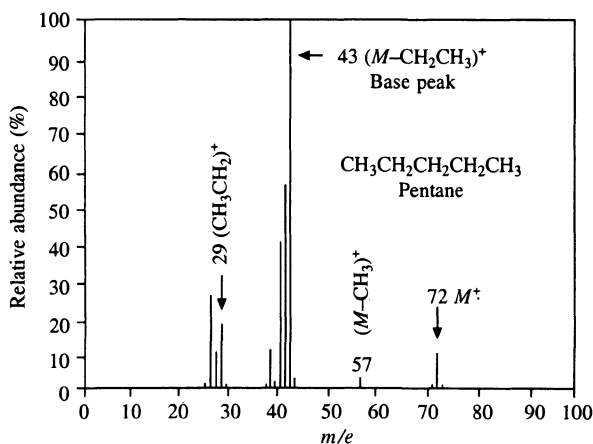
Fig. 8.2 Mass spectrum of pentane
