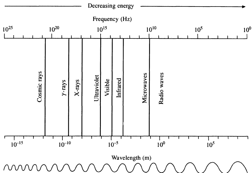
Fig. 1.2 Electromagnetic spectrum
