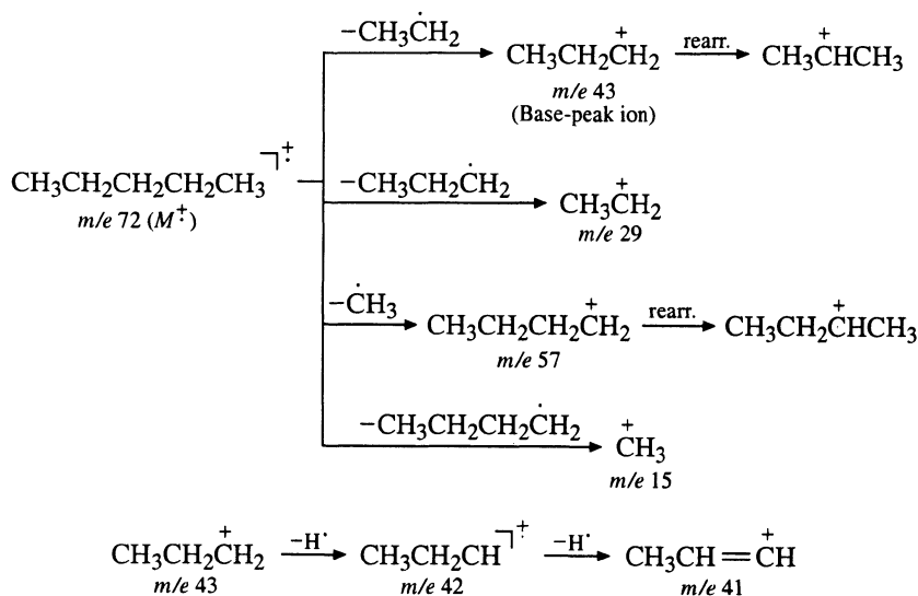
Scheme 8.1 Mode of fragmentation of pentane
