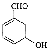
m -hydroxybenzaldehyde
