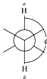
Anti ( \phi = 180^\circ )
