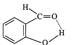
o -hydroxybenzaldehyde
