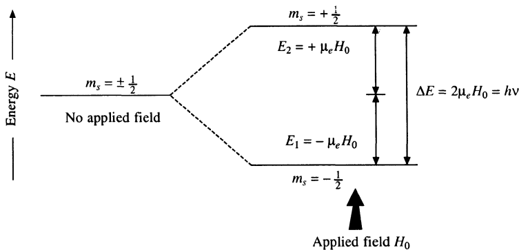
Fig. 7.1 Energy states of an unpaired electron in an applied magnetic field H_0
