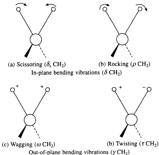
Fig. 3.3 Bending vibrations (deformations) of a CH 2 group (+ and – signs indicate movements perpendicular to the plane of the paper)
