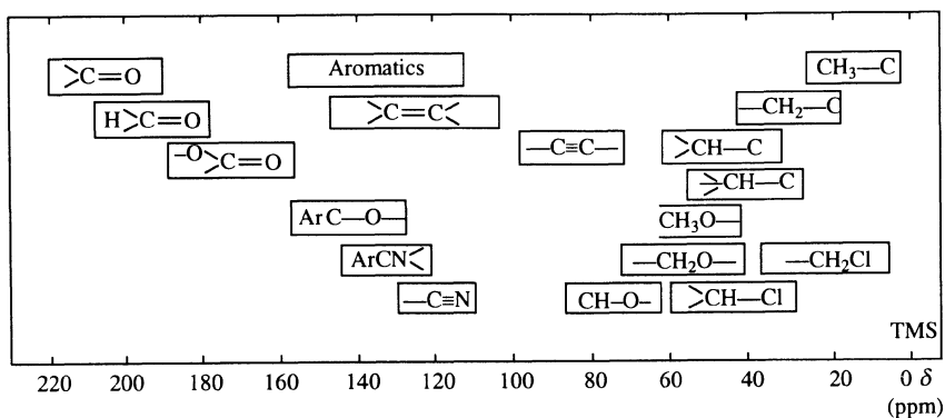
Fig. 6.4 General regions of 13 C chemical shifts
