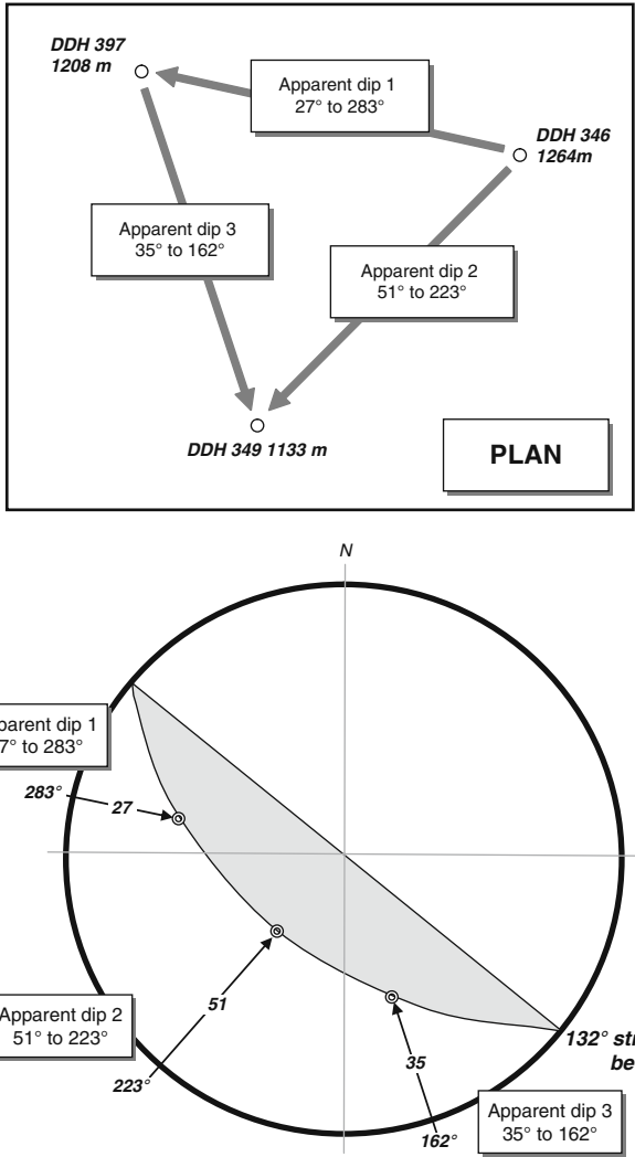
Fig. C.2 Using a stereonet to determine the strike and dip of planar surface intersected in three drill holes. The intercepts are projected onto a plan and labelled with the height of each intersection above a common datum. The line that joins any pair of intersections is an apparent dip on the bed and can be described by its dip and dip direction. Where v is the vertical height difference between each pair of intersections, and h their horizontal separation, the apparent dip ( a ) can be calculated using \text{Tan } a = v/h . The dip direction is measured directly from the plan with a protractor. Three apparent dips can be calculated in this way. On the stereonet, the three apparent dips plot as three points. The net overlay is rotated to bring the points to lie on a great circle girdle. This girdle is the plot of the bed and its strike (and true) dip can be easily read off. (Actually, only 2 apparent dips are necessary to define the surface, but using a third line provides extra accuracy.)
