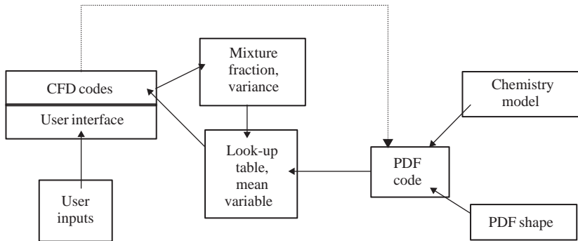
FIGURE 7.19 Generic coupling between a PDF solver and a CFD solver.
