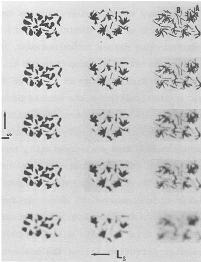
FIGURE 5.3 Scale and intensity of segregation (from Brodkey, 1975).
