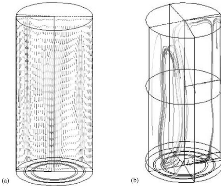
FIGURE 11.17 Typical results obtained for double ring sparger (From Ranade and Tayalia, 2001). (a) Vector plot, (b) particle streak lines.
