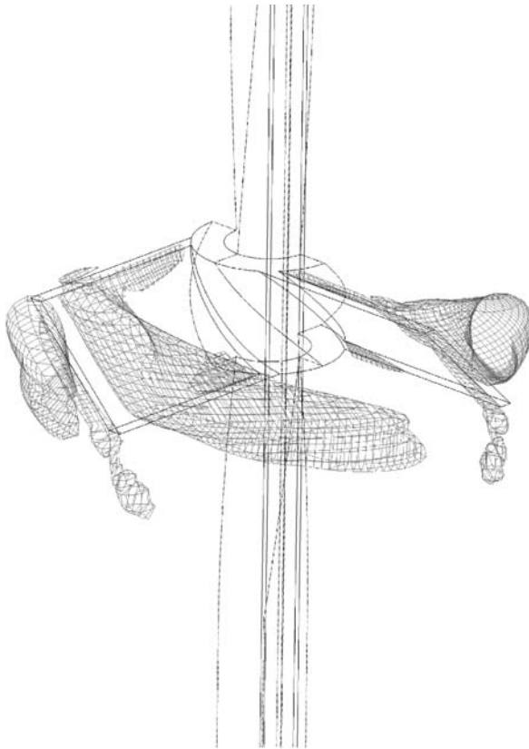
Iso-surface of Z-vorticity ( \omega D/U_{tip} = -7 ) Impeller rotation: from right to left
