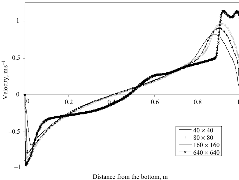
FIGURE 6.23 Influence of grid size for low viscosity fluid ( \mu = 0.001 Pa.s).
