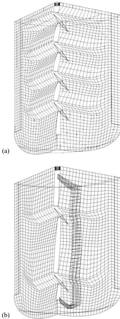
FIGURE 9.4 Two alternatives to enhance reactor performance. (a) Four pitched blade turbine, (b) two pitched blade turbine with cage.
