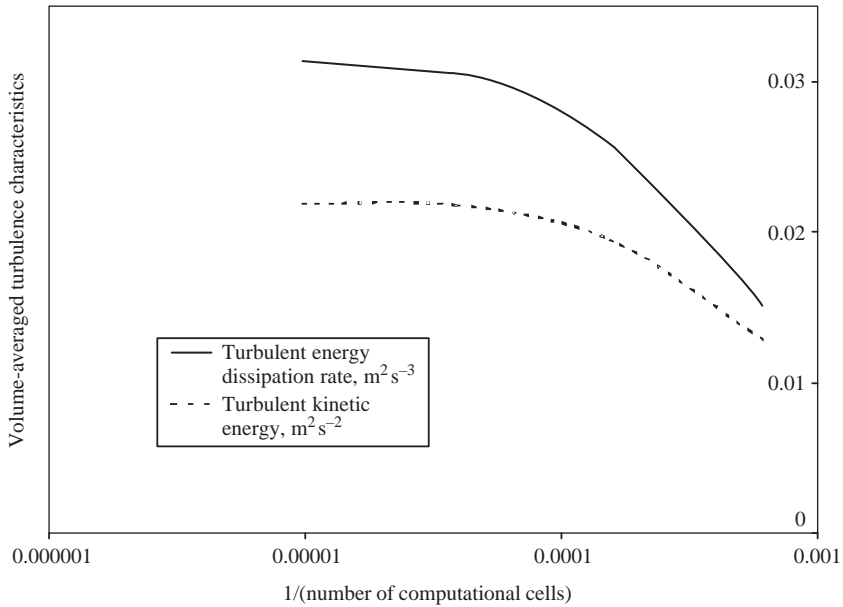
FIGURE 7.2 Influence of grid size on volume averaged turbulent characteristics.
