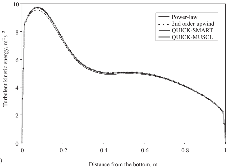
FIGURE 7.7 Influence of discretization schemes on predicted results. (a) U velocity at x = 0.5 m, (b) Turbulent kinetic energy at x = 0.5 m.
