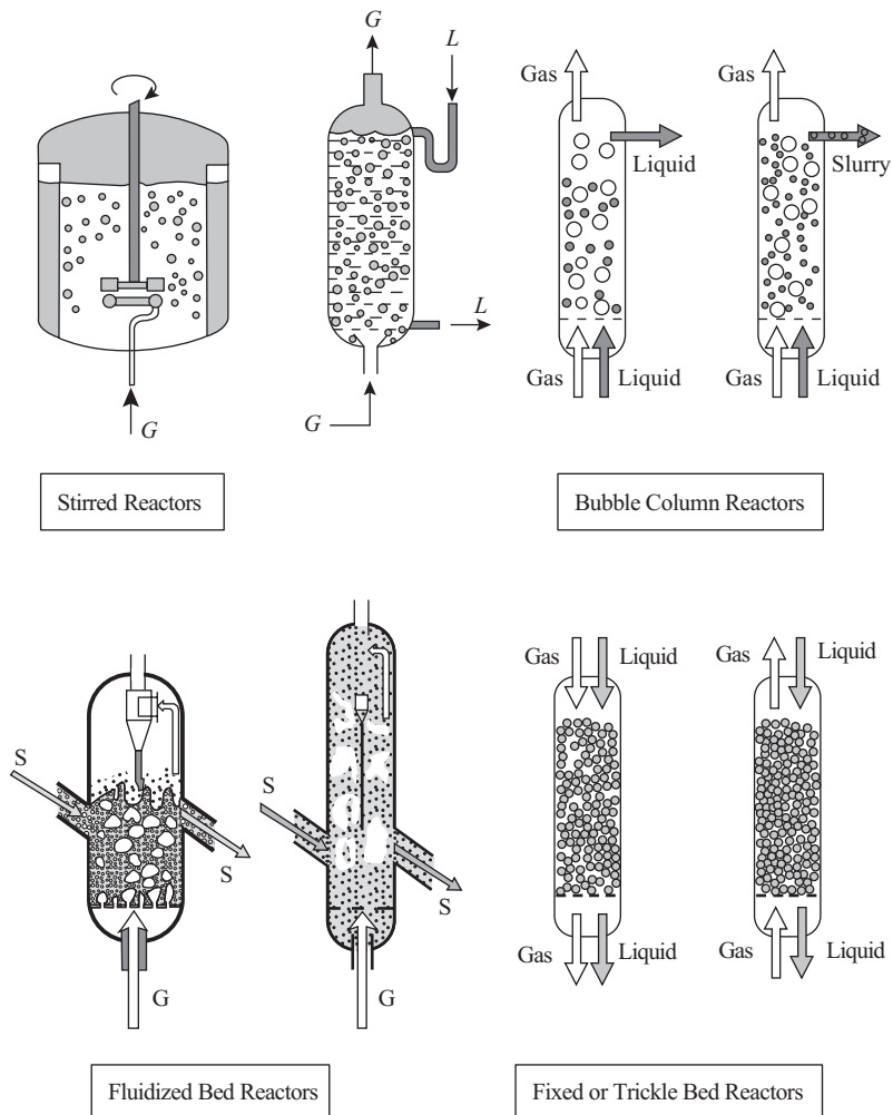
FIGURE I.2 Commonly used reactor types.
