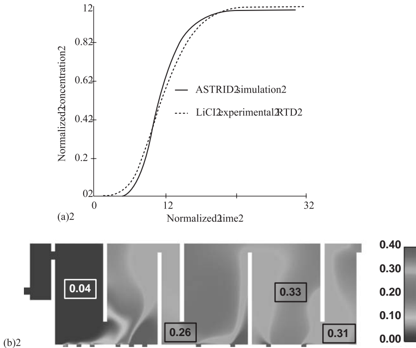
FIGURE 11.19 Validation of computational model (from Cockx et al. , 1999). (a) Predicted and measured cumulated tracer plots. (b) Predicted and measured concentration of dissolved ozone (numbers in squares indicate experimental data).
