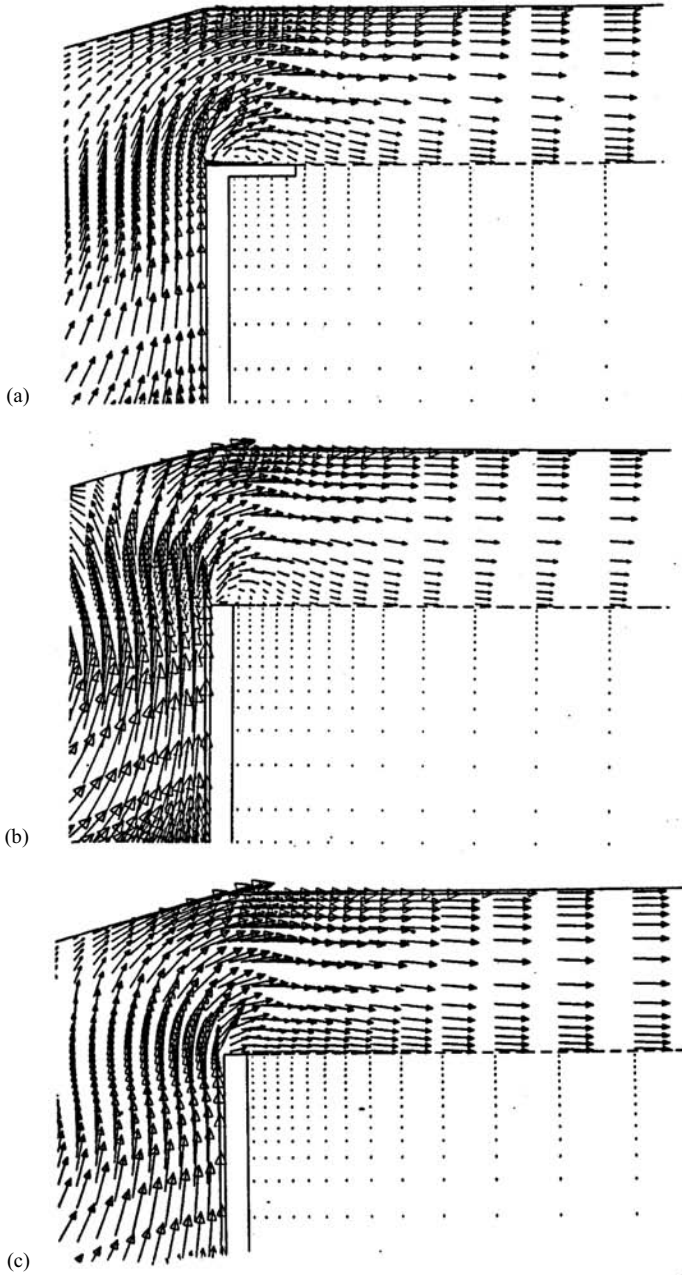
FIGURE 13.6 Predicted flow field near top cover plate (see Fig. 13.5 for details of configurations (a), (b) and (c)).
