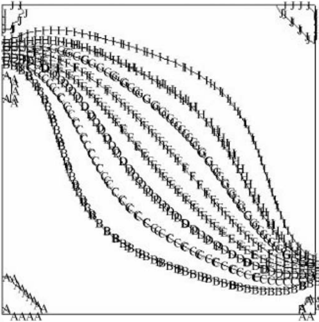
FIGURE 6.15 Typical simulation results; Grid: 40 \times 40 . Vector: maximum length 1 \text{ m s}^{-1} . Contours of stream function: 10 uniform contours between 0 to 0.001 (Lowest level: A; Highest level: J).
