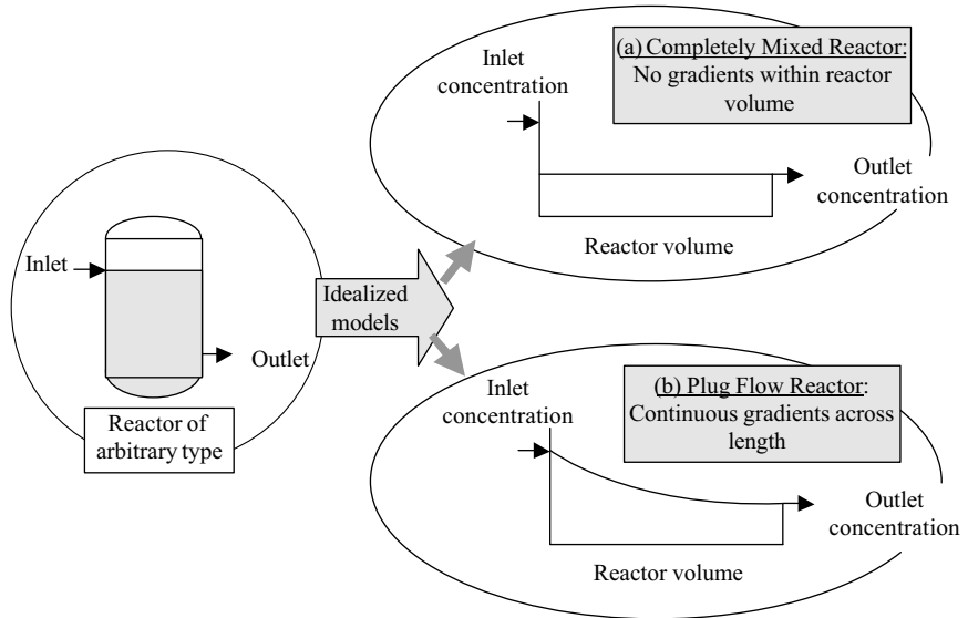
FIGURE 1.4 Ideal reactors.
