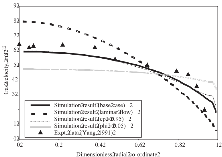
FIGURE 12.12 Comparison of simulation results with experimental data at low solids flux ( d_p = 54 \mu\text{m} , \rho_s = 1545 \text{ kg m}^{-3} , D = 0.14 \text{ m} , U_g = 4.33 \text{ m s}^{-1} , G_s = 10 \text{ kg m}^2 \text{ s}^{-1} ) (from Ranade, 1999).
