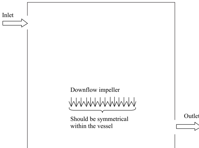
FIGURE 7.3 Configuration with downflow impeller.
