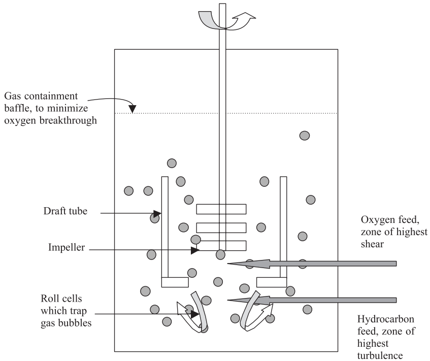
FIGURE 10.2 Schematic of liquid phase oxidation reactor patented by Roby (1997).
