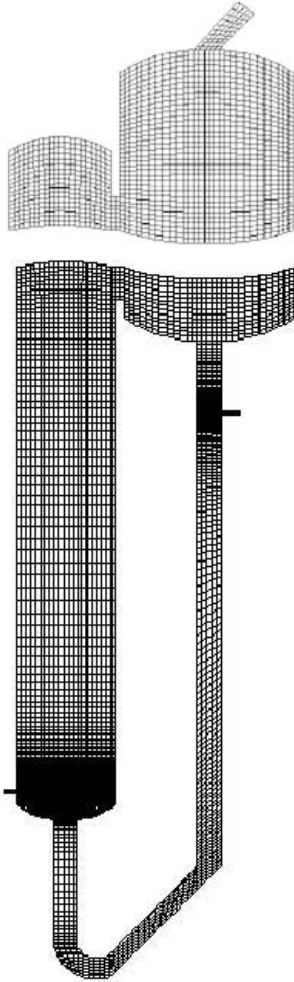
FIGURE 9.20 Computational grid.
