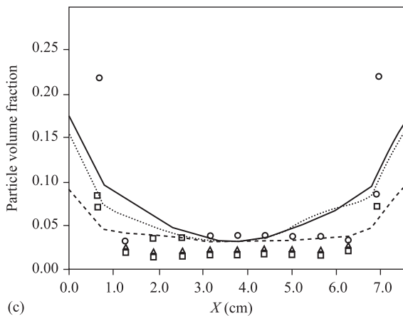
FIGURE 12.17 Some simulation results for gas-solids flows in a riser. (a) Axial particle diameter profiles for different superficial gas velocities ( V_{SUP} ) (from Mathiesen et al. , 2000). (b) Radial solid volume fraction profiles at 0.7 m from the bottom, V_{SUP} = 1.0 \text{ m s}^{-1} (from Mathiesen et al. , 2000). (c) Radial solids volume fraction profiles at different heights: solid line and circles 1.86 m; short-dashed line and squares 4.18 m; long-dashed line and diamonds 5.52 m (from Neri and Gidaspaw, 2000).
