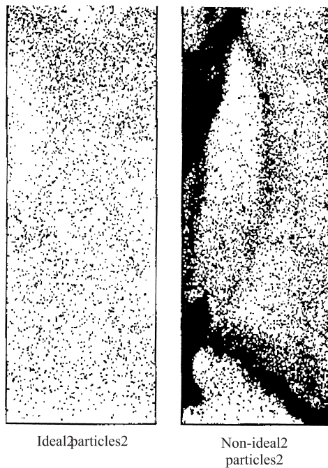
FIGURE 12.8 Simulated fluidization behavior for ideal and non-ideal particles in a Riser reactor (from Hoomans, 2000).
