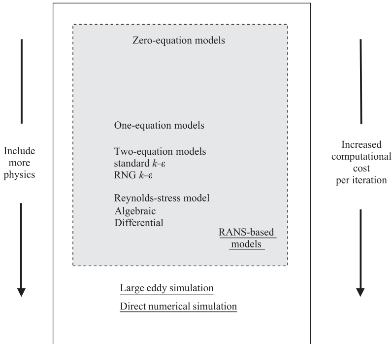
FIGURE 3.3 Modeling approaches for turbulent flows.
