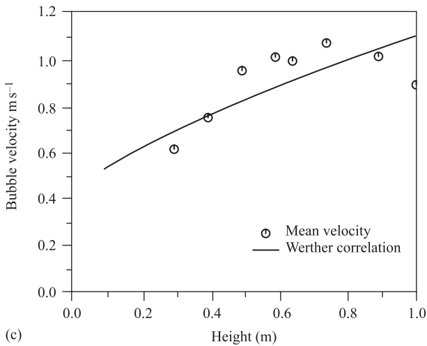
FIGURE 12.18 Comparison of simulated bubbling fluidization of Geldart group A particles with experimental data (from Ferschneider and Mege, 1996).
