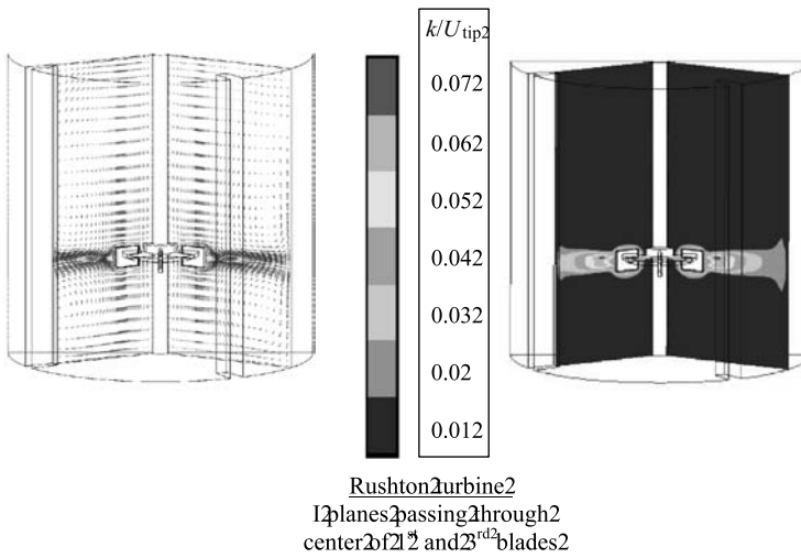
FIGURE 10.7 Predicted flow field at typical r - z planes (from Ranade et al. , 2001a).
