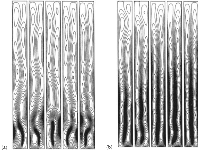
FIGURE 9.15 Predicted streamlines of liquid flow (from Bauer and Eigenberger, 1999). (a) Neglecting mass transfer, (b) accounting for mass transfer.
