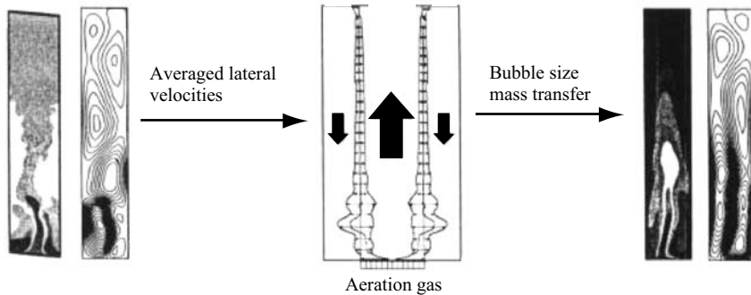
FIGURE 9.14 Iterative process used in multiscale modeling (from Bauer and Eigenberger, 1999).
