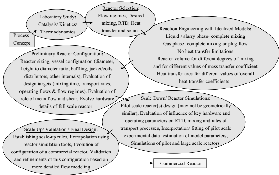
FIGURE I.10 Methodology of reactor engineering.
