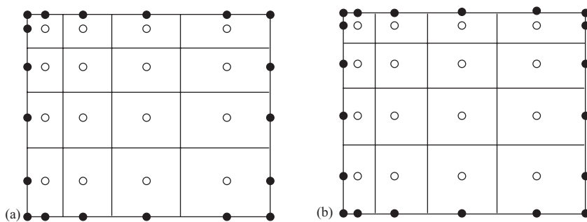
FIGURE 6.1 Finite volume grid, nodes centered in control volumes (left) and faces centered between nodes (right).
