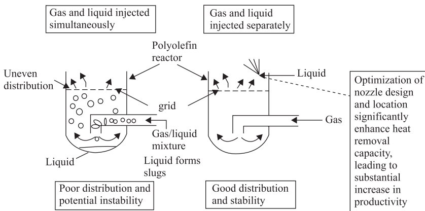
FIGURE 1.13 Super-condensed mode of olefin polymerization.
