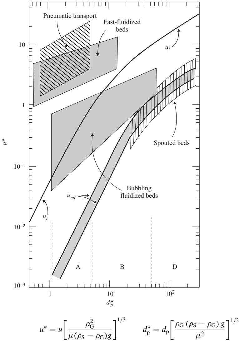
FIGURE 12.4 General flow regime map for gas-solids flows (from Kunii and Levenspiel, 1991).
