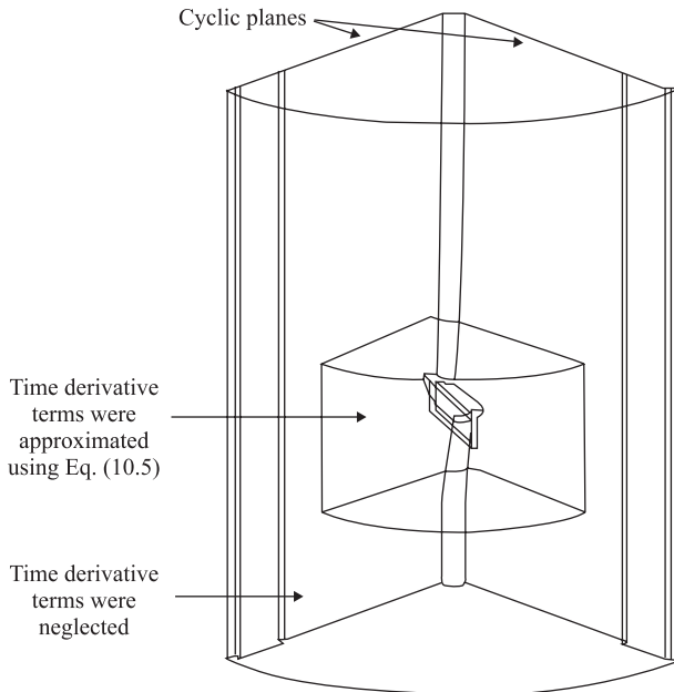
FIGURE 10.13 Solution domain and boundary conditions for pitched blade turbine simulation.
