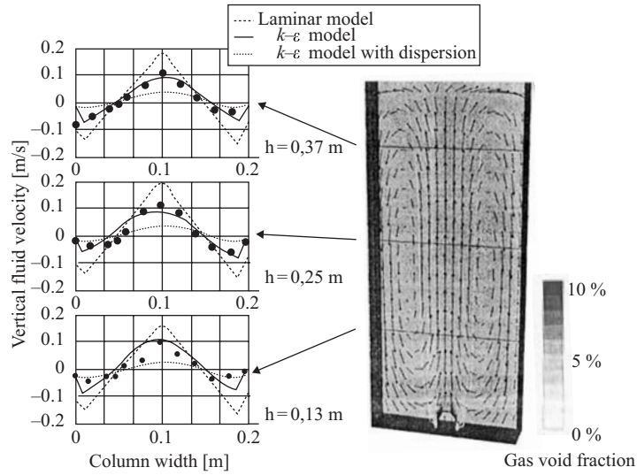
FIGURE 11.3 Simulated results for rectangular 2D bubble column (from Pflieger et al., 1999) (a) Time-averaged results, (b) transient results.
