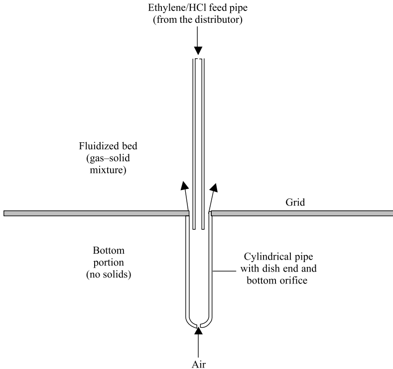
FIGURE 9.7 Schematic of mixing cup (from Ranade, 1999b).
