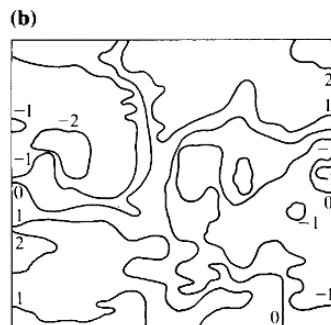
Figure 4.39 Results of a direct shear test on a 127 mm × 152 mm graphite-coated joint, carried out at a constant normal force of 28.9 kN. (a) Shear force–shear displacement curves; (b) surface profile contours before testing (mm); (c) relative positions on a particular cross section after 25 mm of sliding (after Jaeger, 1971).
