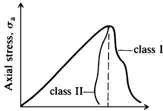
Figure 4.12 Two classes of stress–strain behavior observed in uniaxial compression tests (after Wawersik and Fairhurst, 1970).
