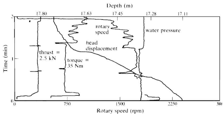
Figure 3.18 Strip chart record of a short instrumented diamond drilling run (after Barr and Brown, 1983).
