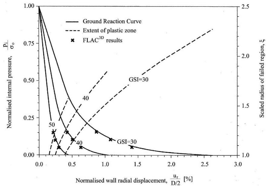
Figure 11.8 Analysis of convergence and the extent of the plastic zone in a tunnel in a rock mass having a Hoek-Brown strength criterion and subject to an initial hydrostatic stress field: (a) problem definition and data; (b) ground reaction curves and normalised extent of the plastic zone at section SS' for three values of GSI. The crosses are values calculated using the code FLAC^{3D} (after Carranza-Torrens and Fairhurst, 1999).
