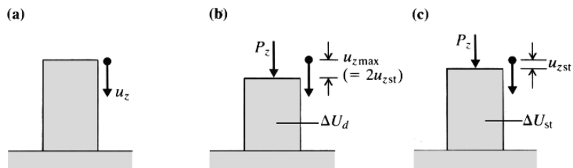
Figure 10.4 Problem geometry for examining energy partitioning in a pillar under dynamic load.
