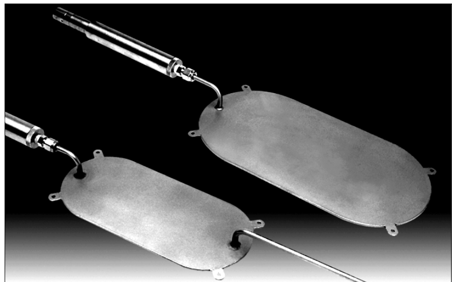
Figure 18.6 Tangential (left) and radial (right) total pressure cells. (Photograph by Slope Indicator Company.)
