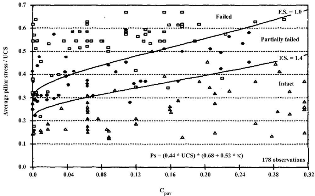
Figure 13.13 Pillar behaviour domains mapped in terms of normalized pillar stress and normalised state of internal pillar confinement, C_{pav} (after Lunder and Pakalnis, 1997).
