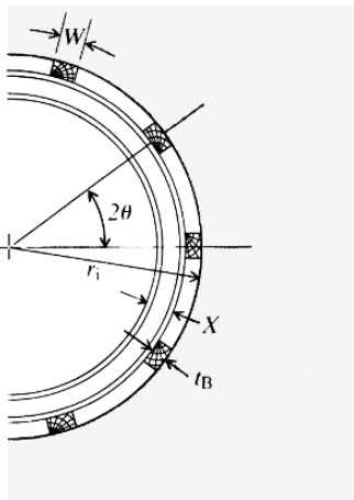
Figure A.8 Blocked steel set.
