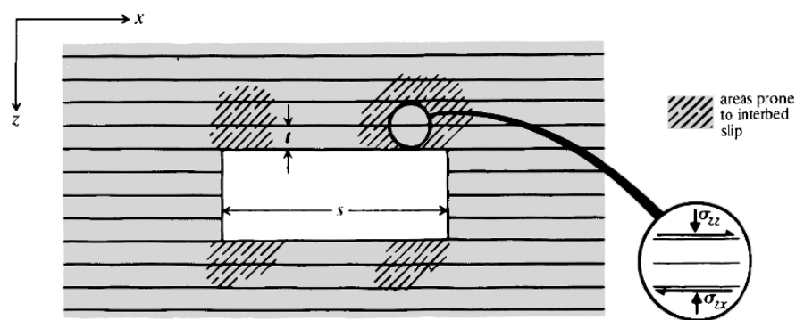
Figure 8.2 Slip-prone zones around an excavation in stratified rock.
