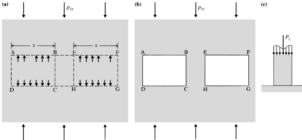
Figure 10.1 (a) Pre-mining state of loading around rooms in a stratiform orebody subject to uniaxial stress; (b) post-excitation state; (c) free-body diagram showing induced axial pillar load.
