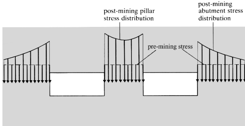
Figure 13.4 Redistribution of stress in the axial direction of a pillar accompanying stope development.
