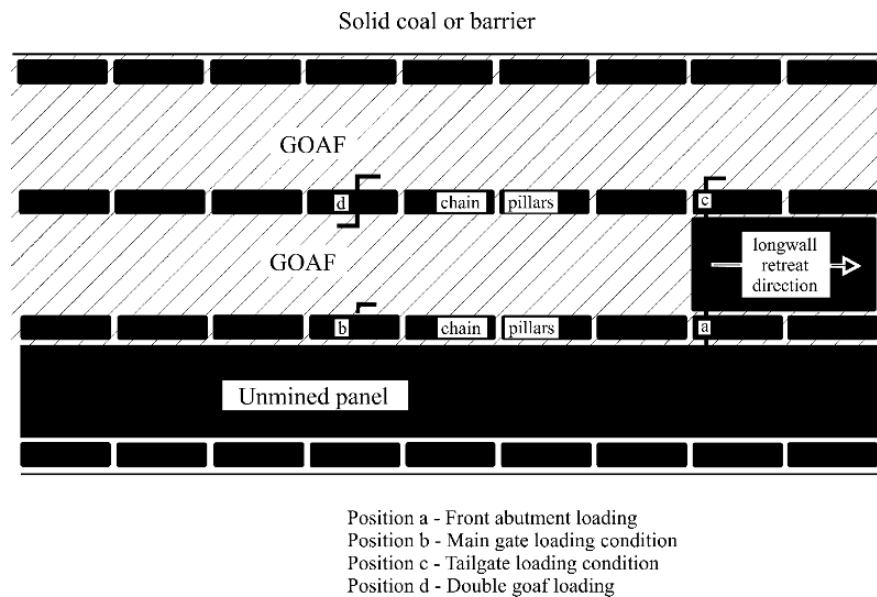
Figure 15.7 Development and extraction of adjacent longwalls using multiple roadways illustrating the chain pillar loading cycle (after Colwell et al. , 1999).
