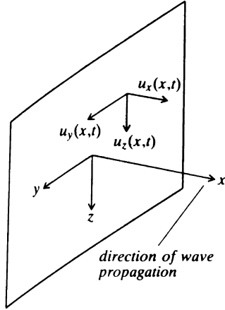
Figure 10.8 Specification of plane waves propagating in the x co-ordinate direction.
