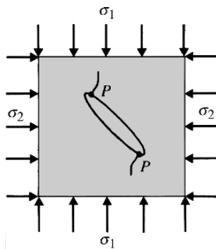
Figure 4.26 Griffith crack model for plane compression.
