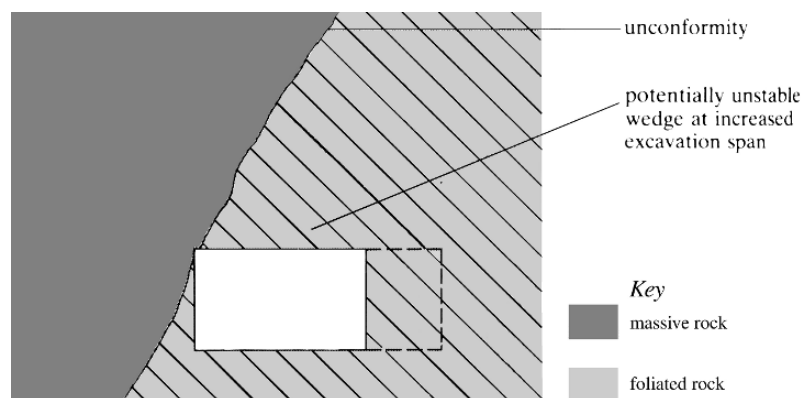
Figure 9.18 Problem geometry demonstrating how an increase in excavation span increases the volume of a roof prism, without comparable increase in the restraining force.
