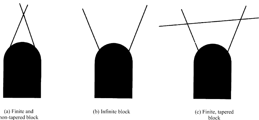
Figure 9.2 Two-dimensional views of types of blocks that can be formed in an excavation boundary.
