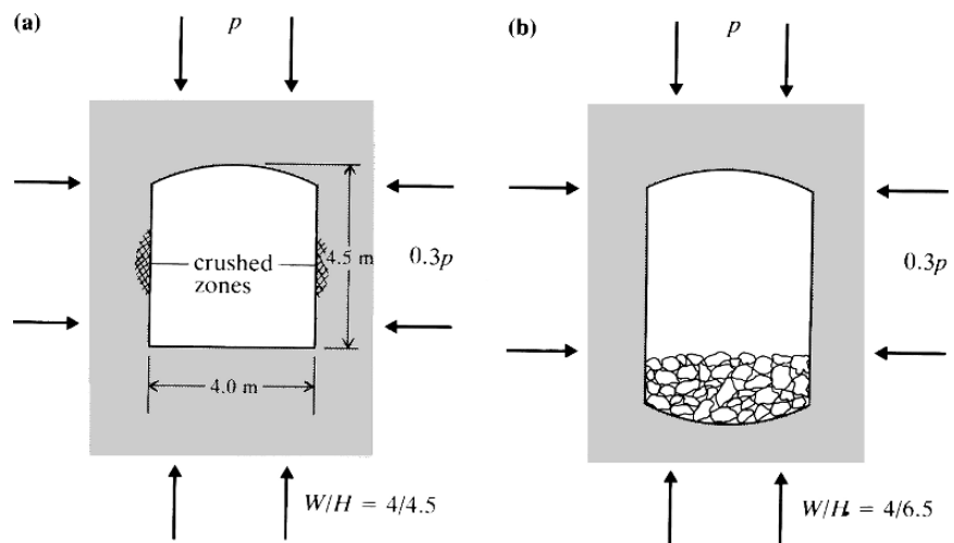
Figure 7.14 Effect of changing the relative dimensions of a mine haulage drive, to mitigate sidewall failure.
