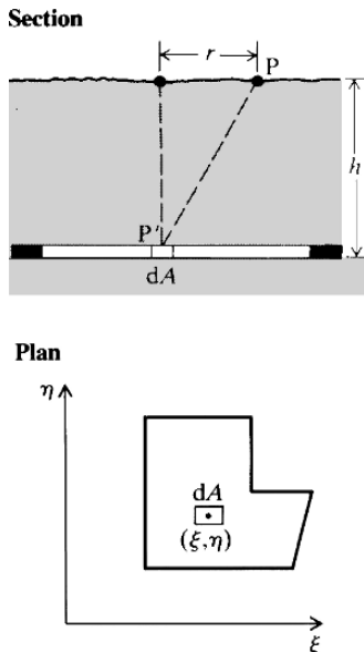
Figure 16.23 Extraction of an element dA (after Berry, 1978).
