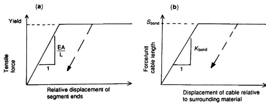
Figure 11.21 (a) Axial performance of a reinforcement segment; (b) shear performance of grout annulus between tendon and borehole surfaces (after Itasca, 2003).
