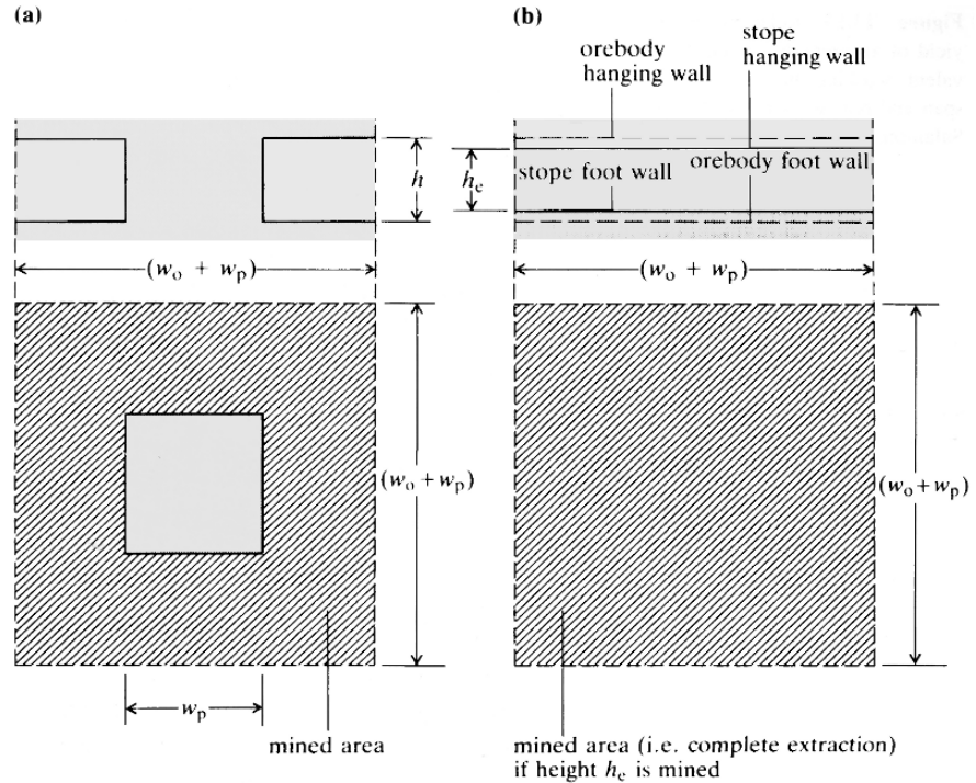
Figure 13.16 Representation of a partial extraction operation (a) in terms of an equivalent volume, total area extraction (b).
