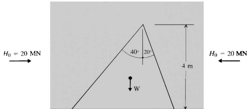
Figure 11.14 Example of a triangular roof prism.
