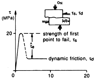
Figure 15.2 Shear stress drop in the transition from static to dynamic conditions on a fault (after Ryder, 1987).
