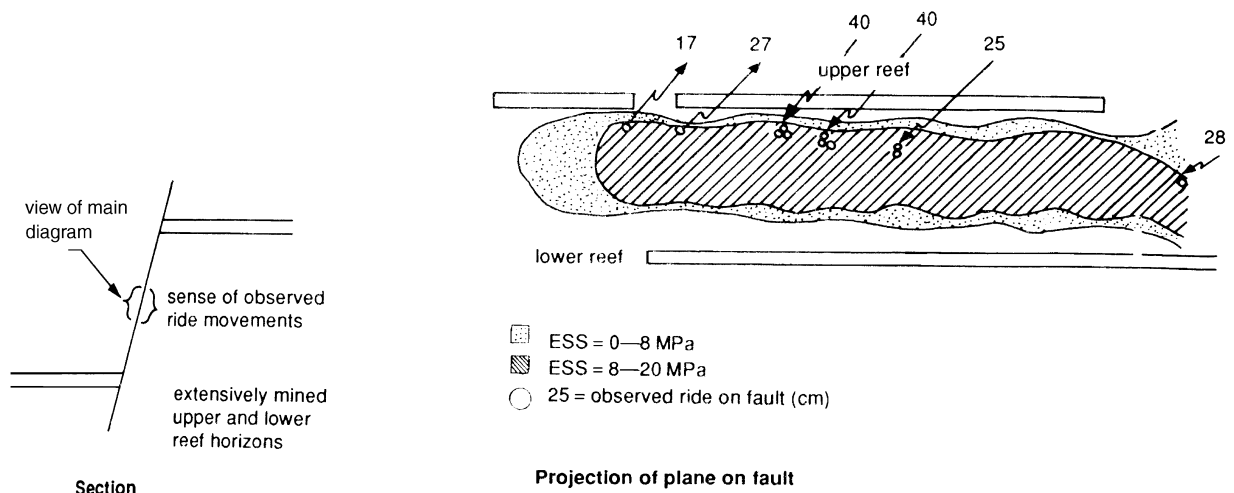
Figure 15.3 Retrospective analysis of a large seismic event in terms of excess shear stress (after Ryder, 1987).
