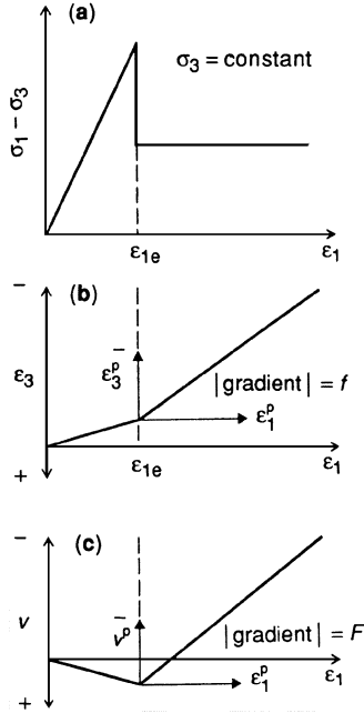
Figure 11.5 Idealised elastic-brittle stress-strain model (after Brown et al. , 1983).
