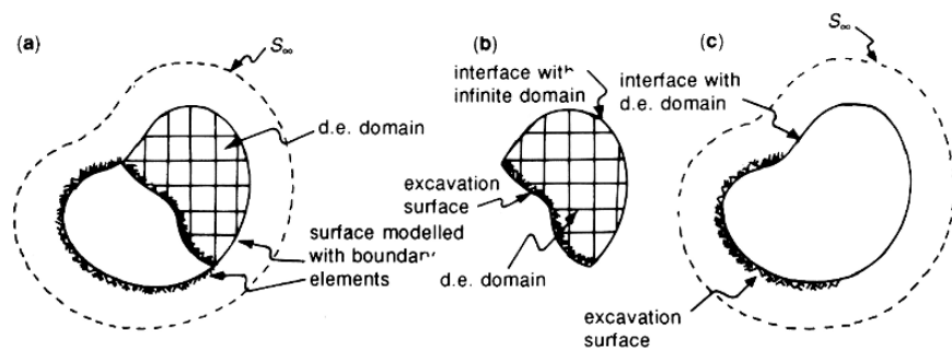
Figure 6.12 Resolution of a coupled distinct element–boundary element problem into component problems.
