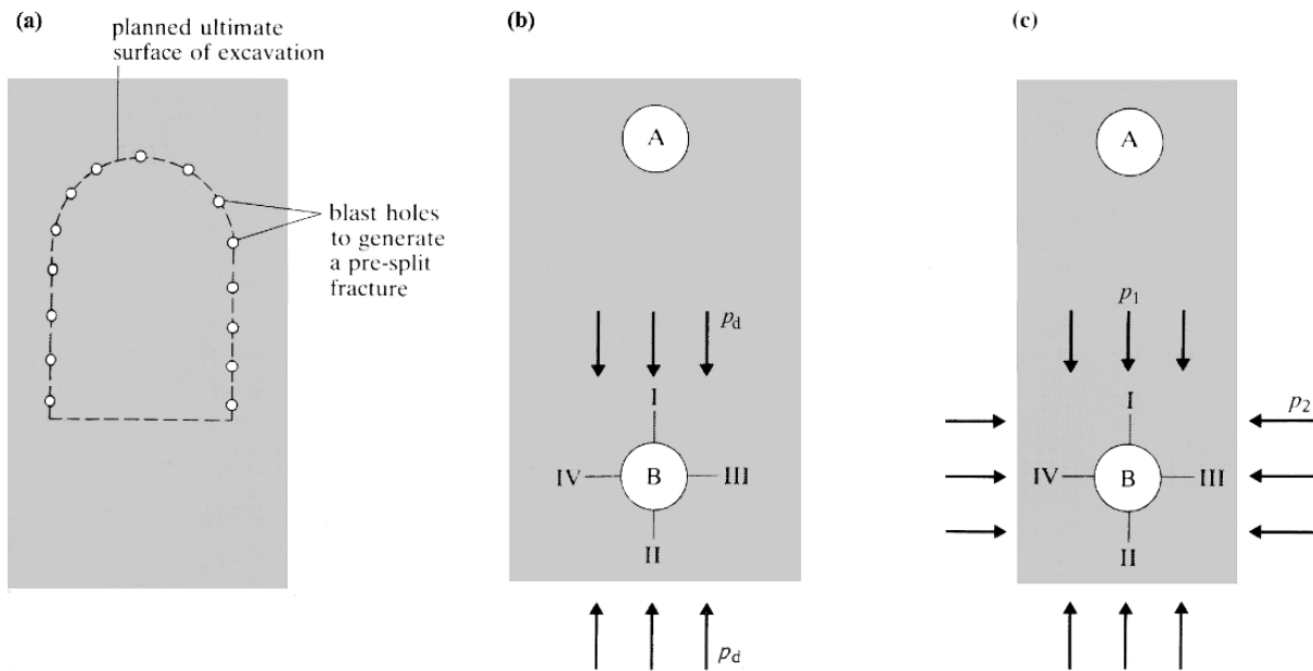
Figure 17.8 Layout of blast holes in a pre-split blast, and transient stress conditions around a blast hole for very short and short delay between initiation of adjacent blast holes.
