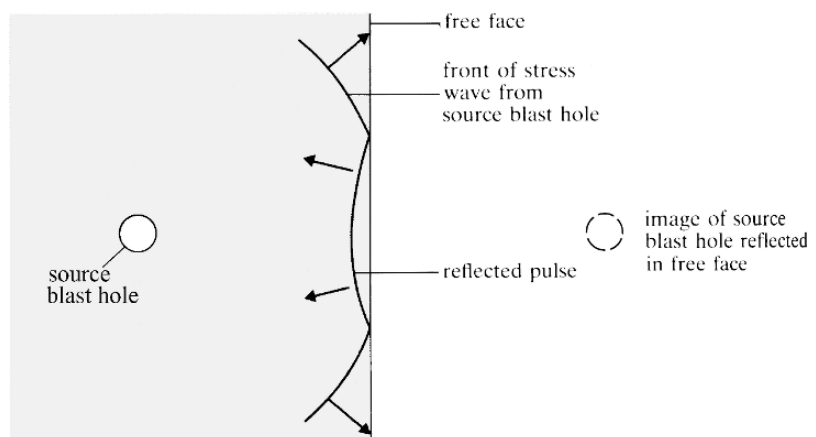
Figure 17.4 Reflection of a cylindrical wave front at a free face.
