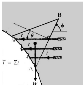
Figure 11.15 Design of a rockbolt or cable system to prevent sliding of a triangular prism (after Hoek and Brown, 1980).
