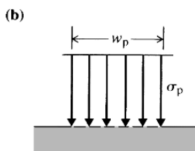
Figure 13.19 Model of yield of country rock under pillar load, and load geometry for estimation of bearing capacity.
