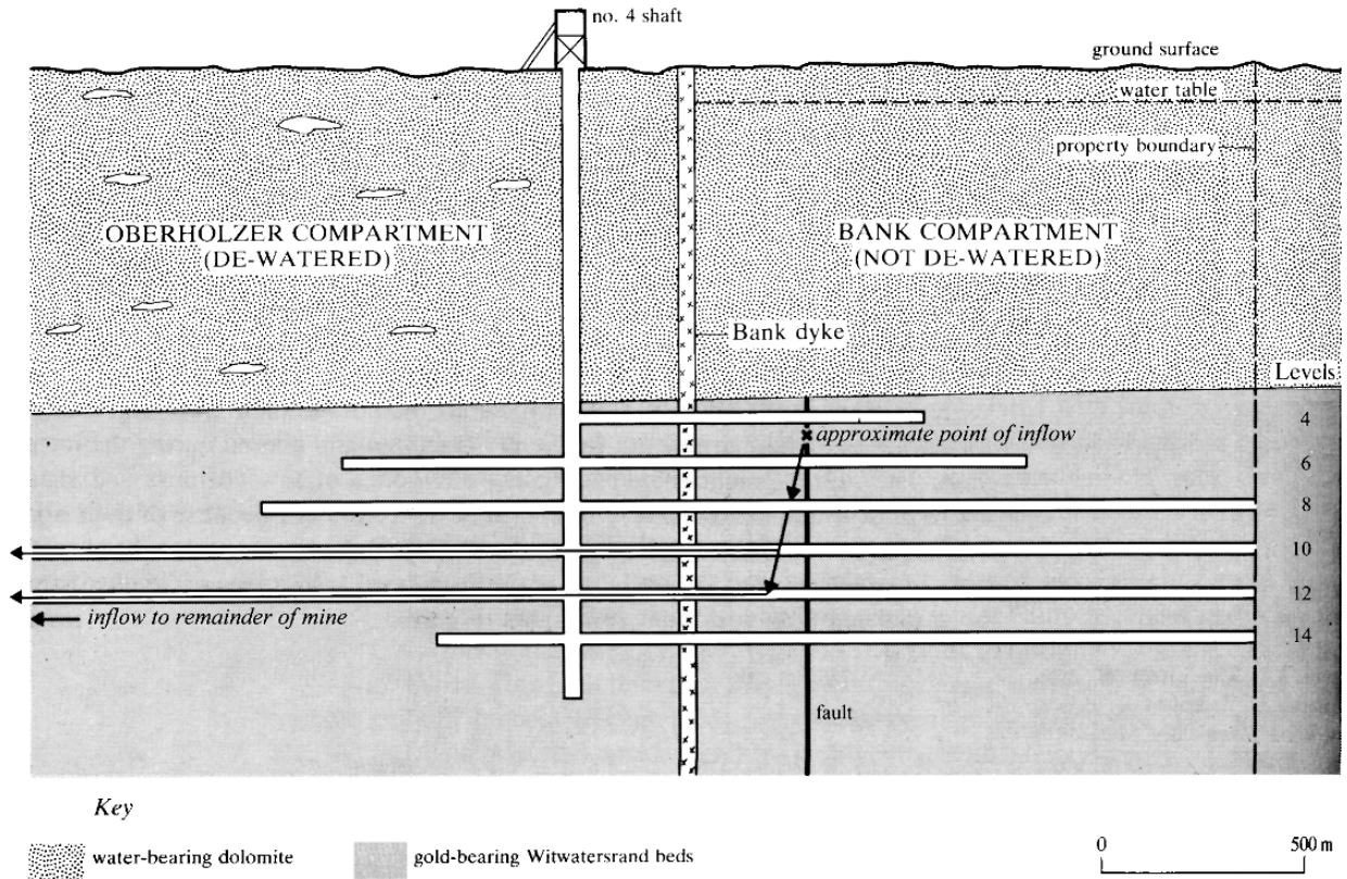
Figure 3.5 Diagrammatic longitudinal section illustrating inrush of water from Bank compartment, West Dreifontein Mine, 26 October 1968. Total inflow was approximately 100 000 gal/day ( \approx 45.5 \times 10^4 l/day) (after Cartwright, 1969).
