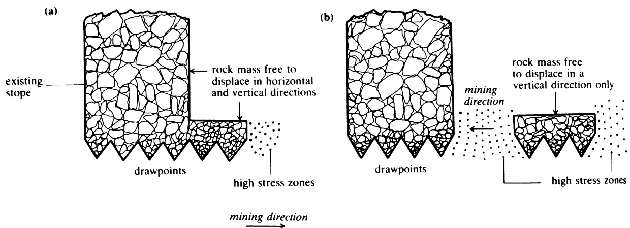
Figure 15.38 The initiation of caving of a block adjacent to an existing caved block for (a) the preferred mining direction, and (b) an unfavourable mining direction (after Ferguson, 1979).
