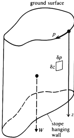
Figure 16.5 General block geometry for limiting equilibrium analysis of chimney caving.
