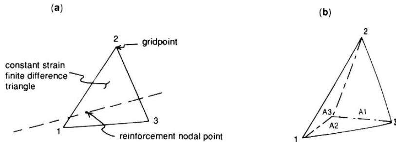
Figure 11.22 Basis of natural co-ordinates for interpolating rock displacements (after Itasca, 2003).
