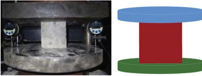
Figure 5.92 Test setup of uniaxial compression test.
