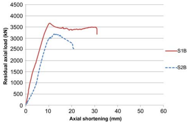
Figure 5.42 Effect of axial load on residual performance.
