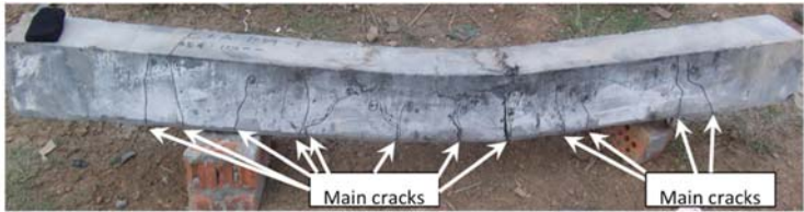
U6A specimen with 1000 kN axial load under 70 kg charge weight loading
