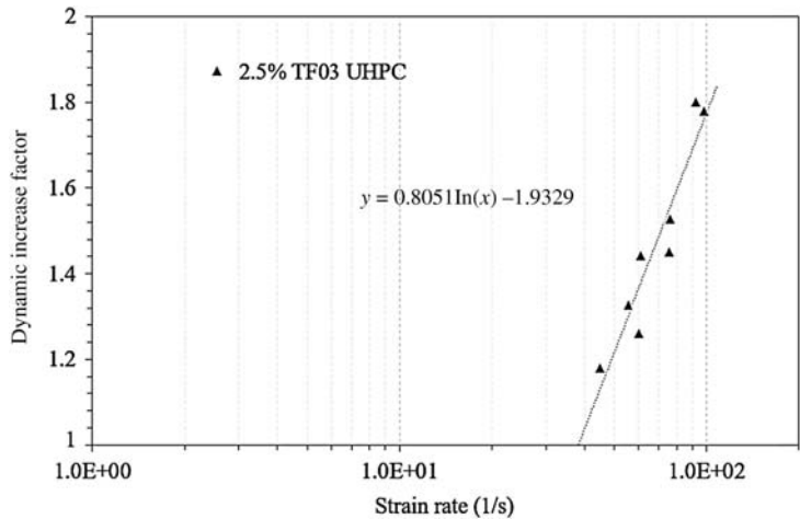
Figure 4.32 DIFs for UHPC under compression.
