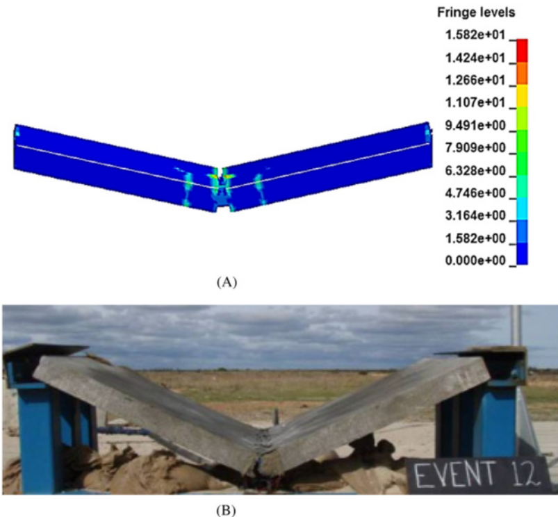
Figure 3.11 UHPC-D3B response: (A) numerical observation and (B) experimental observation.
