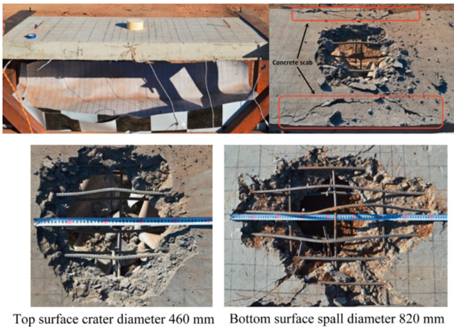
Figure 3.32 Blast event 2.
