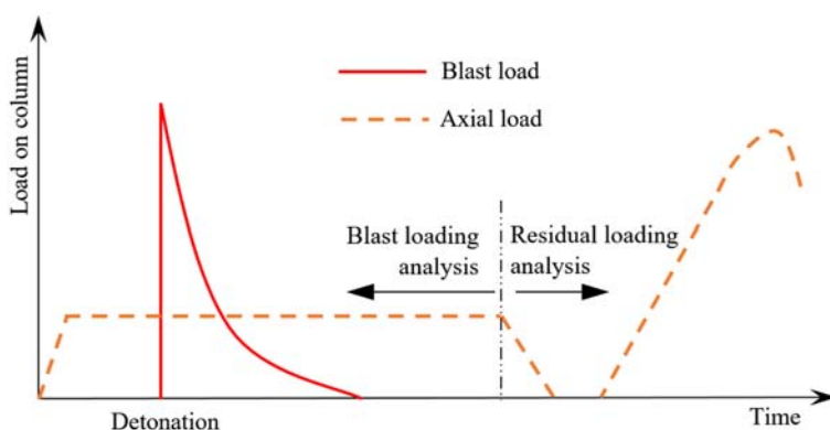
Figure 4.41 Schematic loading on UHPC column.
