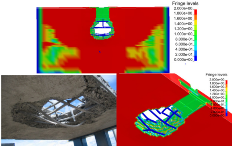
Figure 3.25 Slab NSC bottom response.
