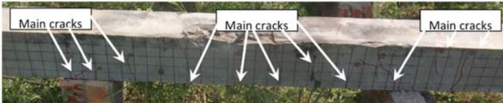
H7B specimen with no axial load under 11.2 kg charge weight loading
