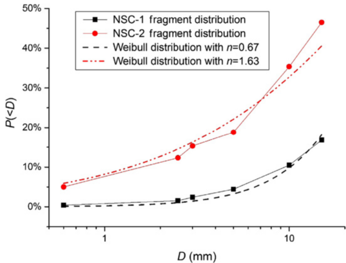
Figure 3.44 Weibull distribution for fragments from NSC specimens.
