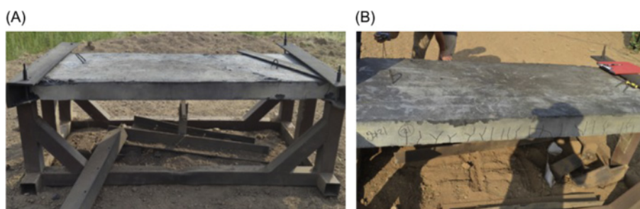
Figure 3.57 SWM-SF slab after 12 kg TNT detonation from 1.5 m standoff distance: (A) SWM-SF slab after test and (B) crack distribution on the slab.
