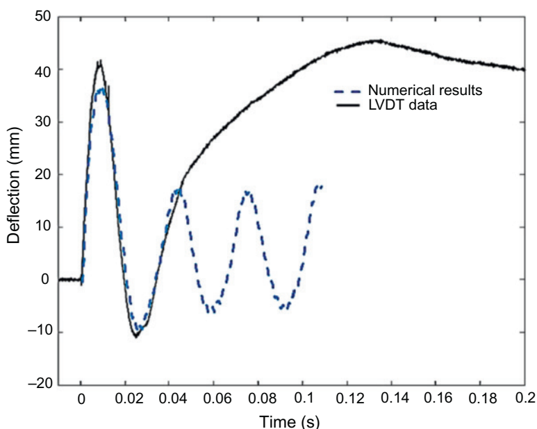
Figure 3.14 UHPC-D2 response.
