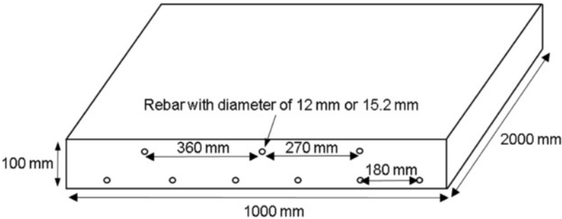
Figure 3.1 Slab dimension and reinforcement.
