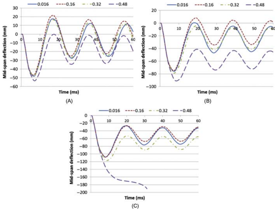
Figure 5.103 Displacement–time histories for different axial load ratios: (A) 80 kg TNT, (B) 120 kg TNT, and (C) 160 kg TNT.
