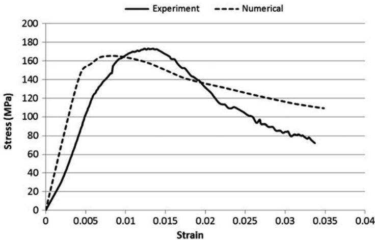
Figure 5.93 Uniaxial compression test results.
