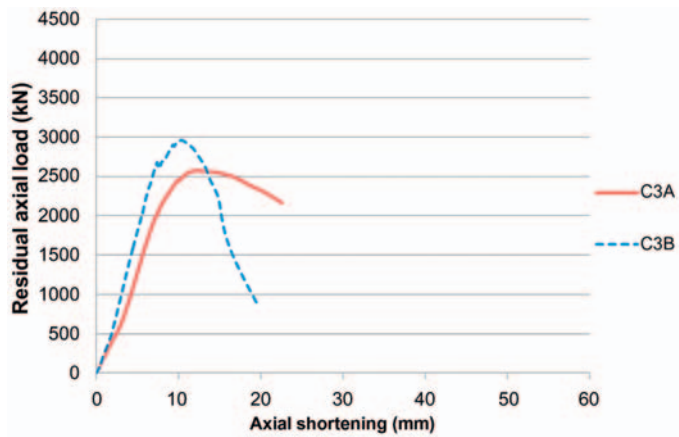
Figure 5.41 Effect of hollow core on residual performance.
