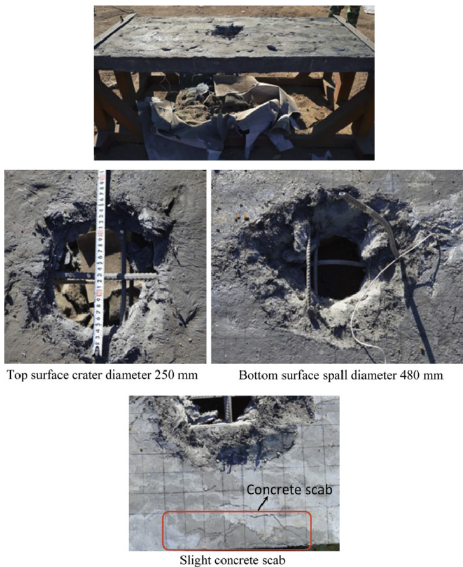
Figure 3.37 Blast event 7.
