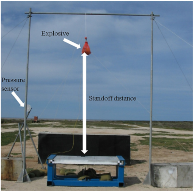
Figure 3.3 Testing system.
