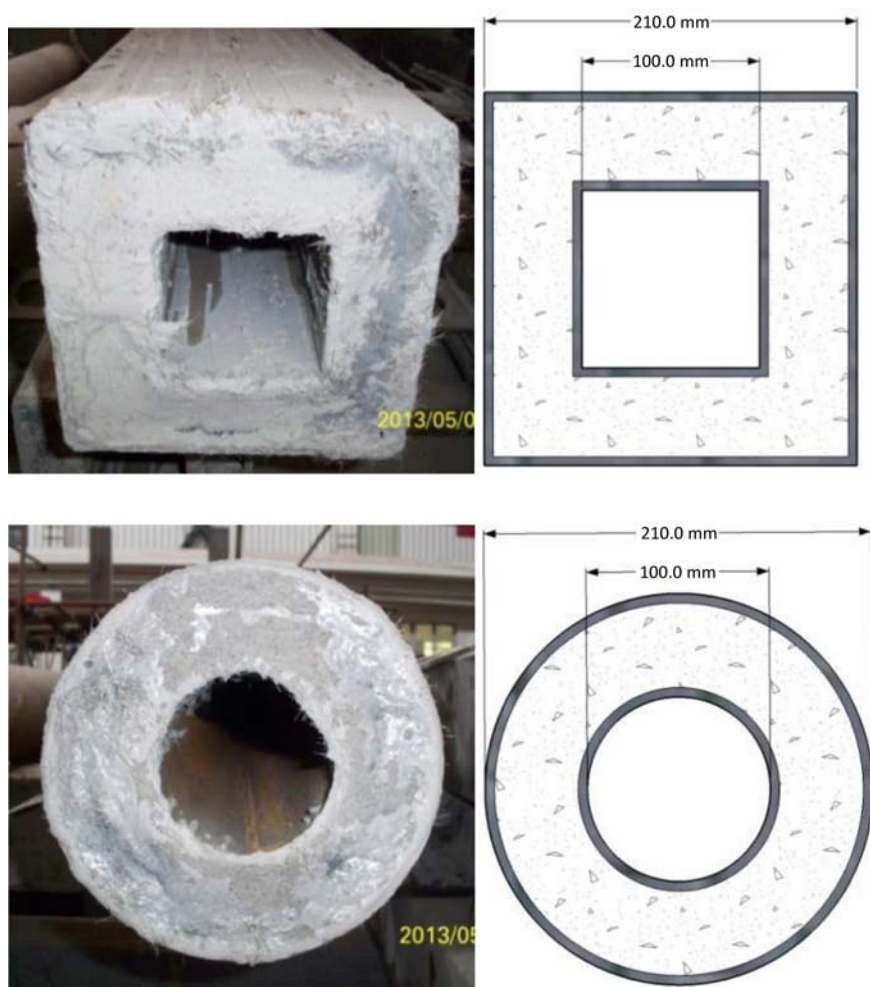
Figure 5.14 Cross-sections of a square and a circular CFDST specimen.
