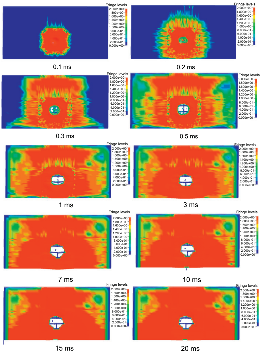
Figure 3.24 Slab NSC top surface response.
