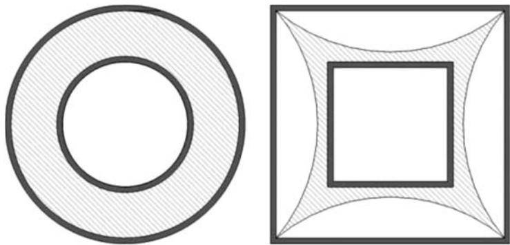
Figure 5.78 Effective confinement area ( shaded ) for both circular and square cross-section [37].
