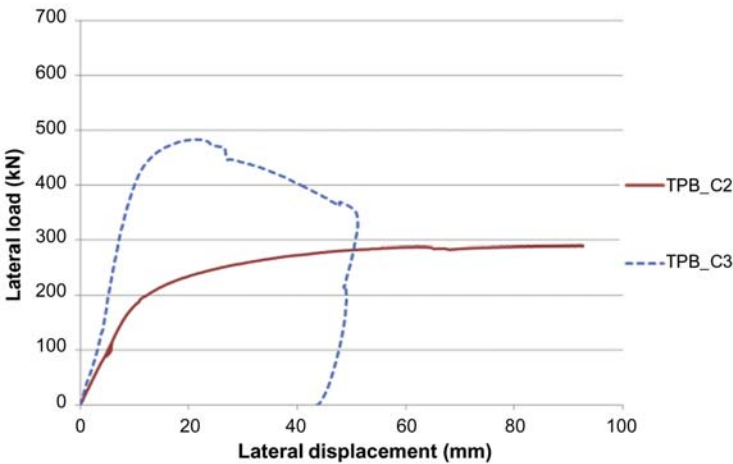
Figure 5.30 Effect of axial load.
