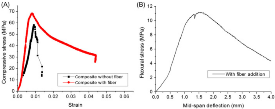
Figure 3.47 Static performance of concrete composite reinforced with 2.0% 12 mm fiber: (A) compressive stress–strain curve and (B) flexural strength.
