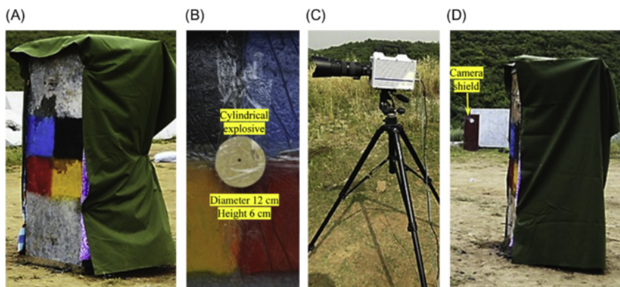
Figure 3.72 Test setup and high speed camera: (A) frame with canvas cover, (B) 1 kg TNT, (C) Photron SZ, and (D) slab ready for test.
