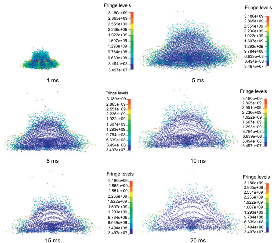
Figure 3.23 Explosion expansion.
