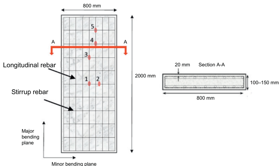
Figure 3.29 Slabs configuration.
