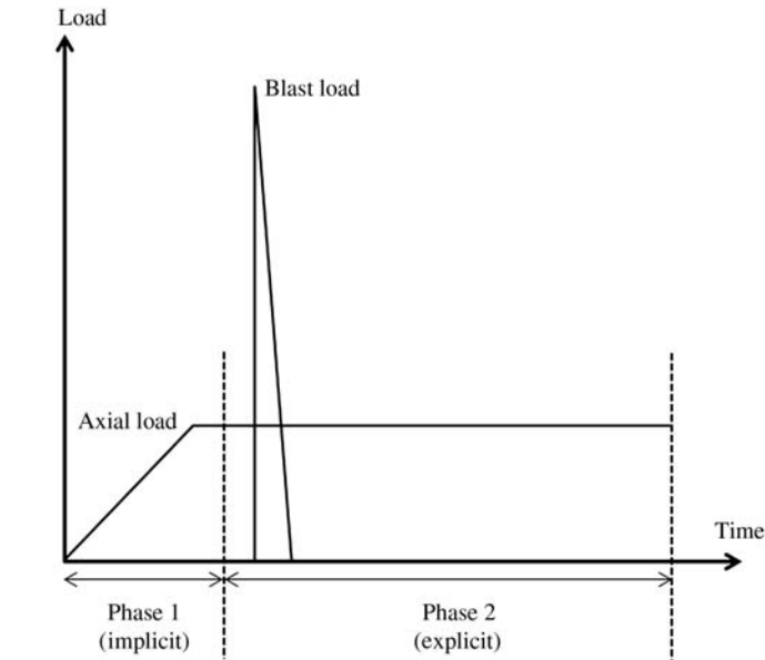
Figure 5.83 Two loading phases (not to scale).
