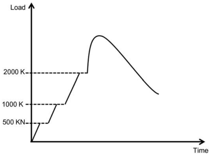
Figure 5.37 The loading schematic for residual capacity test.
