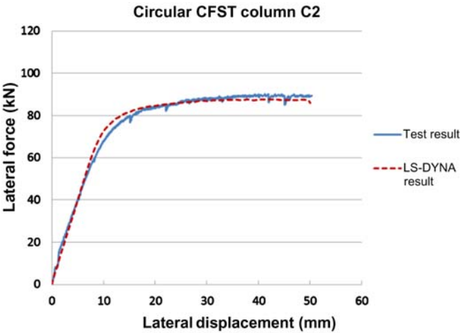
Figure 5.49 Comparison between the numerical results and test results for column C2.
