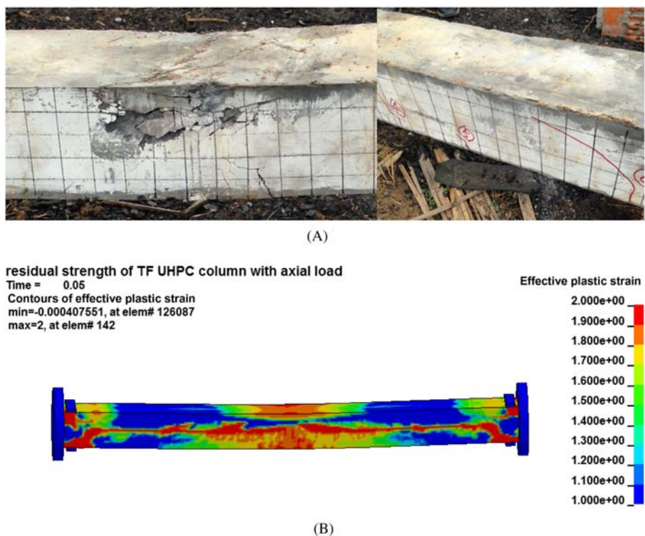
Figure 4.39 Column damage after 35 kg TNT equivalence detonation at 1.5 m standoff. (A) Field damage observation and (B) Numerical damage prediction.
