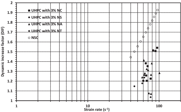
Figure 2.17 Comparison of DIF curves between NSC and UHPC.
