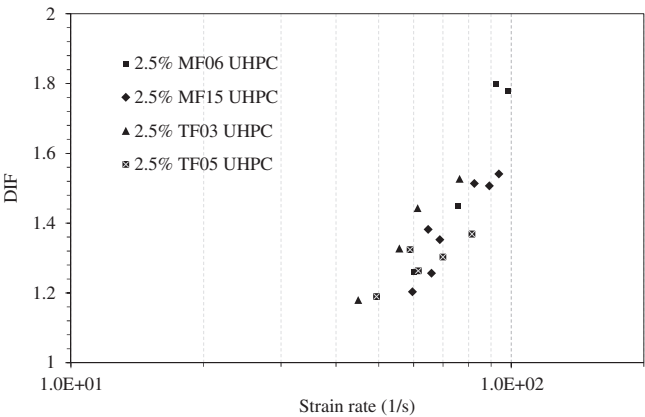
Figure 2.34 DIF curves of UHPC with various types of fibers.
