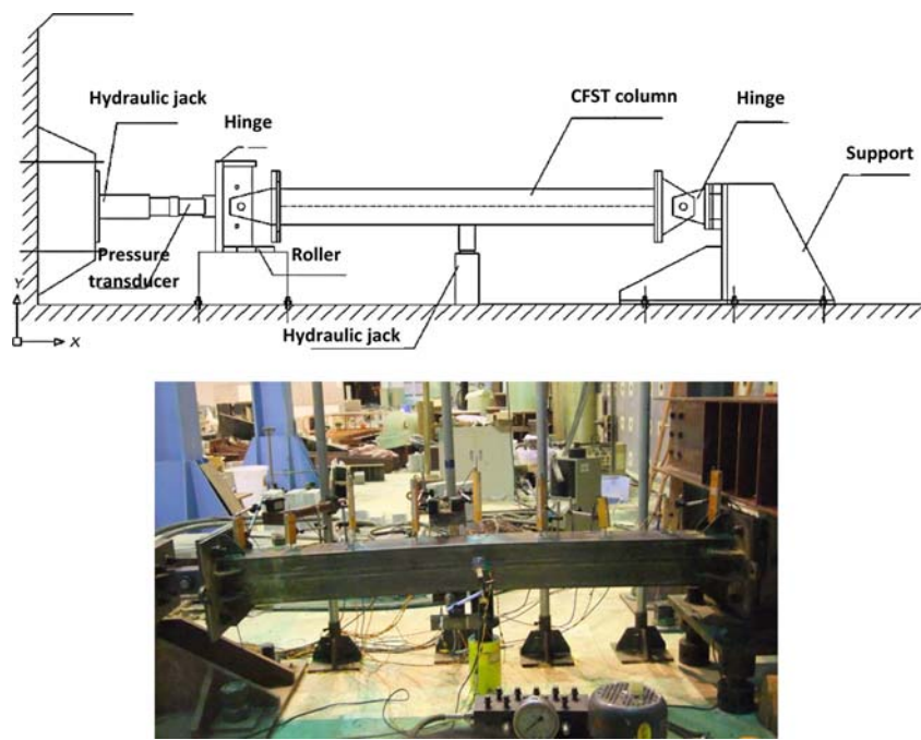
Figure 5.1 Experimental setup for three-point bending test.
