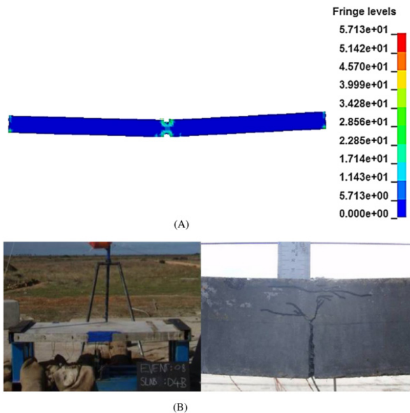
Figure 3.12 UHPC-D4 response: (A) numerical observation and (B) experimental observation.
