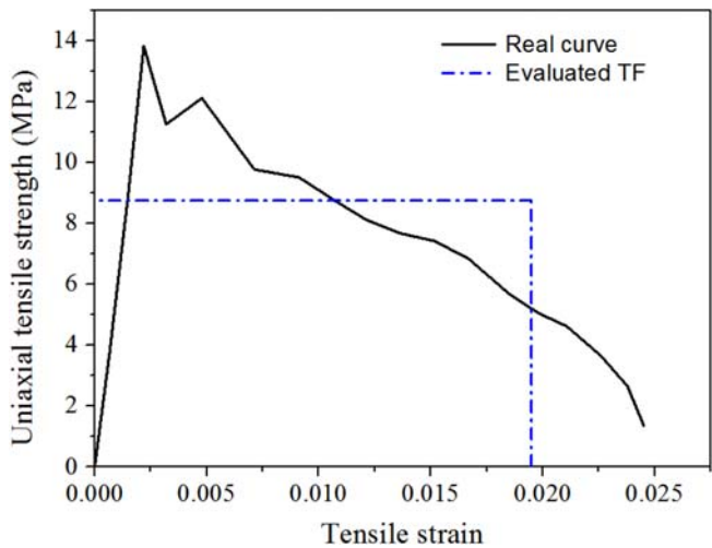
Figure 4.31 Inverse analysis on FPBTs.
