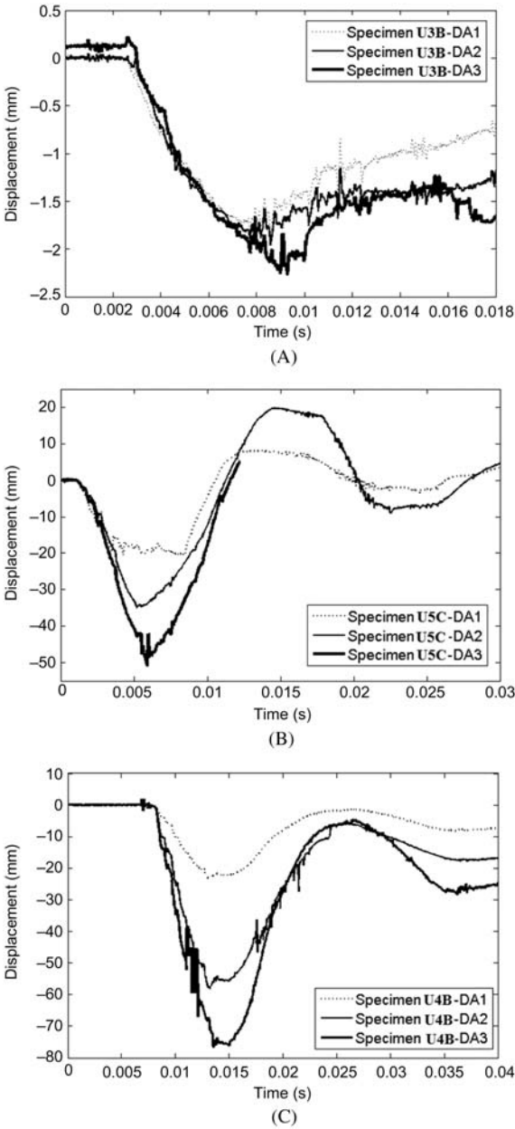
Figure 4.8 Deflection-time profiles recorded on UHPC columns with TF reinforcement. (A) 1.4 kg explosive on U3B. (B) 35 kg explosive on U5C, and (C) 48 kg explosive on U4B.
