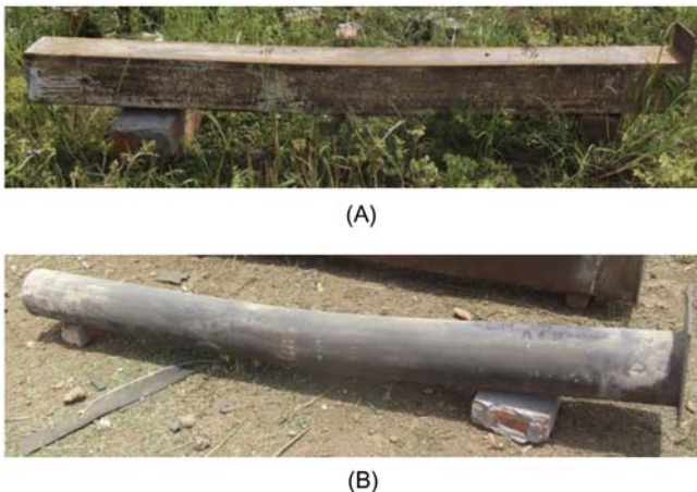
Figure 5.25 Deformed shapes of specimens S1A and C1A: (A) S1A and (B) C1A.
