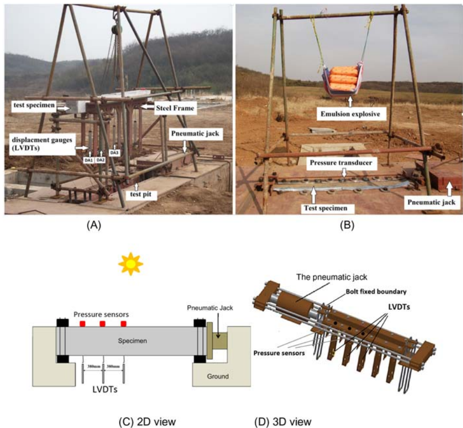
Figure 4.5 Blast test setup (A) before, (B) after the specimen being installed into the test pit, (C) 2D view of test, and (D) 3D view of the test.
