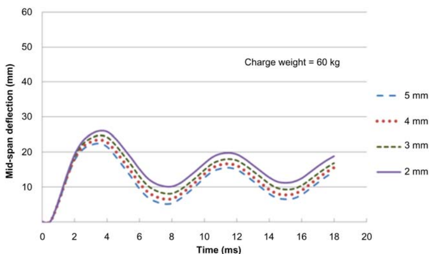
Figure 5.71 Influence of inner tube thickness when charge weight = 60 kg.
