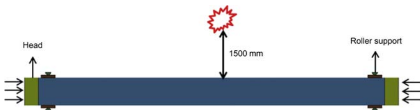
Figure 5.51 The numerical model for the blast test.
