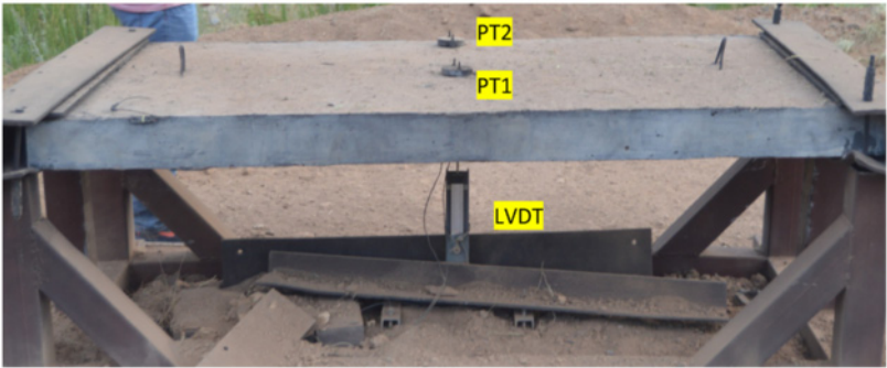
Figure 3.81 Pressure sensor installation on the UHMWPE-1 slab under 6 kg TNT at 1.5 m standoff distance.
