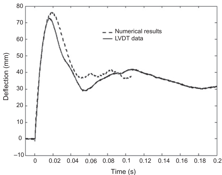
Figure 3.16 UHPC-D4 response.
