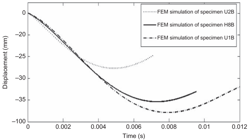
Figure 4.53 Deflection-time histories of FEM prediction of UHPFRC and HSRC columns under 35 kg charge weight.
