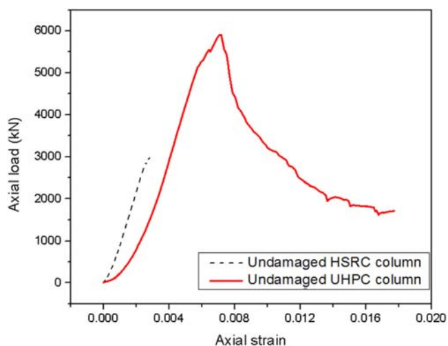
Figure 4.18 Axial load–strain relationships of undamaged columns.
