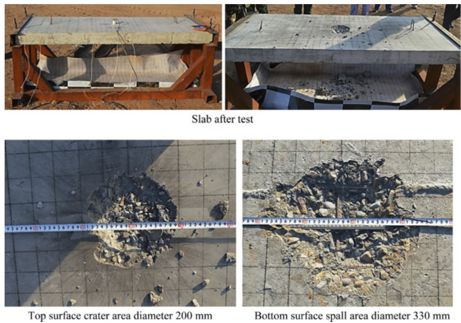
Figure 3.31 Blast event 1.
