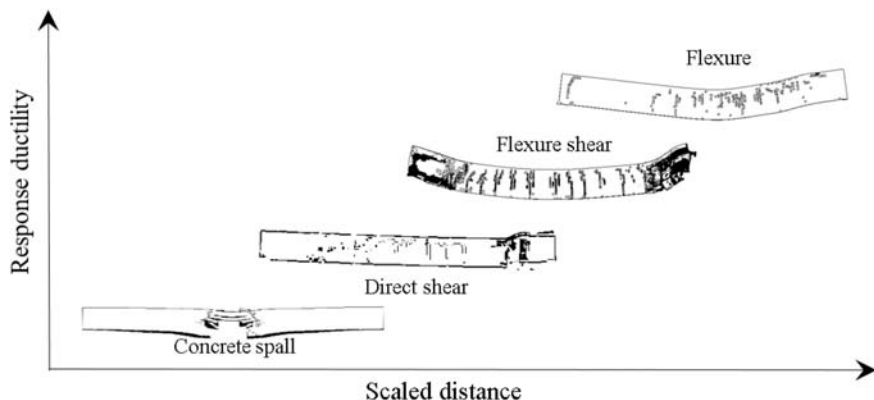
Figure 1.6 Structural-member failure modes under blast loads [68].
