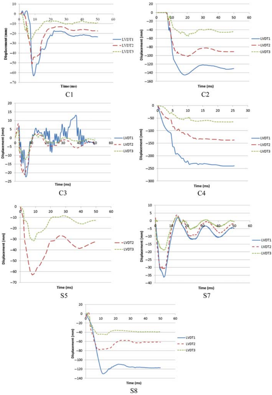
Figure 5.4 Displacement–time histories.
