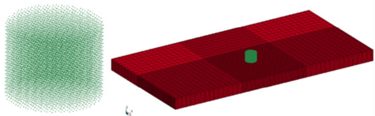
Figure 3.22 Coupled FE model and SPH particles.
