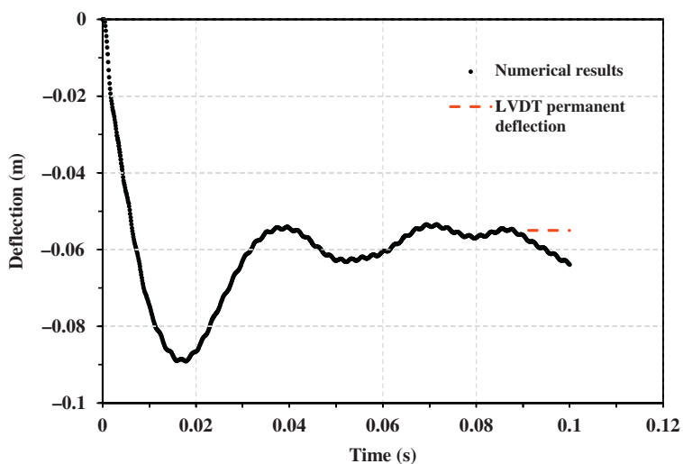
Figure 3.13 UHPC-D1 response.
