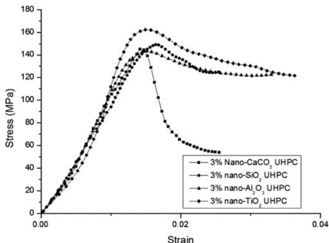
Figure 2.9 Stress—strain curves from quasi-static compressive tests.
