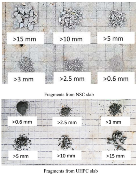
Figure 3.41 Samples of fragments with different sizes.
