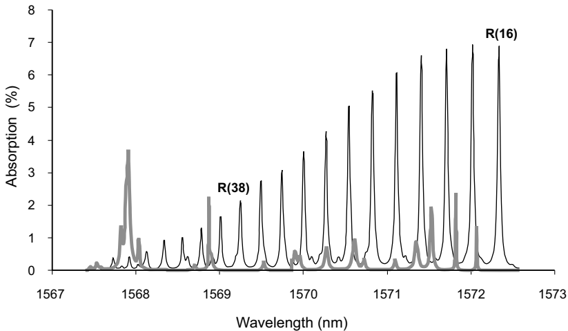
Fig. 3.3. Rotational structure of the 301-100 \text{CO}_2 vibration band overlapped by water vapour rotational lines (absorption lines R38 and R16 are free from interference)
