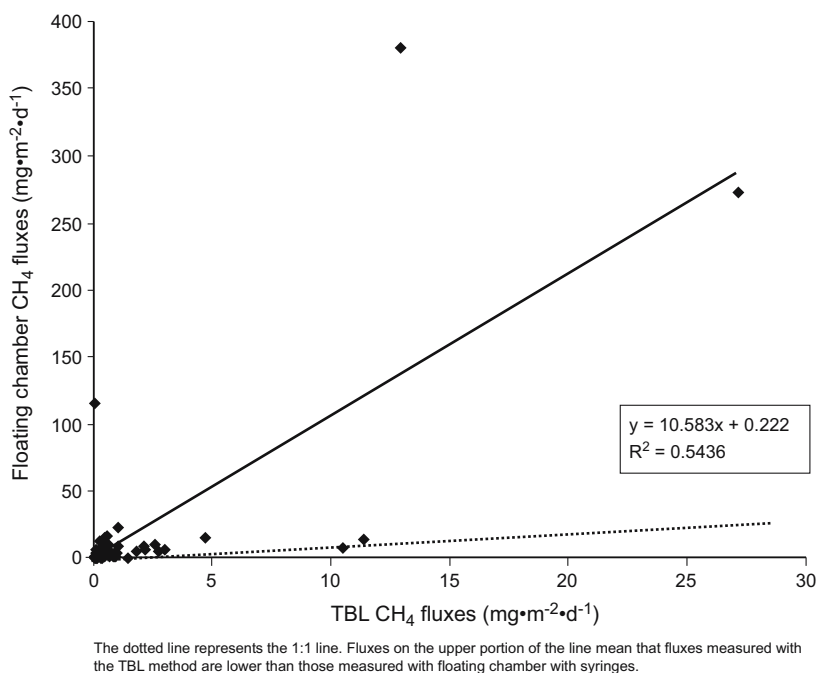
Fig. 2.5. Comparison of CH 4 fluxes (mg·m -2 ·d -1 ) measured with TBL and with floating chambers with syringes
