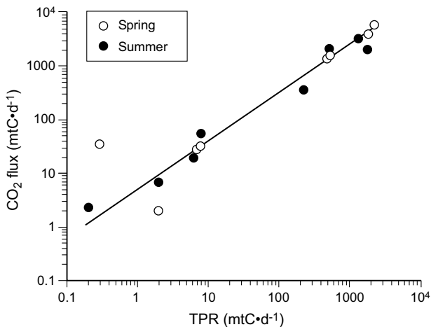
Fig. 20.9. Relationship between evasive CO 2 flux and the total plankton respiration (TPR) for the four reservoirs and four lakes in the LG-2 region for spring (○) and summer (●)
