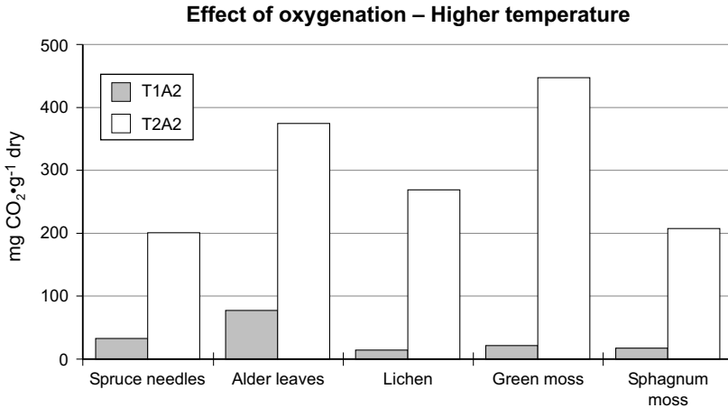
Fig. 13.16 Effect of the level of dissolved oxygen on the production of carbon dioxide from vegetation samples immersed in water during 345 days under higher temperature
