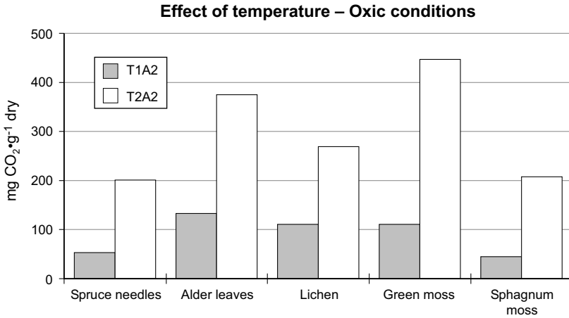
Fig. 13.14 Effect of temperature on the quantities of carbon dioxide produced from vegetation samples immersed in water during 345 days under oxitic conditions
