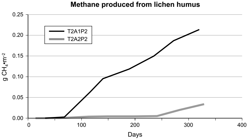
Fig. 13.4 Evolution of methane produced from lichen humus under different sets of experimental conditions
