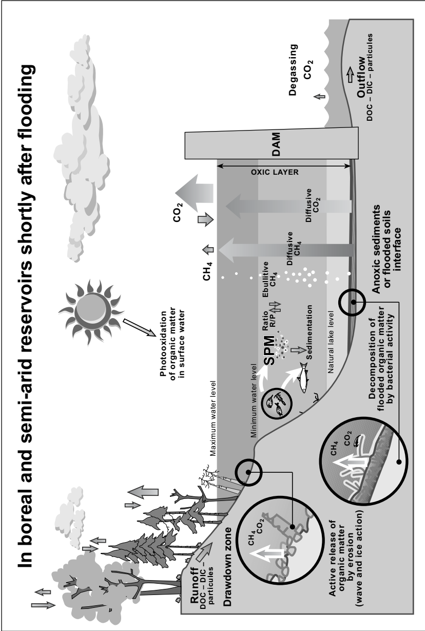
Fig. 26.2. Major processes occurring in boreal and semi-arid reservoirs shortly after flooding (<10 years)
