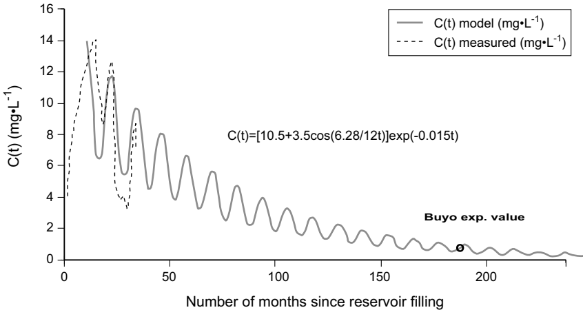
Fig. 12.2. Modeled Variations of dissolved \text{CH}_4 concentrations in the Petit Saut reservoir over a 20-year period based on the three first years of measurements and data from an older reservoir with similar characteristics, in Ivory Coast (Buyo)
