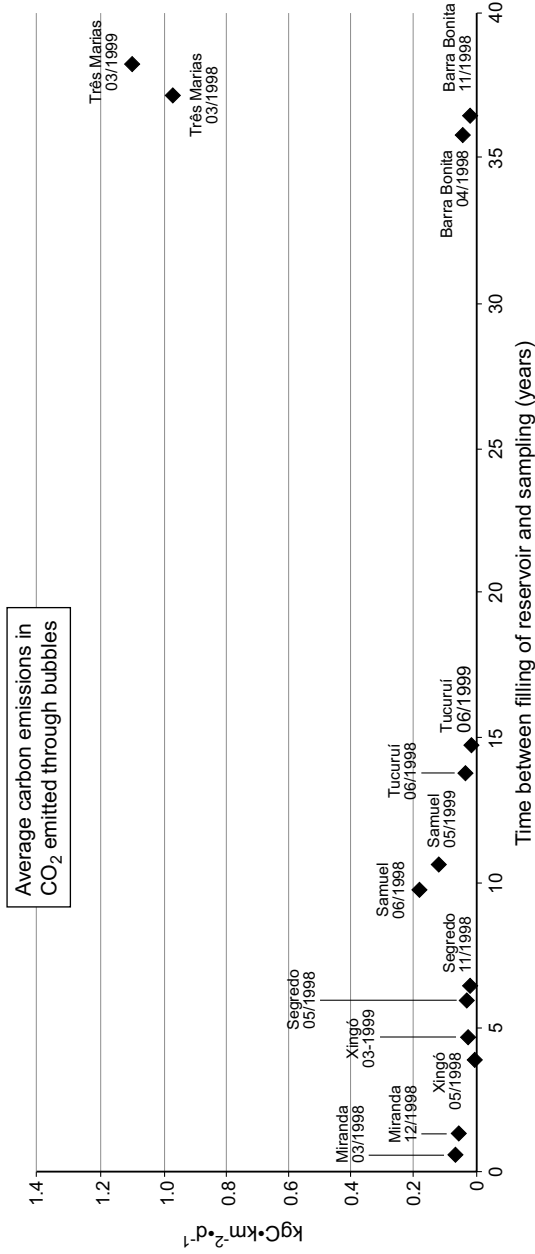
Fig. 11.4. Average carbon emissions in CO 2 emitted through bubbles in seven Brazilian hydroelectric reservoirs
