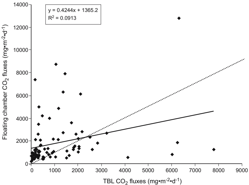
Fig. 2.4. Comparison of \text{CO}_2 fluxes ( \text{mg}\cdot\text{m}^{-2}\cdot\text{d}^{-1} ) measured with TBL and with floating chambers with syringes
