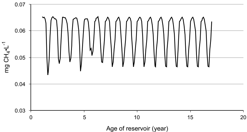
Fig. 25.16. Concentration of dissolved \text{CH}_4 in the surface water layer as computed by the model for zone 4 of the nine zone segmented Robert-Bourassa reservoir
