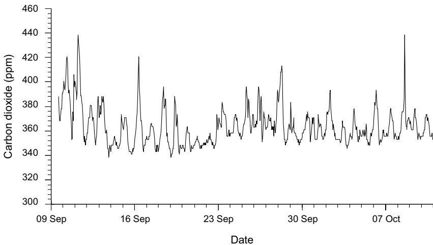
Fig. 23.4. \text{CO}_2 in air at the fresh air intake of the Freshwater Institute, Winnipeg, MB, Canada. Measured with a Li-Cor LI-6262 IRGA
