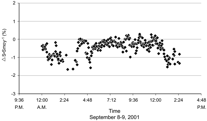
Fig. 3.16. CO 2 concentration gradients (an example of mainly negative values) measured at Robert-Bourassa hydroelectric reservoir. September 9, 2001
