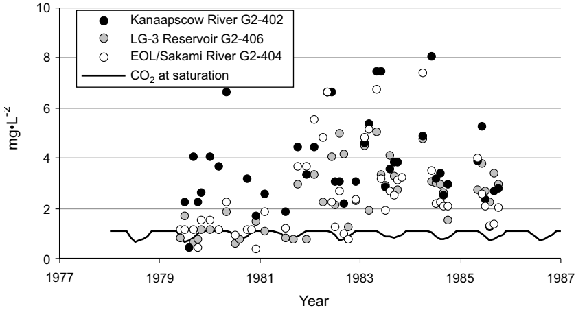
Fig. 25.9. Concentrations of carbon dioxide in the influents to Robert-Bourassa reservoir as calculated from measurements of C_{\text{INORG}} and \text{HCO}_3
