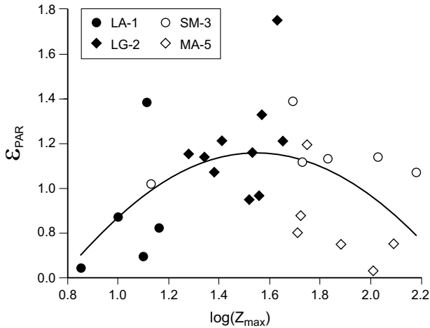
Fig. 20.8. Relationship between the light extension coefficient (ε PAR ) and log 10 maximum depth (Z max ) for reservoir stations (LA-1 = ●, LG-2 = ■, SM-3 = ○ and MA-5 = □)
