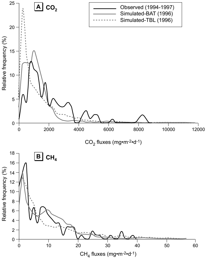
Fig. 24.2. Relative frequencies of observed and simulated CO 2 and CH 4 surface fluxes, LA-1 reservoir
