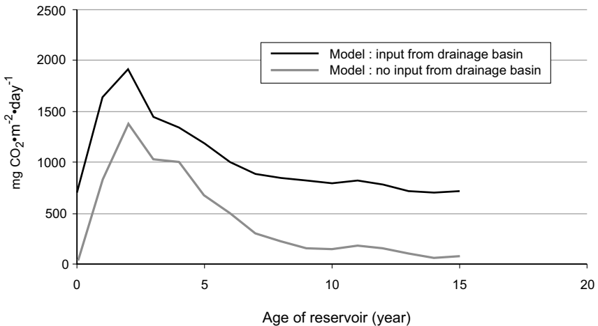
Fig. 25.15. Yearly averaged fluxes of \text{CO}_2 emitted from zone 4 of the Robert-Bourassa reservoir considering the influent influx of \text{CO}_2 from the drainage basin or neglecting it completely (influent dissolved \text{CO}_2 at equilibrium with the atmospheric \text{CO}_2 only)
