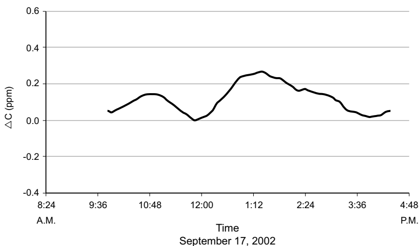
Fig. 3.5. Temporal variations of positive \text{CH}_4 concentration gradients recorded at Lake Piché, Montmorency Forest experimental site, September 17, 2002
