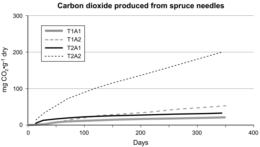
Fig. 13.7 Evolution of carbon dioxide produced from spruce needles under different sets of experimental conditions
