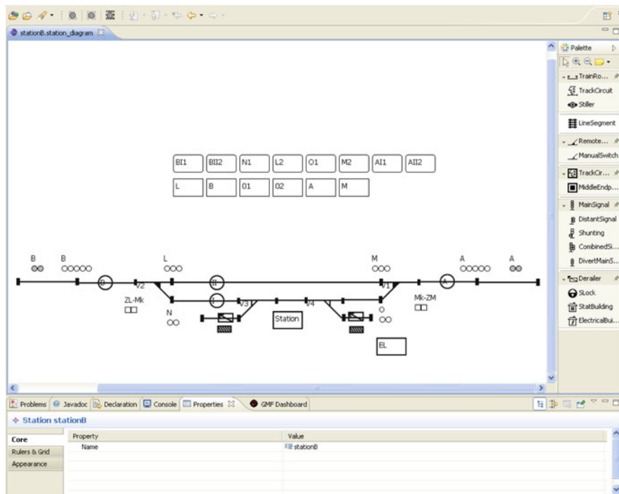
Fig. 4 TCL editor
