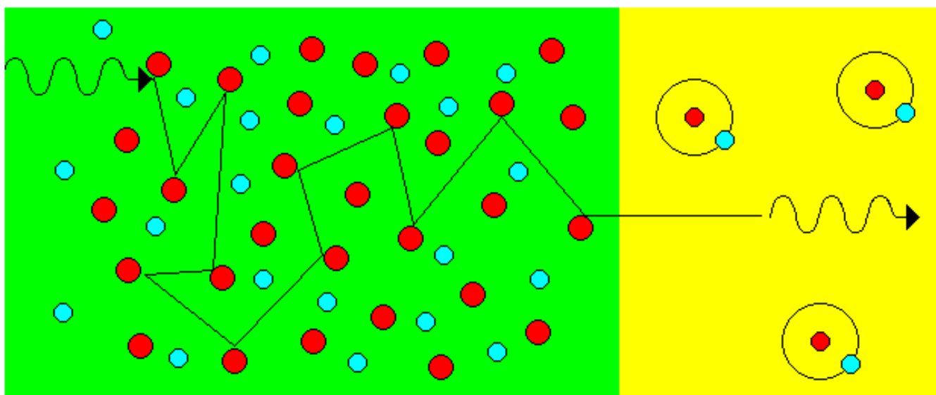
atomic hydrogen
