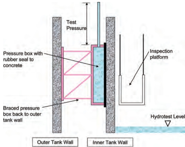
Fig. 12.2.5.1(a)—General layout of external pressure box test.
