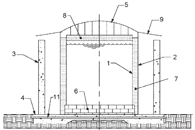
Fig. RA.1b(a)—Double-containment tank system with elevated slab and no slab heating.
