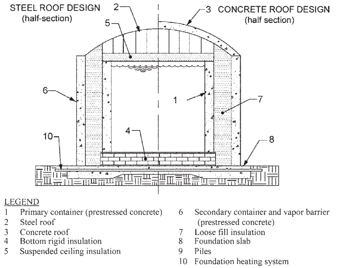
Fig. RA.1e(b)—Full-containment concrete tank system with heated slab.
