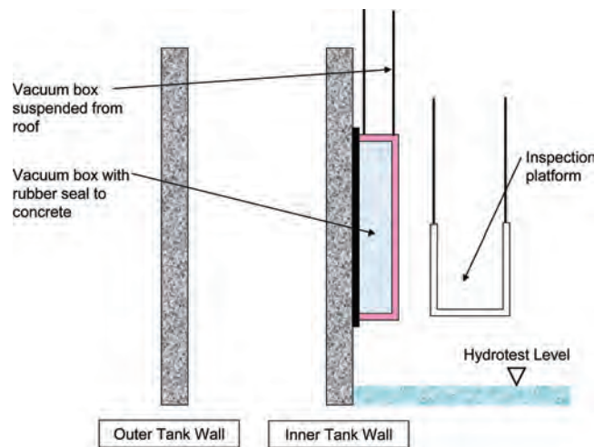
Fig. 12.2.5.1(b)—General layout of internal vacuum box test.
