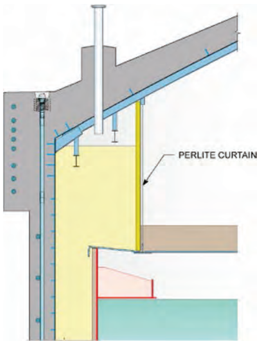
Fig. RA.2a(b)—Example of fixed-base full containment for LNG—detail at roof.
