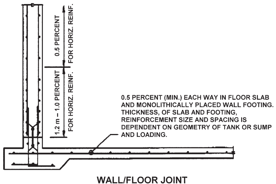
Fig. R9.2.2.2—Recommendations for increased reinforcing percentage parallel to bonded joints.
