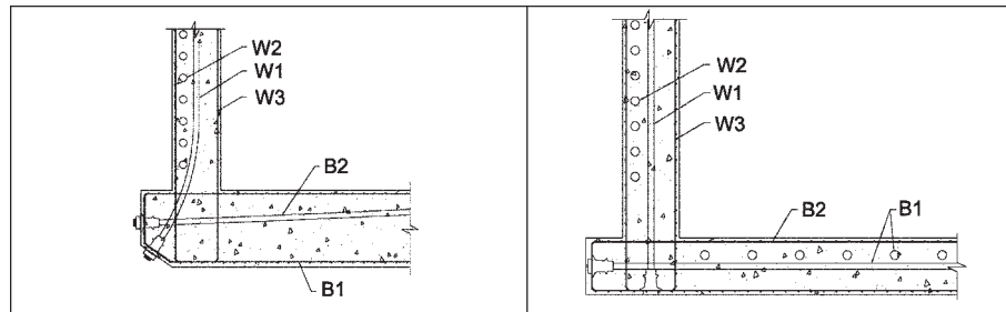
Fig. RA.3c—Example of sliding wall-to-base joint details.
