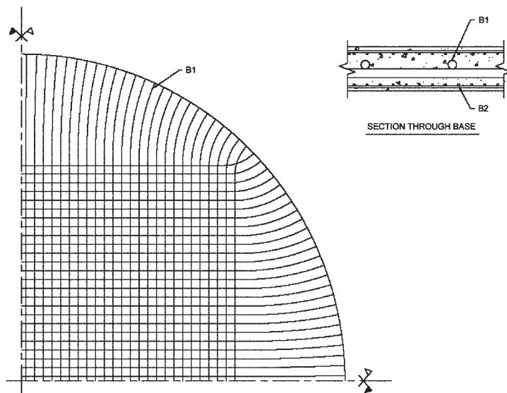
Fig. RA.3d—Examples of tendon prestressing details.
