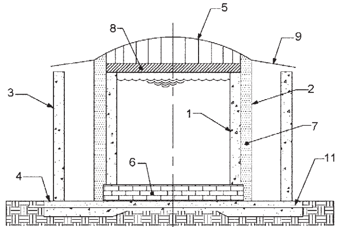
Fig. RA.1c(a)—Double-containment concrete tank system with elevated slab and no slab heating.
