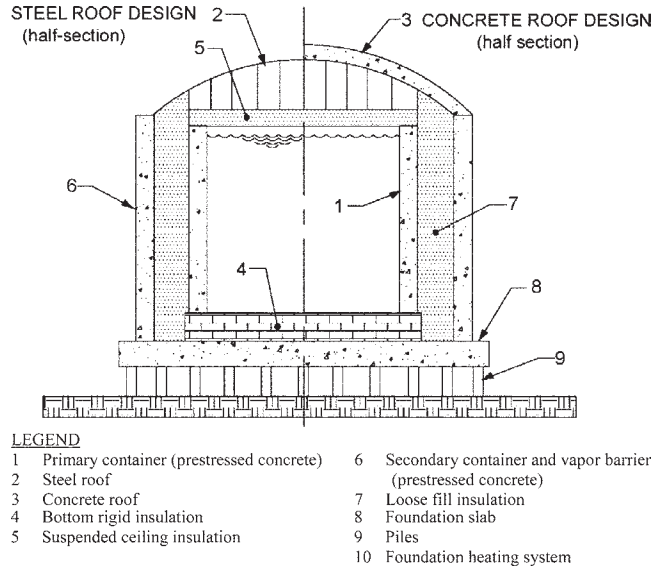
Fig. RA.1e(a)—Full-containment concrete tank system with elevated slab and no slab heating.
