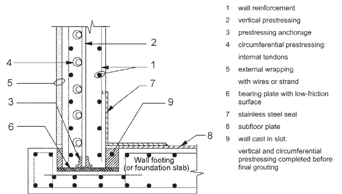
Fig. RA.3b—Example of pinned wall-to-base joint details.
