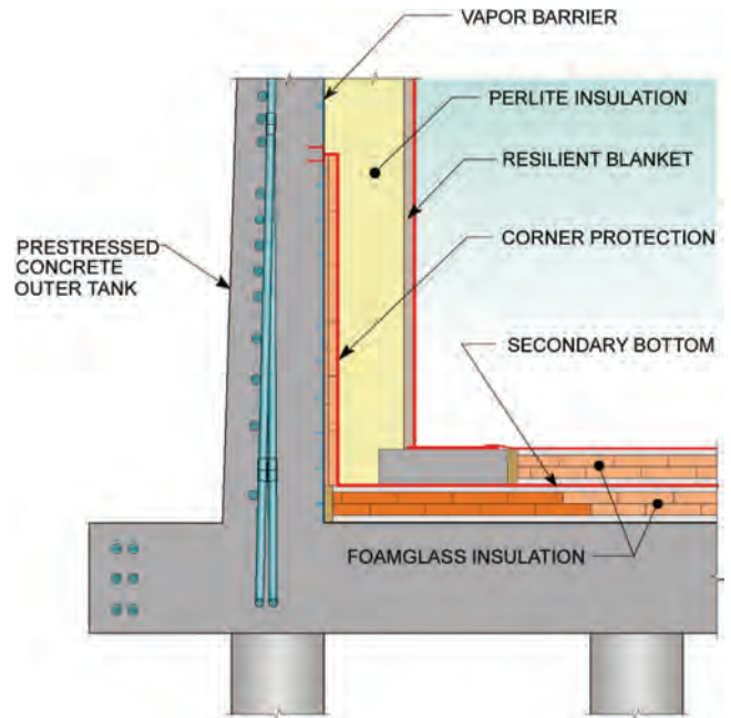
Fig. RA.2a(c)—Example of fixed-base full containment for LNG—detail at foundation.
