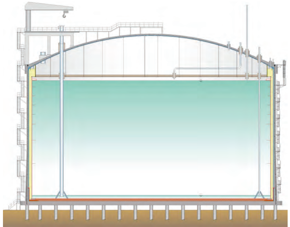
Fig. RA.2a(a)—Example of fixed-base full containment for LNG (internally prestressed concrete secondary outer tank and 9-Ni steel primary tank).
