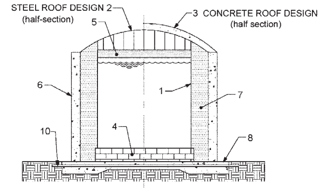
Fig. RA.1d(a)—Full-containment tank system with elevated slab and no slab heating.
