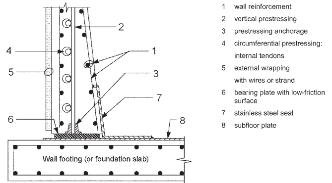
Fig. RA.3c—Example of sliding wall-to-base joint details.
