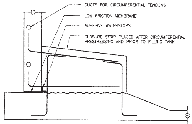
Fig. RA.3a(b)—Example of fixed wall-to-base joint details (closure strip).
