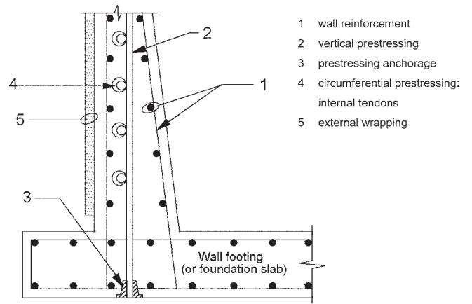
Fig. RA.3a(a)—Example of fixed joint details (monolithic construction).
