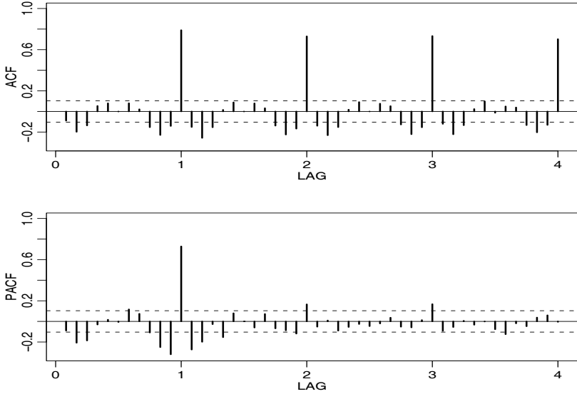
Fig. 3.23. ACF and PACF of differenced production, (1 - B)x_t .
