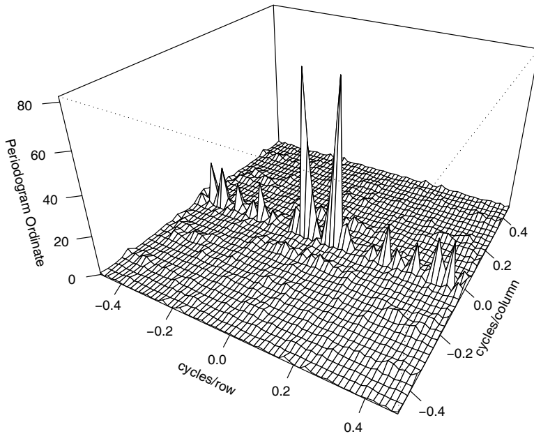
Fig. 4.30. Two-dimensional periodogram of soil temperature profile showing peak at .0625 cycles/row. The period is 16 rows, and this corresponds to 16 \times 17 ft = 272 ft.
