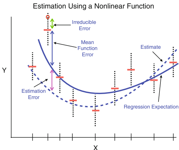
Fig. 1.5 Estimation a nonlinear response surface under the true nonlinear model perspective (The broken line is an estimate from a given dataset, solid line is the expectation of such estimates, the vertical dotted lines represent conditional distributions of Y with the red bars as each distribution's mean.)
