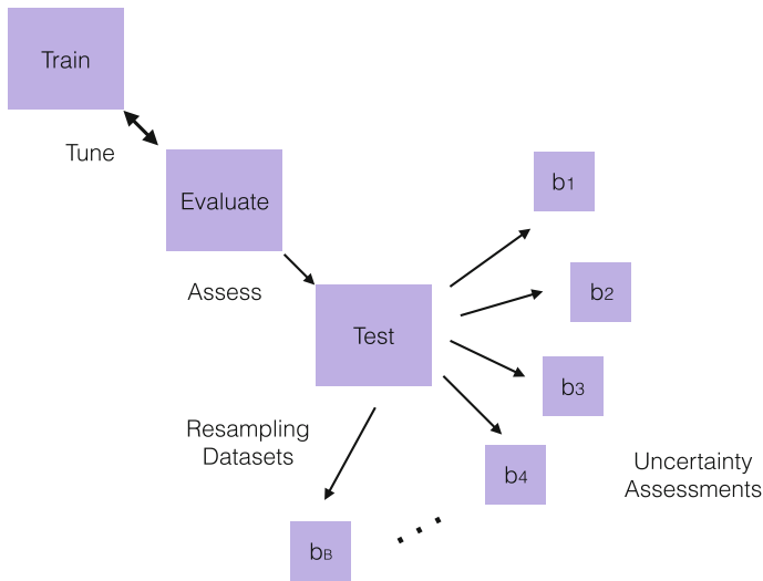
Fig. 2.34 A split sample approach for a level II analysis that includes tuning with an evaluation sample, assessment with a test sample, and uncertainty addressed with bootstrap resampling
