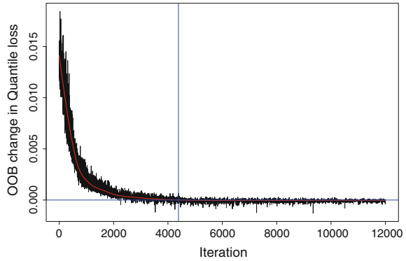
Fig. 6.9 Changes in the quantile loss function with OOB Titanic data and with iteration 4387 as the stopping point ( N = 1045 )
