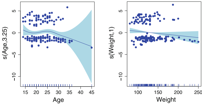
Fig. 2.31 A GAM analysis of new born low birthweight as a function of background characteristics of mothers (The mother's age and weight are on the horizontal axes, the centered fitted logits are on the vertical axes, and shaded are represent error bars. N = 189 )
