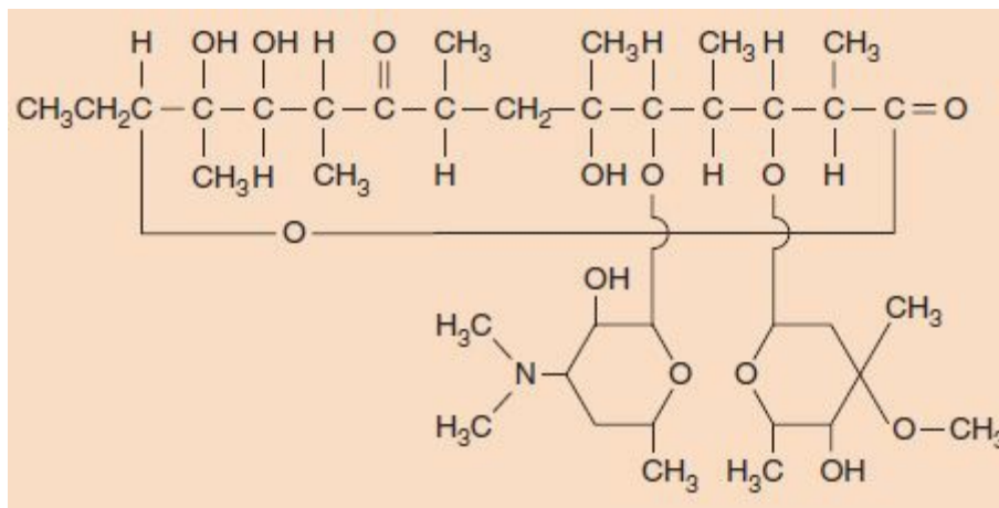
FIGURE 10–8 Erythromycin.
