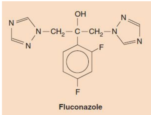
FIGURE 10–12 Fluconazole.
