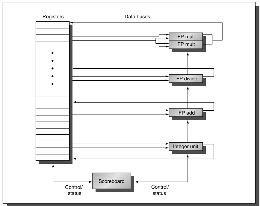
FIGURE A.51 The basic structure of a MIPS processor with a scoreboard. The scoreboard's function is to control instruction execution (vertical control lines). All data flows between the register file and the functional units over the buses (the horizontal lines, called trunks in the CDC 6600). There are two FP multipliers, an FP divider, an FP adder, and an integer unit. One set of buses (two inputs and one output) serves a group of functional units. The details of the scoreboard are shown in Figures A.52–A.55.
