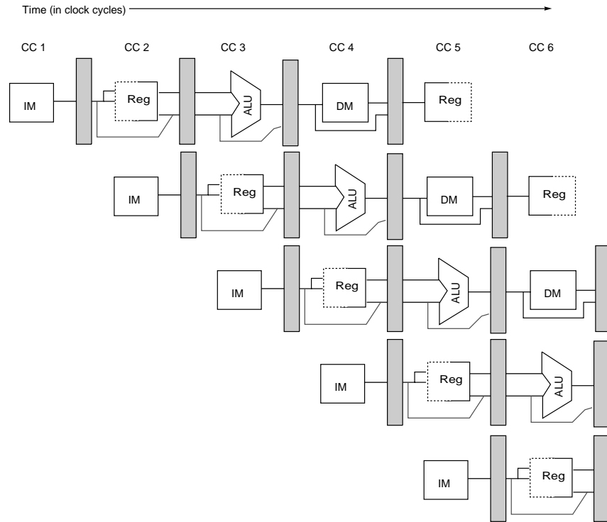
FIGURE A.3 A pipeline showing the pipeline registers between successive pipeline stages. Notice that the registers prevent interference between to different instructions in adjacent stages in the pipeline. The registers also play the critical role of carrying data for a given instruction from one stage to the other. The edge-triggered property of registers—i.e., that they values change instantaneously on a clock edge—is critical. Otherwise, the data from one instruction could interfere with the execution of another!
