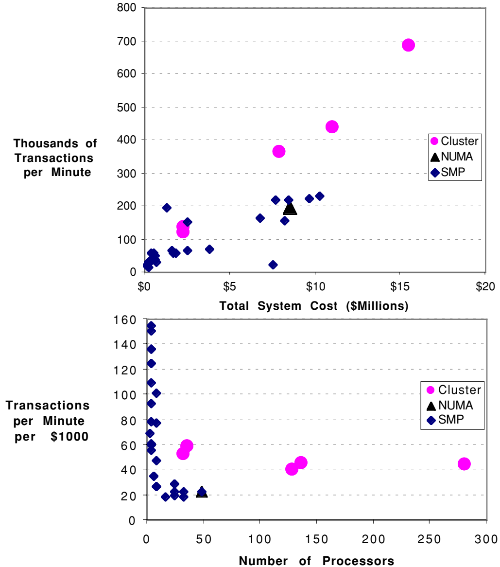
FIGURE 8.31 Performance, Cost, and Cost-Performance per Processor for TPC-C. Not only do clusters have the highest tpmC rating, they have better cost performance ($/tpmC) for any SMP with a total cost over $1M. The bottom graph shows that clusters get high performance by scaling. They can sustain 40 to 50 transactions per minute per $1000 of cost from 32 to 280 processors. Figure 8.40 on page 636 describes the leftmost cluster, and Figure 8.41 on page 637 shows the cost model of TPC-C in more detail. These plots are for all computers that have run version 5 of the TPC-C benchmark as of August 2001.
