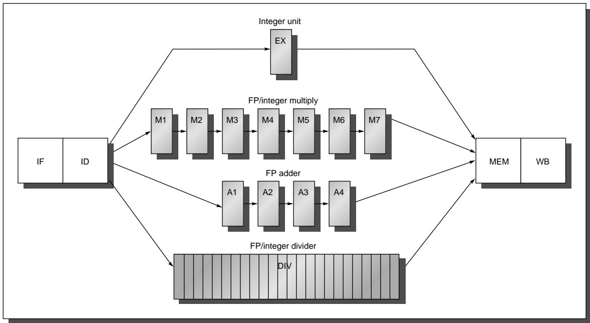
FIGURE A.31 A pipeline that supports multiple outstanding FP operations. The FP multiplier and adder are fully pipelined and have a depth of seven and four stages, respectively. The FP divider is not pipelined, but requires 24 clock cycles to complete. The latency in instructions between the issue of an FP operation and the use of the result of that operation without incurring a RAW stall is determined by the number of cycles spent in the execution stages. For example, the fourth instruction after an FP add can use the result of the FP add. For integer ALU operations, the depth of the execution pipeline is always one and the next instruction can use the results. Both FP loads and integer loads complete during MEM, which means that the memory system must provide either 32 or 64 bits in a single clock.
