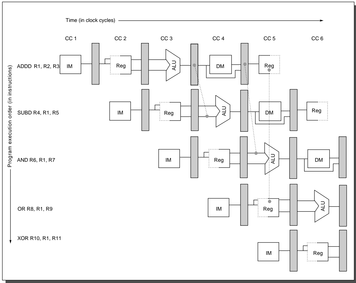
FIGURE A.7 A set of instructions that depend on the ADD result use forwarding paths to avoid the data hazard. The inputs for the SUB and AND instructions forward from the pipeline registers to the first ALU input. The OR receives its result by forwarding through the register file, which is easily accomplished by reading the registers in the second half of the cycle and writing in the first half, as the dashed lines on the registers indicate. Notice that the forwarded result can go to either ALU input; in fact, both ALU inputs could use forwarded inputs from either the same pipeline register or from different pipeline registers. This would occur, for example, if the AND instruction was AND R6, R1, R4 .
