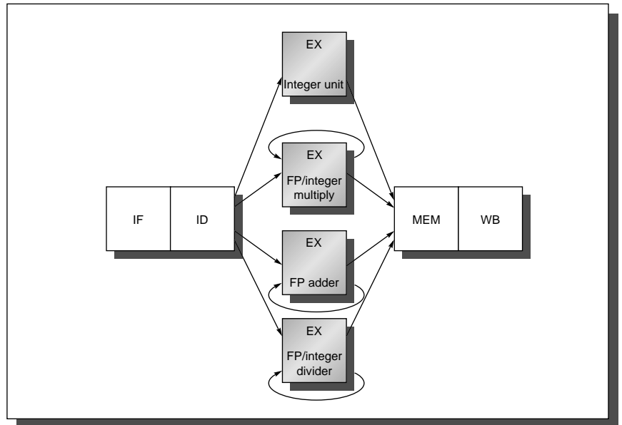
FIGURE A.29 The MIPS pipeline with three additional unpipelined, floating-point, functional units. Because only one instruction issues on every clock cycle, all instructions go through the standard pipeline for integer operations. The floating-point operations simply loop when they reach the EX stage. After they have finished the EX stage, they proceed to MEM and WB to complete execution.
