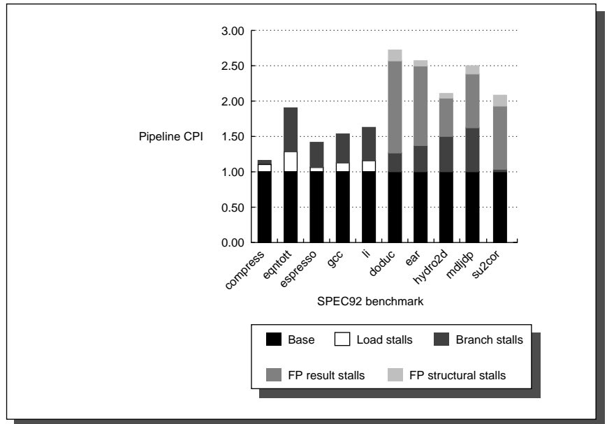
FIGURE A.48 The pipeline CPI for 10 of the SPEC92 benchmarks, assuming a perfect cache. The pipeline CPI varies from 1.2 to 2.8. The leftmost five programs are integer programs, and branch delays are the major CPI contributor for these. The rightmost five programs are FP, and FP result stalls are the major contributor for these. Figure A.49 shows the numbers used to construct this plot.
