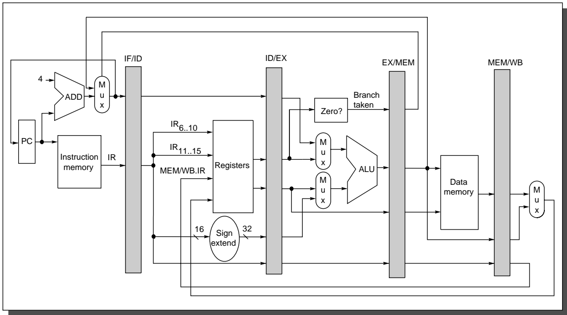
FIGURE A.18 The datapath is pipelined by adding a set of registers, one between each pair of pipe stages. The registers serve to convey values and control information from one stage to the next. We can also think of the PC as a pipeline register, which sits before the IF stage of the pipeline, leading to one pipeline register for each pipe stage. Recall that the PC is an edge-triggered register written at the end of the clock cycle; hence there is no race condition in writing the PC. The selection multiplexer for the PC has been moved so that the PC is written in exactly one stage (IF). If we didn't move it, there would be a conflict when a branch occurred, since two instructions would try to write different values into the PC. Most of the datapaths flow from left to right, which is from earlier in time to later. The paths flowing from right to left (which carry the register write-back information and PC information on a branch) introduce complications into our pipeline.
