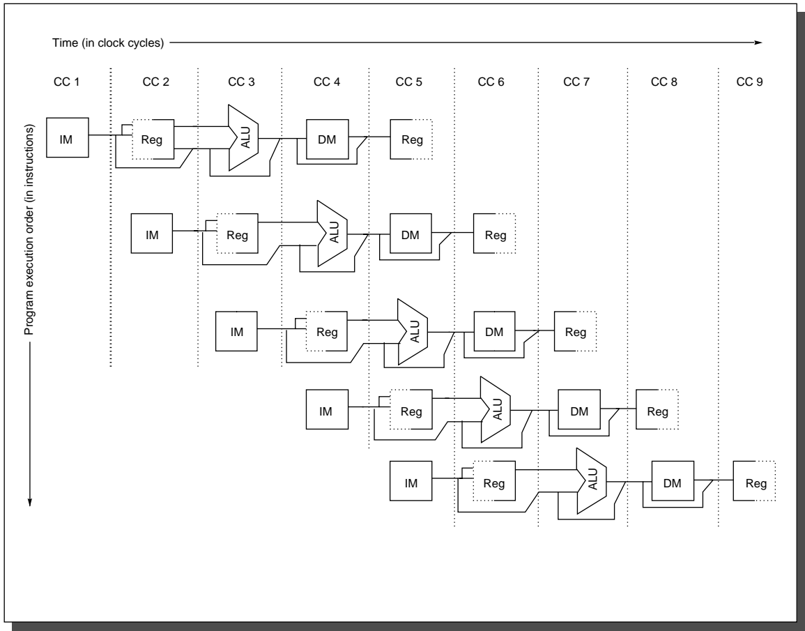
FIGURE A.2 The pipeline can be thought of as a series of datapaths shifted in time. This shows the overlap among the parts of the datapath, with clock cycle 5 (CC 5) showing the steady state situation. Because the register file is used as a source in the ID stage and as a destination in the WB stage, it appears twice. We show that it is read in one stage and written in another by using a solid line, on the right or left, respectively, and a dashed line on the other side. The abbreviation IM is used for instruction memory, DM for data memory, and CC for clock cycle.
