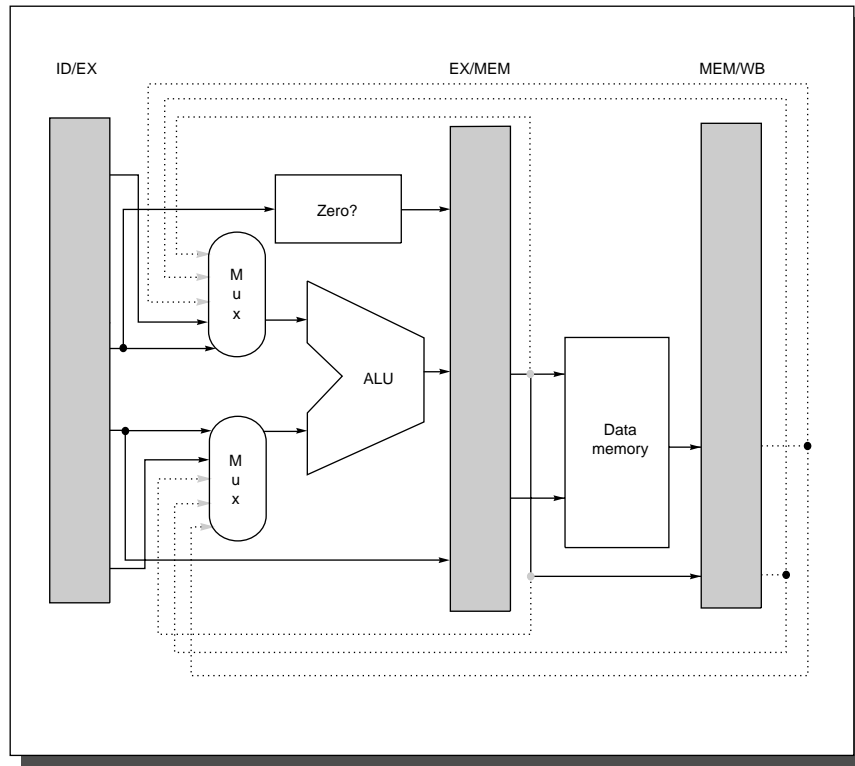
FIGURE A.23 Forwarding of results to the ALU requires the addition of three extra inputs on each ALU multiplexer and the addition of three paths to the new inputs. The paths correspond to a bypass of (1) the ALU output at the end of the EX, (2) the ALU output at the end of the MEM stage, and (3) the memory output at the end of the MEM stage.
