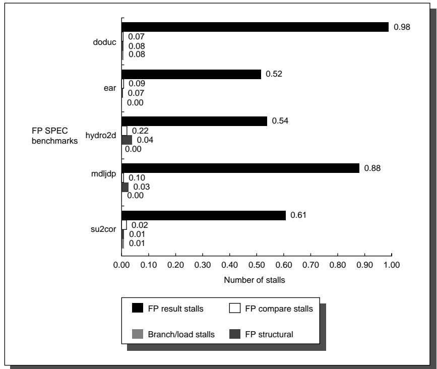
FIGURE A.36 The stalls occurring for the MIPS FP pipeline for five for the SPEC89 FP benchmarks. The total number of stalls per instruction ranges from 0.65 for su2cor to 1.21 for doduc, with an average of 0.87. FP result stalls dominate in all cases, with an average of 0.71 stalls per instruction or 82% of the stalled cycles. Compares generate an average of 0.1 stalls per instruction and are the second largest source. The divide structural hazard is only significant for doduc.
