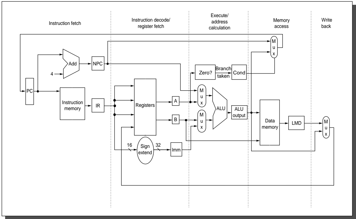
FIGURE A.17 The implementation of the MIPS datapath allows every instruction to be executed in four or five clock cycles. Although the PC is shown in the portion of the datapath that is used in instruction fetch and the registers are shown in the portion of the datapath that is used in instruction decode/register fetch, both of these functional units are read as well as written by an instruction. Although we show these functional units in the cycle corresponding to where they are read, the PC is written during the memory access clock cycle and the registers are written during the write back clock cycle. In both cases, the writes in later pipe stages are indicated by the multiplexer output (in memory access or write back) that carries a value back to the PC or registers. These backward-flowing signals introduce much of the complexity of pipelining, since they indicate the possibility of hazards.
