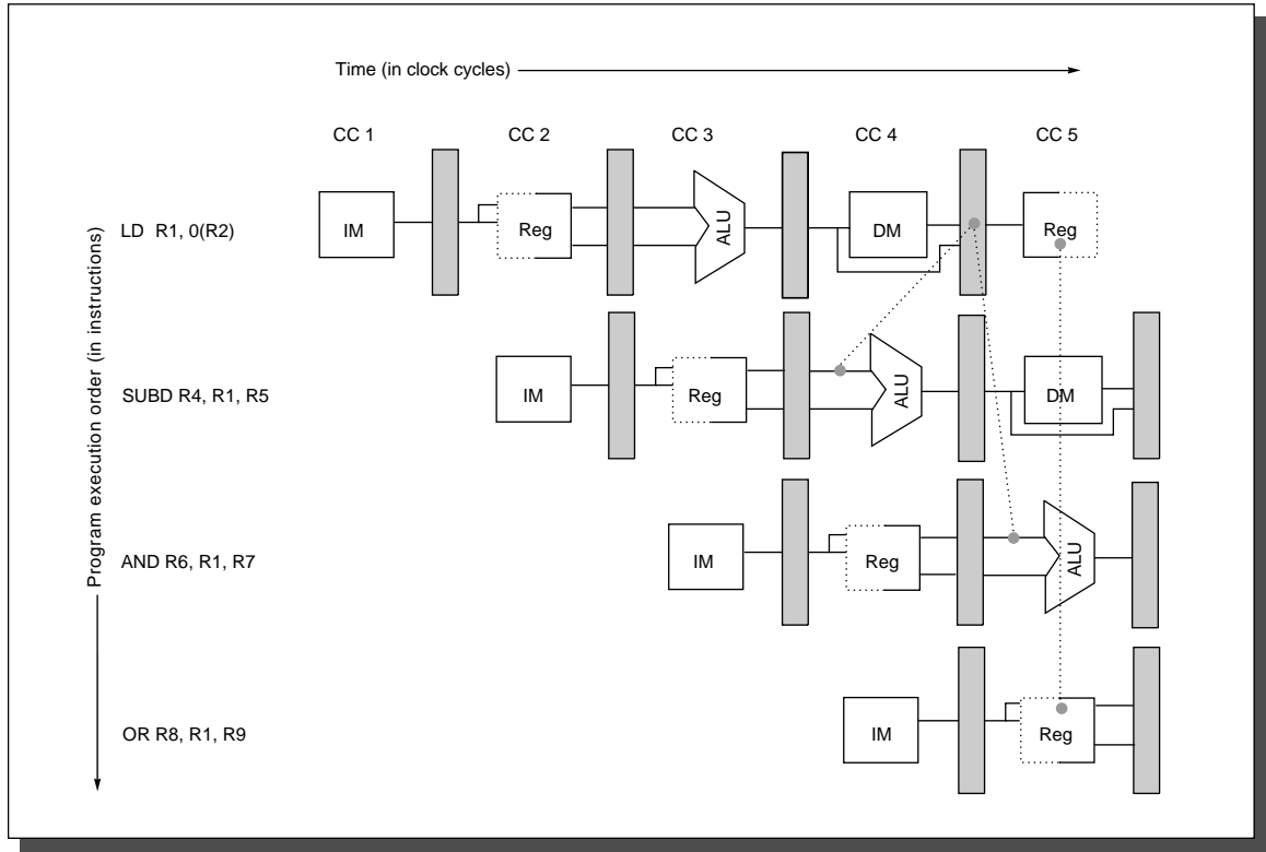
FIGURE A.9 The load instruction can bypass its results to the AND and OR instructions, but not to the SUBD, since that would mean forwarding the result in “negative time.”
