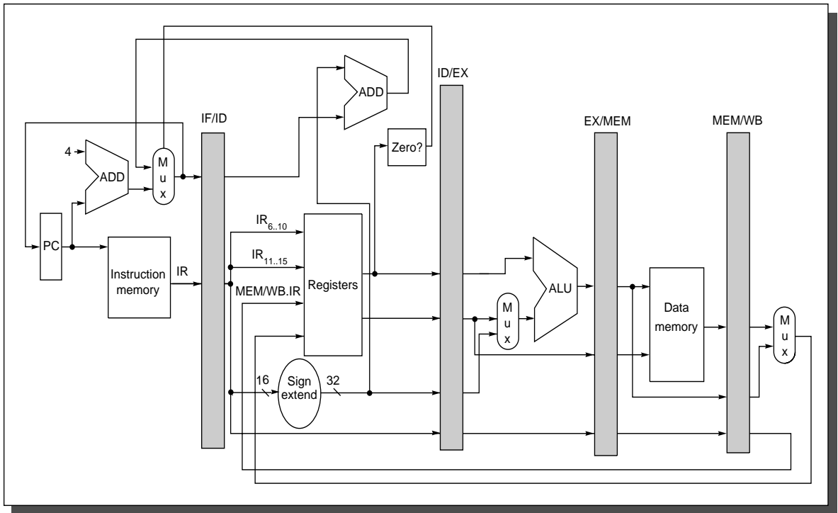
FIGURE A.24 The stall from branch hazards can be reduced by moving the zero test and branch target calculation into the ID phase of the pipeline. Notice that we have made two important changes, each of which removes one cycle from the three cycle stall for branches. The first change is to move both the branch address target calculation and the branch condition decision to the ID cycle. The second change is to write the PC of the instruction in the IF phase, using either the branch target address computed during ID or the incremented PC computed during IF. In comparison, C.18 obtained the branch target address from the EX/MEM register and wrote the result during the MEM clock cycle. As mentioned in C.18, the PC can be thought of as a pipeline register (e.g., as part of ID/IF), which is written with the address of the next instruction at the end of each IF cycle.
