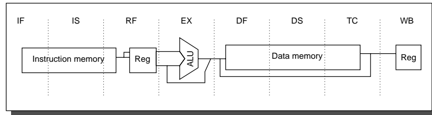
FIGURE A.37 The eight-stage pipeline structure of the R4000 uses pipelined instruction and data caches. The pipe stages are labeled and their detailed function is described in the text. The vertical dashed lines represent the stage boundaries as well as the location of pipeline latches. The instruction is actually available at the end of IS, but the tag check is done in RF, while the registers are fetched. Thus, we show the instruction memory as operating through RF. The TC stage is needed for data memory access, since we cannot write the data into the register until we know whether the cache access was a hit or not.
