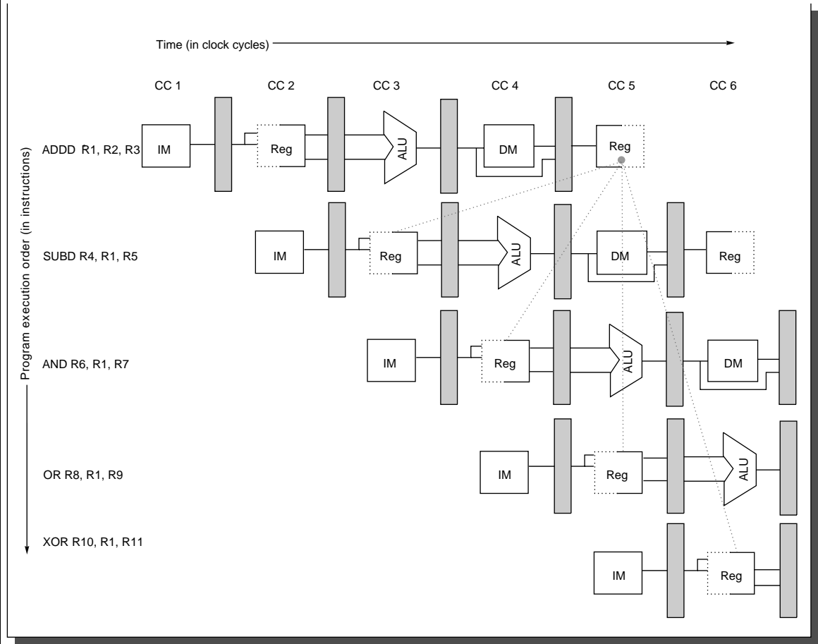
FIGURE A.6 The use of the result of the ADD instruction in the next three instructions causes a hazard, since the register is not written until after those instructions read it.
