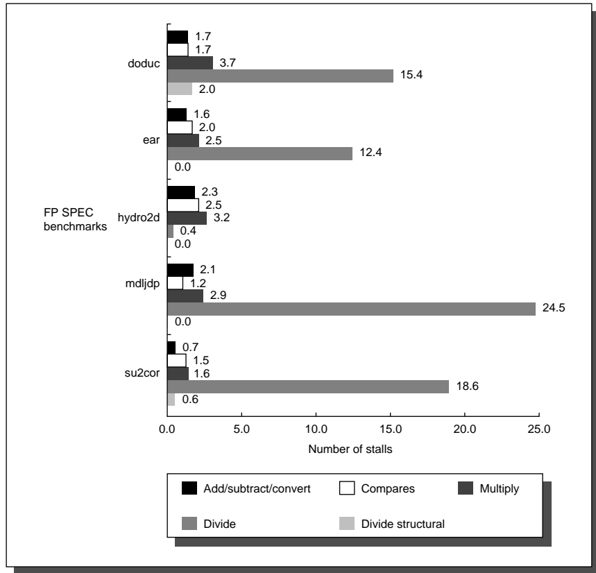
FIGURE A.35 Stalls per FP operation for each major type of FP operation for the SPEC89 FP benchmarks. Except for the divide structural hazards, these data do not depend on the frequency of an operation, only on its latency and the number of cycles before the result is used. The number of stalls from RAW hazards roughly tracks the latency of the FP unit. For example, the average number of stalls per FP add, subtract, or convert is 1.7 cycles, or 56% of the latency (3 cycles). Likewise, the average number of stalls for multiplies and divides are 2.8 and 14.2, respectively, or 46% and 59% of the corresponding latency. Structural hazards for divides are rare, since the divide frequency is low.
