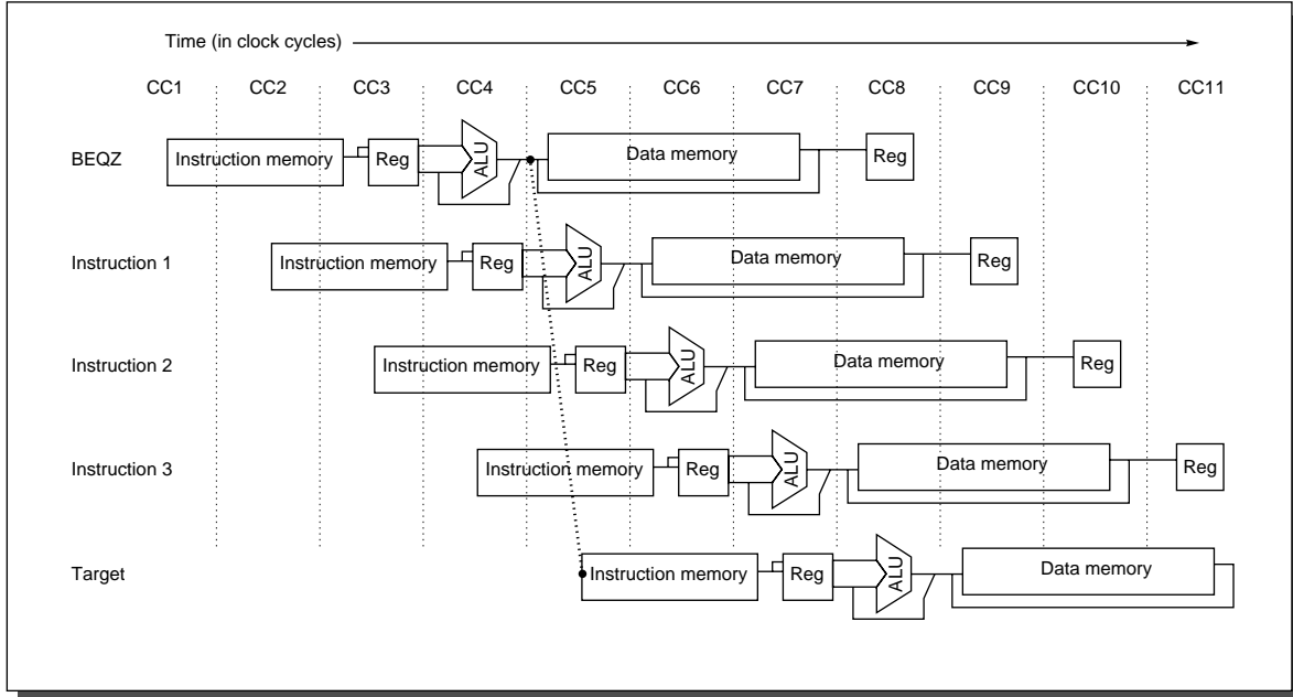
FIGURE A.40 The basic branch delay is three cycles, since the condition evaluation is performed during EX.
