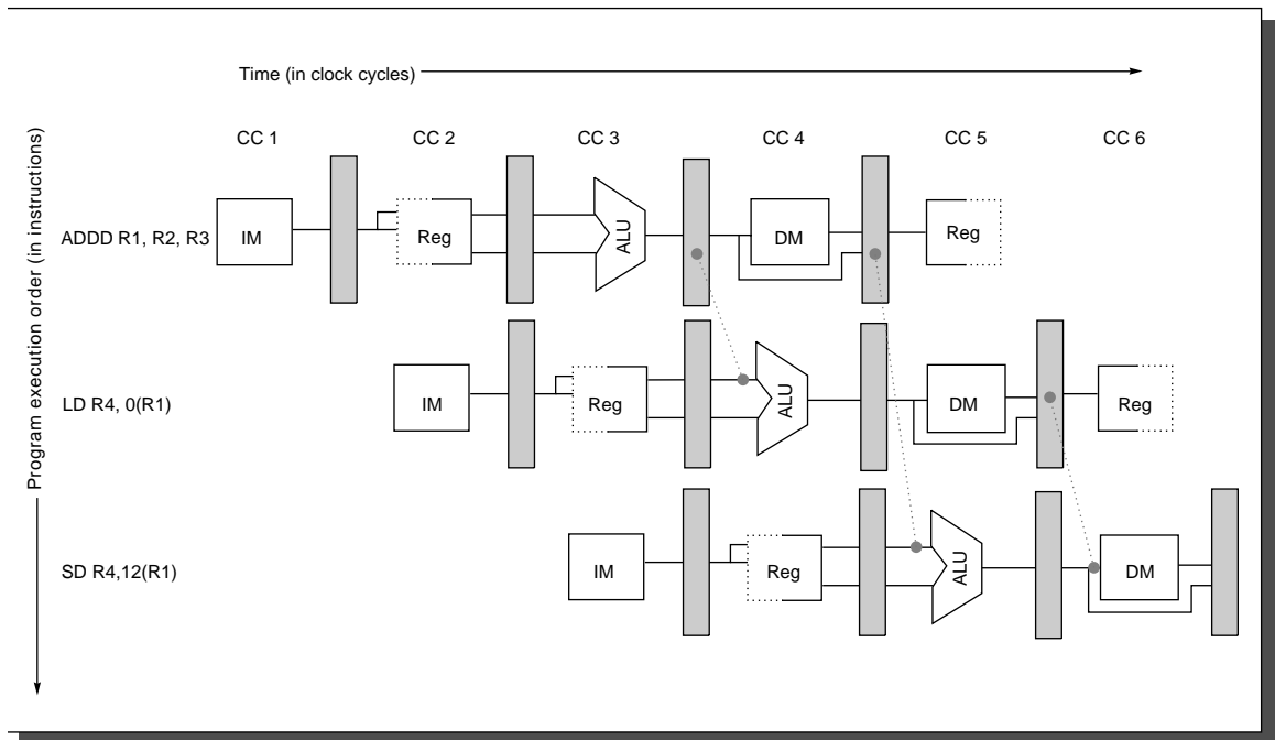
FIGURE A.8 Stores require an operand during MEM, and forwarding of that operand is shown here. The result of the load is forwarded from the memory output to the memory input to be stored. In addition, the ALU output is forwarded to the ALU input for the address calculation of both the load and the store (this is no different than forwarding to another ALU operation). If the store depended on an immediately preceding ALU operation (not shown above), the result would need to be forwarded to prevent a stall.
