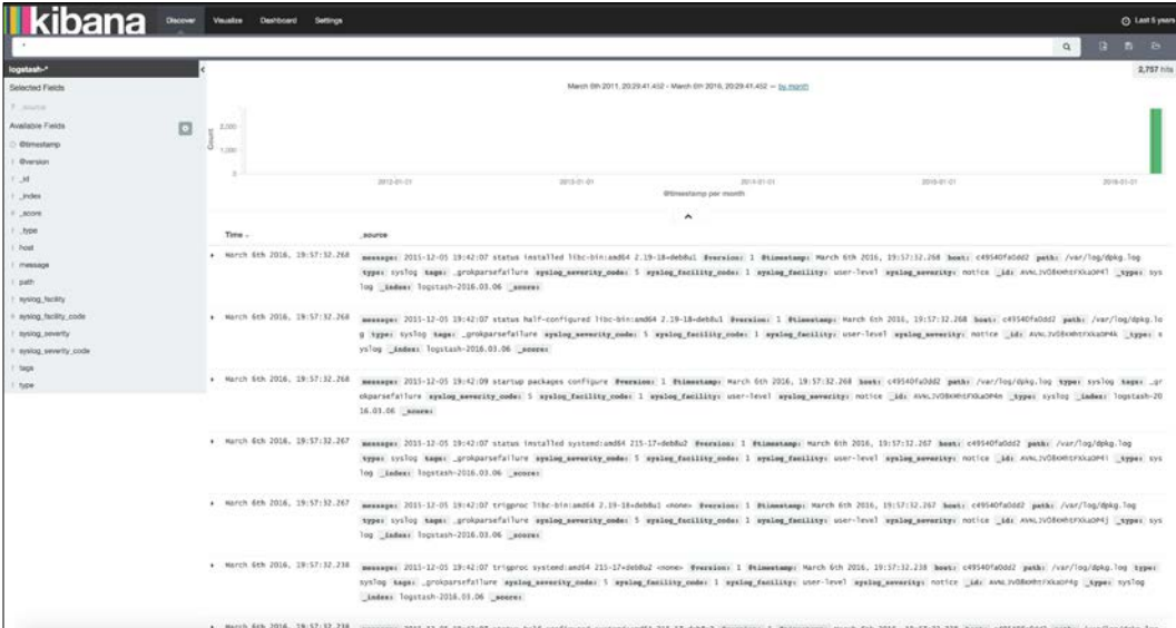
Logstash's logs
