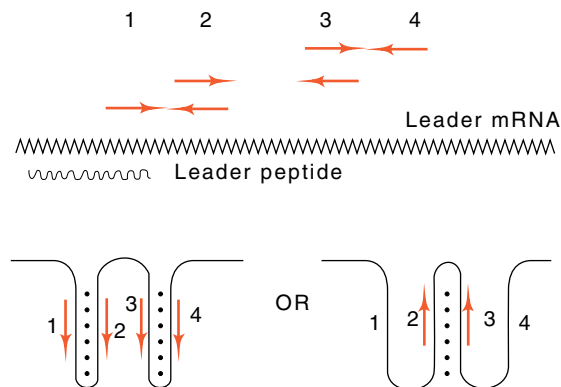
Figure 13.11 The two possible structures that the second half of the trp leader region is capable of assuming. Above is indicated the leader region with the complementary regions. Opposed arrows at the same height above the leader are homologous and can base pair. The wavy line below the leader mRNA is the region encoding the leader peptide.
