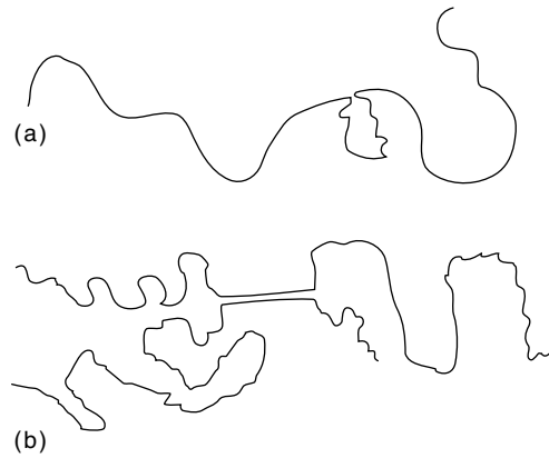
Figure 19.2 (a) DNA heteroduplex between lambda and lambda containing IS2. The single-stranded bubble is the DNA of IS2. (b) DNA heteroduplex formed between two r strands of lambda, each containing IS2 but in opposite orientations.
