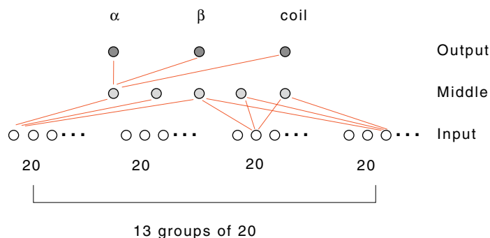
Figure 6.17 A three layer neural network of 20 \times 13 inputs, a middle layer, and an output layer. Each of the input "neurons" is connected to each of the middle layer neurons and each of the middle layer neurons is connected to the three output neurons. The strengths of the interactions are not all equal.
