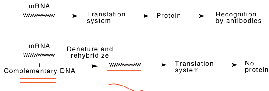
Figure 9.15 Hybridization arrest of translation as an assay for DNA of a gene whose mRNA can be translated into protein.
