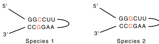
Figure 21.3 How base differences in two regions of RNA strengthen proposals for base pairing between the regions involved.
