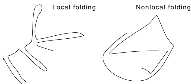
Figure 21.1 Examples of local and nonlocal folding.
