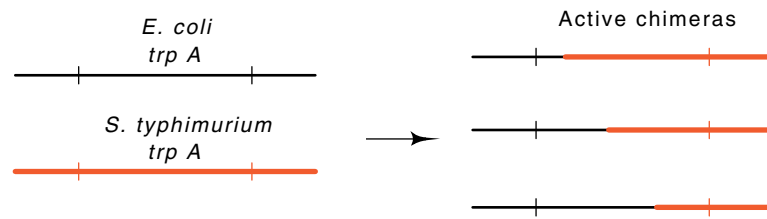
Figure 6.11 Substitution of portions of the E. coli tryptophan synthetase \alpha subunit with corresponding regions from the Salmonella typhimurium synthetase subunit.
