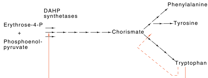
Figure 13.1 Outline of the aromatic amino acid biosynthetic pathway in Escherichia coli . Each arrow represents an enzymatic step. Tryptophan feedback inhibits one of the DAHP synthetases, AroH, as well as the first enzyme of the pathway committed to tryptophan synthesis.
