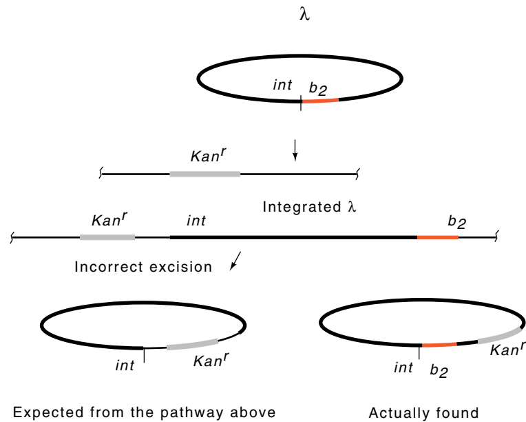
Figure 19.6 The structure of \lambda - kan r expected if the transducing particles were generated by the same mechanism by which \lambda - gal and \lambda - bio transducing phages are produced, and the structure of \lambda - kan actually found.
