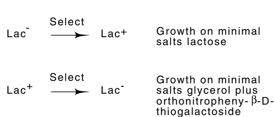
Figure 8.17 Positive selections for \text{Lac}^+ and \text{Lac}^- cells.
