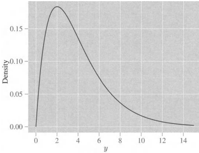
Figure 4.6 A distribution with positive skewness.
