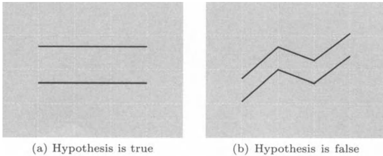
Figure 5.7 Hypothesis H_{03} of equal tests (variables) assuming parallelism.
