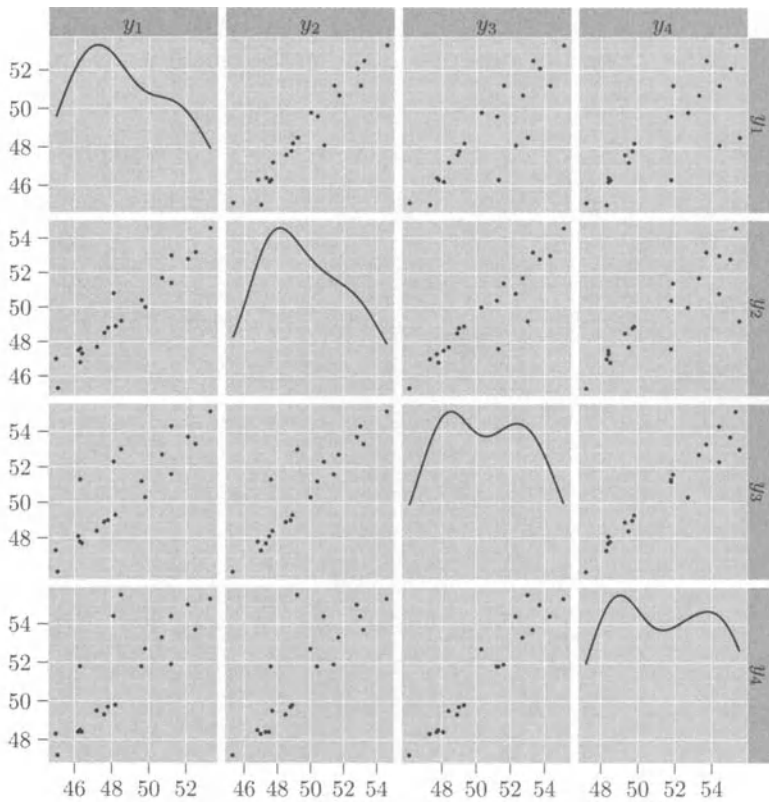
Figure 4.11 Scatterplots for the ramus bone data in Table 3.7, with density curves for each variable.
