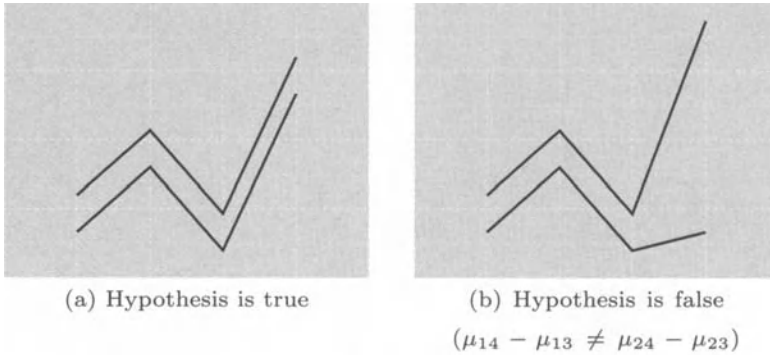
Figure 5.4 Comparison of two profiles under the hypothesis of parallelism.
