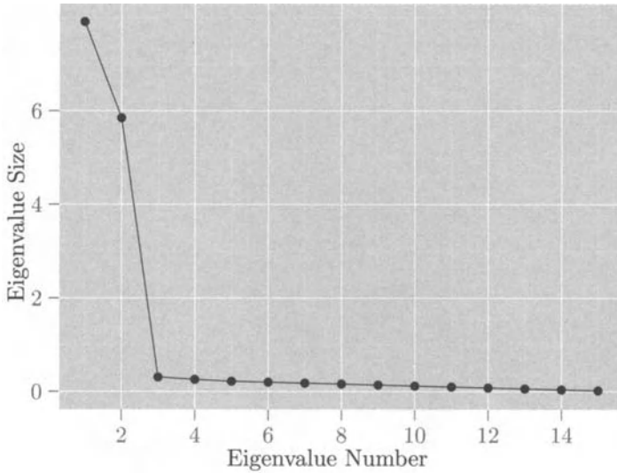
Figure 13.5 Scree graph for voice data.
