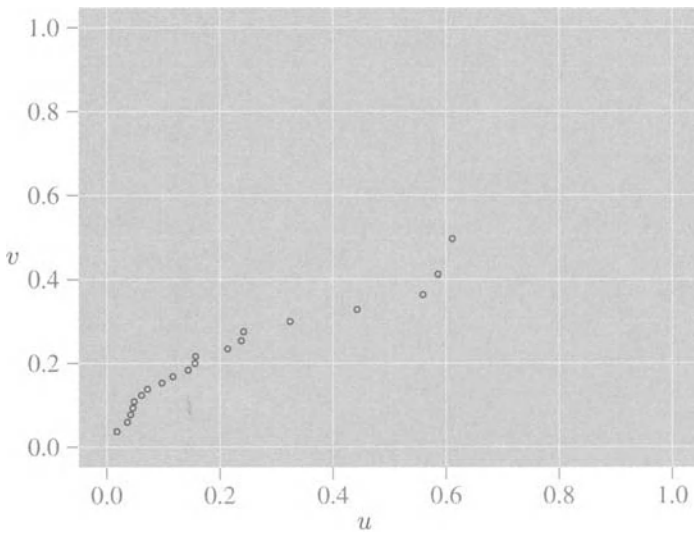
Figure 4.10 Q-Q plot of u_i and v_i for the ramus bone data of Table 3.7.
