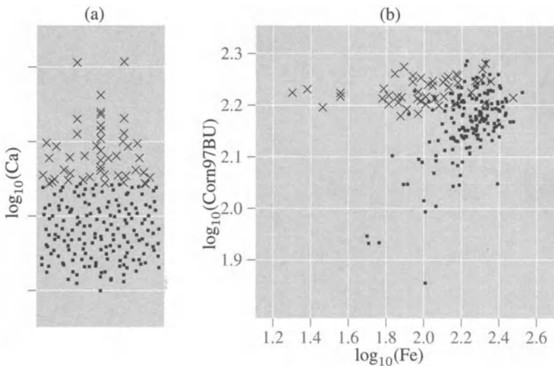
Figure 3.11 Linked and brushed plots of the Baker field data in Table 3.3. The dotplot of Ca in panel (a) is linked to the scatterplot of \log(\text{Fe}) versus \log(\text{yield}) in panel (b), with the points associated with high Ca brushed to appear as X's.
