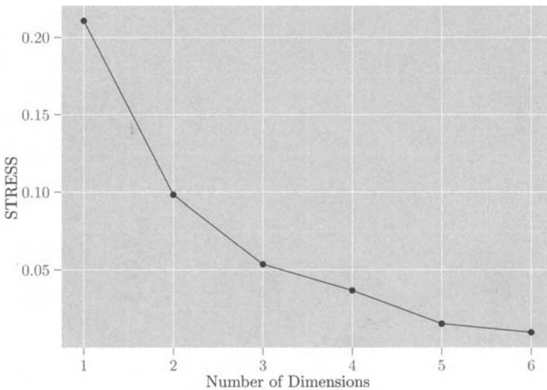
Figure 16.4 Plot of STRESS for each value of k for the voting data in Table 16.2.
