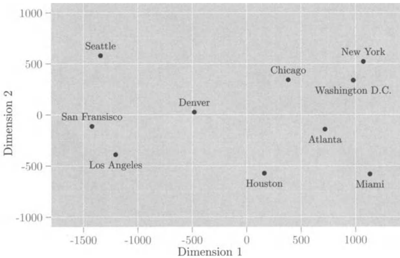
Figure 16.2 Plot of the points found in Example 16.1.2(b).
