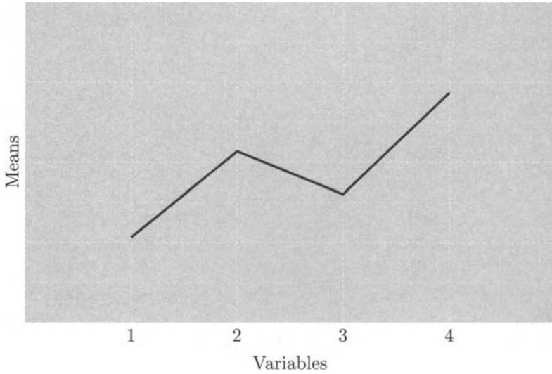
Figure 5.3 Profile of a mean vector.
