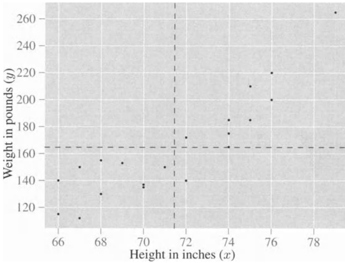
Figure 3.5 Bivariate scatterplot of the data in Figure 3.1.
