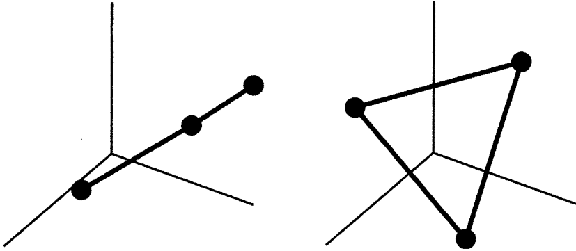
Figure 6.2 Two possible configurations for three mean vectors in 3-space.
