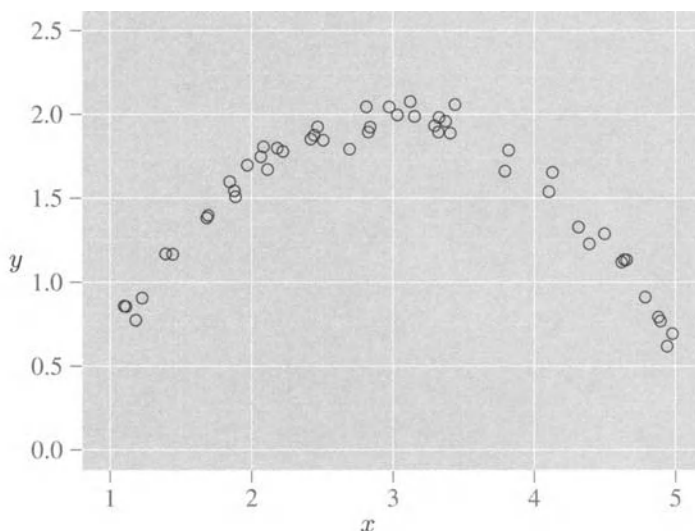
Figure 3.2 A sample from a population where x and y have zero covariance and yet are dependent.
