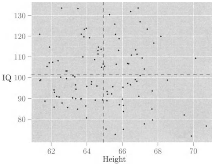
Figure 3.6 A sample of data from a population where x and y are uncorrelated.
