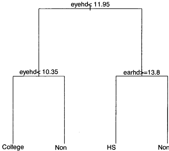
Figure 9.4 Classification tree for classifying subjects into one of three groups using the football data of Table 8.3
