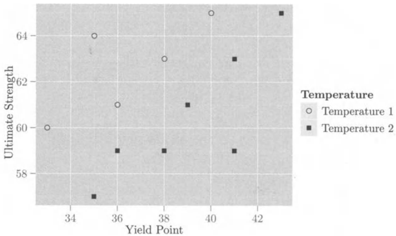
Figure 8.3 Ultimate strength and yield point for steel rolled at two temperatures.
