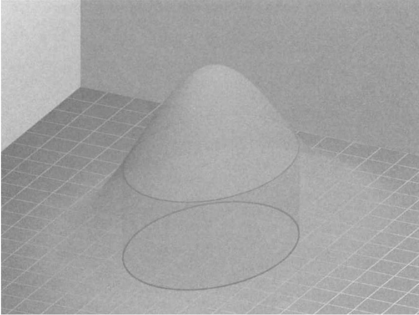
Figure 4.4 Constant density contour for bivariate normal.
