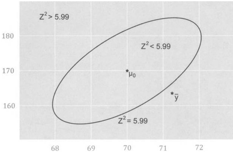
Figure 5.1 Elliptical acceptance region.
