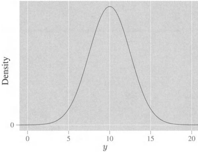
Figure 4.1 The normal density curve.
