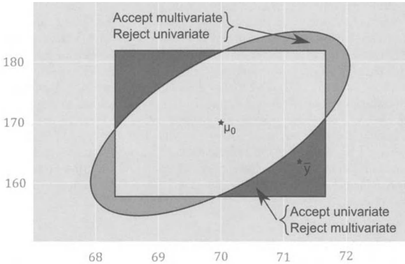
Figure 5.2 Acceptance and rejection regions for univariate and multivariate tests.
