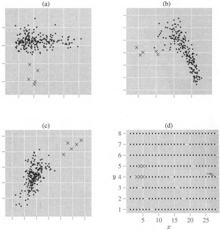
Figure 3.9 Grand tour of the soil richness measurements in Table 3.3. Panels (a), (b), and (c) show three different projections observed during the grand tour, and panel (d) indicates the geographic locations of the five outliers discovered by the grand tour and brushed to become X's instead of dots.
