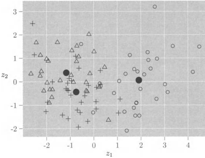
Figure 8.4 Scatterplot of discriminant function values for the football data of Table 8.3.
