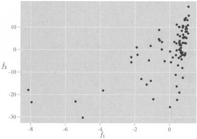
Figure 14.3 Estimated effort score ( \hat{f}_1 ) vs. estimated knowledge mastery score ( \hat{f}_2 ) for 94 students in a business statistics course.
