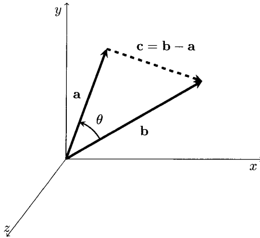
Figure 3.4 Vectors a and b in 3-space.
