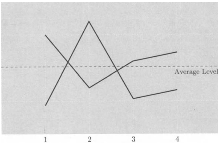
Figure 5.6 Hypothesis H_{02} of equal group effect without parallelism.
