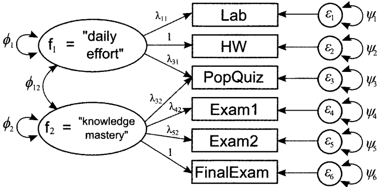
Figure 14.2 Path diagram for the grade data model.
