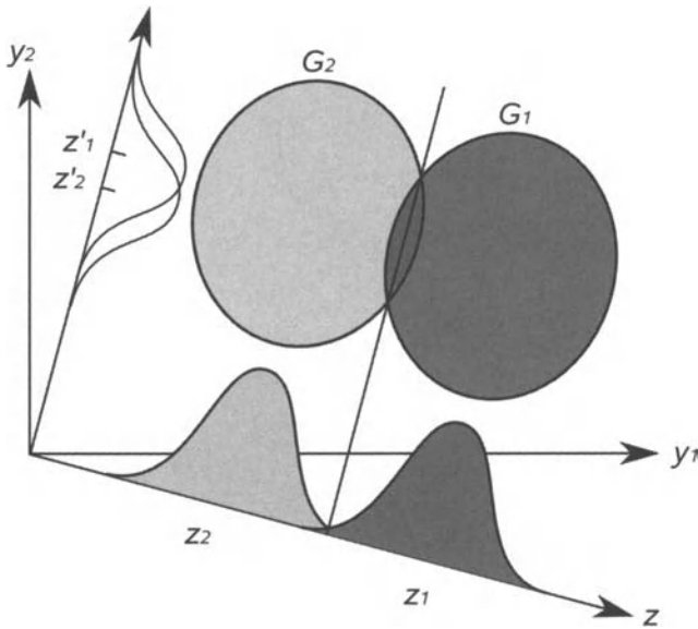
Figure 8.2 Separation achieved by the discriminant function.
