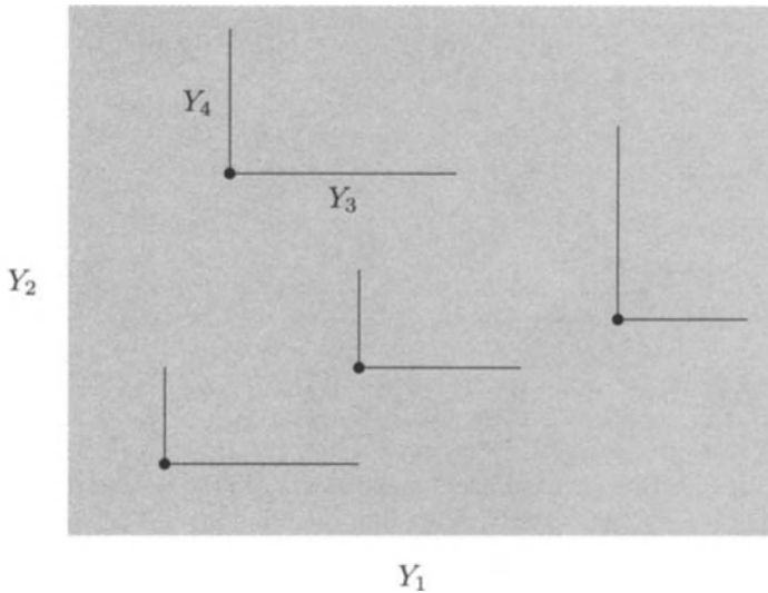
Figure 3.7 Four-dimensional plot.
