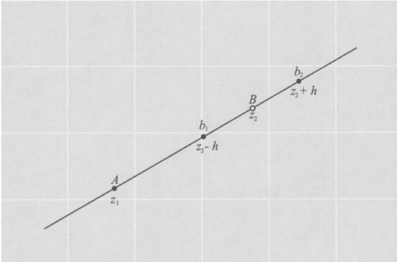
Figure 15.15 Clusters in a single dimension.
