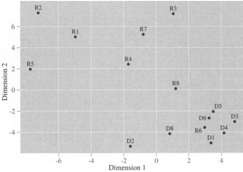
Figure 16.5 Plot of points found using initial points from a multivariate normal distribution.
