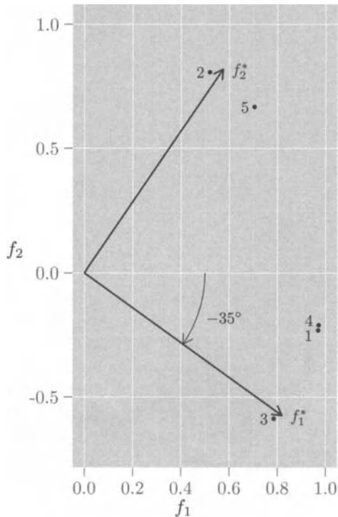
Figure 13.3 Plot of the two loadings for each of the five variables in the perception data of Table 13.1.
