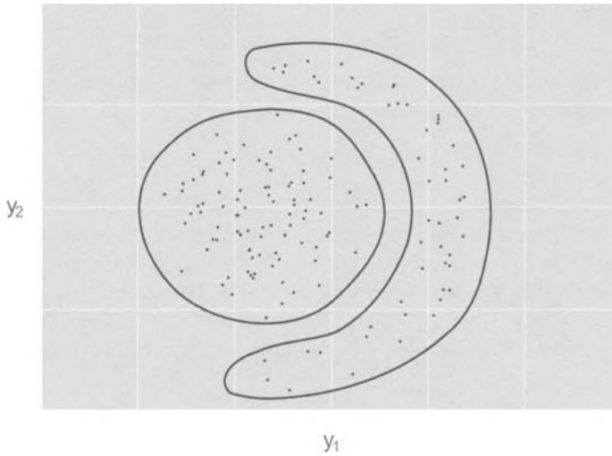
Figure 9.2 Two populations with nonlinear separation.
