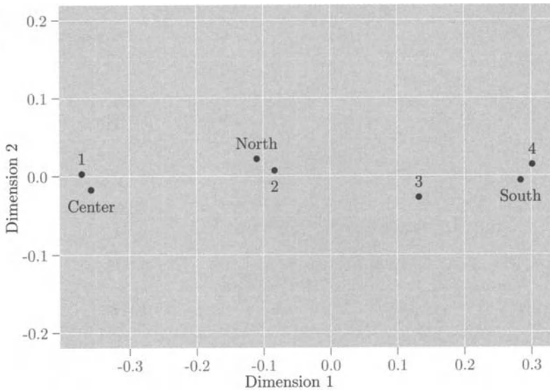
Figure 16.8 Row points (1, 2, 3, 4) and column points (Center, North, South).
