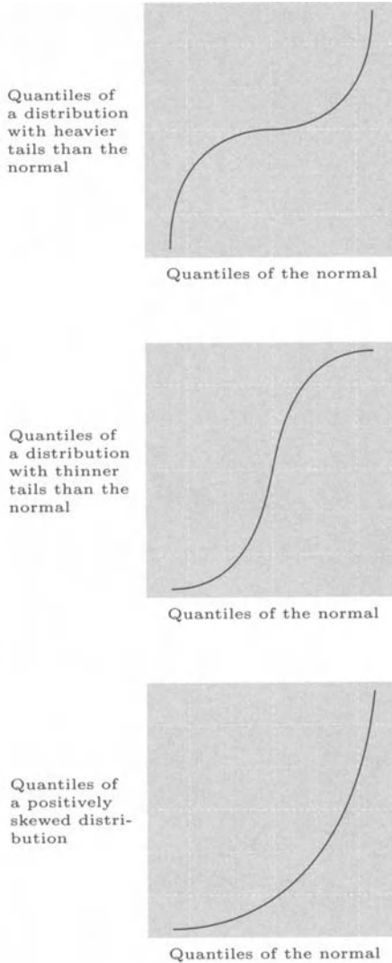
Figure 4.5 Typical Q-Q plots for nonnormal data.
