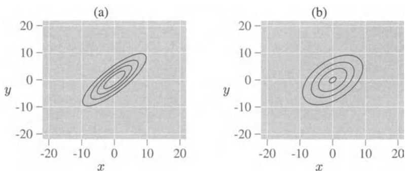
Figure 4.3 Contour plots for the distributions in Figure 4.2.
