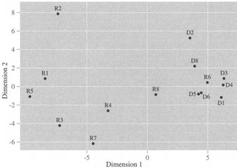
Figure 16.7 Plot of points found using initial points from a metric solution.
