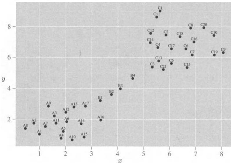
Figure 15.12 Two distinct clusters with intervening individuals.
