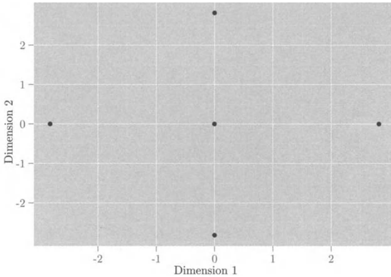
Figure 16.1 Plot of the five points found in Example 16.1.2(a).
