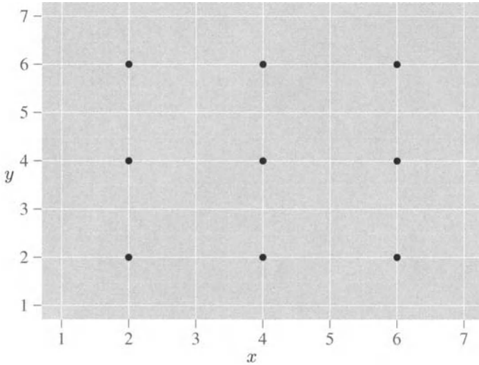
Figure 3.3 A sample of (x, y) values with zero covariance.
