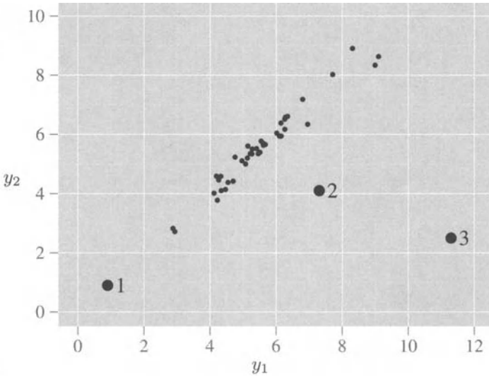
Figure 4.9 Bivariate sample showing three types of outliers.
