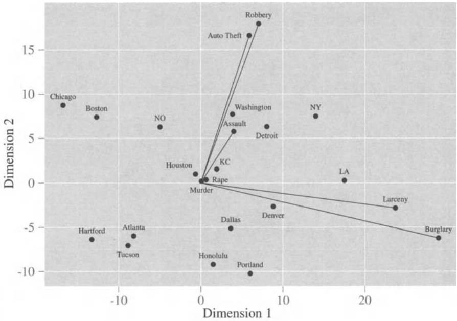
Figure 16.11 Plot of U_2\Lambda_2^{1/2} and V_2\Lambda_2^{1/2} for the City Crime Data in Table 15.1.
