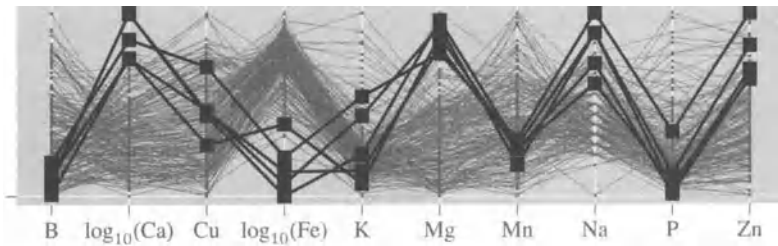
Figure 3.10 Parallel coordinates plot of the soil richness measurements in Table 3.3. Highlighted lines are linked to the points denoted as outliers in Figure 3.9.
