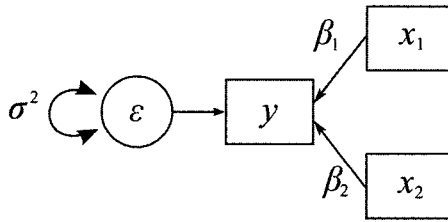
Figure 14.1 Path diagram for multiple regression model y = \beta_1 x_1 + \beta_2 x_2 + \varepsilon , with \text{var}(\varepsilon) = \sigma^2 .
