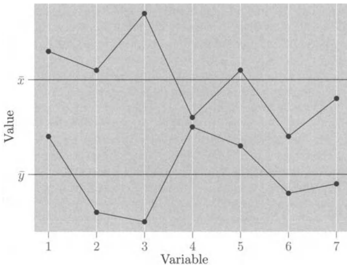
Figure 15.1 Profiles for two observation vectors x and y .
