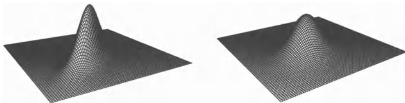
Figure 4.2 Bivariate normal densities.
