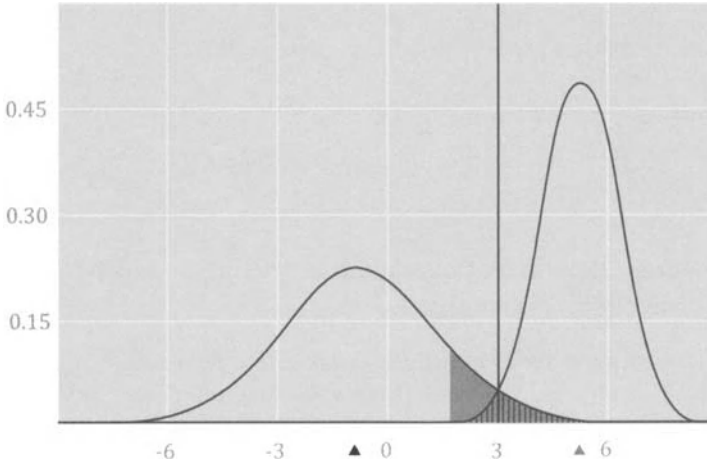
Figure 9.3 Misclassification rates when correctly assuming variances are unequal (hatched area) and when incorrectly assuming variances are equal (gray area).
