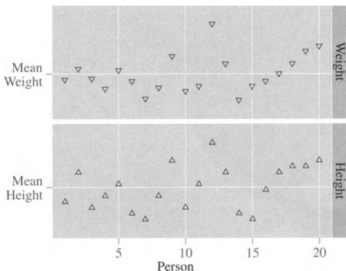
Figure 3.1 Two variables with a tendency to covary.
