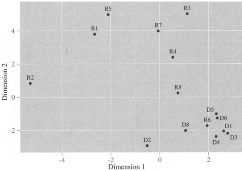
Figure 16.6 Plot of points found using initial points from a uniform distribution.
