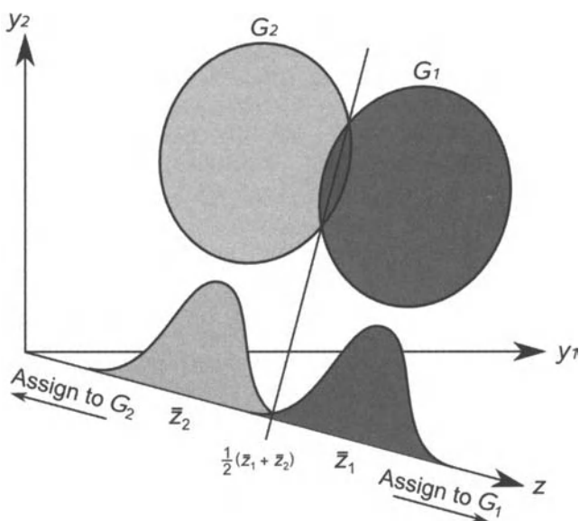
Figure 9.1 Fisher's procedure for classification into two groups.
