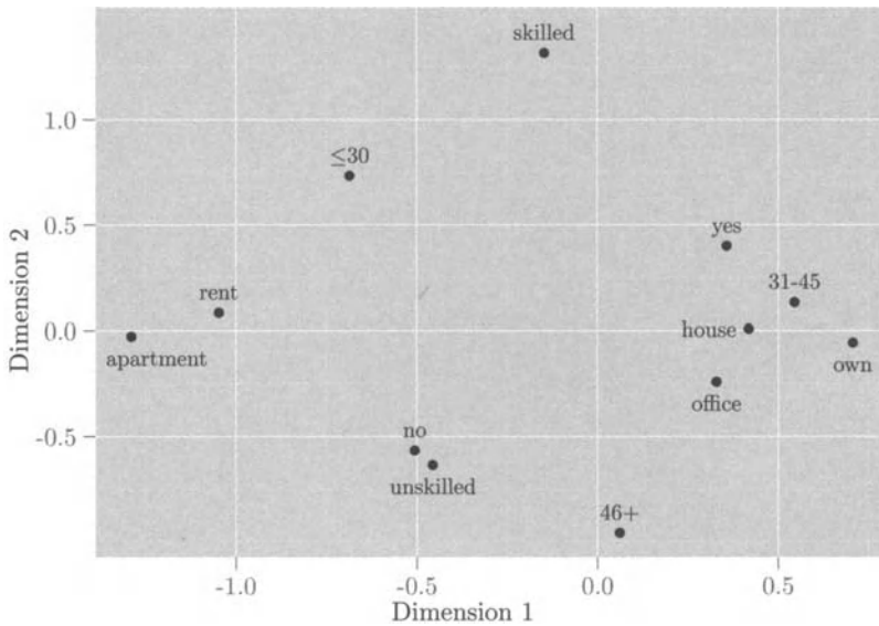
Figure 16.10 Plot of points representing the 12 categories in Table 16.13.
