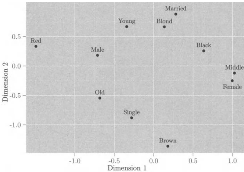
Figure 16.9 Plot of Points Representing the 11 Columns of Table 16.10 or Table 16.11.
