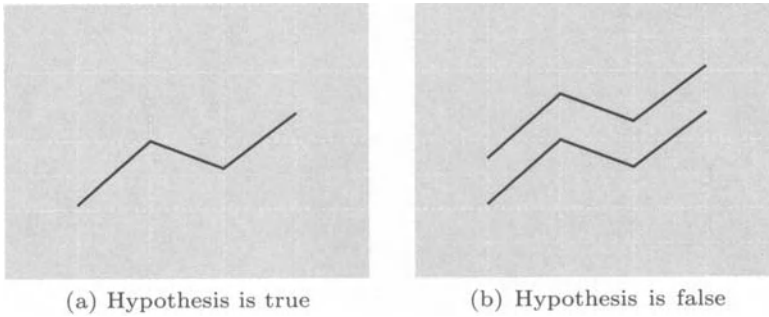
Figure 5.5 Hypothesis H_{02} of equal group effect, assuming parallelism.
