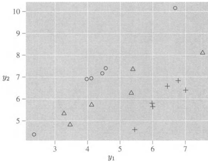
Figure 6.1 Three samples with significant Wilks' \Lambda but nonsignificant F 's.
