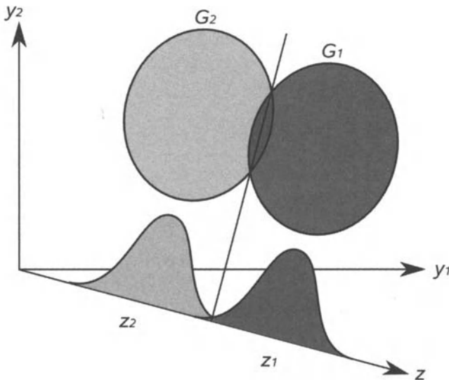
Figure 8.1 Two-group discriminant analysis.
