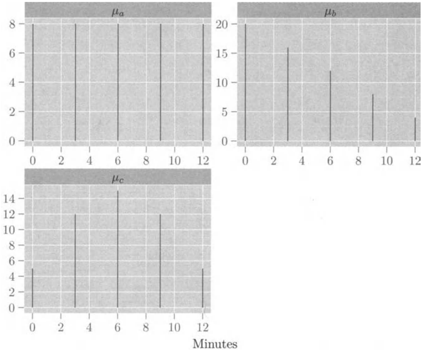
Figure 6.4 Three different patterns for \mu .
