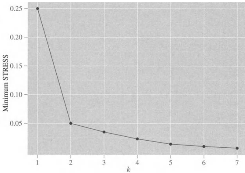
Figure 16.3 Ideal plot of minimum STRESS versus k .
