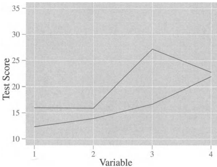
Figure 5.8 Profiles for the psychological data in Table 5.1.
