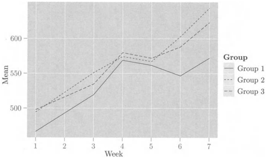
Figure 6.3 Profile of the three groups for the guinea pig data of Table 6.8.
