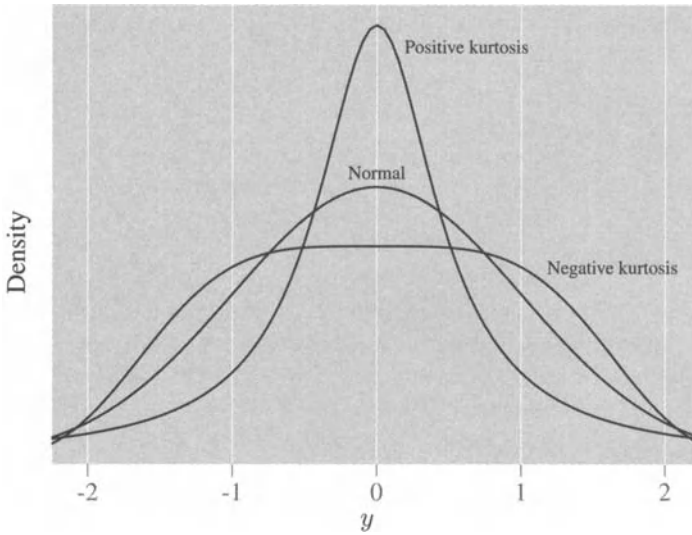
Figure 4.7 Distributions with positive and negative kurtosis compared to the normal.
