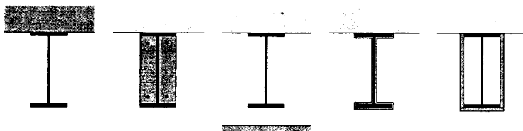
Fig. 30: Passive fire protection measures
