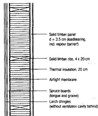
Fig. 5: Horizontal section through wall Beath & Deplazes: private house (Beath-Candinas), Sumvitg (CH), 1998
