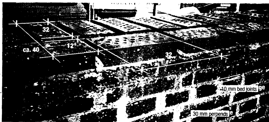
Fig. 85: English cross bond with wide joints
