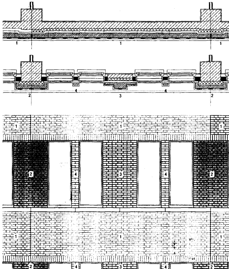
Fig. 83: Details of facade cladding to block: horizontal section through spandrel panel, horizontal section through windows, and elevation on windows and spandrel panel showing individual prefabricated parts and joints: 1 spandrel panel element, 2 column cladding, 3 lesene, 4 mullion Hans Kollhoff: high-rise block, Potsdamer Platz, Berlin (D), 1999
