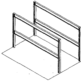
Fig. 39: Frame with continuous columns
