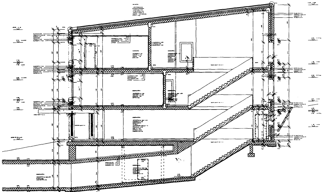
Fig. 144: Section, 1:200 1:50 working drawing (reduced)
