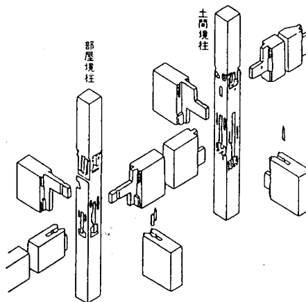
Fig. 64: Traditional Japanese house design Column-beam wood joint
