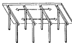
Fig. 59: One-way-spanning continuous slab
