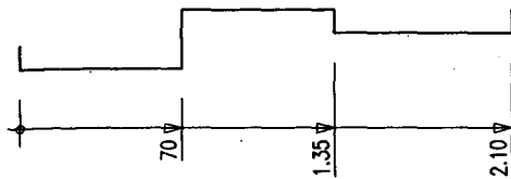
Fig. 6: Chain dimensions
