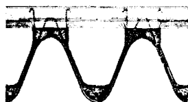
Fig. 8: Detail of floor construction: V-shaped precast ferrocement elements; wall thickness: 3 cm; total depth of floor (incl. floor finish): 50 cm Pier Luigi Nervi: Gaibani office building, Milan (I), 1955/56
