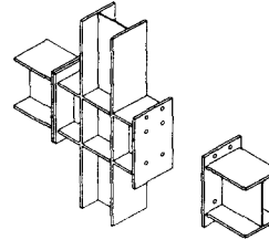
Bolted, with projecting end plates, stiffeners welded to column in line with beam flanges
