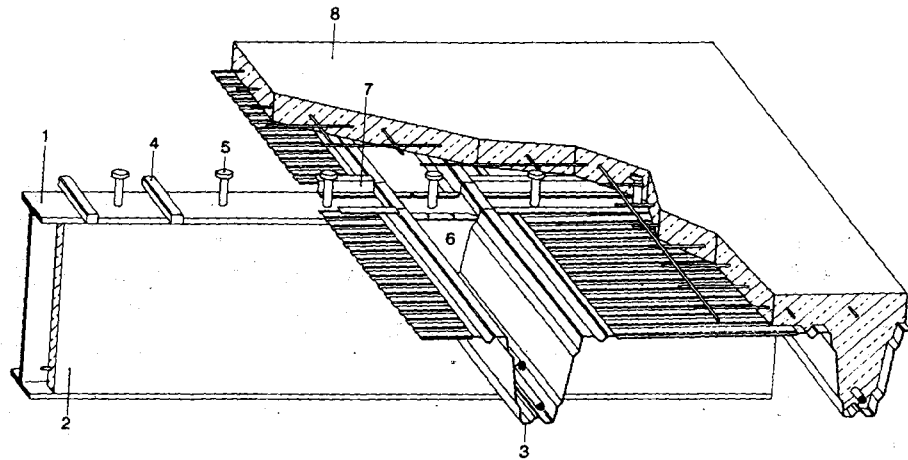
Fig. 41: Composite floor slab with deep trapezoidal sections
