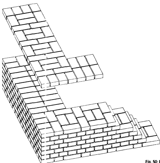
Fig. 50: Dutch bond
