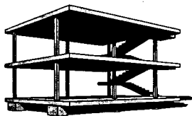
Fig. 18: Sketch of principle of column-and-slab system Le Corbusier: "Dom-ino" construction system, 1914
