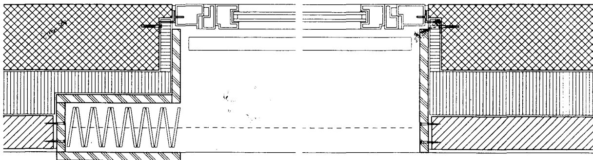
Fig. 114: Horizontal section, 1:10
