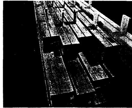
Fig. 58: Beams with heart cuts and wedges driven in
