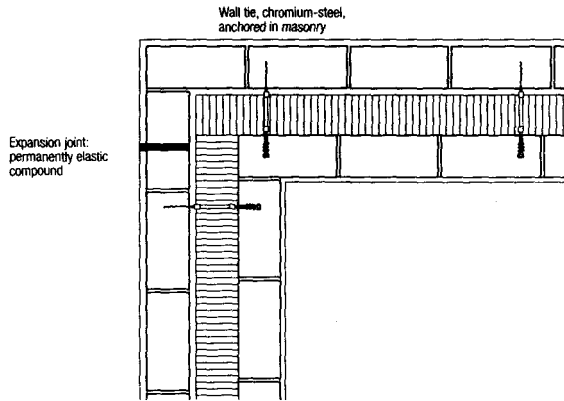
Plan, course 1
