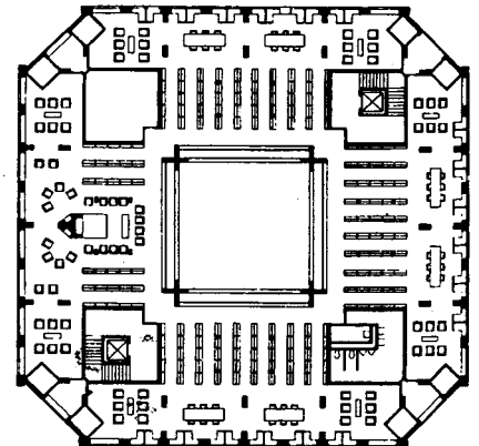
Fig. 94: Section, plan of 3rd floor Louis I. Kahn: Phillips Exeter Library, Exeter (New Hampshire, USA), 1968-72
