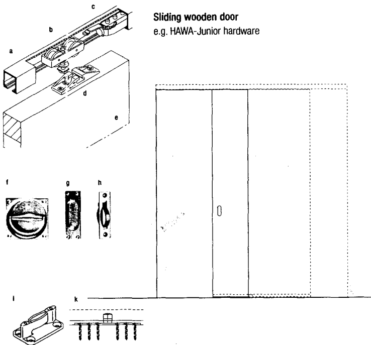
Fig. 72: Schematic drawing of sliding door
