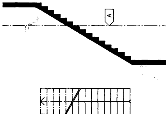
Fig. 15: Single-storey stairs Plan and section
