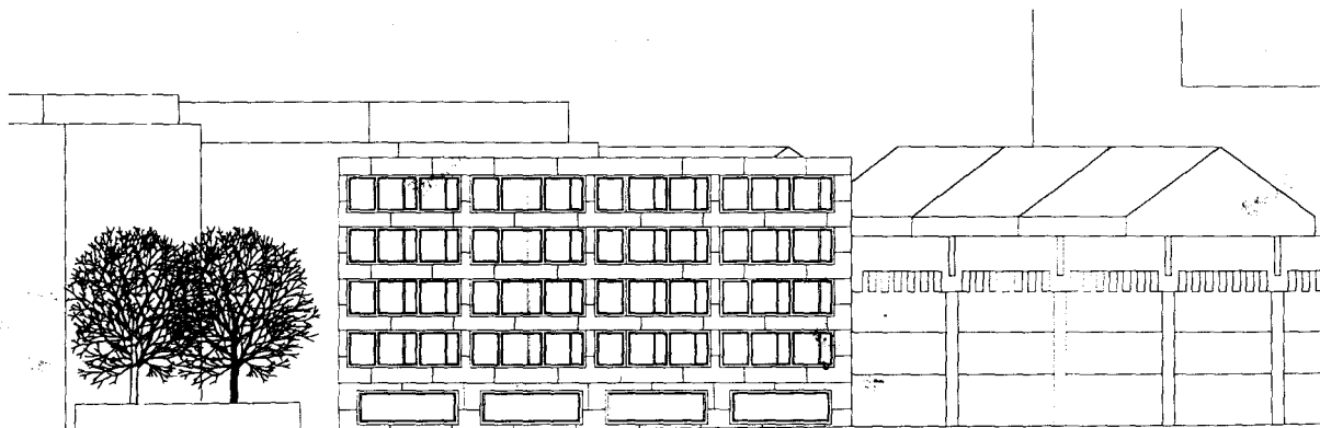
Fig. 165: East elevation showing layout of formwork panels, 1:500
