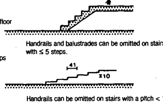
⑥ Stairs without handrail(s)
