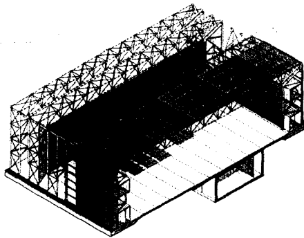
Fig. 69: Identical structure and building envelope for roof and walls, axonometric view of loadbearing construction with and without cladding Norman Foster: Sainsbury Centre for Visual Arts, Norwich (GB), 1978
