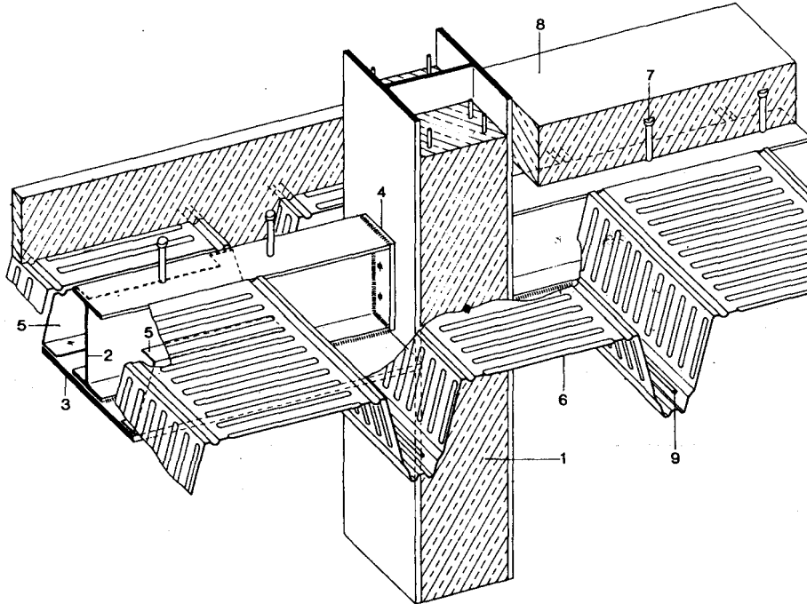
Fig. 47: Composite floor slab with deep trapezoidal sections
