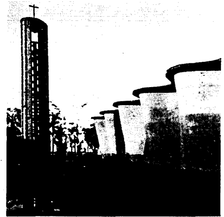
Fig. 24: Curving brickwork shells Eladio Dieste: Church in Atlántida (Uruguay), 1960
