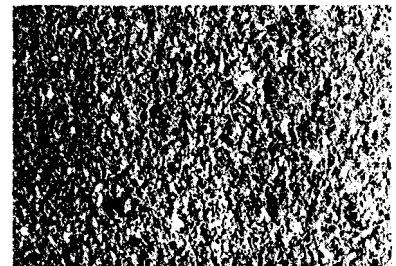
Fig. 29: Point-tooled surface Medium-coarse quality
