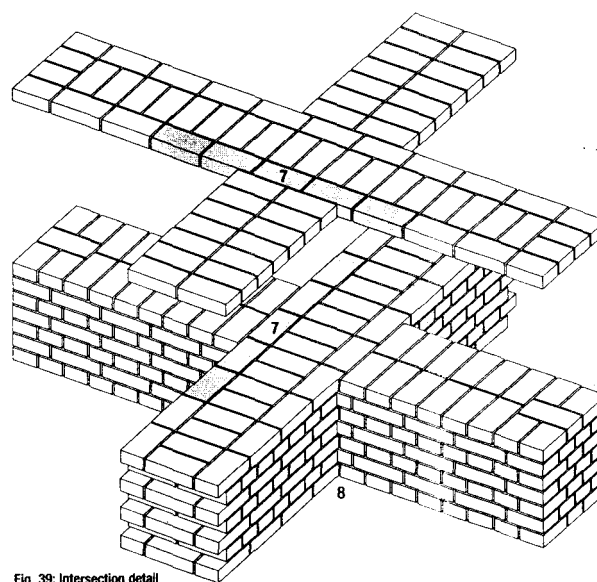
Fig. 39: Intersection detail
