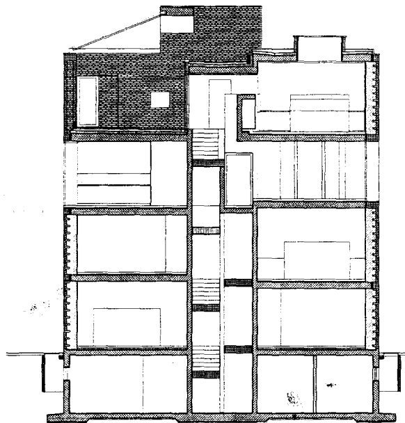
Fig. 44: Section Showing rooftop terrace to penthouse
