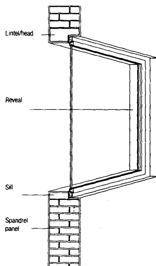
Fig. 23: Isometric view of opening rebates
