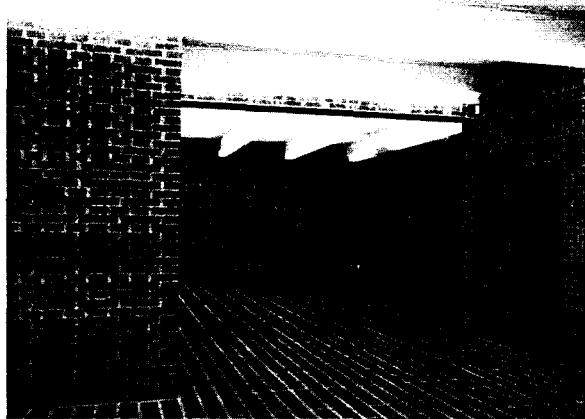
Fig. 83: Artificial lighting fitted to bottom flanges of beams
