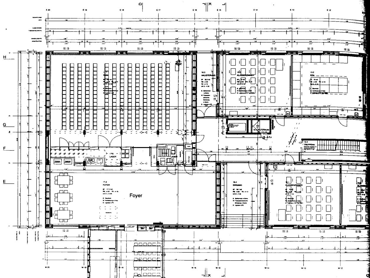
Fig. 272: Plan of ground floor (reduced 1:50 working drawing)
