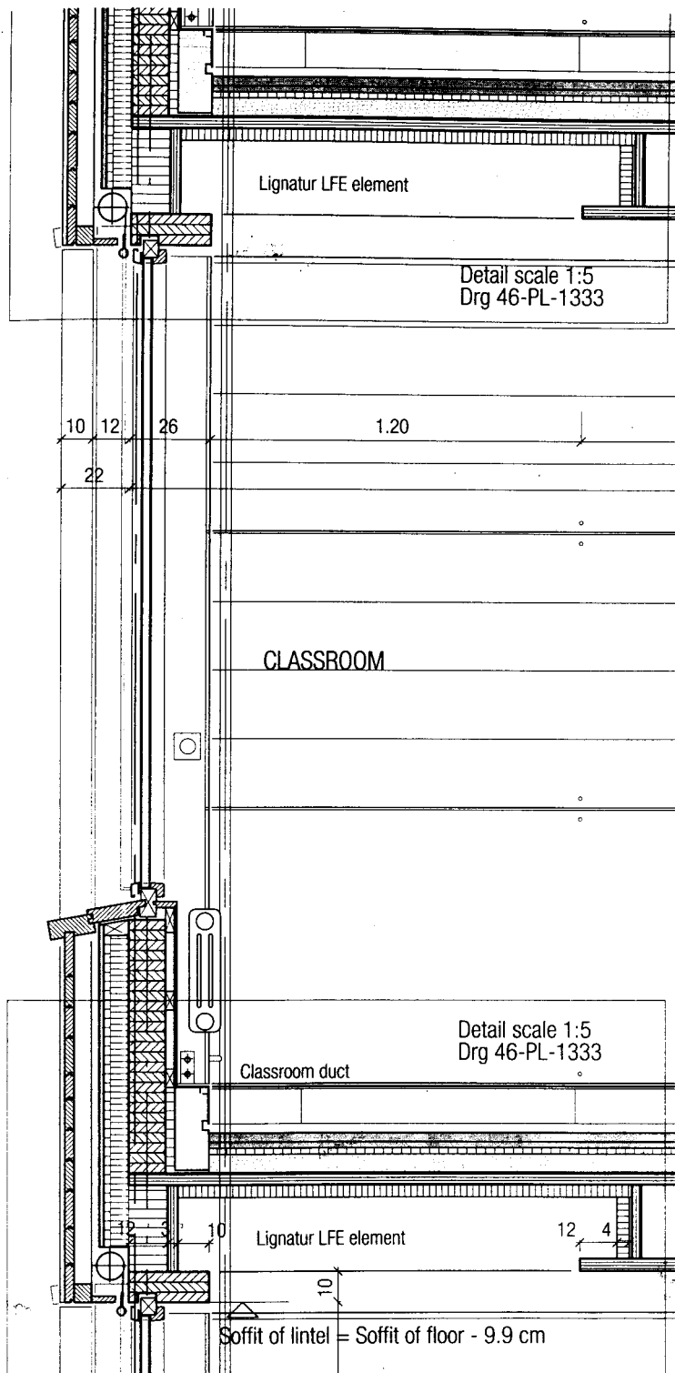
Fig. 279: Window detail, 1:20
