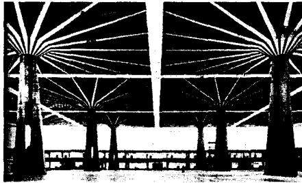
Fig. 76b: Canopies of concrete and steel, bay size 38 x 38 m Pier Luigi Nervi: Hall of Labour, Turin (I), 1961
