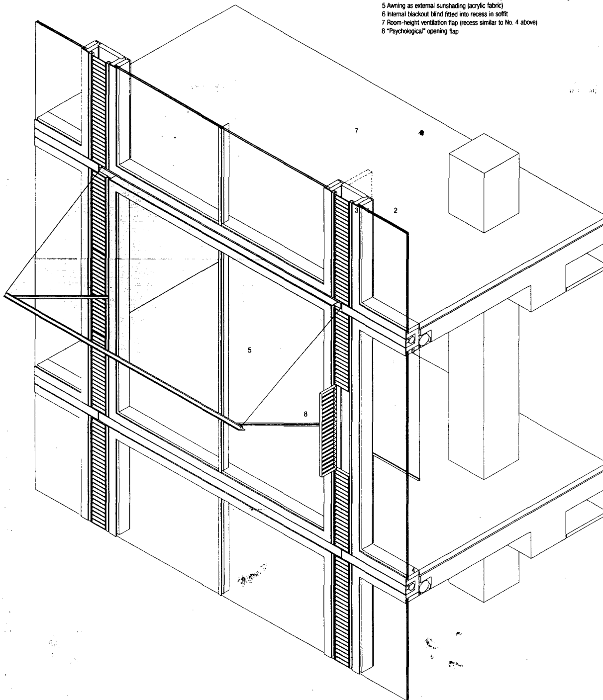
Fig. 247: Facade details
