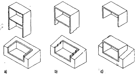
Fig. 69: Plinth forms for sloping sites a) Building in open excavation (“protective screen”) b) Building, or rather superstructure, supported on sides of excavation c) “Basement storey” supporting upper floor
