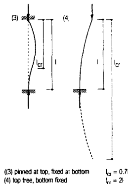
(1) pinned top and bottom l_{cr} = l (2) fixed top and bottom l_{cr} = 0.5l
