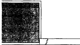
Fig. 64: Frame in opening, finished flush (internal and external doors) rebated door leaf flush with frame
