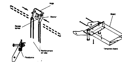
Fig. 41: A Installation work in the factory, temporary fittings in the form
