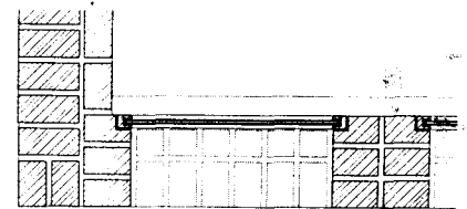
Fig. 80: Horizontal section through window showing special reveal bricks
