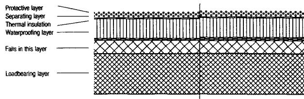
Fig. 13: Section through upside-down roof
