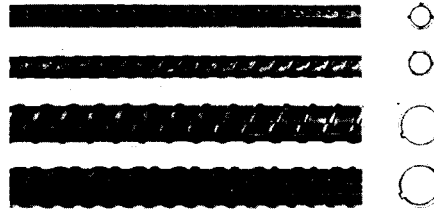
Fig. 13: Profiles of reinforcing bars
