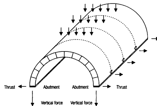
Fig. 40: Barrel vault
