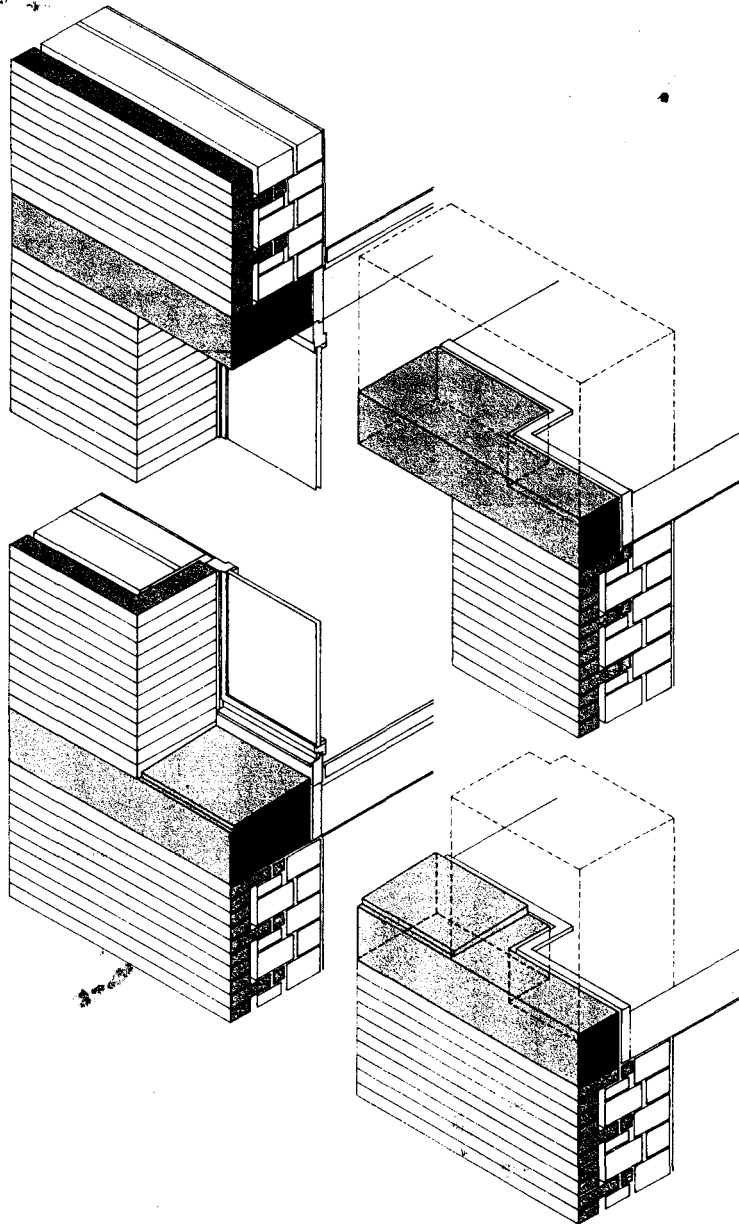
Fig. 50: Axonometric view "Thickening" of slab edge elements adjacent to window
