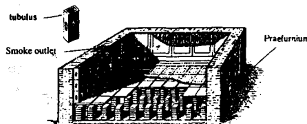
Fig. 90: Isometric view of hypocaust (hypocaust = heating from below)
