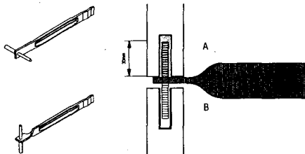
Fig. 45: Cast-in dowel in horizontal joint
