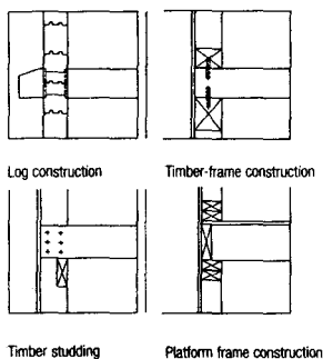
Fig. 9: Various types of timber construction
