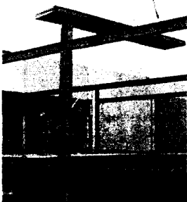
Fig. 49: Erecting a floor of hollow-core planks
