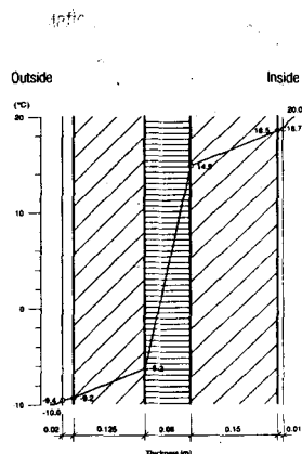
Fig. 1: Multi-layer wall construction Temperature gradient within the layers
