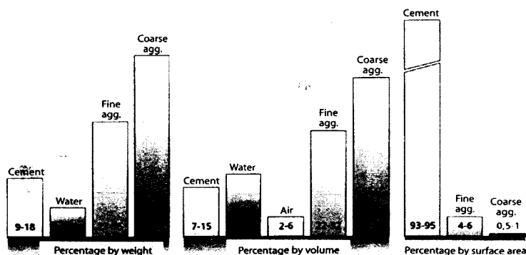
Fig. 7: Composition of concrete
