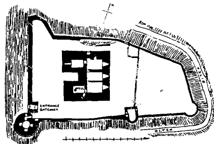
Fig. 74: Plan of whole complex Borthwick Castle, Midlothian (Scotland, GB), 15th century
