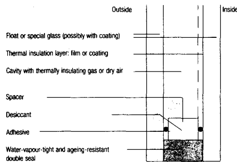
Fig. 26: Schematic diagram of insulating glazing construction
