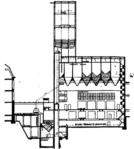
Fig. 44: Section through boiler house
