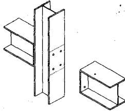
Bolted, end plate welded to beam
