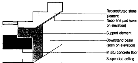
Fig. 33: Detail of support
