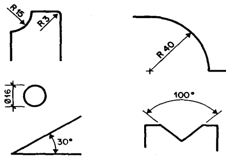
Fig. 7: Specifying radii, diameters and angles
