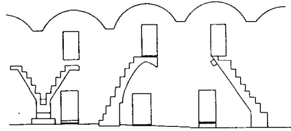
Fig. 68: Ghorfa type B Elevation, 1:200
