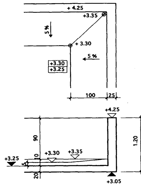
Fig. 10: Example: levels on plan and in section
