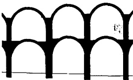
Fig. 17: Cross-section Ksar Ferich, fortified storehouse (Tunisia)
