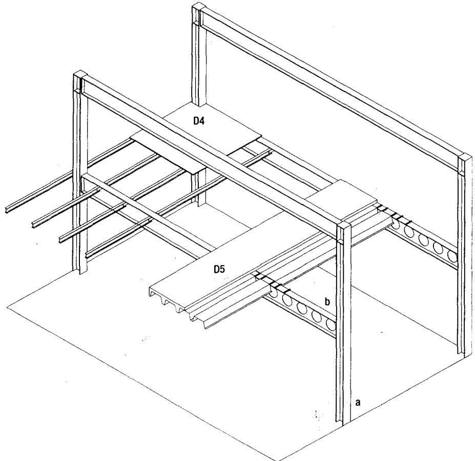
Fig. 40: Frame with continuous columns Shown here with floor constructions shallower than the beams
