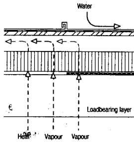
Fig. 14: Schematic drawing of building performance parameters
