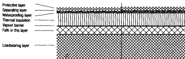
Fig. 9: Section through warm deck (bituminous roof covering)
