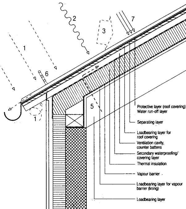
Fig. 46: Pitched roof, ventilated sheet metal, scale 1:20
