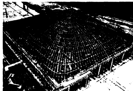
Abb. 71: Shell designed as membrane form, built over centering Heinz Isler (with VSK and Frei Architekten): COOP warehouse, Otten (CH), 1960
