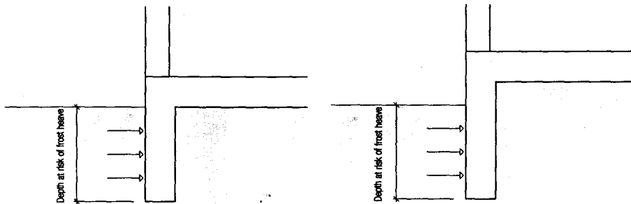
Fig. 45: Stem wall to provide frost protection
