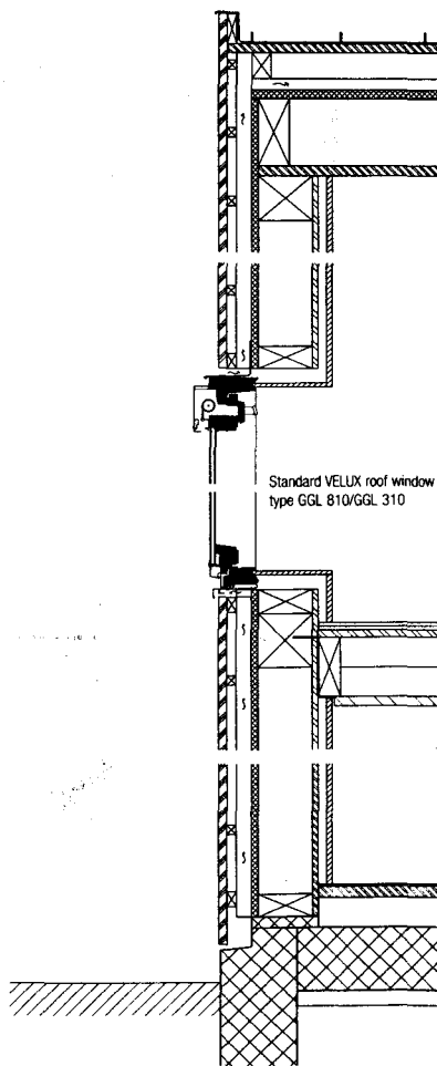
Fig. 301: Section through facade, 1:20
