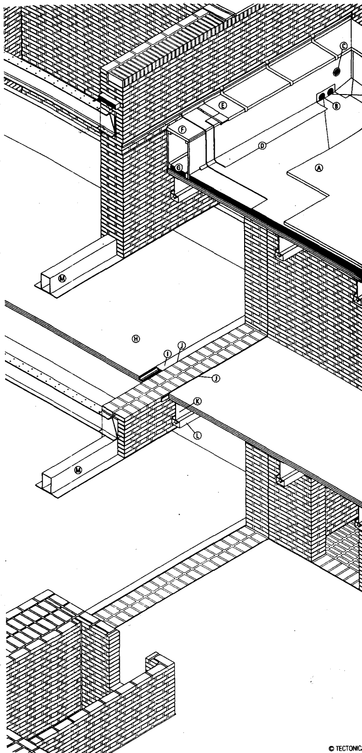
Fig. 75: Bearing for floor beam
