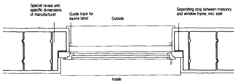
Plan of course 2
