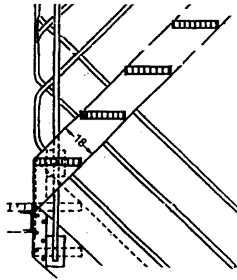
Fig. 41: Detail of stairwell
