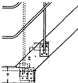
Fig. 43: Detail of connection between outer string and landing
