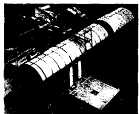
Fig. 54: Loadbearing structure and building envelope united in the form of semicircular, loadbearing sandwich elements, shown here almost complete. Jean Prouvé: La Méridienne de l'observatoire, Paris (F), 1951
