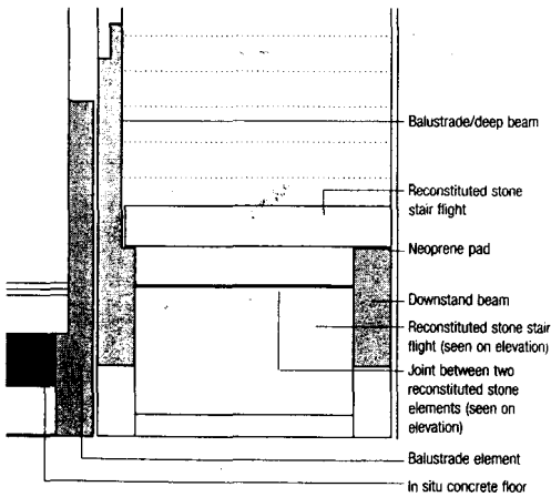
Fig. 34: Cross-section through stair
