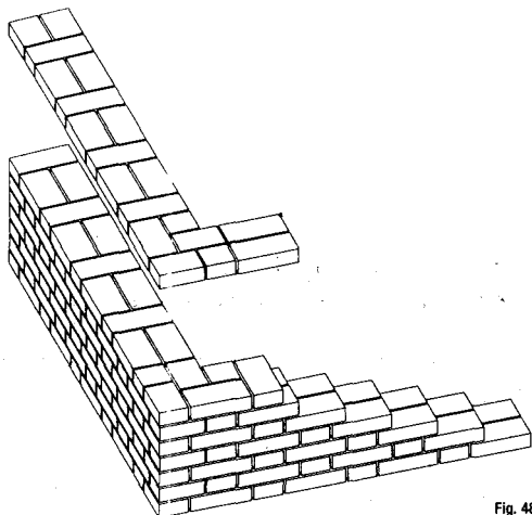
Fig. 48: Flemish bond
