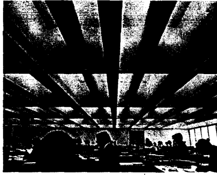
Fig. 27: Floor slab without intervening columns, with ventilation ducts and lighting units between the ribs SOM: American Republic Insurance Company, Des Moines (Iowa, USA), 1965
