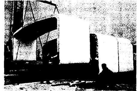
Fig. 129: Shell-type building envelope made from polyurethane Addition of self-supporting room segments
