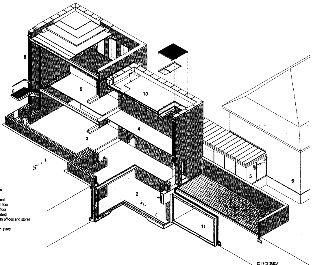
Fig. 74: Axonometric view
