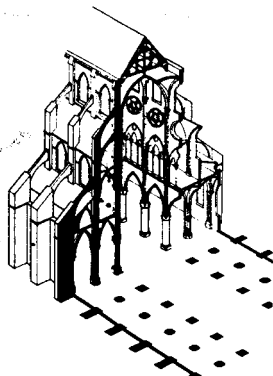
Fig. 32: Flying buttresses to transfer thrust, e.g. from vaulting Axonometric cut-away view of a Gothic cathedral
