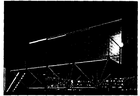
Fig. 70: The space frame distributes the loads of the building to four pad foundations. Bentham Crouwel: private house, Almere (NL), 1984
