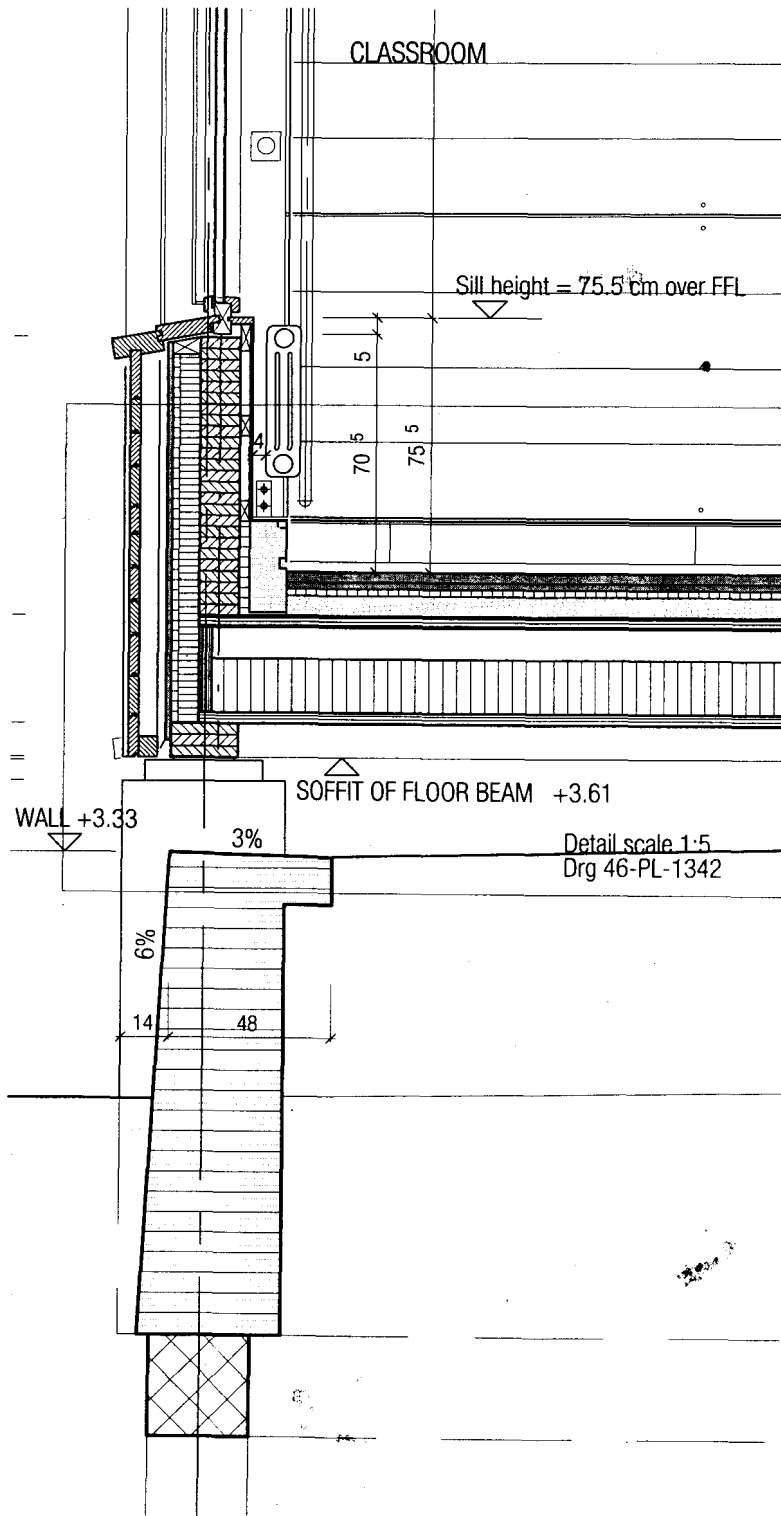
Fig. 276: Plinth detail, 1:20
