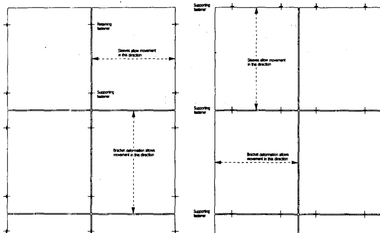
Fig. 46: Elevation on panels
