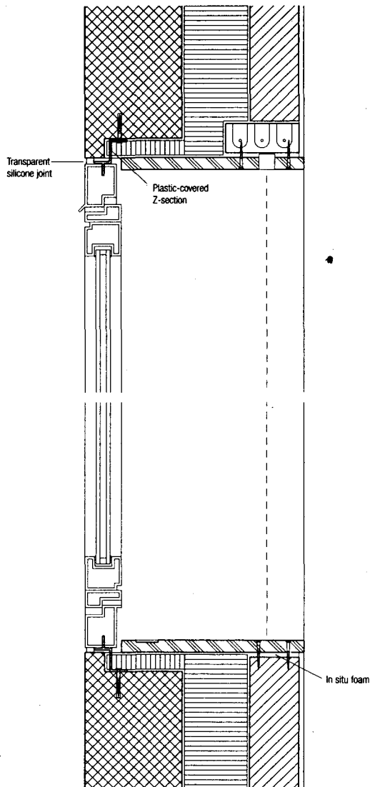
Fig. 113: Section through window, 1:10
