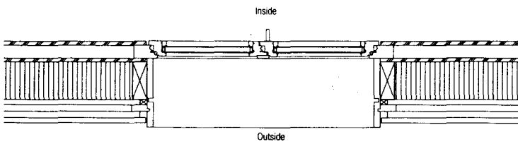
Plan 1
