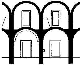
Fig. 59: Ghorfa type A Section, 1:200
