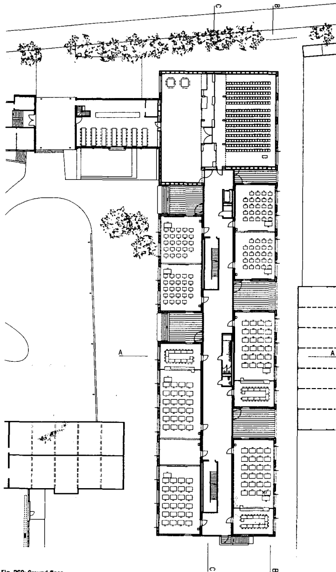
Fig. 260: Ground floor
