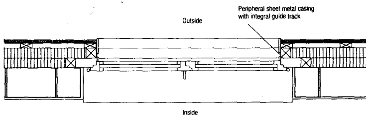
Plan of course 2
