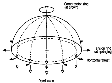
Fig. 42: Dome (body of revolution)
