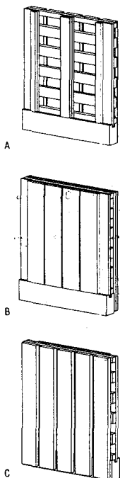
Fig. 31: Lignotrend wall elements A) Open both sides B) Closed on both sides C) Closed on one side
