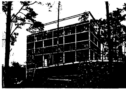
Fig. 10: Steel frame during construction Wassili and Hans Luckhardt: house on Rupenhorn, Berlin (D), 1928
