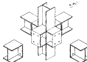
Bolted, end plates welded to column
