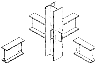
Bolted, cleats welded to column
