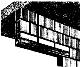
Fig. 30: Solid lintel element ("Stahlton") Prestressed shallow lintel with make-up units to maintain the masonry courses
