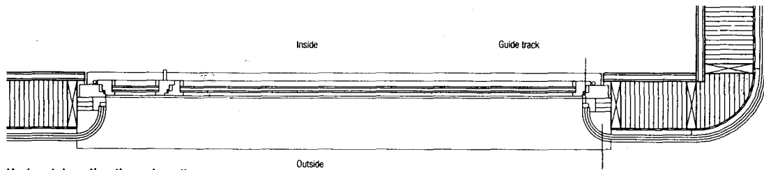
Horizontal section through wall
