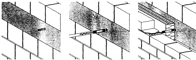
Fig. 56: Installation sequence, wall tie in concrete - Drill hole in concrete and insert metal anchor. - Screw in wall tie. - Push insulation over wall tie, cast tie into bed joint of second (facing) leaf.
