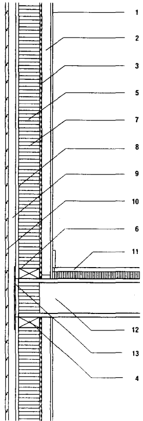
Section through wall-floor junction Horizontal sheathing
