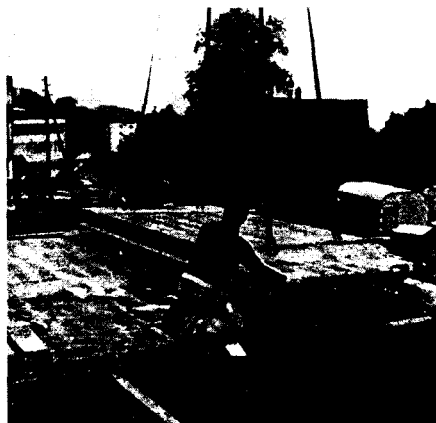
Fig. 1: Top: hollow clay blocks and reinforced concrete ribs; bottom: erection of factory-prefabricated elements (here: Bricosol products)
