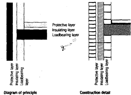
Fig. 16: Case study: double-leaf masonry, wall-floor junction The protective layer is realised as a self-supporting masonry leaf, e.g. using clay or calcium silicate bricks, and partial tying back to the loadbearing layer is necessary owing to the instability of the non-loadbearing external leaf in the case of multistorey buildings. The use of double-leaf masonry results in the thickest wall construction.
