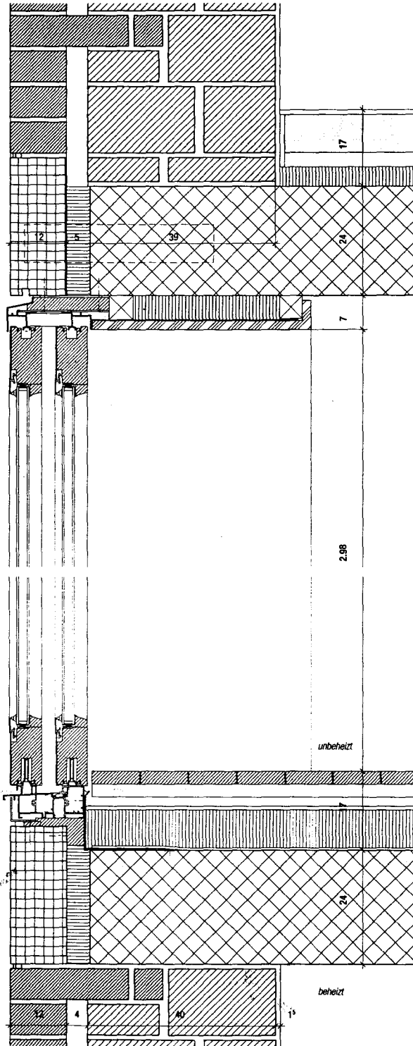
Fig. 63: Section, 1:10 At the sliding windows the slab edge elements are fixed with OMEGA anchors.
