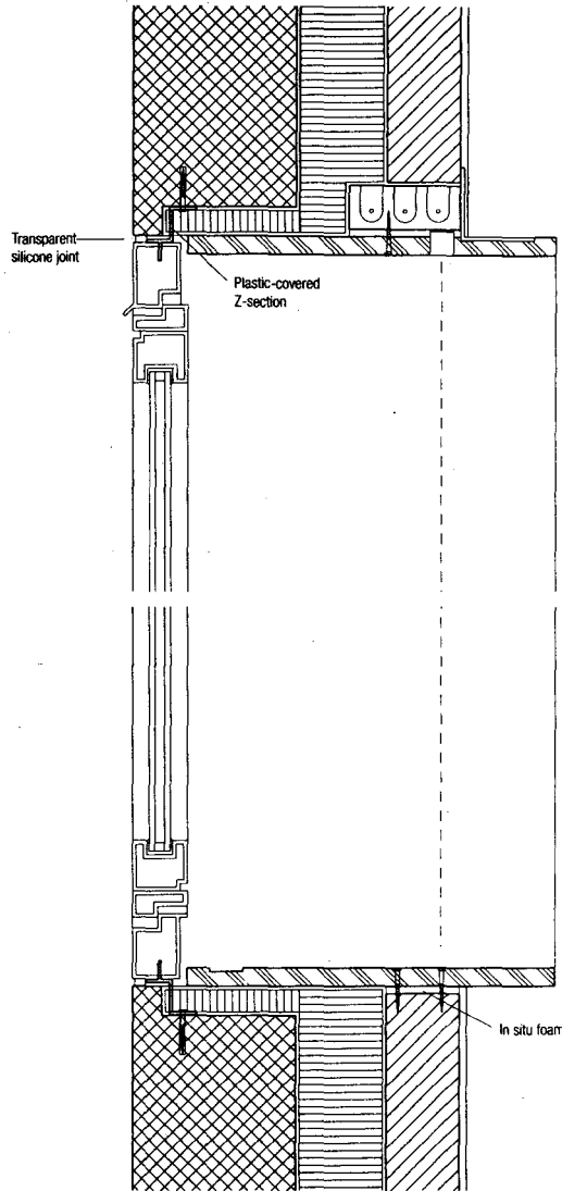
Fig. 118: Section through window, 1:10
