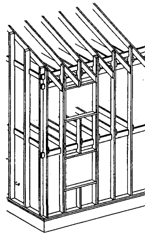
Fig. 40: Balloon frame construction, timber stud construction
