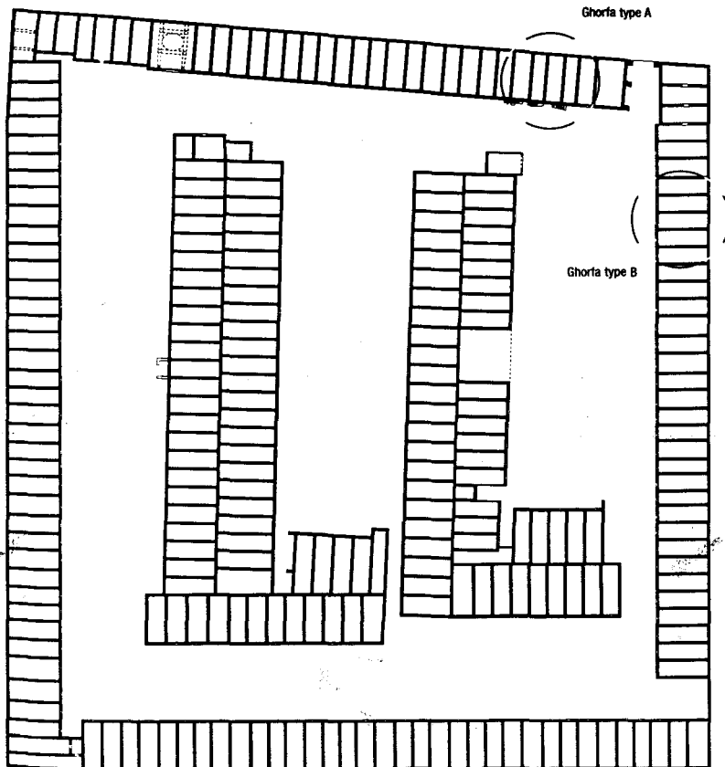
Fig. 58: Ksar Ferich Plan of ground floor, 1:1000
