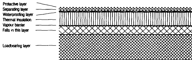
Fig. 8: Section through warm deck (synthetic roof covering)
