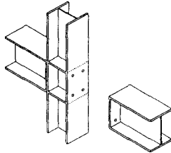
Bolted, stiffeners welded to column in line with beam flanges
