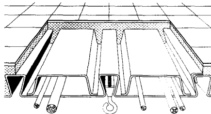
Holorib® metal sheeting
