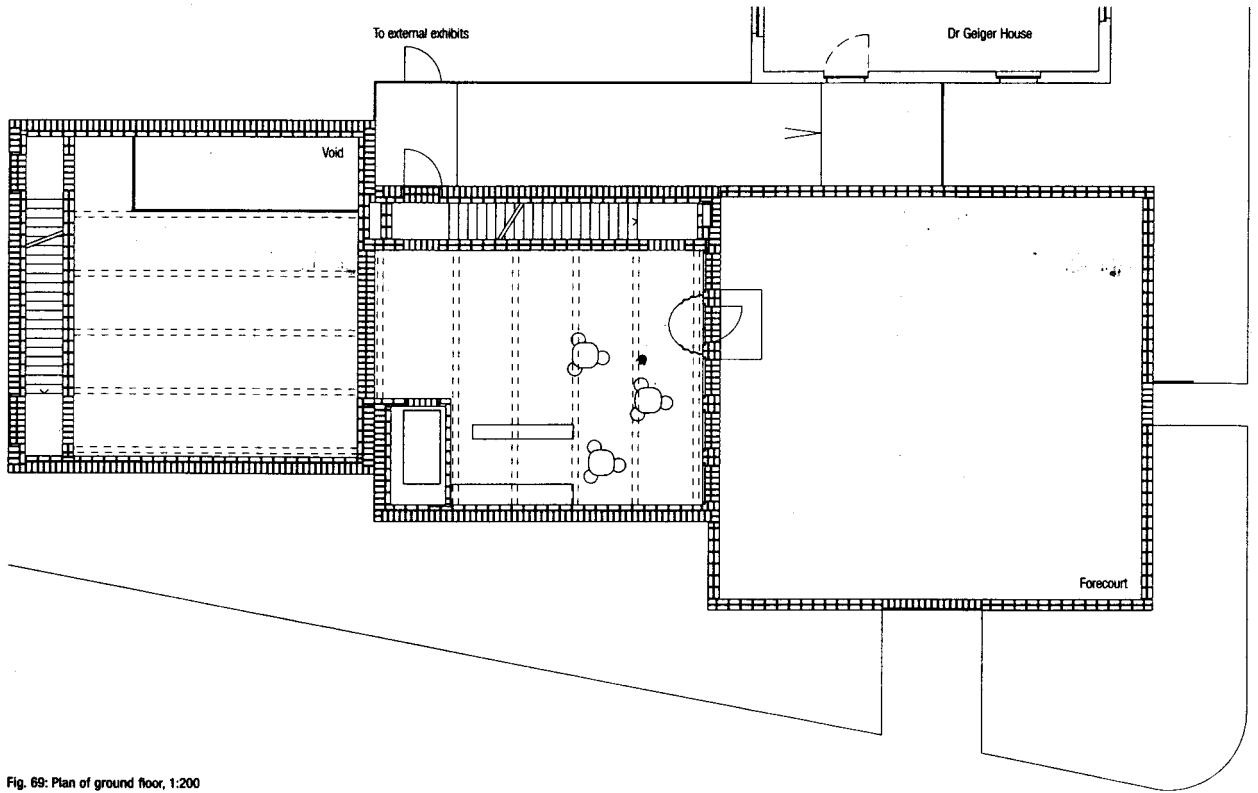
Fig. 69: Plan of ground floor, 1:200
