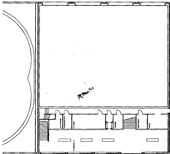
Fig. 160: Plan of ground floor, 1:500
