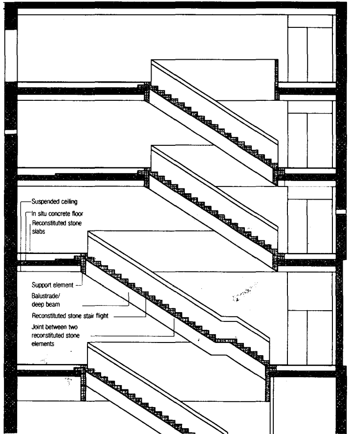
Fig. 35: Section through stair shaft
