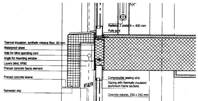
Fig. 231: Floor slab edge detail, 1:20
