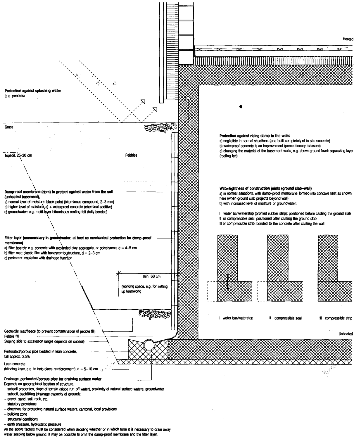
Fig. 70: External wall, scale 1:20
