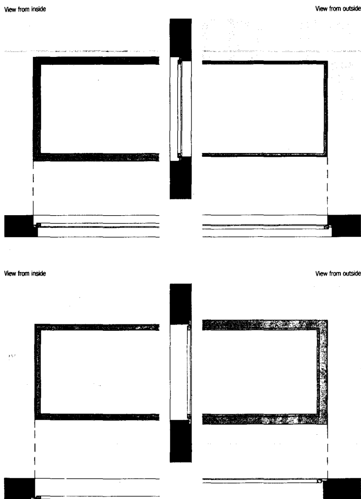
Fig. 24: Window opening inwards (top), opening outwards (bottom)
