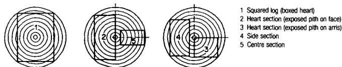
Fig. 10: Conversion options for squared sections and battens (to Swiss standard SIA 256/1 5.3.6.1: Timber construction – supplementary provisions)
