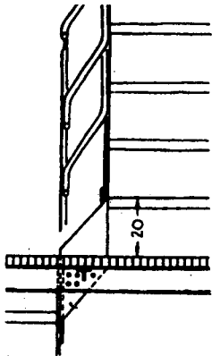
Fig. 42: Detail of stair/landing junction
