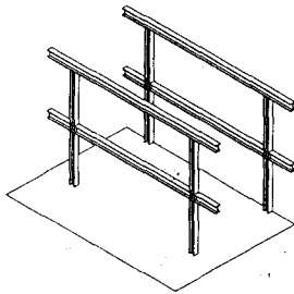
Fig. 35: Frame with cantilevering beams
