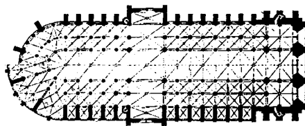
Fig. 33: The external loadbearing structure (flying buttresses) resulted in recesses which were later converted into chapels (along bottom edge of plan). Notre Dame Cathedral, Paris (F), begun in 1163
