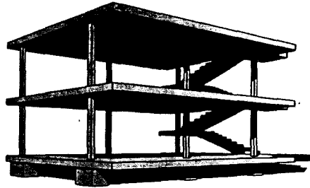
Fig. 115: Loadbearing structure in concrete, with cantilevering floor slabs and bracing provided by the staircase Le Corbusier: Dom-ino project, 1914
