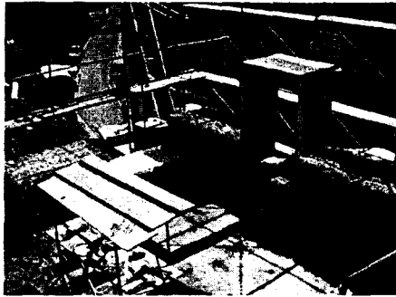
1 Reveals to openings mounted on concrete foundation; first course of straw bales in position
