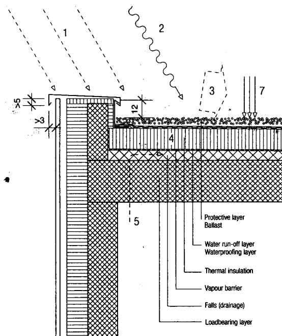
Fig. 45: Flat roof, warm deck, scale 1:20
