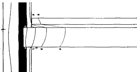
Fig. 35: Isotherms diagram
