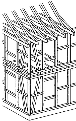
Fig. 39: Timber-frame construction
