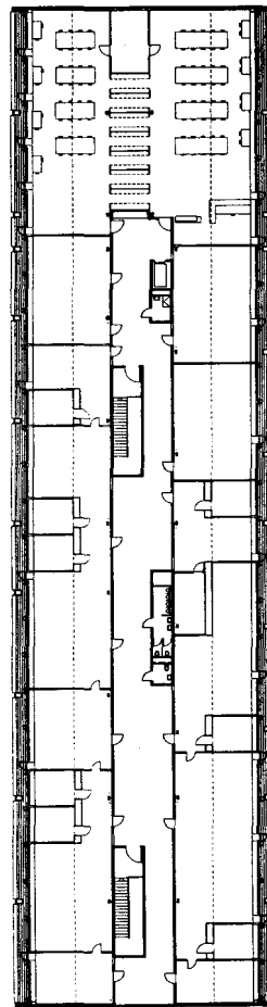
Fig. 265: 3rd floor
