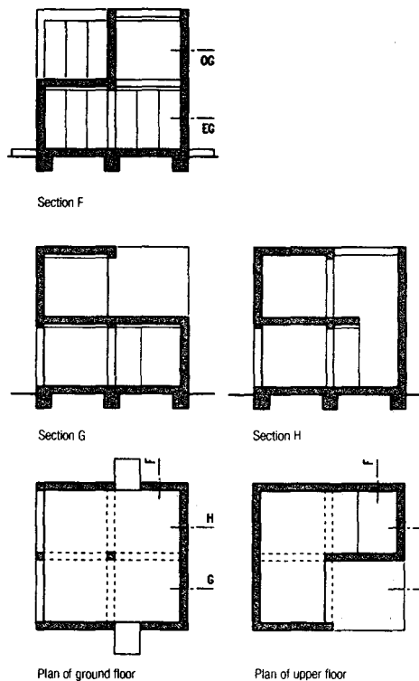
Fig. 13: Standard projection Representation of a sectioned object
