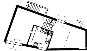
Fig. 293: Ground floor
