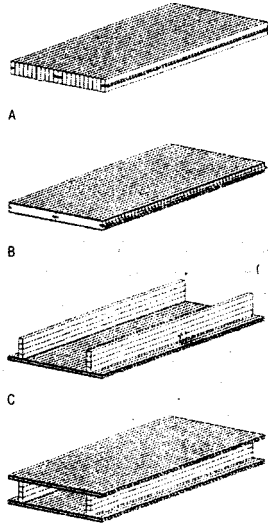
Fig. 28: Schuler solid timber panel A) Single-ply panel B) 3- and 5-ply panels C) Ribbed panel D) Box panel
