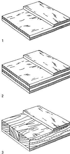
Fig. 17: Lay-up of plywood 1: 3-ply plywood 2: 5-ply plywood 3: Wood-based core plywood
