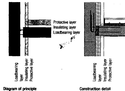
Fig. 19: Case study, floor support separated, continuous insulating layer This type of construction is only possible in reinforced concrete because the chromium steel anchors must be integrated into the wall and floor reinforcement. Compression-resistant insulation must be incorporated between the face of a wall and the edge of the floor. Such insulation is often included with the respective anchor system (e.g. Schöck-Isokorb).
