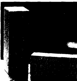
Fig. 37: Wood welding The application of ultrasonic energy causes the plastic to form a connection with the wood at the macroporous level.
