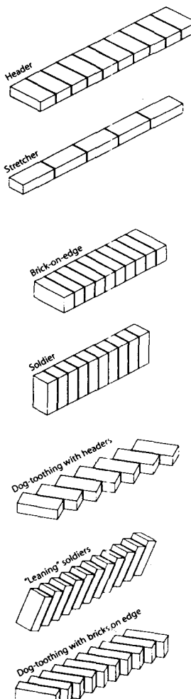
Fig. 33: Different types of course
