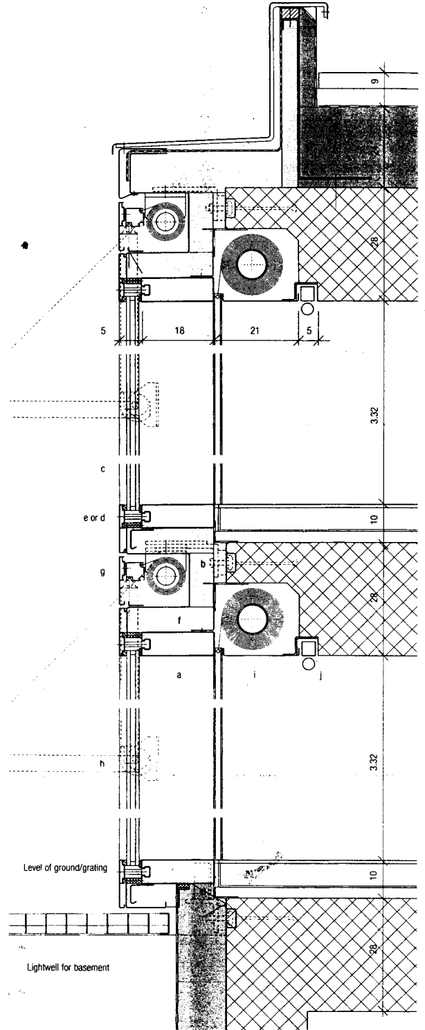
Fig. 250: Vertical section
