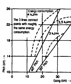
④ Energy consumption for an adult climbing a flight of stairs
