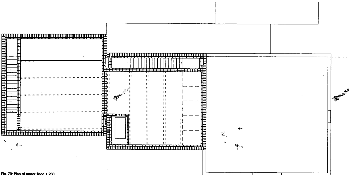
Fig. 70: Plan of upper floor, 1:200
