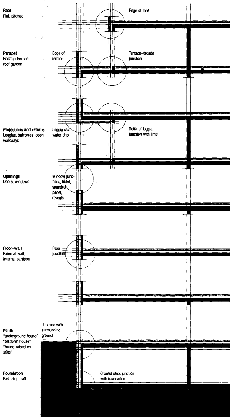
Fig. 14: Diagram of layers, loadbearing layer inside
