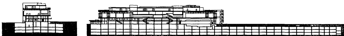
Fig. 3: The internal layouts of substructure and superstructure have developed independently of each other but still use a common column grid. Roland Rohn: Hoffmann-La Roche staff accommodation, Basel (CH), 1971
