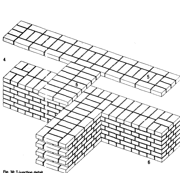
Fig. 38: T-junction detail
