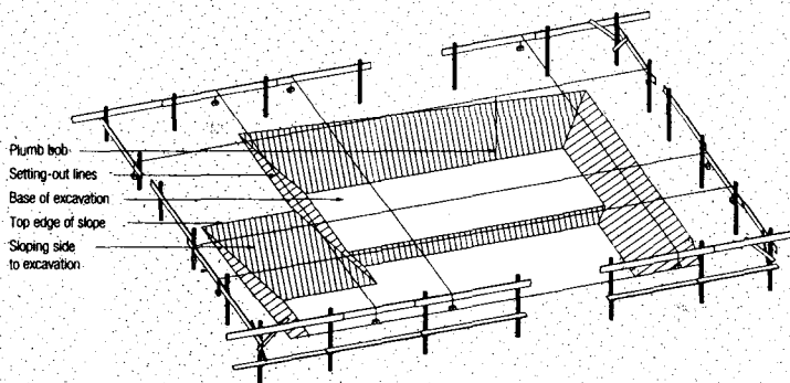
Fig. 40: Excavation with sloping sides
