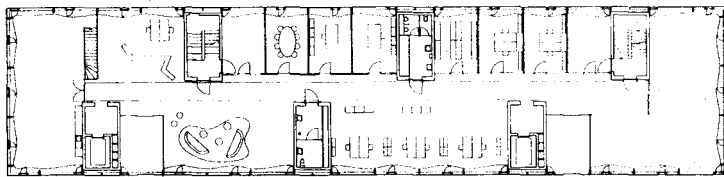
Fig. 6: Column-free plan layout with loadbearing facade and cores (lifts, wet rooms or stairs) Beath & Deplazes: ÖKK offices, Landquart (CH), 2001/02
