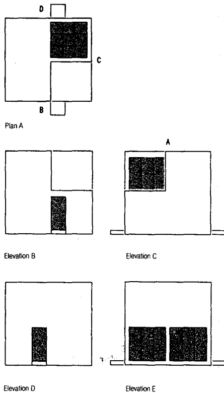
Fig. 11: Standard projection Representation of a non-sectioned object
