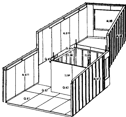
Fig. 48: Axonometric view of wall elements offset to accommodate split-level floor
