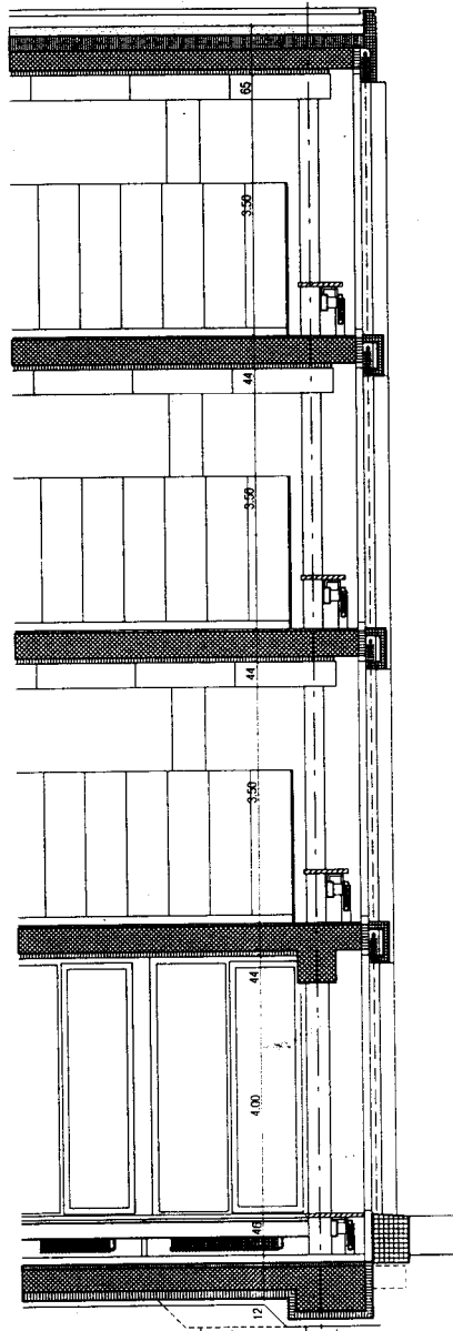
Fig. 221: Section, 1:50
