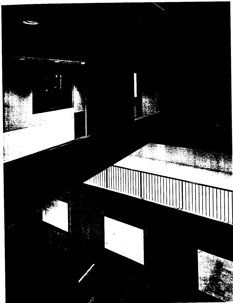
Fig. 192: Upper atrium, looking down towards entrance level. The walls without intermediate supports act as storey-high deep beams.
