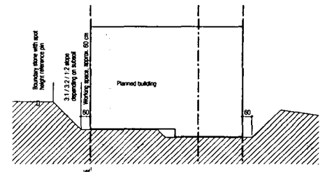
Fig. 41: Schematic section through excavation
