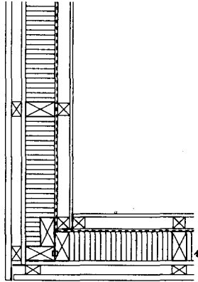
Horizontal section through corner joint Horizontal sheathing
