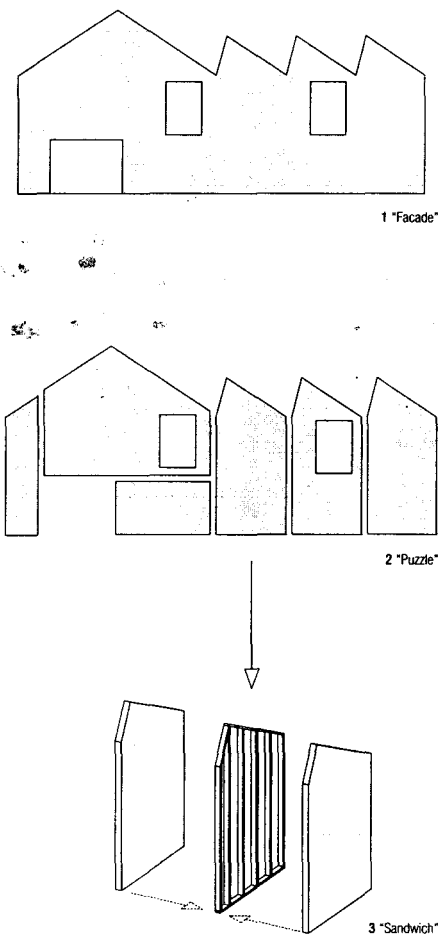
Fig. 49: Timber platform frame construction as a "building kit"
