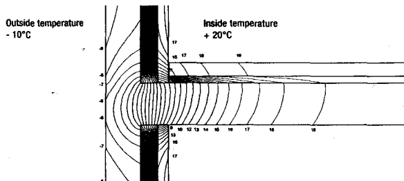
Fig. 30: Isotherms diagram
