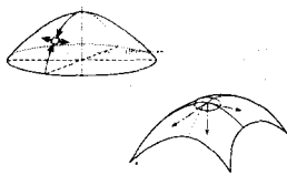
Fig. 67: Forms with double curvature
