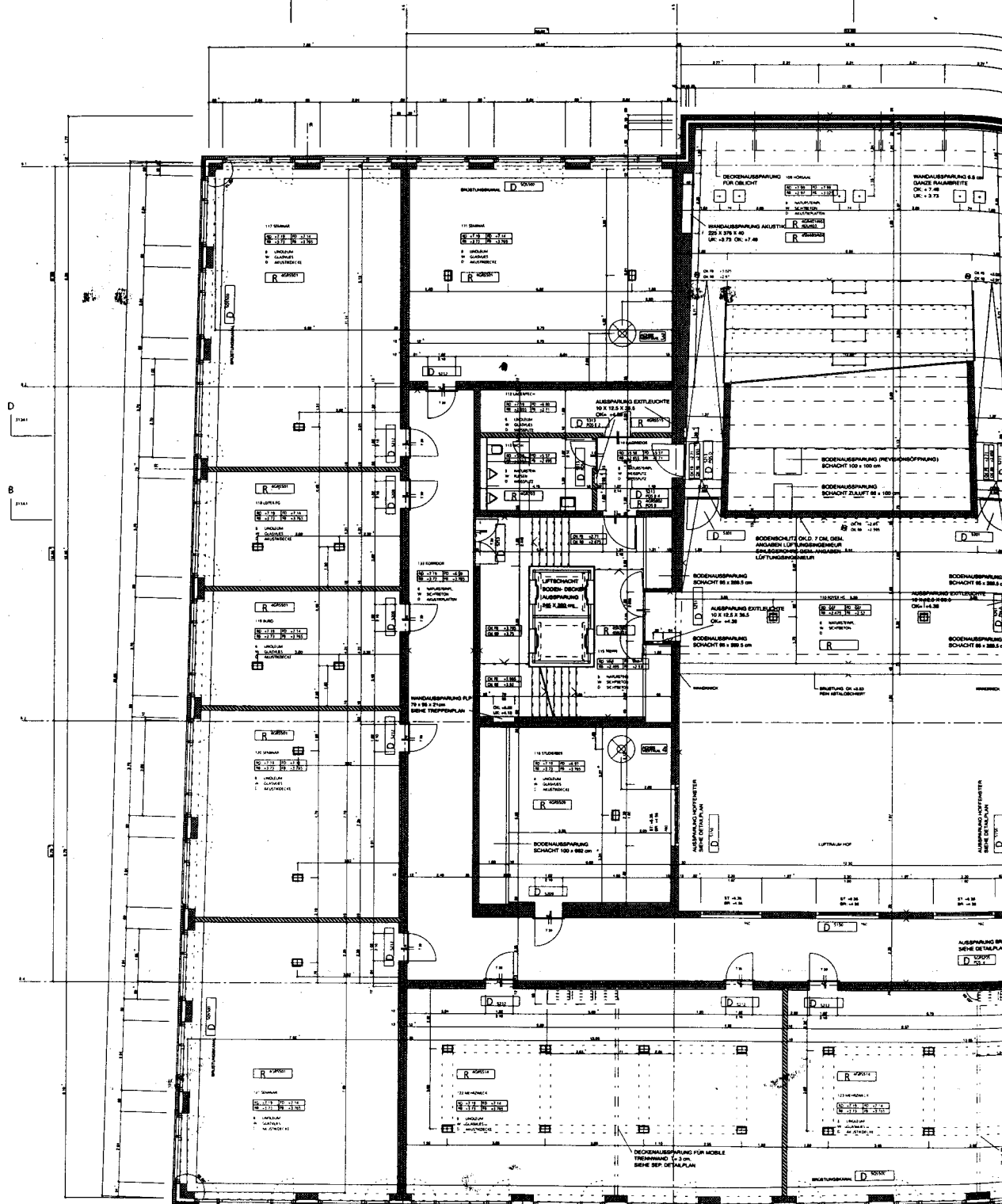
Fig. 193: Working drawing of 1st floor, 1:50 (reduced here to 1:200)
