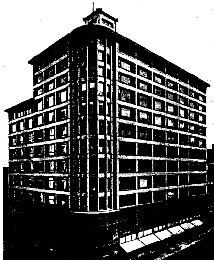
Fig. 6: The opening–wall ratio points to a frame behind the facade. Louis Henry Sullivan: Schlesinger & Mayer department store, Chicago (USA), 1904
