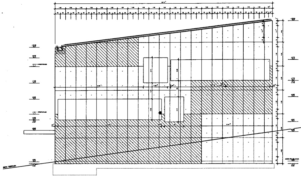
Fig. 145: South elevation, formwork layout, 1:200 1:50 working drawing (reduced)
