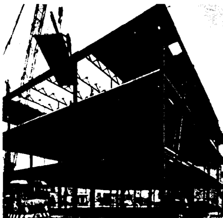
Fig. 12: Primary structure of (solid) rolled sections, secondary structure of (open) lattice beams
