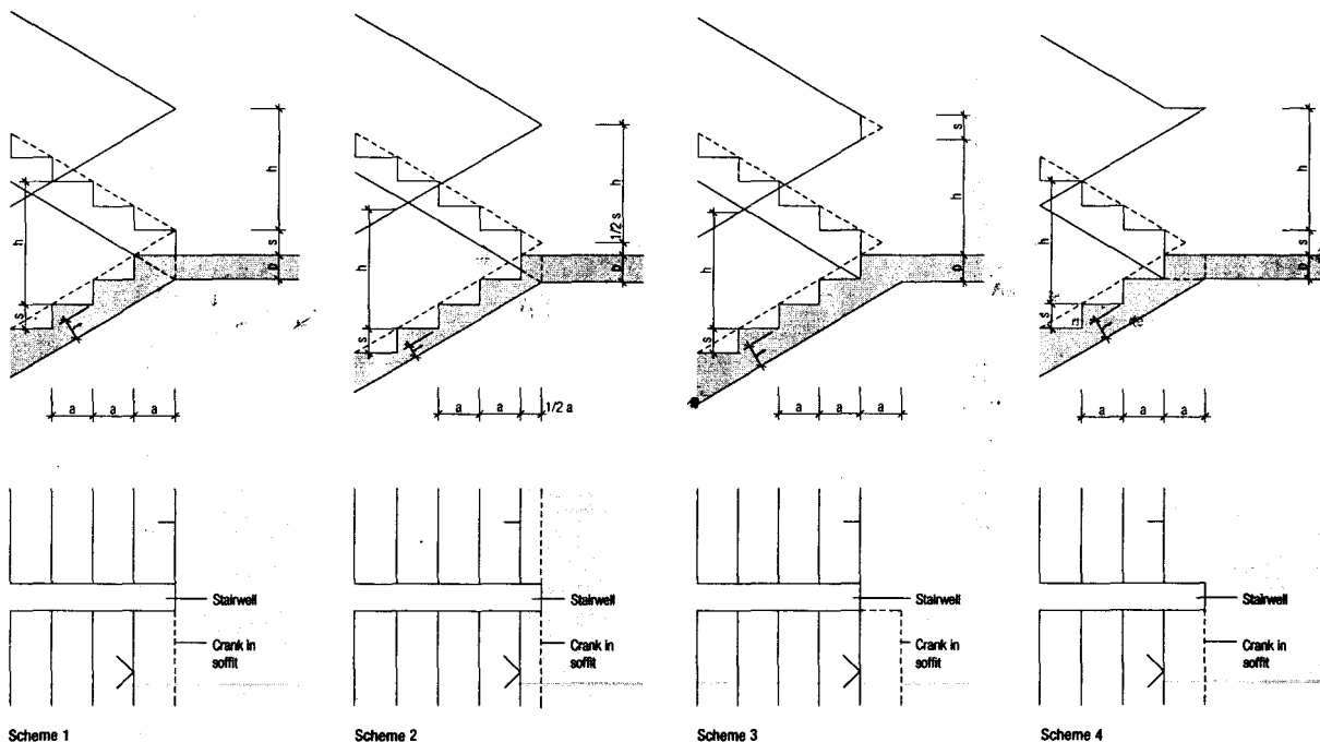
Fig. 22: Schemes (above) a Going (step depth) s Rise (step height) h Height of balustrade p Thickness of landing slab t Thickness of stair slab
