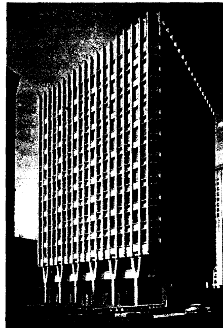
Fig. 23: Amalgamation of loadbearing structure and vertical service ducts Paul Rudolph, with Anderson, Beckwith & Haible: Blue Cross Building, Boston (Mass., USA), 1958
