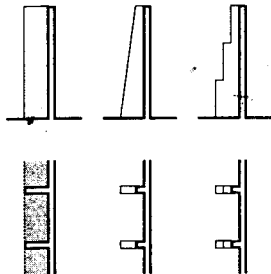
Fig. 29: Walls reinforced with ribs, sections (top) and plans (bottom) for increasing the inherent stability
