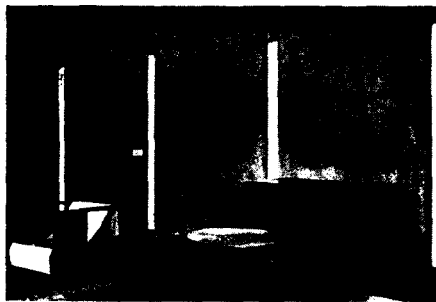
Fig. 128: The concrete panels were cast on the ground (top) and afterwards lifted into position (bottom). Rudolf Schindler: Schindler House, Los Angeles (USA), 1921–22
