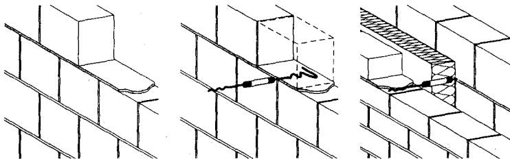
Fig. 55: Installation sequence, wall tie in mortar joint - Spread mortar. - Place wall tie in mortar and lay masonry unit on top. - Push insulation over wall tie, cast tie into bed joint of second (facing) leaf.
