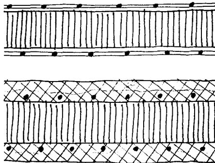
Fig. 3: Sketches of wall construction (horizontal sections) Top: the rigid PU foam insulation between two layers of reinforcing mesh serves as permanent formwork. Bottom: rigid PU foam insulation panel covered with two coats of sprayed concrete both sides Philip Johnson: Gate House, New Canaan (USA), 1995
