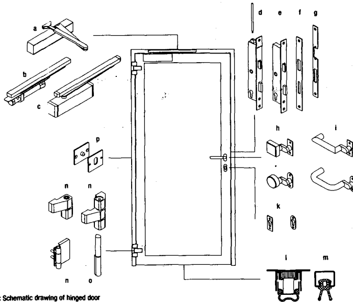
Fig. 71: Schematic drawing of hinged door
