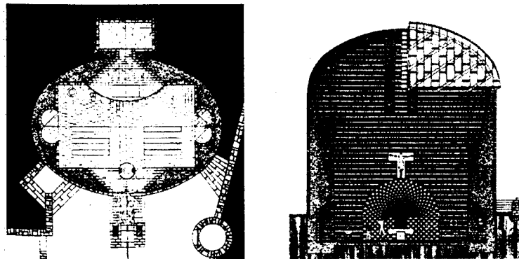
Fig. 47: Plan (above), section (right) Mario Botta: church in Mogno (CH), 1986-95
