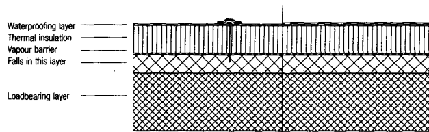
Fig. 11: Section through uncoated roof
