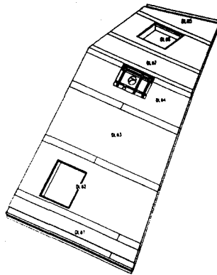
Fig. 295: Axonometric view of roof
