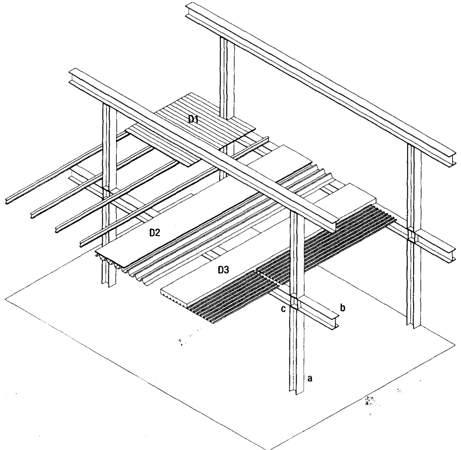
Fig. 36: Frame with continuous beams Shown here with floor constructions above level of primary structure
