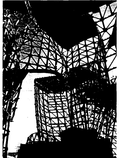
Fig. 18: The dynamic forms were translated into linear lattice structures. Frank O. Gehry: Guggenheim Museum, Bilbao (E), 1997
