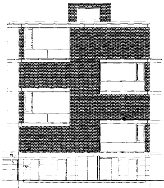
Fig. 46: North elevation
