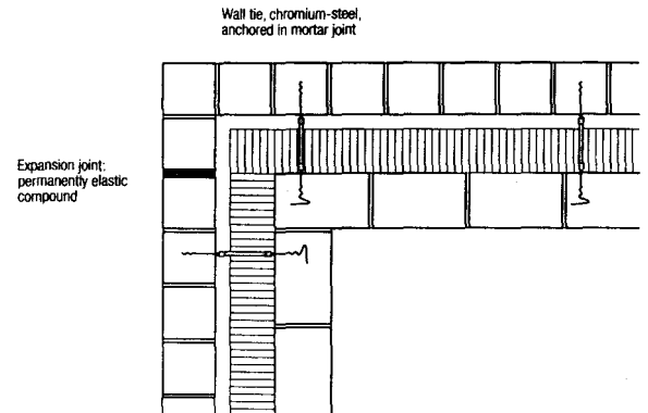
Plan, course 1
