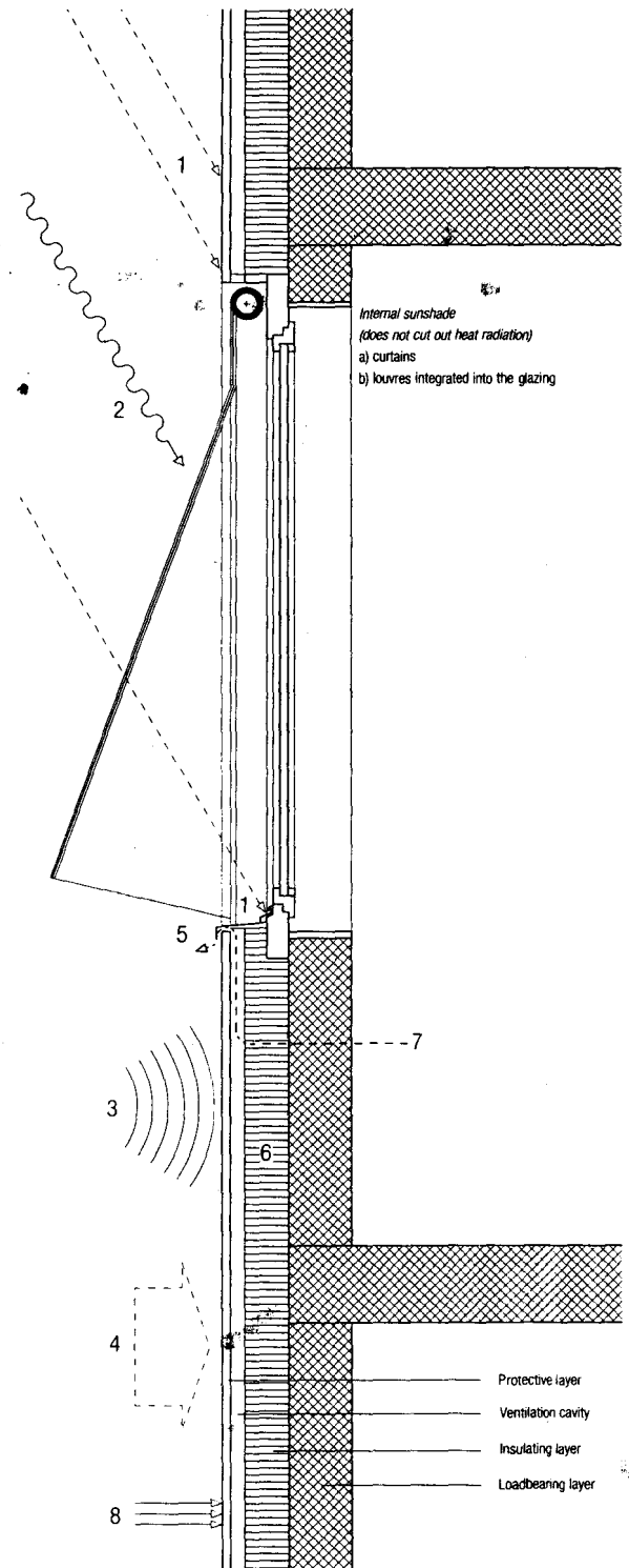
Fig. 73: Schematic section, scale 1:20
