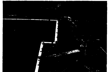
Fig. 51: Close-up of formwork The slab edge elements act as a permanent formwork; gypsum boards provide a space for the insulation.
