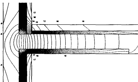
Fig. 32: Isotherms diagram
