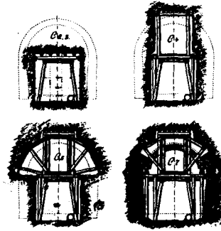
Fig. 11: Securing underground galleries with timber, enlarged upon provision of the lining Tunnel cross-sections through Albula railway line
