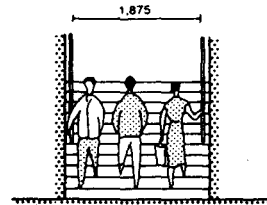
⑬ Minimum width for three persons
