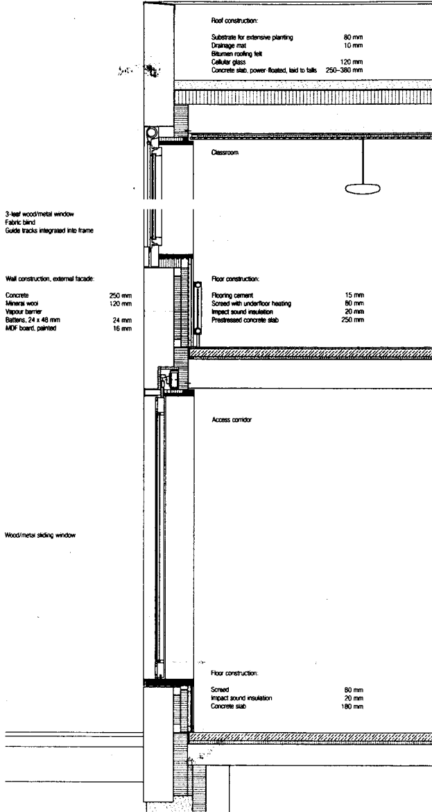
Fig. 166: Section through external facade
