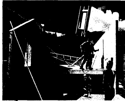
Fig. 47: Erection of platform frame elements with sheathing both sides Bearth & Deplazes: private house (Willimann), Sevgein (CH), 1998
