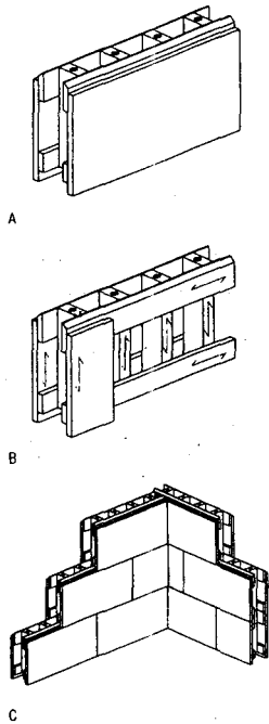
Fig. 35: Steko wall system A) Steko basic module B) Structure of module and direction of grain C) Wall corner detail
