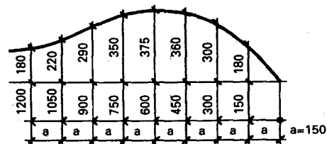
Fig. 8: Specifying an irregular curve
