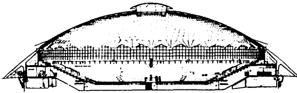
Fig. 41: The tension ring is below ground underneath the column foundations (abutments). Pier Luigi Nervi: Palazetto dello Sport, Rome (I), 1957
