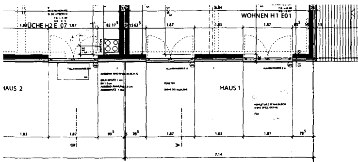
Example: dimensions on working drawings
