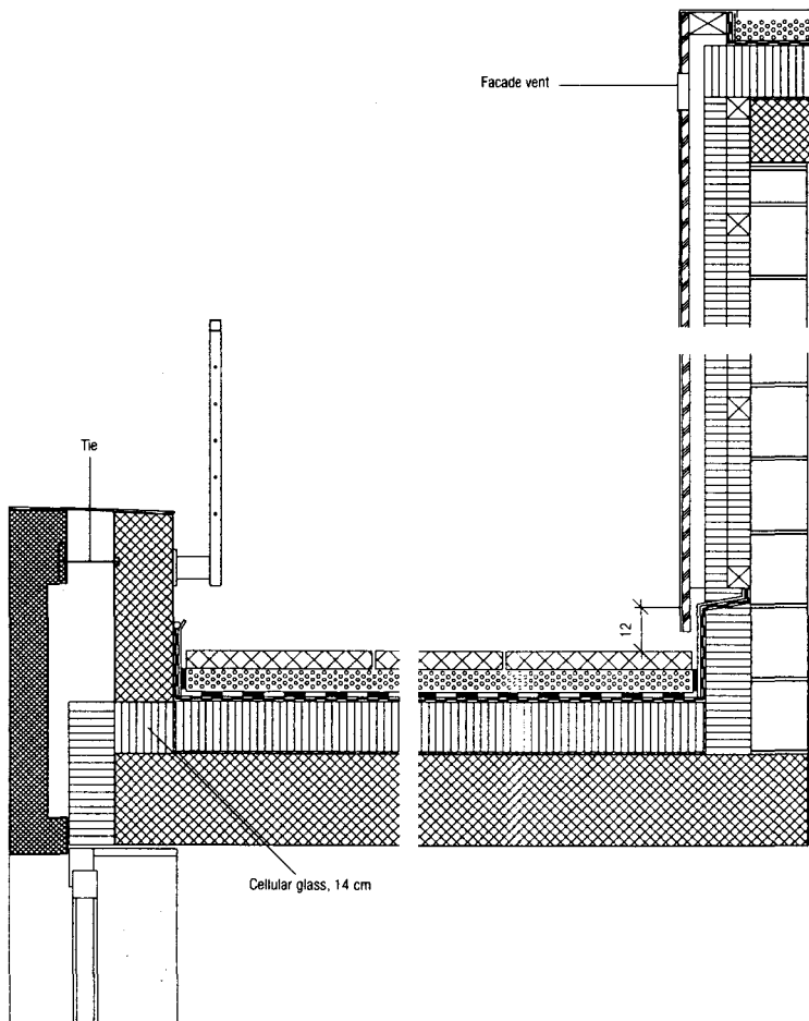
Warm deck, suitable for foot traffic, parapet; longitudinal section
