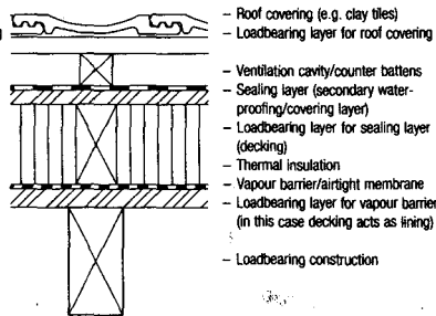
Fig. 2: Pitched roof with seamless secondary waterproofing/covering layer (warm deck)
