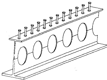
Fig. 44: Cellular beam Example with different top and bottom flanges to save weight
