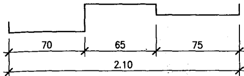
Fig. 5: String of dimensions with overall dimension
