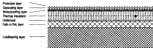
Fig. 10: Section through compact roof
