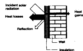
Conventional insulation
