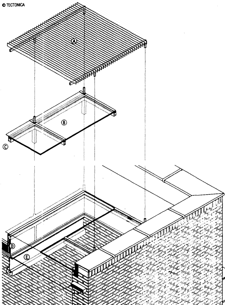
Fig. 82: Exploded diagram of rooflight
