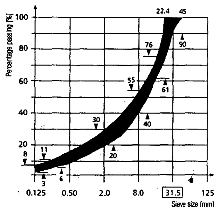
Fig. 12: Grading curve
