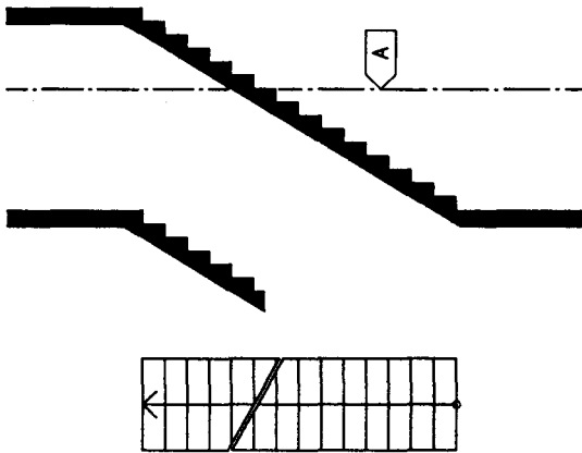
Fig. 14: Multi-storey stairs Plan and section
