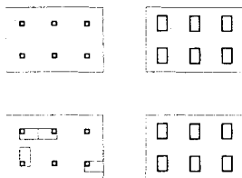
Fig. 8: Hollow columns – slender floor slabs Schemes showing load-bearing structure (top) and interior fitting-out (bottom); the wet rooms are linked to the loadbearing structure containing the services.
