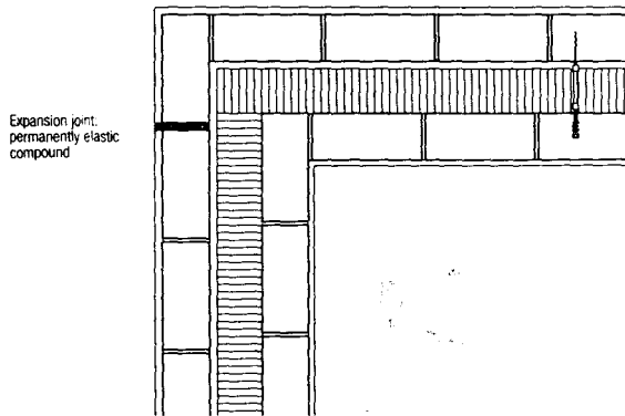
Plan, course 2
