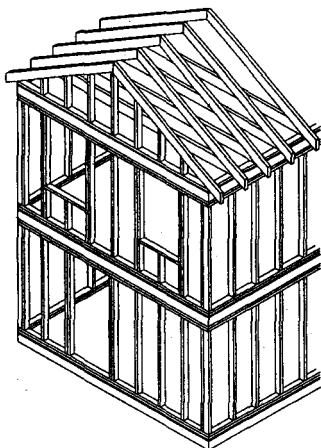
Fig. 41: Platform frame construction
