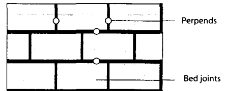
Fig. 35: Joint definitions
