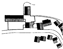
Fig. 18: Site plan Conradin Clavuot: School in St Peter (CH), 1997
