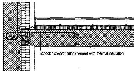
Fig. 38: Construction detail
