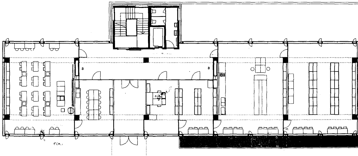
Fig. 238: Plan of ground floor The rooms are reached without the need for corridors. a) Vertical service shafts
