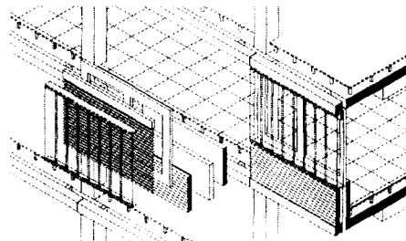
Fig. 80: Left: the various layers; right: element assembled and erected Swisscom headquarters: exploded axonometric view of facade
