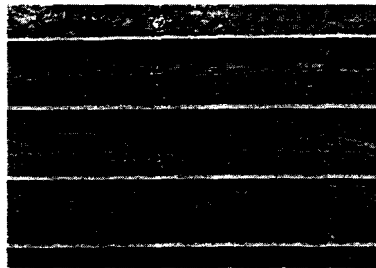
Fig. 25: Horizontal timber boards Formwork made from 18 cm wide, 3 cm thick Douglas fir boards, chamfered edges, tight butt joints between boards. Characteristic, projecting concrete fins are the result.
