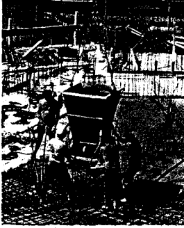
Fig. 21: Placing concrete by crane skip
