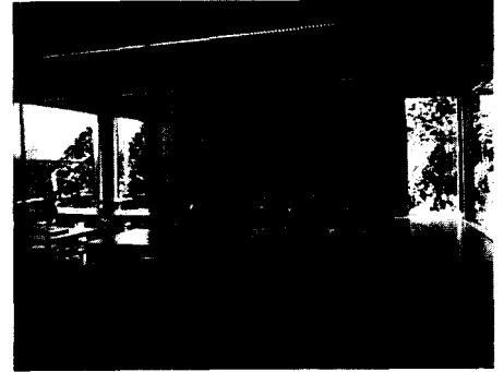
Fig. 240: Seminar room A suspended ceiling between the downstand beams, but only the bare concrete soffit adjacent to the facade (see section)
