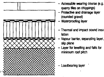
Fig. 5: Flat roof without ventilation (warm deck) accessible
