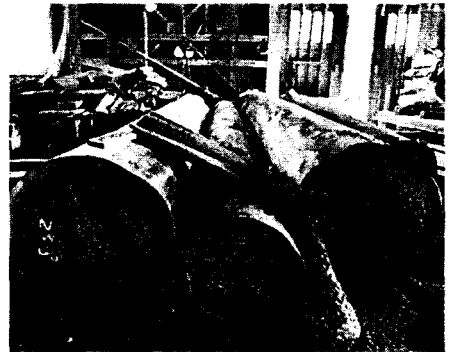
Fig. 55: Three tree trunks marked ready for cutting in the sawmill Visible here are the marked-out sections plus additional information such as building name, component name, component number, and trunk number.
