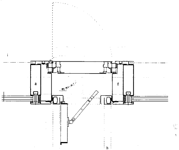
Fig. 249: Horizontal section Vertical joint with internal and external ventilation flaps
