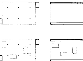
Fig. 9: Slender columns – hollow floors Schemes showing load-bearing structure (top) and interior fitting-out (bottom); the wet rooms are positioned independently of the loadbearing structure. Multistorey circulation is via perimeter shafts which can also function as vertical loadbearing elements. (see also figs 24–27).
