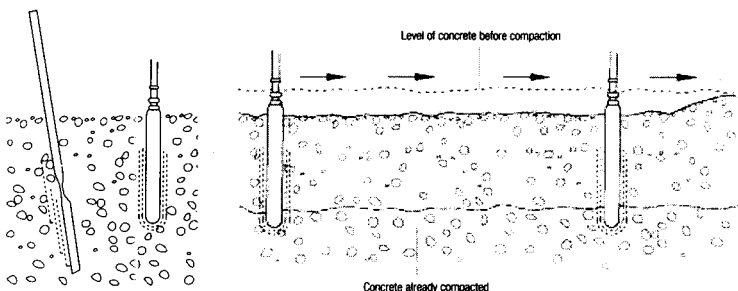
Figs 19 and 20: Compacting with a rod (punning) (left) and a poker vibrator (right)
