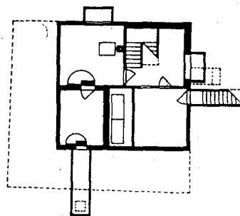
Fig. 99: Plan of basement
