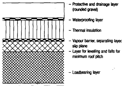
Fig. 4: Flat roof without ventilation (warm deck) not accessible
