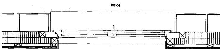
Plan of course 1
