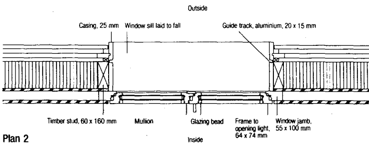
Plan 2
