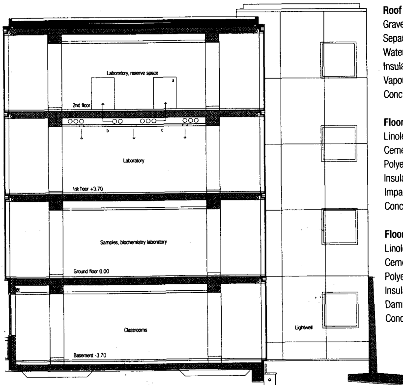
Fig. 244: Section The stacked concrete "platforms" and staircase tower, which in the basement is coupled with the lightwell. a) Laboratory benches/media supply points; b) horizontal media zone/distribution; c) lighting unit
