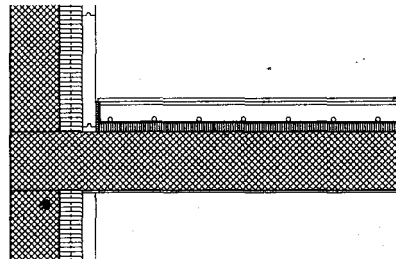
Fig. 36: Construction detail
