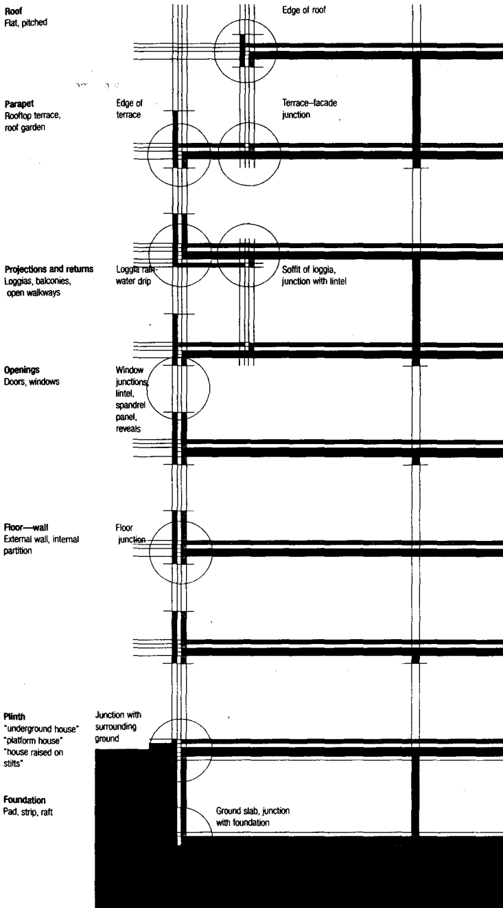
Fig. 17: Diagram of layers, loadbearing layer outside
