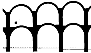
Fig. 69: Ghorfa type B Section, 1:200
