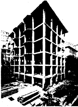
Fig. 5: The skeletal frame
