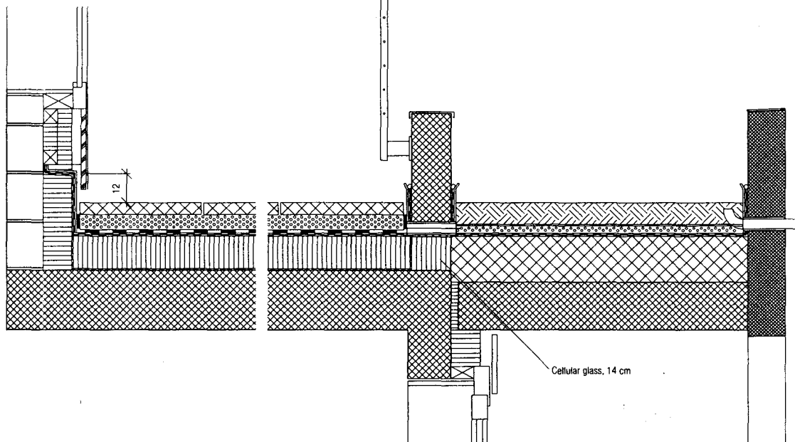
Warm deck, suitable for foot traffic, terrace
