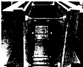
Fig. 14: Timber formwork with formwork ties
