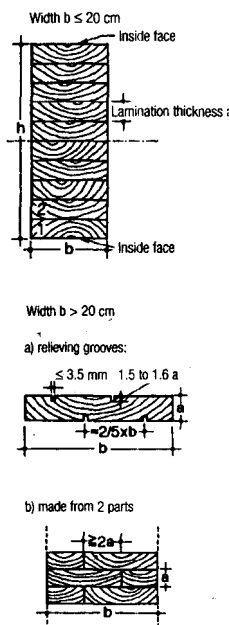
Fig. 13: Lay-up of glued laminated timber (glulam)
