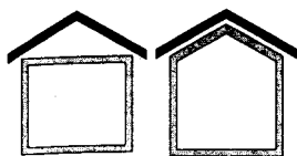
Fig. 38: Cold deck pitched roof cold roof space (screed)
