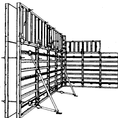
Fig. 17: Steel wall forms
