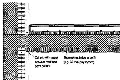
Fig. 37: Construction detail
