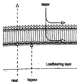
Fig. 12: Schematic drawing of building performance parameters
