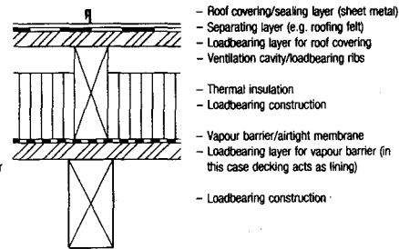
Fig. 3: Pitched roof without secondary waterproofing/covering layer (cold deck)
