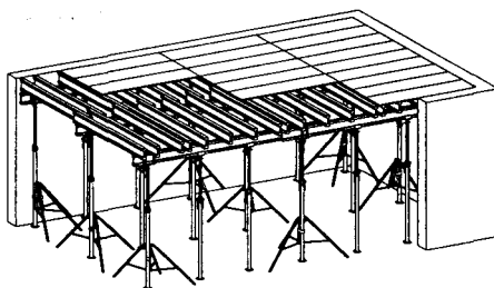
Fig. 16: Table form for floor slab
