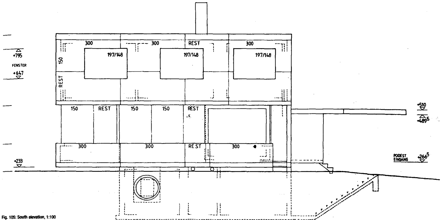
Fig. 105: South elevation, 1:100
