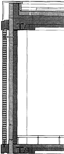
Fig. 79: Section through prefabricated facade element Swisscom headquarters, Winterthur (CH)
