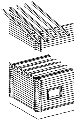
Fig. 43: Log construction
