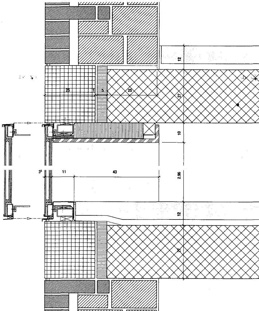
Fig. 56: Section, 1:10
