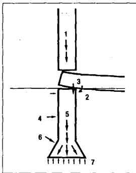
Fig. 44: Load transfer
