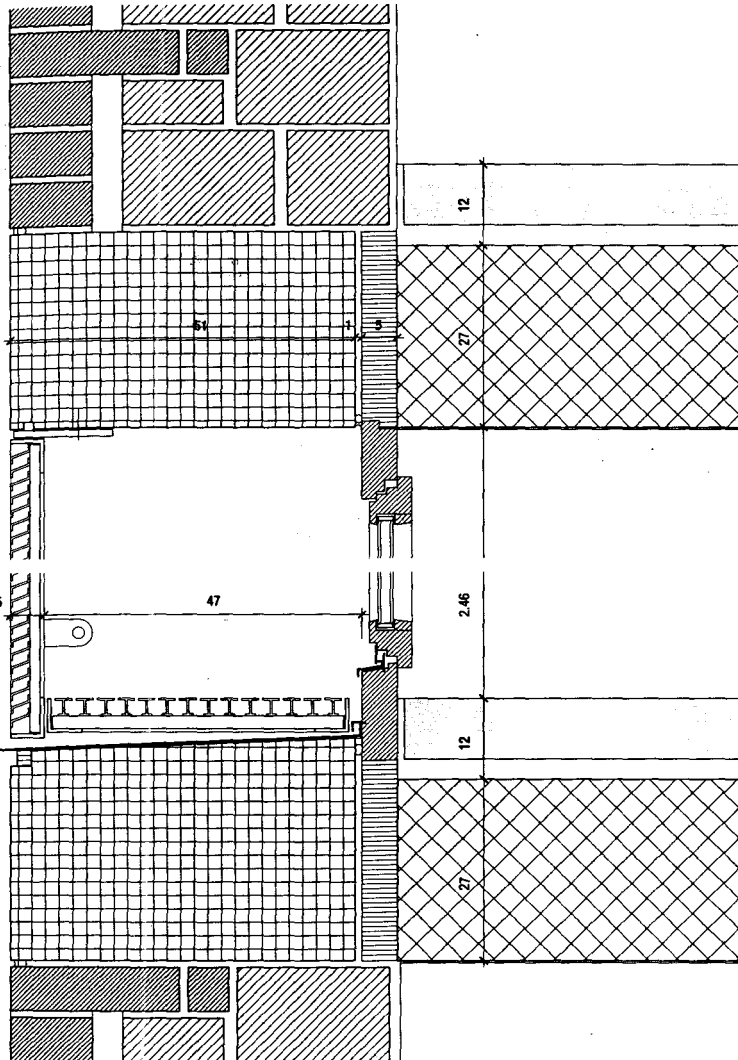
Fig. 53: Section, 1:10
