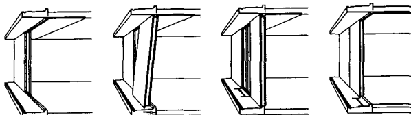
Fig. 1: Erection and fixing of a facade element
