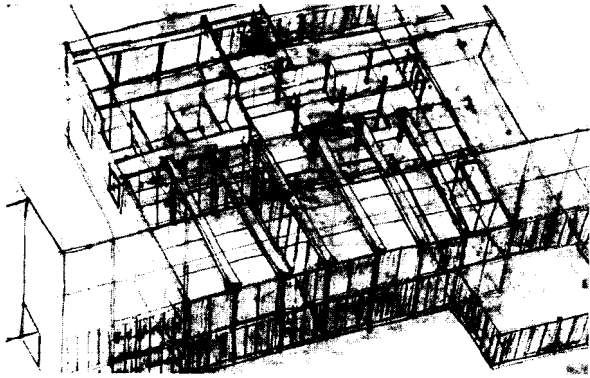
Fig. 212: Isometric view Checking the room layout and loadbearing structure around the music room, dining hall and library (sketch)
