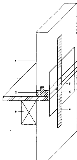
Fig. 26: Homogen80, detail of wall-floor junction
