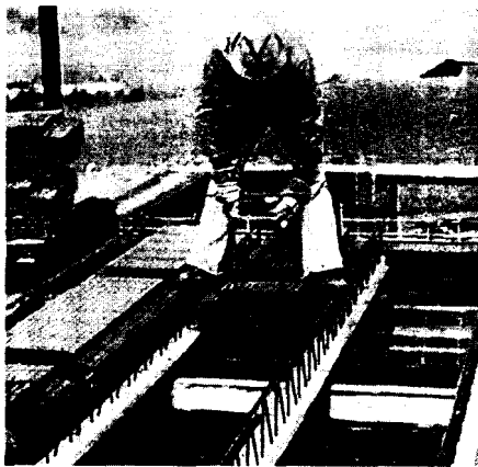
Fig. 2: Fitting the individual Hourdis-type elements between the reinforced concrete beams
