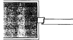
Fig. 65: Frame in opening, centred in reveal (internal and external doors) rebated door leaf
