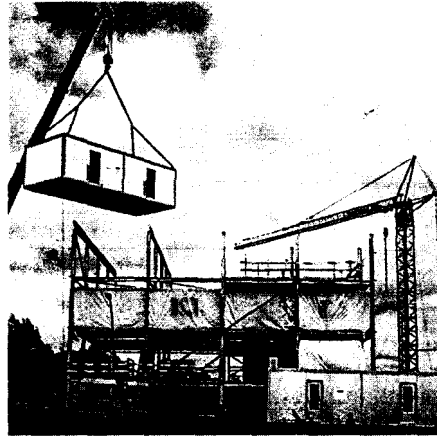
Fig. 126: Container (e.g. as meeting room) supported on steel frame Dollmann + Partner: office building, Fellbach (D), 1999
