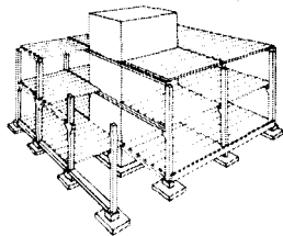
Fig. 55: Principle of a multi-storey framed building using precast concrete columns, beams and floor elements. The in situ concrete core stabilises the building by resisting the horizontal forces.
