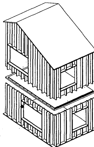
Fig. 42: Panel construction
