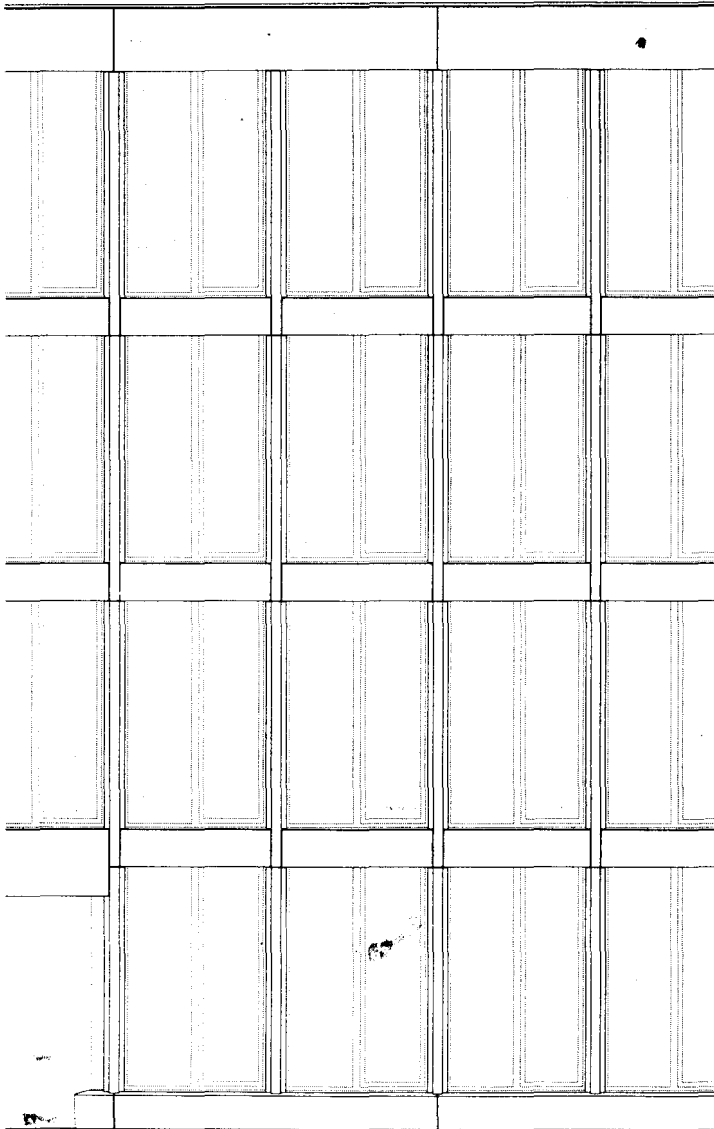
Fig. 219: Elevation, 1:50
