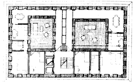
Fig. 102: Plan of standard floor Catherine Gay: Towers at Kreuzplatz, Zurich (diploma thesis, ETH Zurich), 1999
