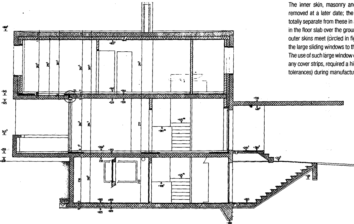
Fig. 103: Section A-A, 1:100 1:50 working drawing (reduced)
