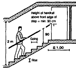
③ Favourable standard rise/going ratio 17/29; step length = 2 going + 1 rise = approx. 62.5 cm
