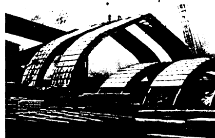
Fig. 121: Erection of prefabricated half-shells Salt warehouse
