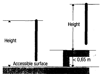
Fig. 25: Height of safety elements
