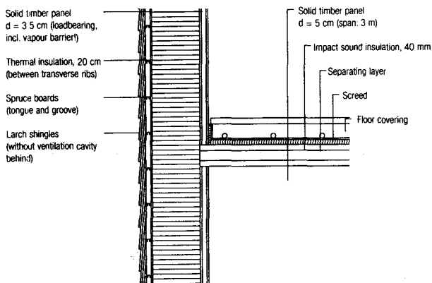
Fig. 4: Section through wall-floor junction Beath & Deplazes: private house (Beath-Candinas), Sumvitg (CH), 1998
