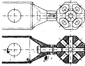
Fig. 67: "Mero" node with member attached Elevation and section
