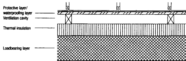
Fig. 15: Section through cold roof
