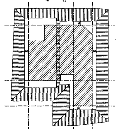
Fig. 42: Schematic plan of excavation (showing sloping sides)
