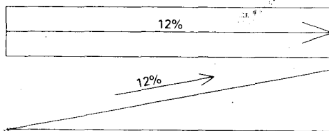
Fig. 3. Indicating an incline on plan and in section
