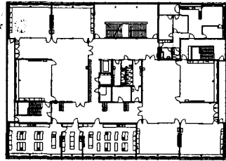
Fig. 205: Plan of 2nd floor
