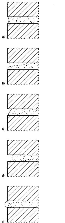
Fig. 34: Examples of jointing a) Bucket handle b) Flush c) Weathered (non-facing side of masonry partially exposed to weather) d) Recessed (non-facing side of masonry partially exposed to weather) e) Protruding (joint material severely exposed to weather)
