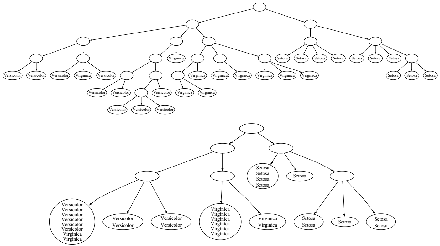
FIGURE 4.21 Hierarchical clusterings of the iris data.
