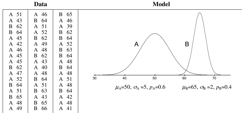
FIGURE 9.5 A two-class mixture model.
