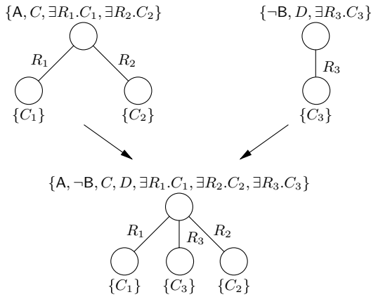
Fig. 9.5. Joining expansion trees for A and \neg B .
