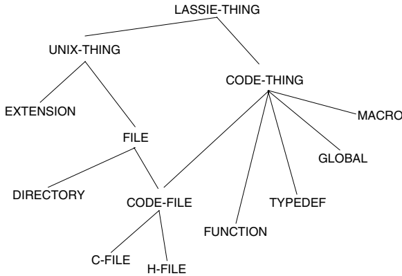
Fig. 11.1. The Lassie code-level ontology.
