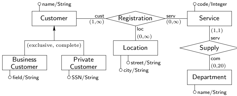
Fig. 4.8. An Entity-Relationship schema.
