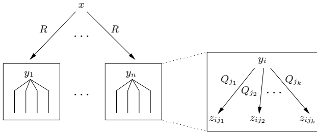
Fig. 3.1. The AND-tree structure of the tableau obtained by applying rules for \sqcap and \exists R.C to D_1 \sqcap D_2 \sqcap D_3(x) . Applying the rule for \leq 2 R(x) would lead to several OR-branches (as many as the possible identifications of ys ).
