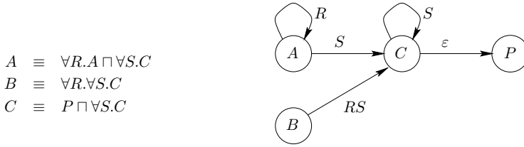
Fig. 2.7. A TBox and the corresponding automaton.
