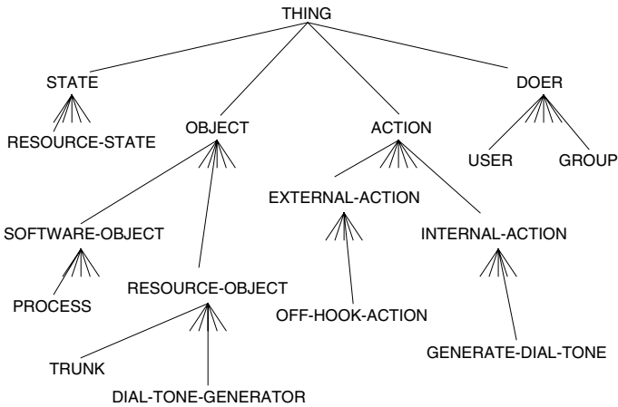
Fig. 11.2. The Lassie telephony ontology.
